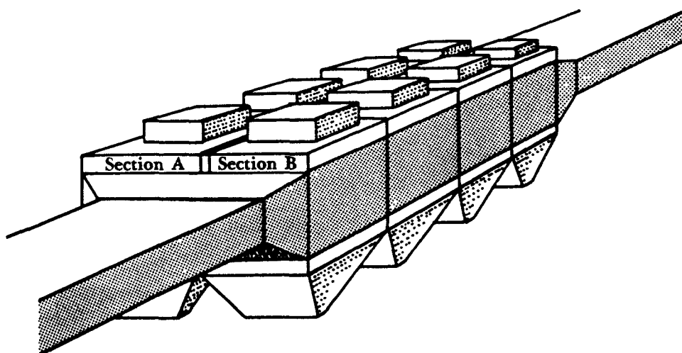
Figure 8-8. Chambers of a Precipitator.
