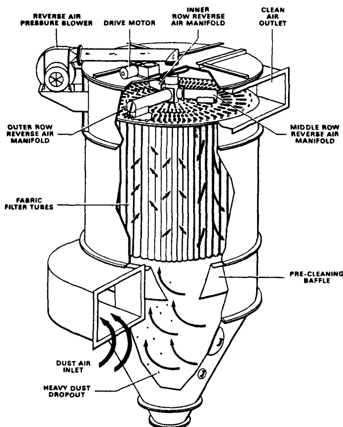
Figure 8-4. Reverse Air Fabric Filter (Outside-to-Inside Flow).
