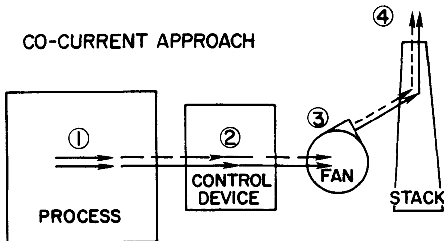
Figure 8-2. Co-Current Inspection Approach.
