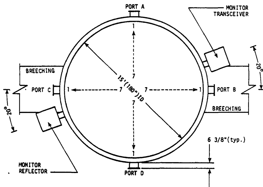
FIGURE 4-7. PST REPORT RECOMMENDED FORMAT: MONITOR LOCATION SCHEMATIC
