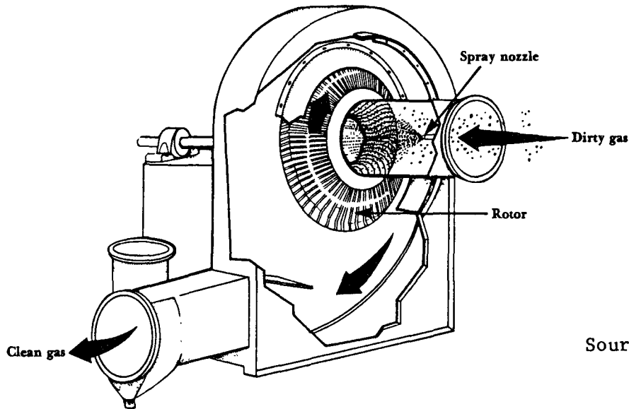
Figure 8-14. Mechanically Aided Scrubber.
