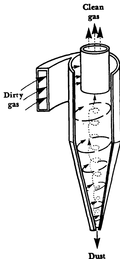
Figure 8-17. Large Diameter Cyclone.
