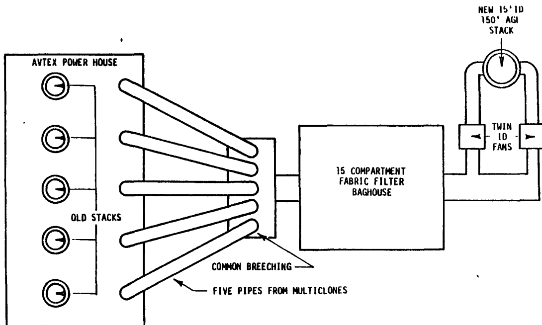
FIGURE 4-6. PST REPORT RECOMMENDED FORMAT: PLANT SCHEMATIC
