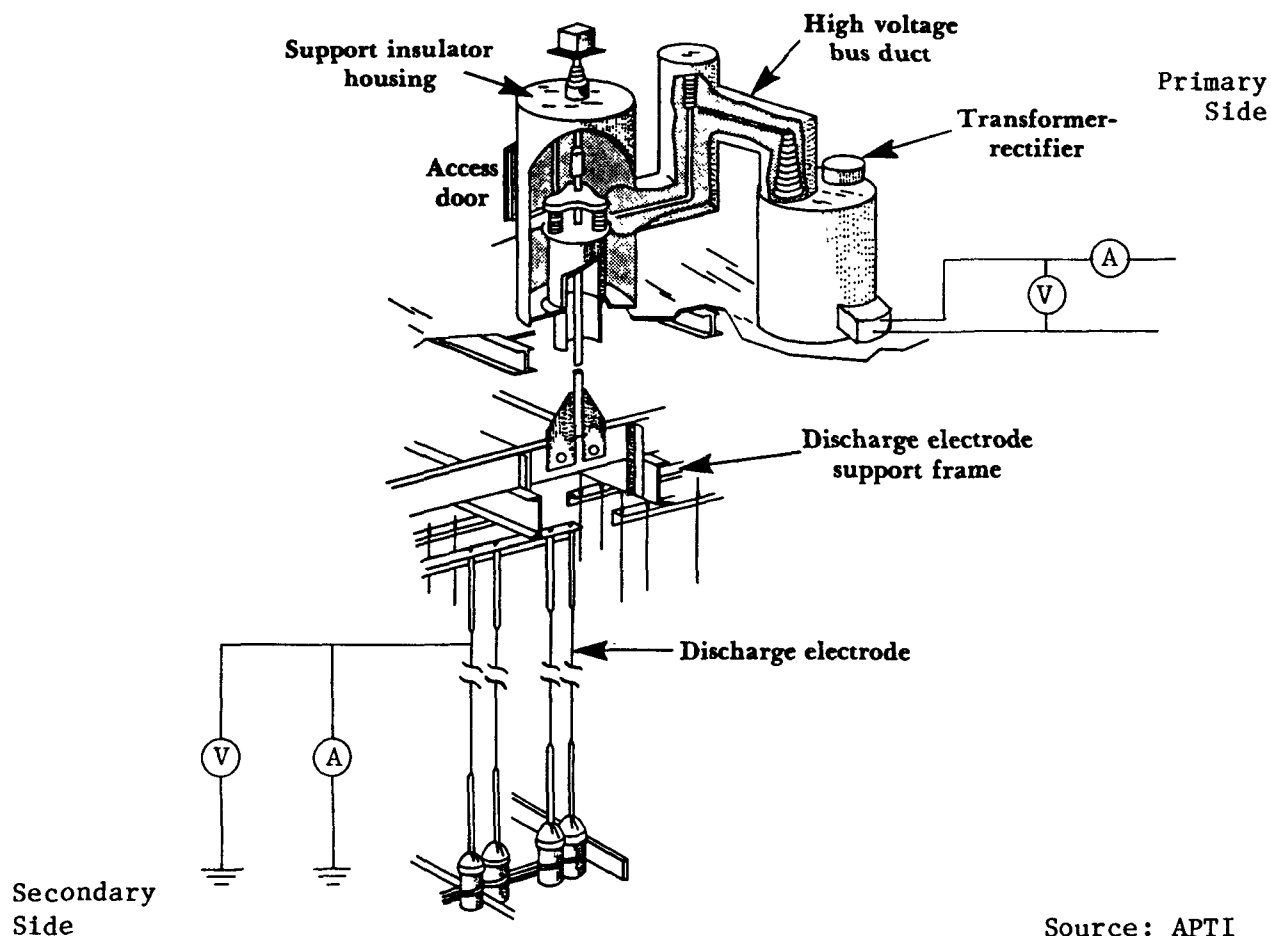
Figure 8-9. Field Electrical Conditions.
