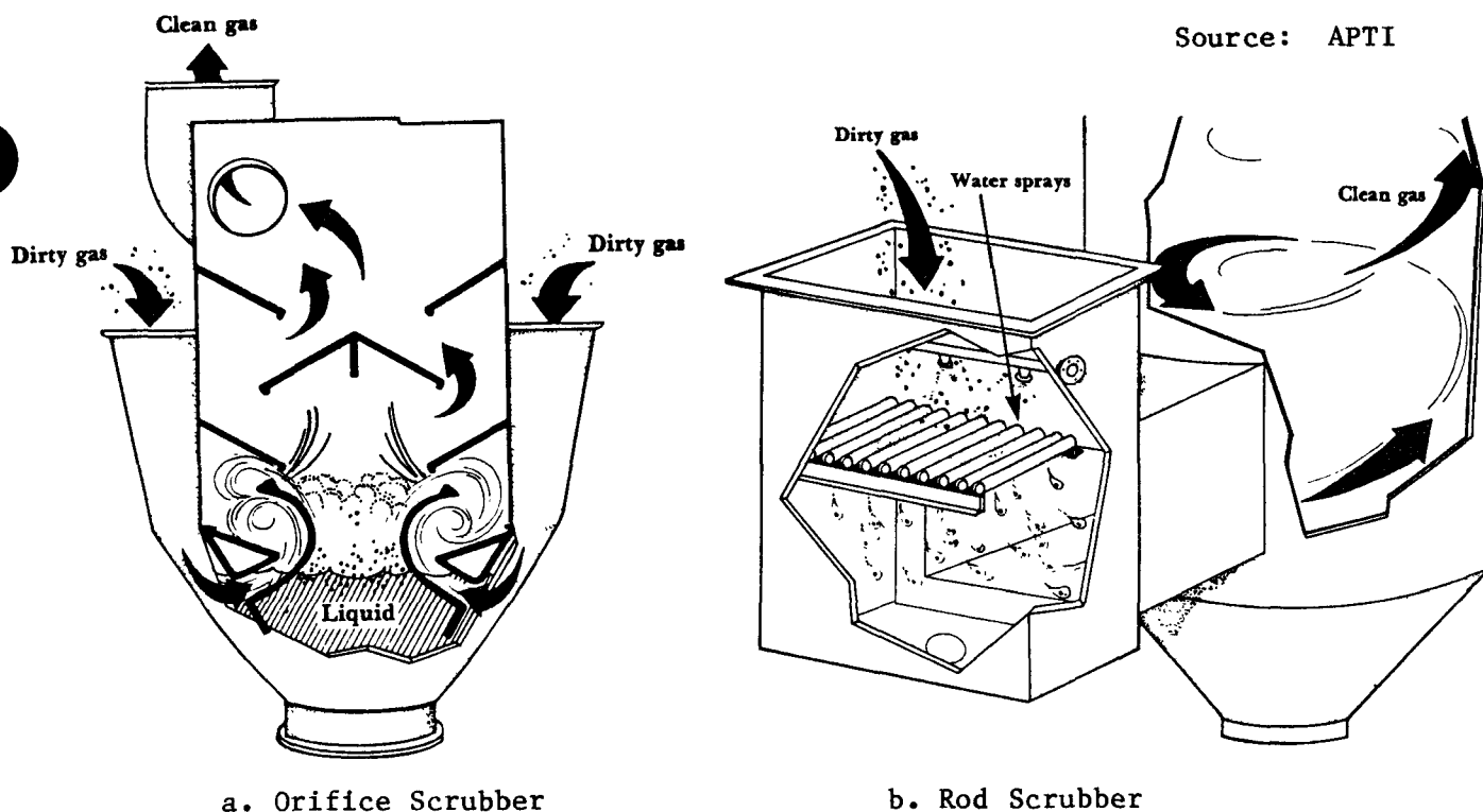
Figure 8-16. Gas-Atomized Scrubbers.
