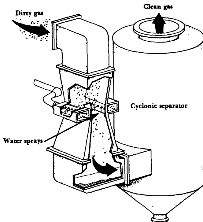
Figure 8-15. Venturi Scrubber.
