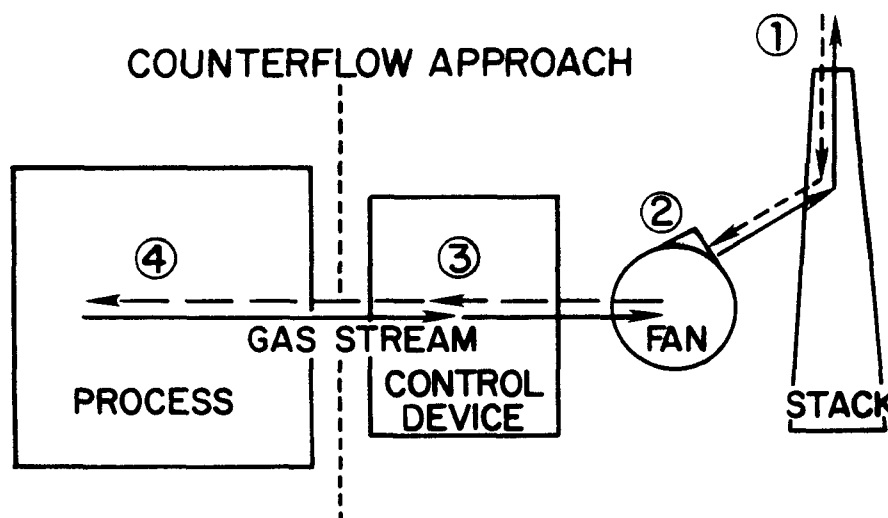
Figure 8-1. Counterflow Inspection Approach.
