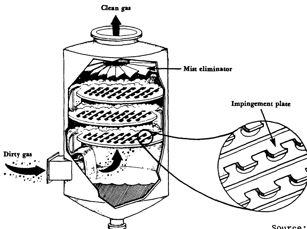
Figure 8-13. Tray Tower Scrubber.
