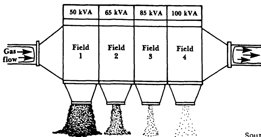
Figure 8-7. Fields in Series.
