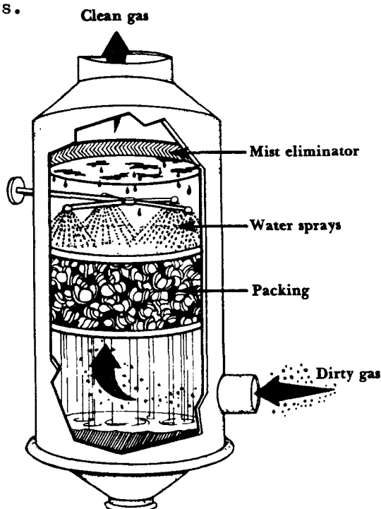
Figure 8-11. Packed Bed Scrubber.
