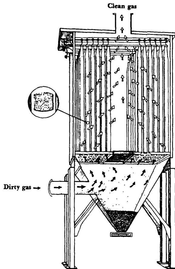
Figure 8-6. Shaker Fabric Filter.
