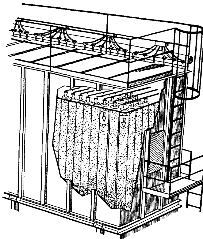
Figure 8-3. Sketch of a Pulse Jet Fabric Filter.
