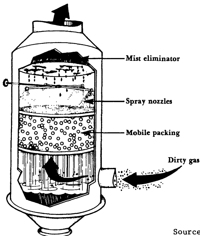
Figure 8-12. Moving Bed Scrubber
