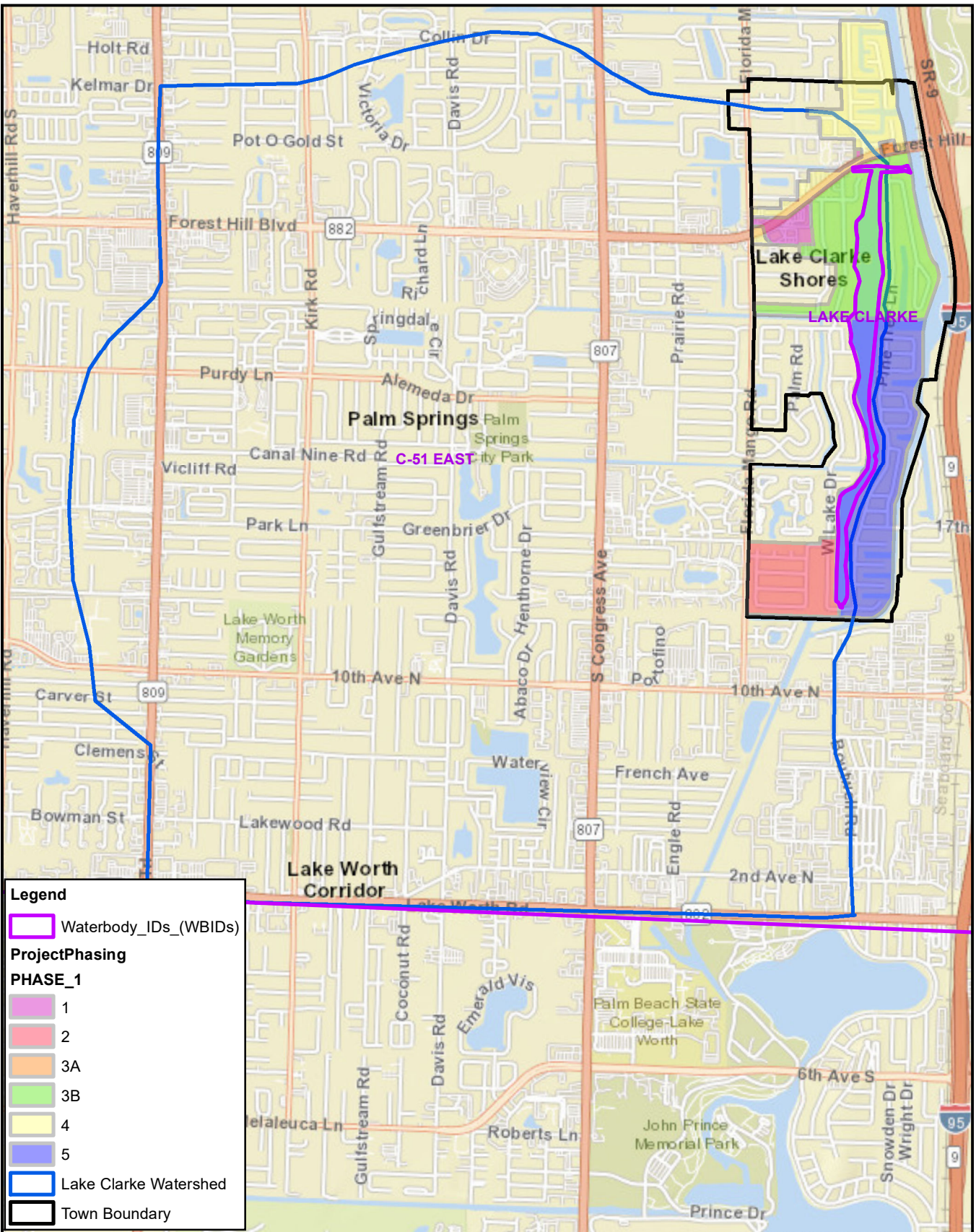
Watershed Boundary and Proposed Improvement Areas
