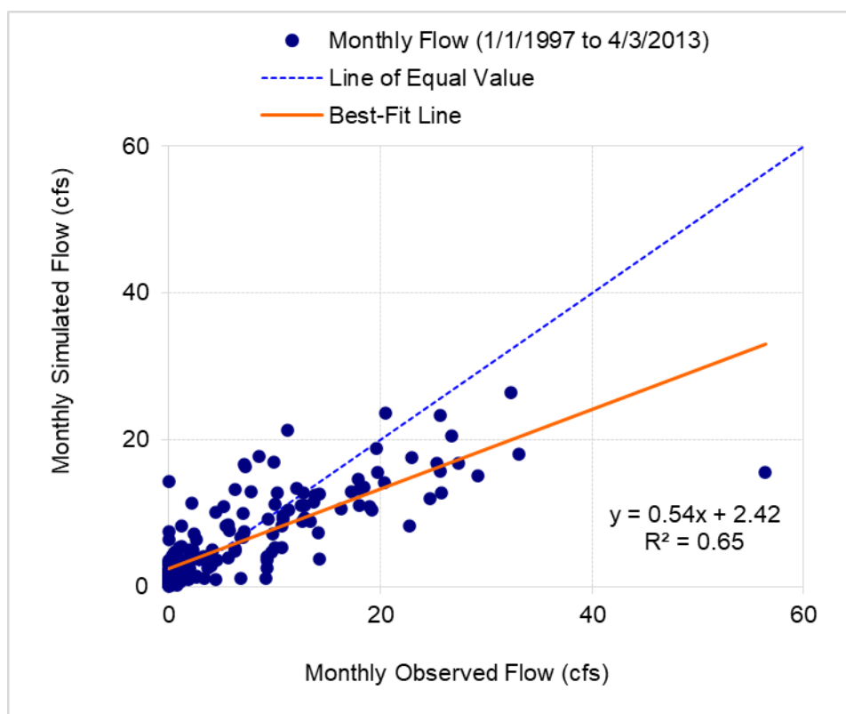
Figure A-91. Monthly flow regression and temporal variation: Model output at Reach 107 versus USGS 02293241 San Carlos Canal at Cape Coral (01/01/1997 – 04/03/2013)
