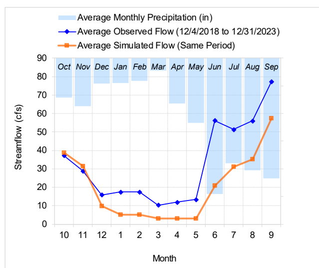
Figure A-104. Seasonal regression and temporal aggregate: Model output at Reach 186 versus USGS 02292490 Goodno Canal Below S-78 Near Labelle, FL (12/04/2018 – 12/31/2023)
