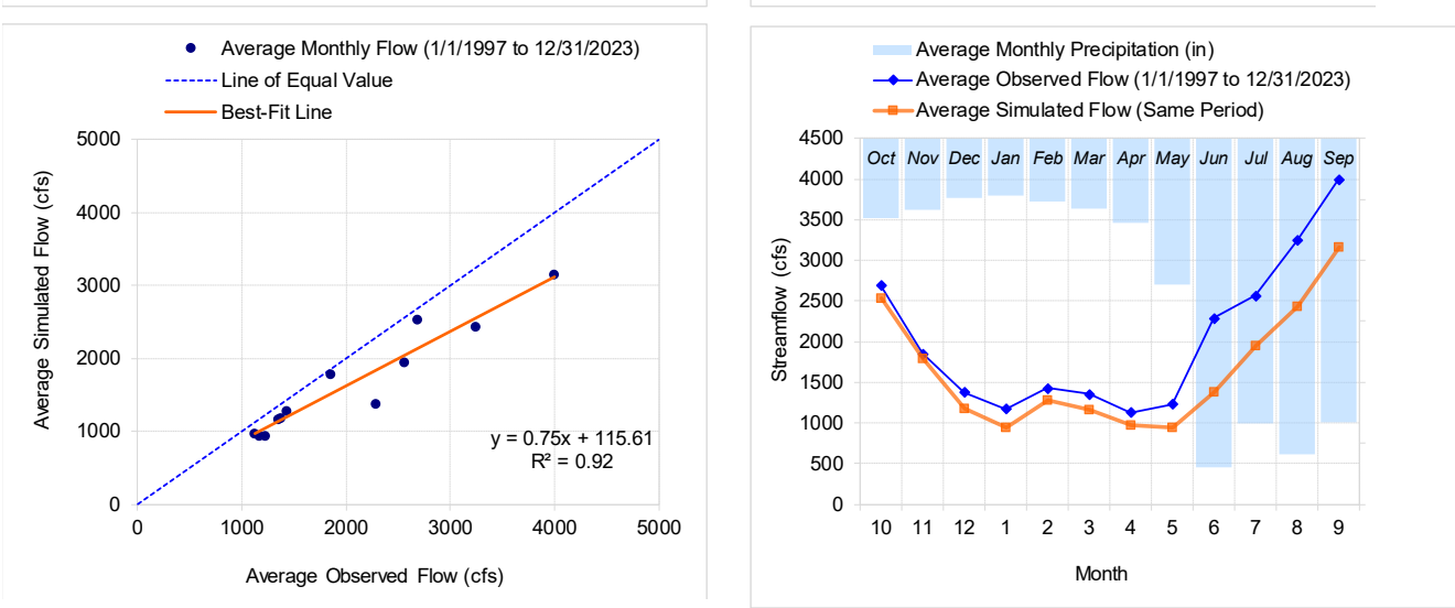
Figure A-43. Seasonal regression and temporal aggregate: Model output at Reach 147 versus USGS 02292900 Caloosahatchee River at S-79 near Olga, FL (01/01/1997 – 12/31/2023)
