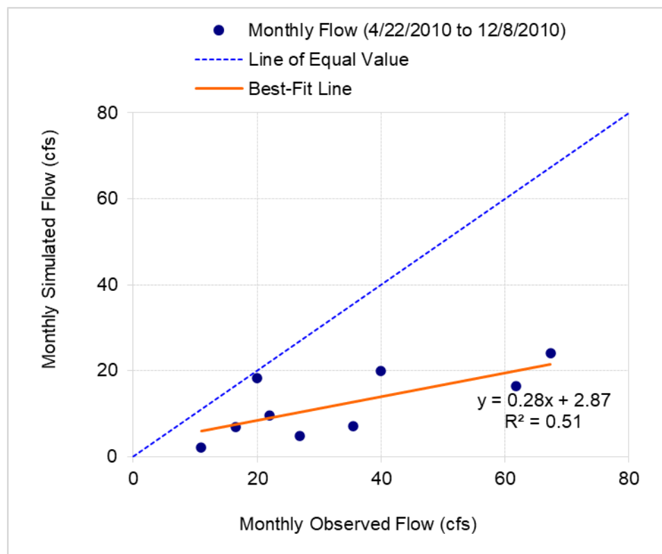
Figure A-138. Monthly flow regression and temporal variation: Model output at Reach 173 versus DEP Fast Creek at SR 80 (04/22/2010 – 12/08/2010)
