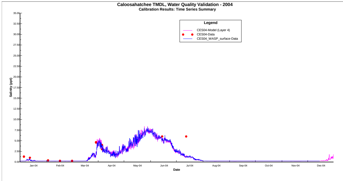
006_Salinity_CES04__Surface
