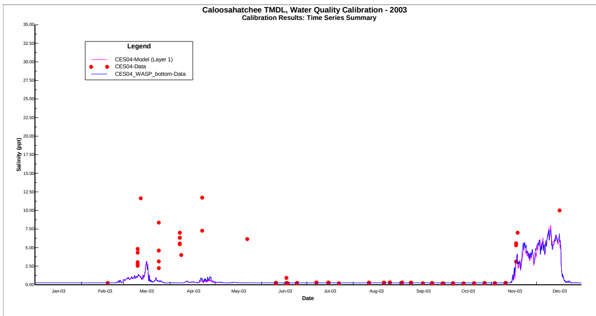
Salinity_CES04_Bottom
