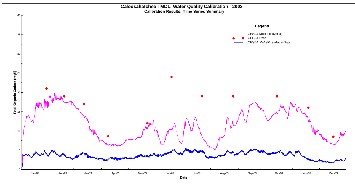
107_TOC_CES04_Surface
