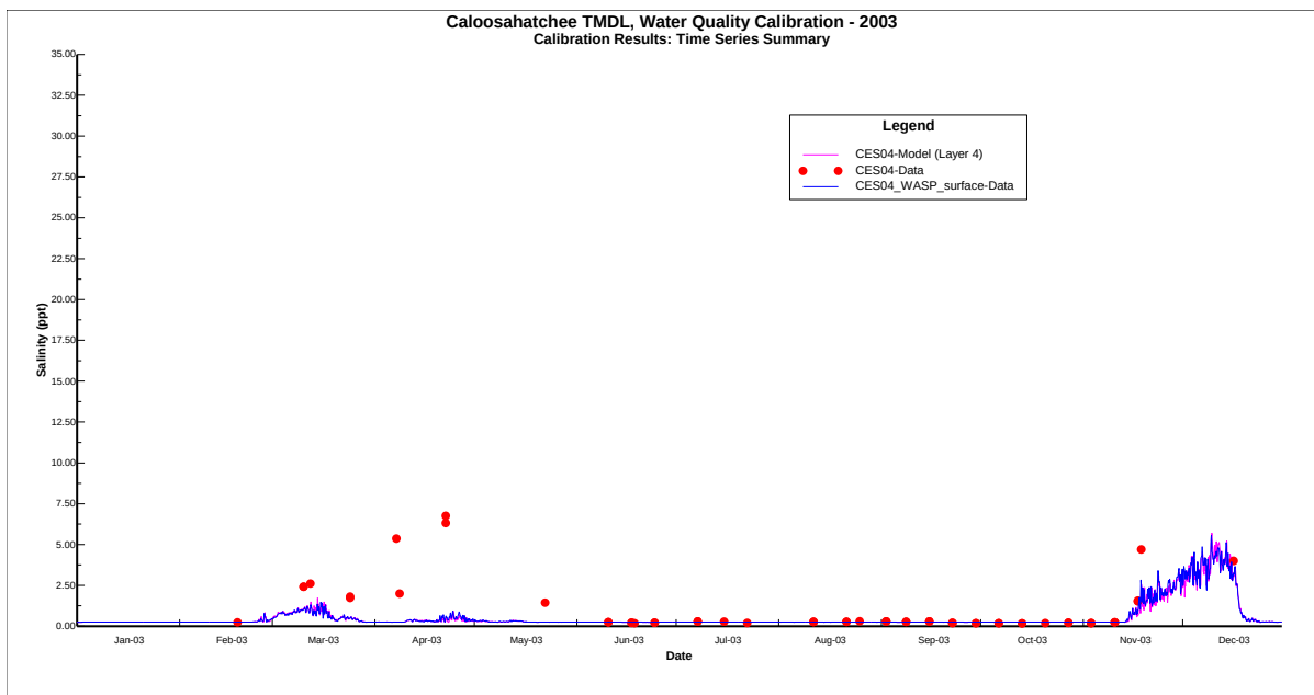
Salinity_CES04 Surface
