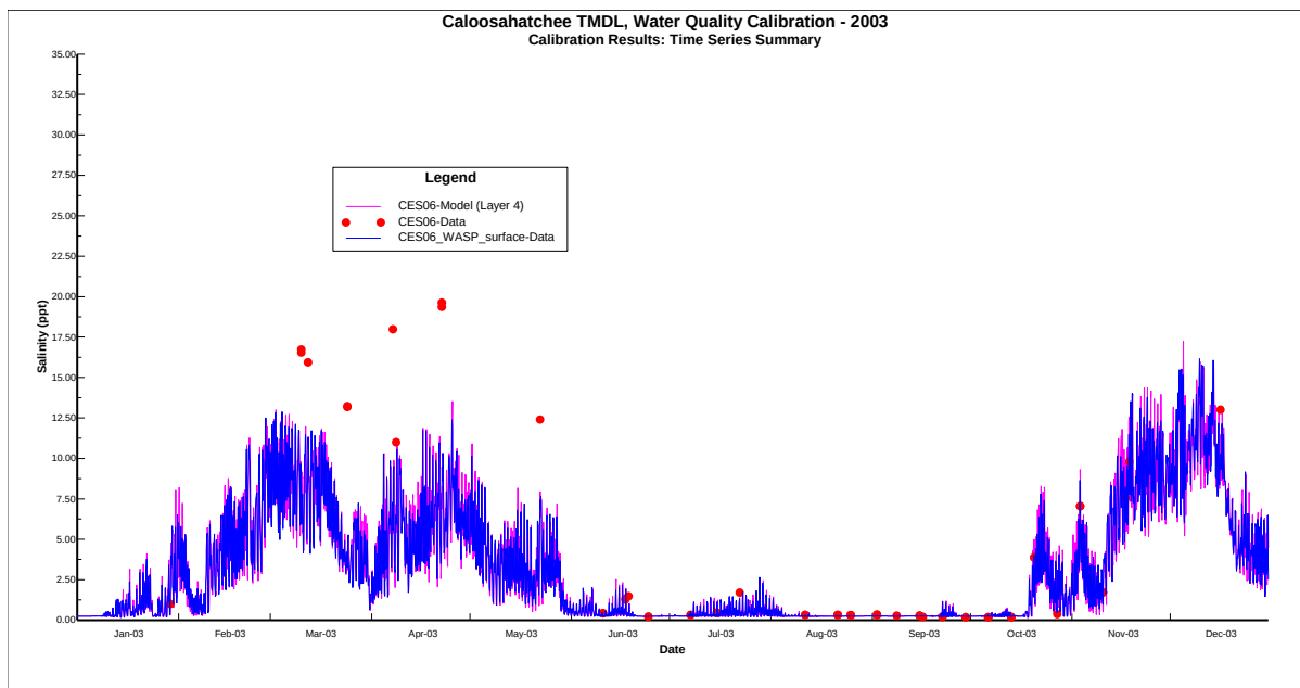
Salinity_CES06_Surface
