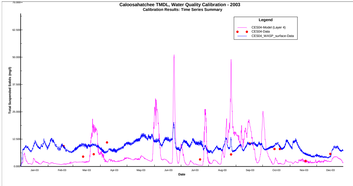
115_TSS_CES04_Surface
