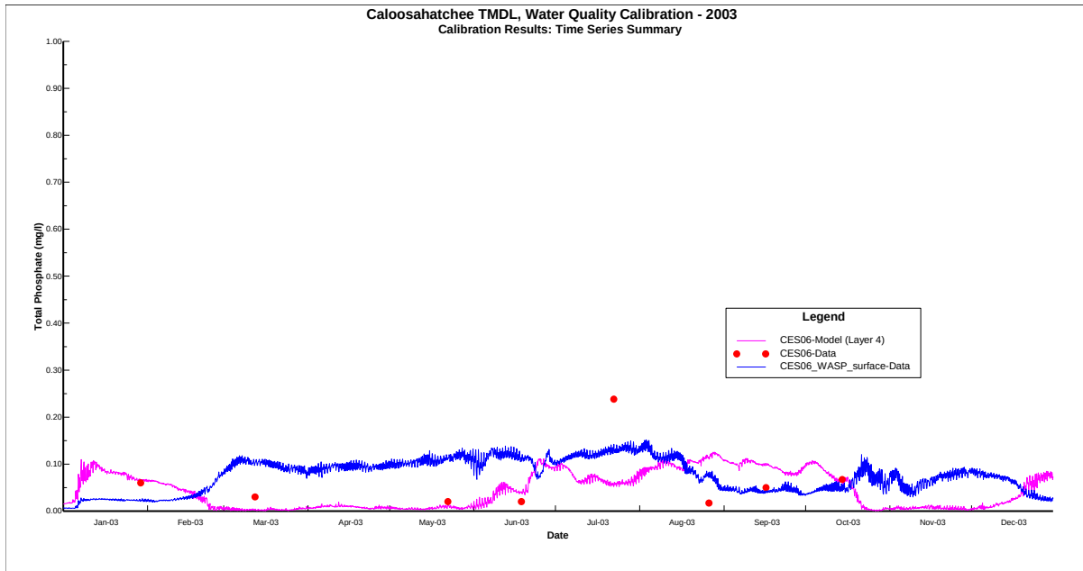
077_TPO4-P_CES06_Surface
