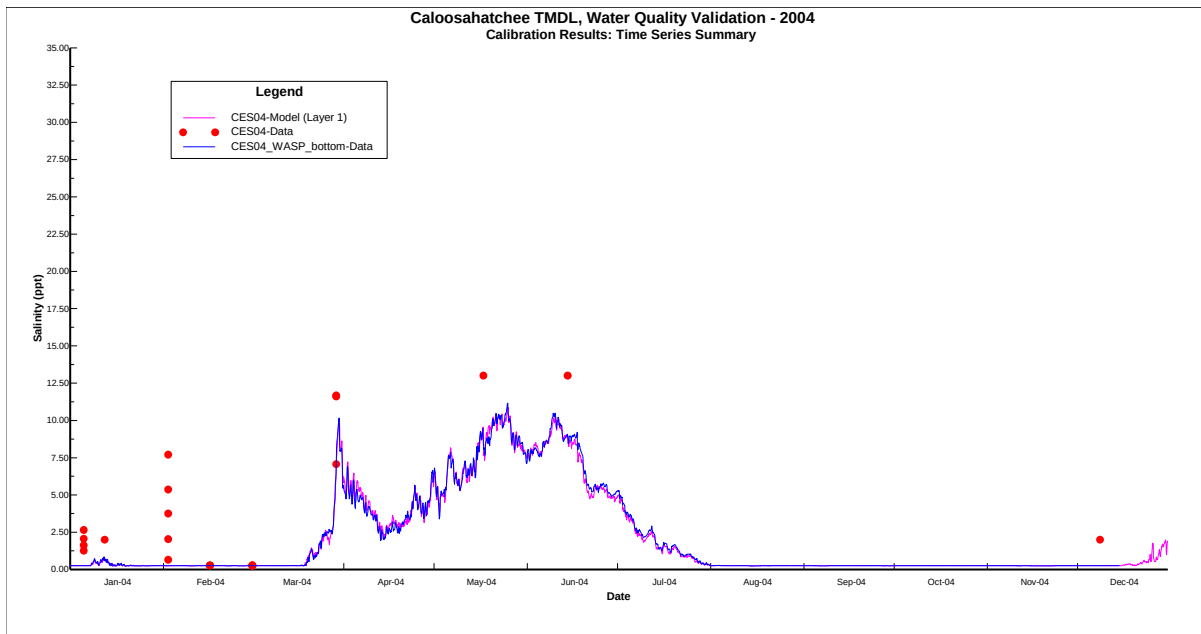
007_Salinity_CES04__Bottom
