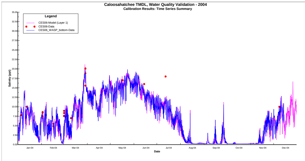
011_Salinity_CES06__Bottom
