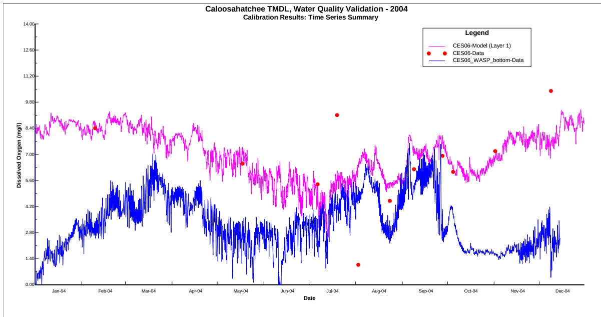
053_DO_CES06__Bottom
