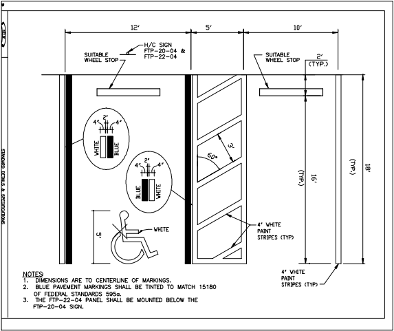
CITY PARKING DETAIL
