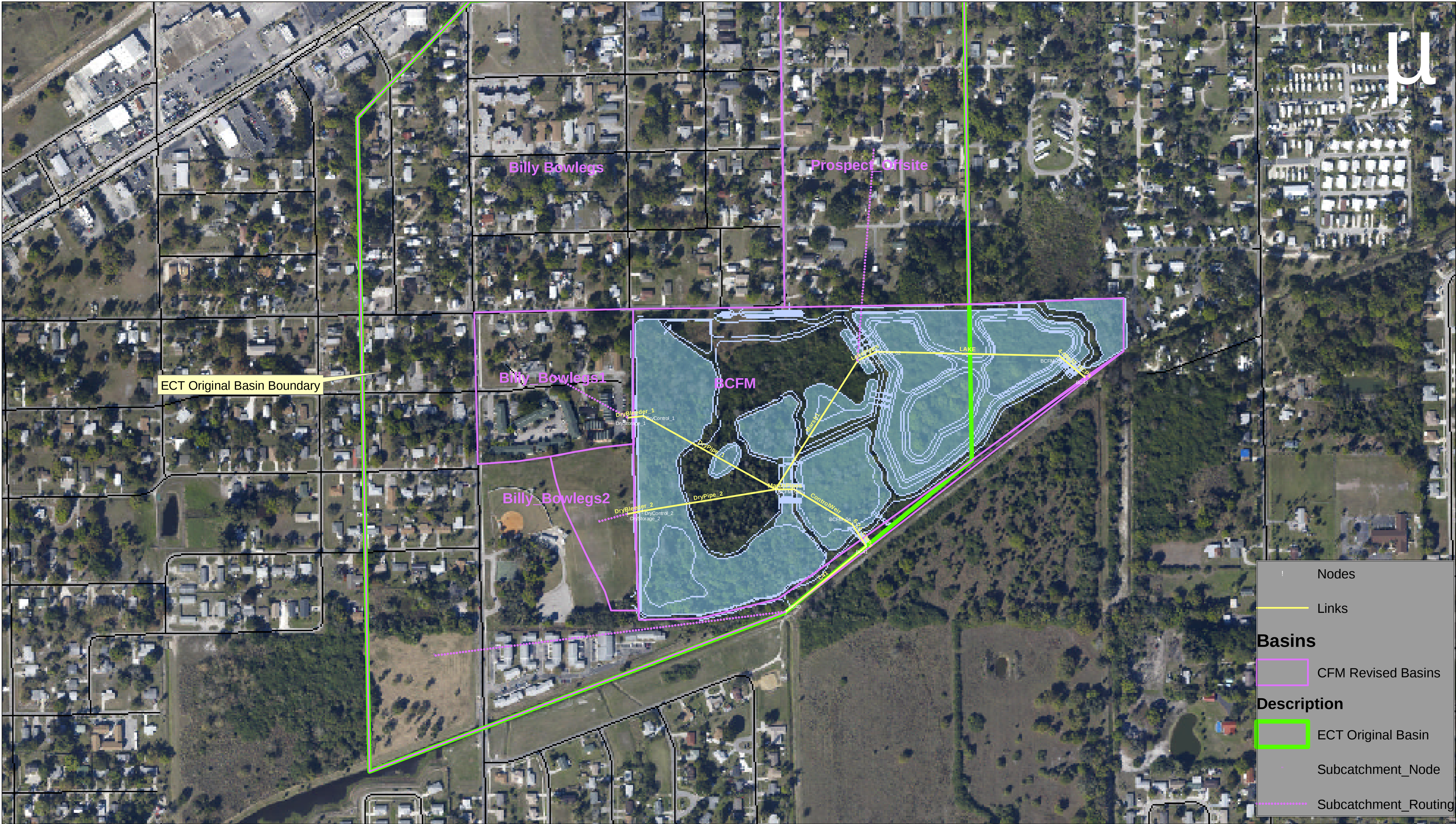
Billy Creek Filter Marsh - Node/Link Diagram EXHIBIT B-1
