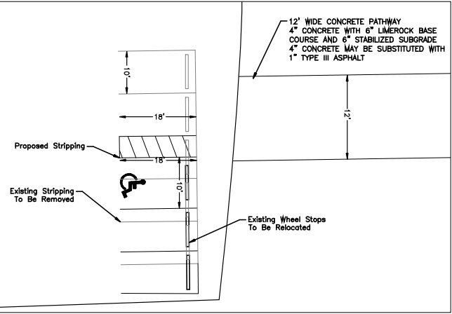
PARKING LOT AREA SCALE: 1' = 40'
