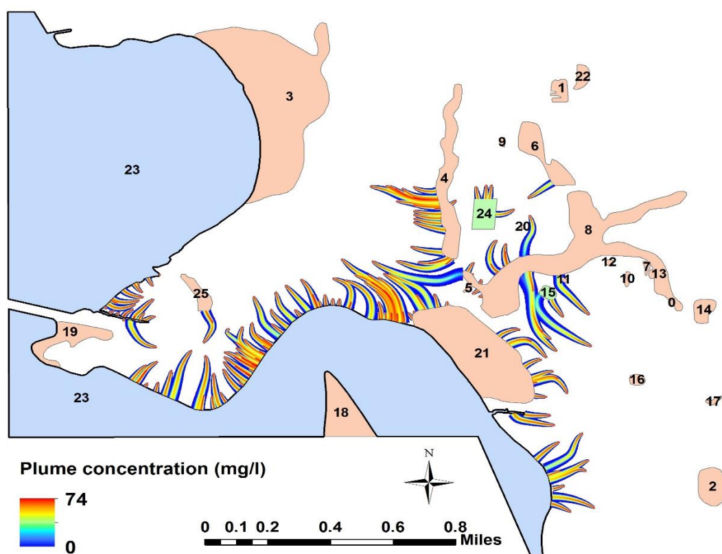
Figure 4-4. Simulated flow paths from septic systems to surface waterbodies. Parameter values specific to Case 3 are \alpha_L = 2.134 m, \alpha_T = 0.0549 m, and k = 0.001 d -1 .
