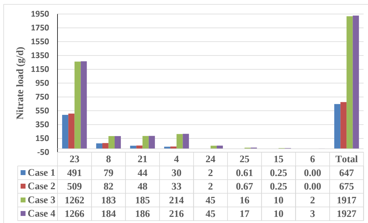
Figure ES-2. Nitrogen loading (g/d) to the individual waterbodies for the four modeling cases.
