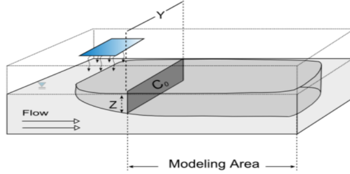
Figure 2-1. Conceptual model of nitrate transport in groundwater adapted from Aziz et al. (2000). The unsaturated zone is bounded by the rectangular box delineated by the dotted lines; the groundwater zone is bounded by the box delineated by the solid lines
