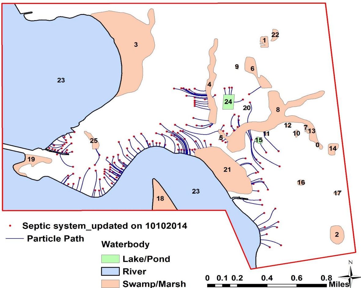
Figure 4-1. Simulated flow paths from septic systems to surface waterbodies.
