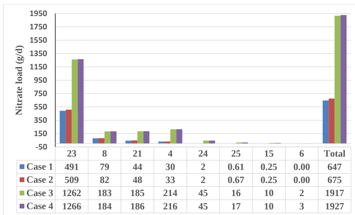
Figure 4-6. Nitrogen loading (g/d) to the individual waterbodies for the four modeling cases.
