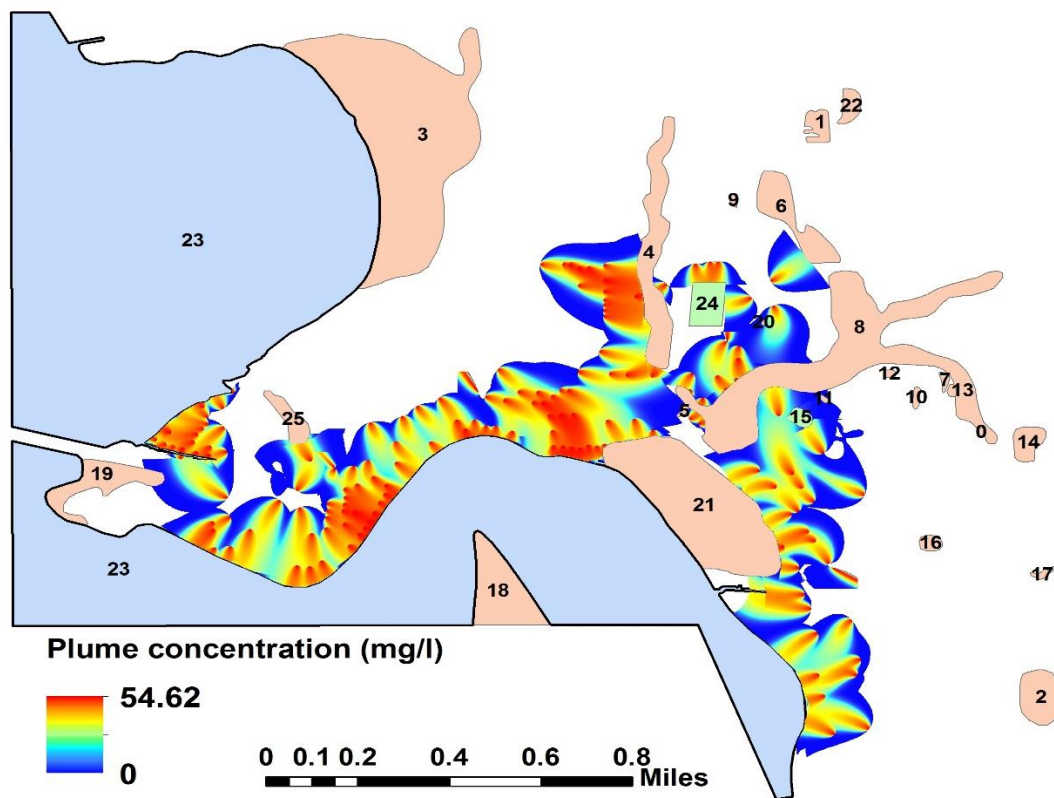
Figure 4-5. Simulated flow paths from septic systems to surface waterbodies. Parameter values specific to Case 4 are \alpha_L = 6 m, \alpha_T = 2.5 m, and k = 0.001 d -1 .
