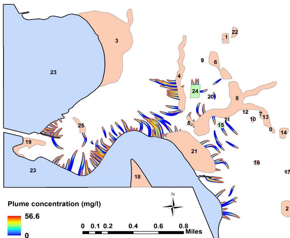
Figure 4-2. Simulated flow paths from septic systems to surface waterbodies. Parameter values specific to Case 1 are \alpha_L = 2.134 m, \alpha_T = 0.0549 m, and k = 0.011 d -1 .
