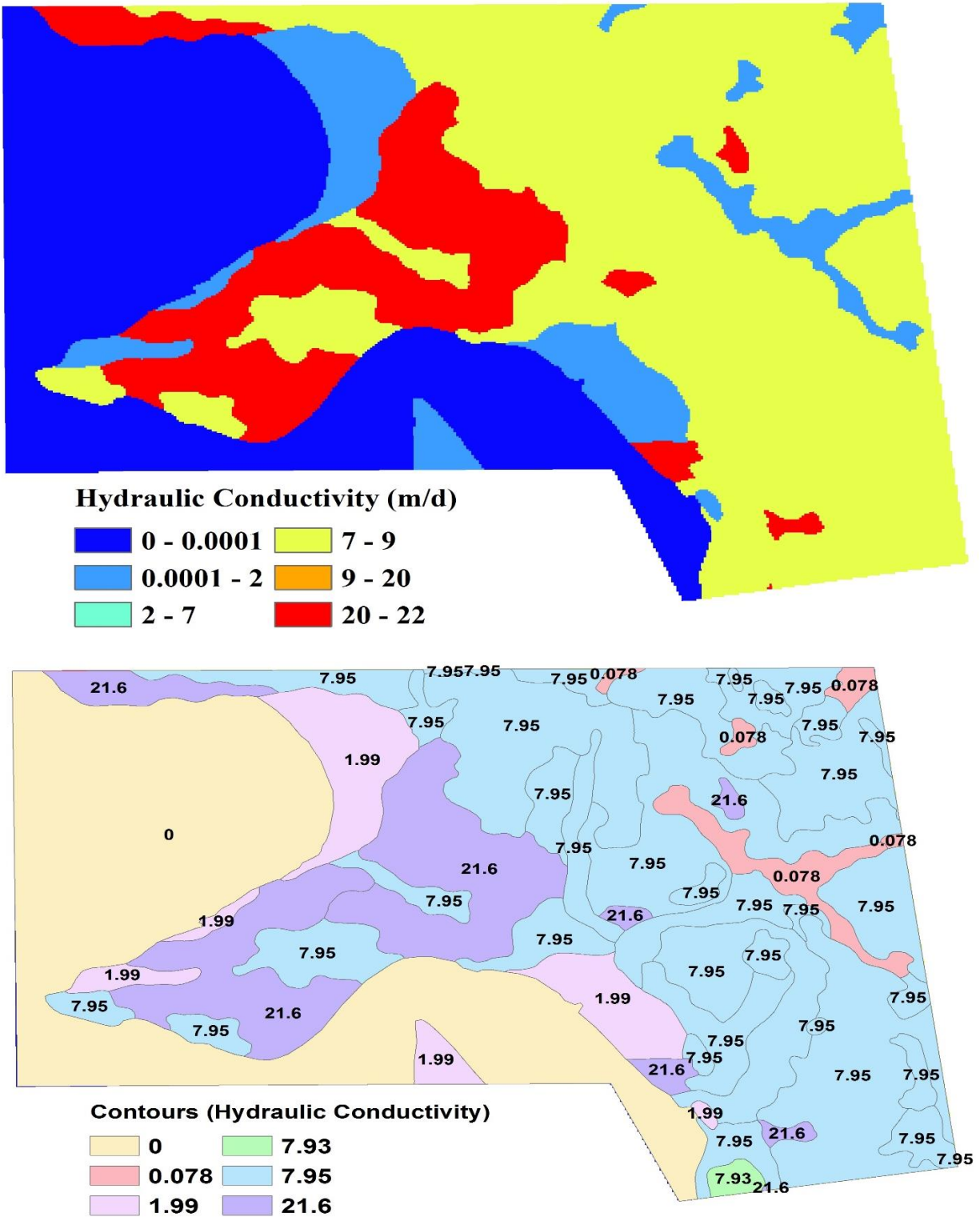
Figure 3-6. Heterogeneous hydraulic conductivity (m/d) (top) and contours (bottom) of soil units.
