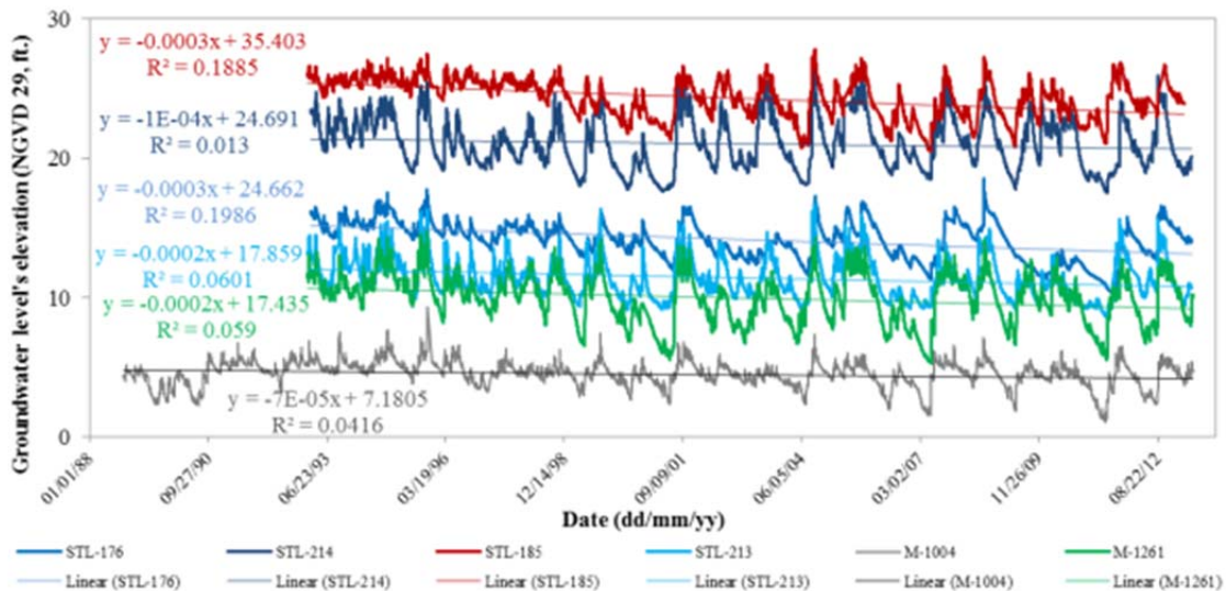
Figure 3-17. Time series of daily groundwater levels at six monitoring wells
