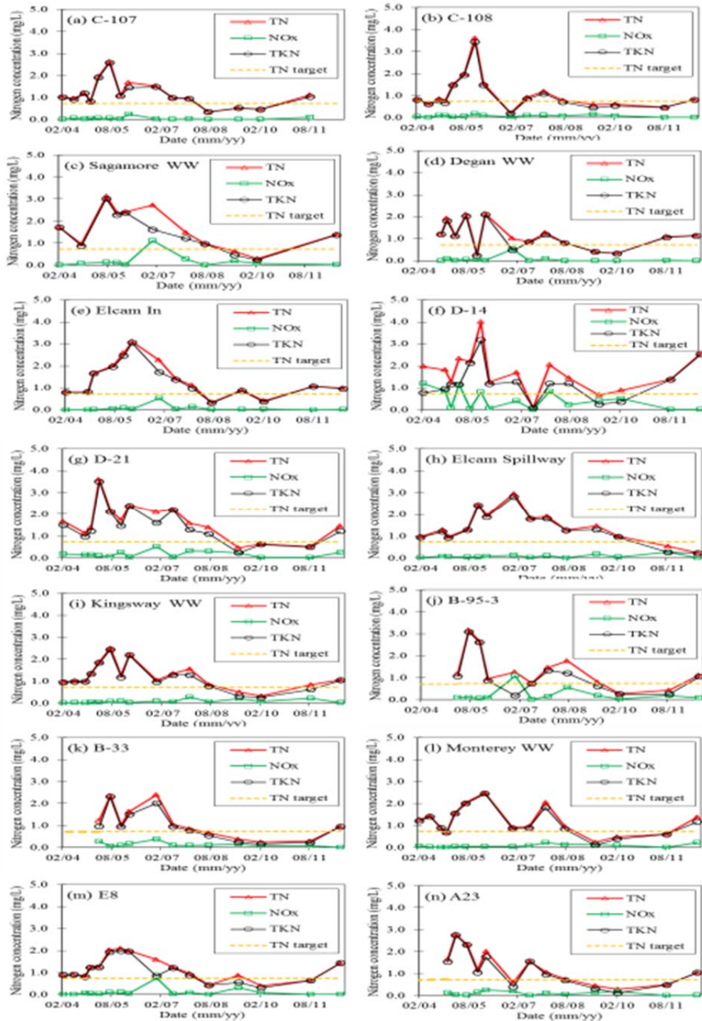
Figure 3-5. Time series of the concentrations (mg/l) of total nitrogen (TN), NOx (nitrite and nitrate), and TKN at monitoring stations of the City of Port St. Lucie. The horizontal line indicates the annual TMDL water quality TN target specified in the BMAP for the St. Lucie River and Estuary Basin (BMAP, 2013).
