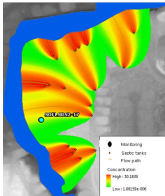
Figure 4-8. Simulated flow paths and plumes by the calibrated ArcNLET model in Martin County around well SOFLSUS2-17 (highlight in figure). Surface water bodies are plotted in blue.
