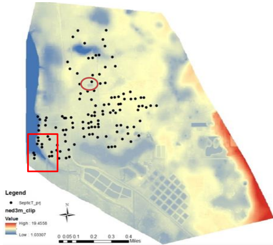
Figure 3–3. Plot of DEM maps and septic system locations. The red circle and rectangular highlight two areas where the ArcGIS layer of waterbodies (Figure 3-2) is updated to be consistent with the DEM data.
