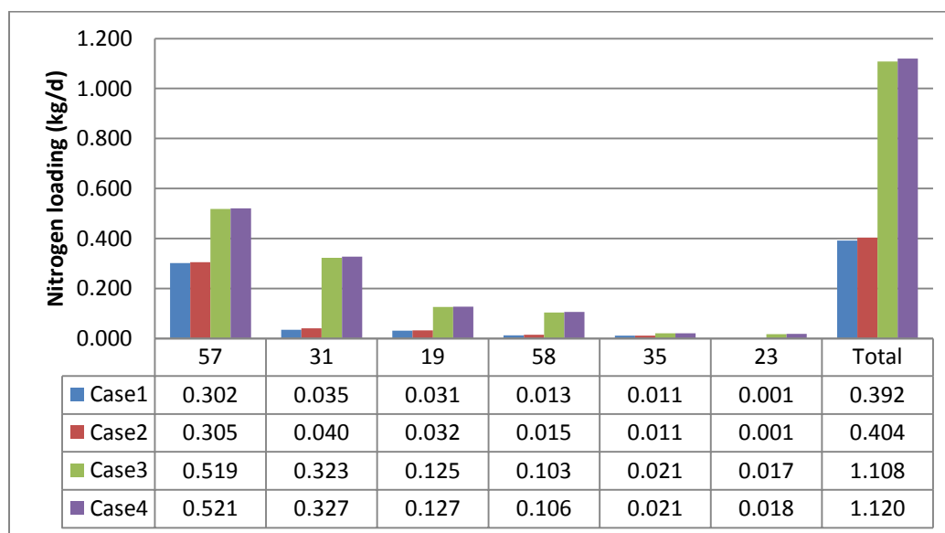
Figure ES-2. Nitrogen loading (kg/d) to the individual waterbodies for the four modeling cases.
