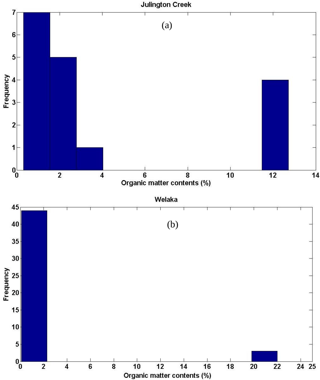
Figure 3-10. Histograms of soil organic matter contents at (a) Julington Creek area and (b) Welaka town
