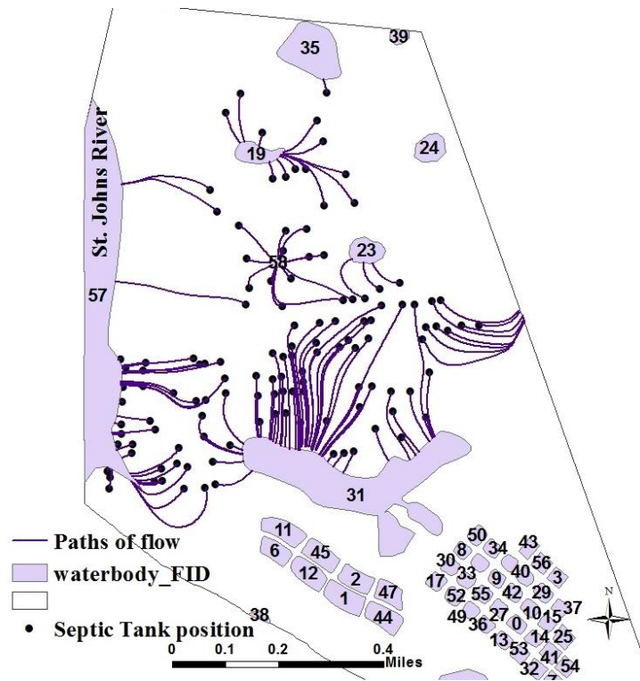
Figure ES-1. Waterbodies FID, Septic tank locations and the particle flow paths
