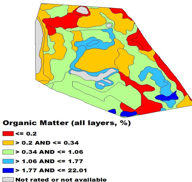
Figure 3–9. Soil organic matter contents in the Welaka town modeling area.
