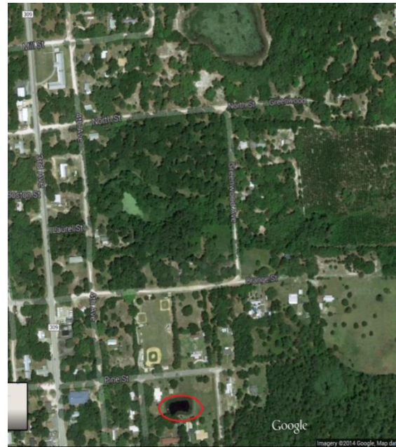
Figure 3–4. Google earth picture shows a small pond in red circle that is missing in the ArcGIS layer of waterbodies.
