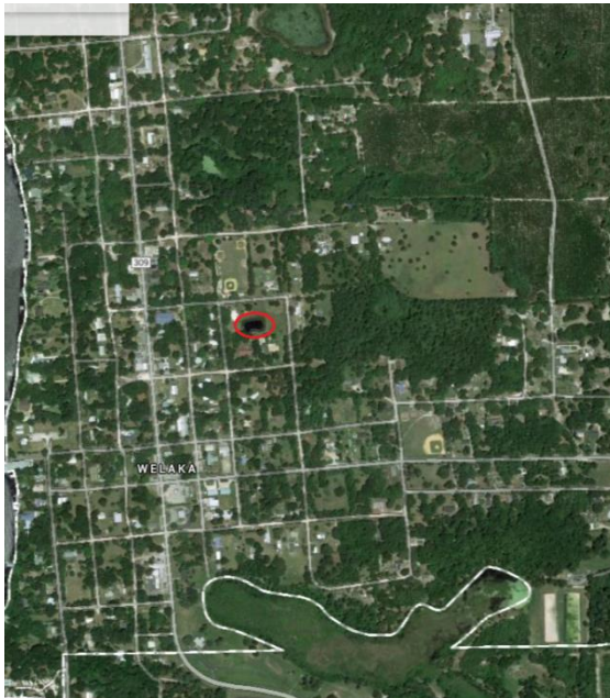
Figure 3–4. Google earth picture shows a small pond in red circle that is missing in the ArcGIS layer of waterbodies.
