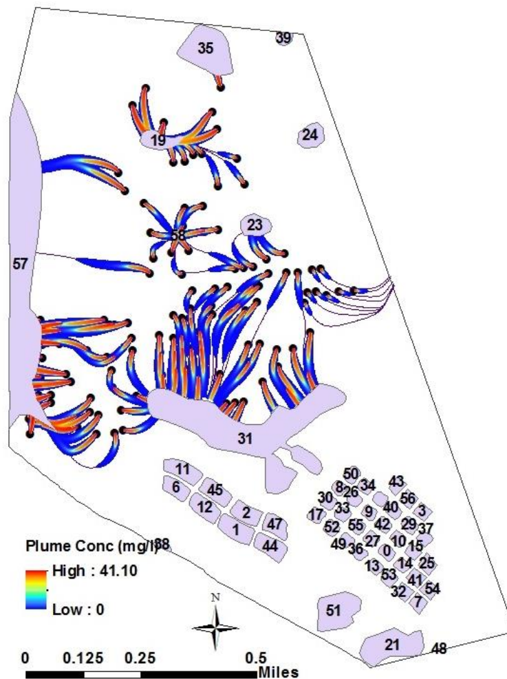
Figure 4-2. Simulated flow paths from septic systems to surface waterbodies. Parameter values specific to Case 1 are \alpha_L = 2.134 m, \alpha_T = 0.0549 m, and k = 0.011 d -1 .
