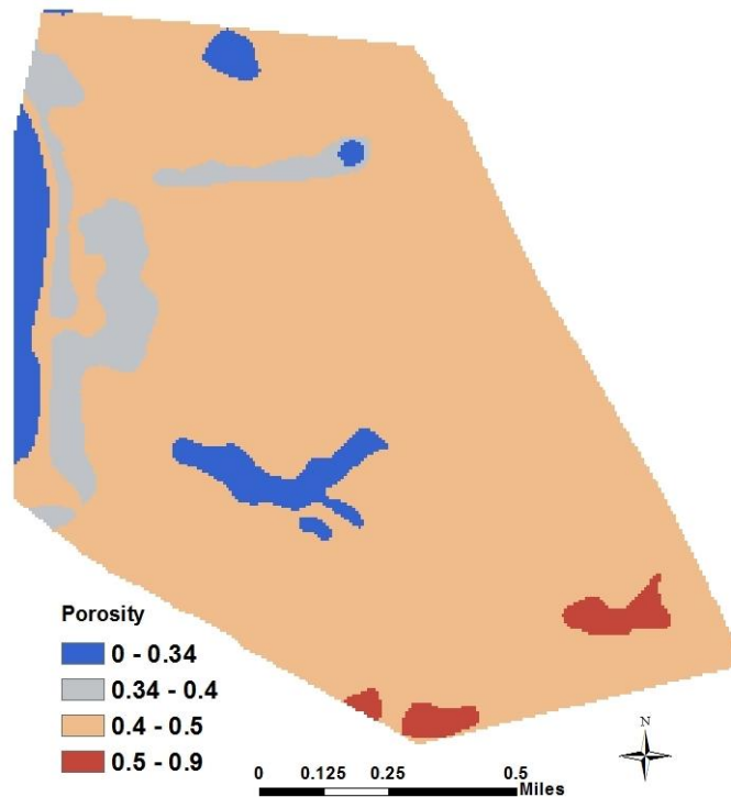
Figure 3–7. Heterogeneous porosity ([-]) of soil units.
