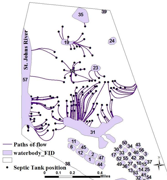
Figure 4–1. Simulated flow paths from septic systems to surface waterbodies.
