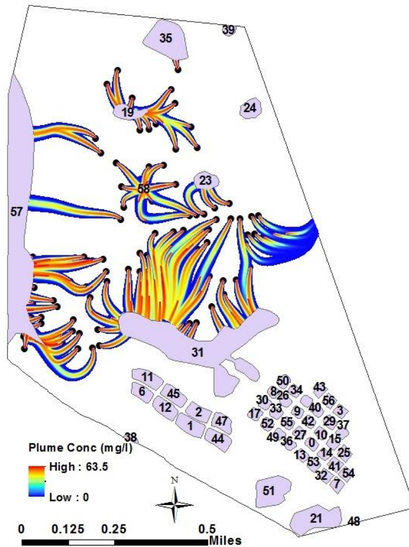
Figure 4-4. Simulated flow paths from septic systems to surface waterbodies. Parameter values specific to Case 3 are \alpha_L = 2.134 m, \alpha_T = 0.0549 m, and k = 0.001 d -1 .
