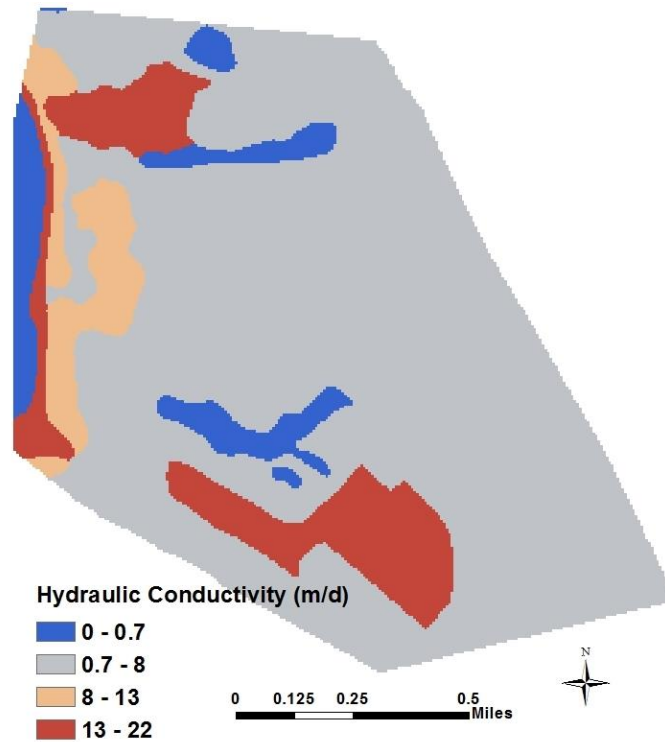
Figure 3–6. Heterogeneous hydraulic conductivity (m/d) of soil units.
