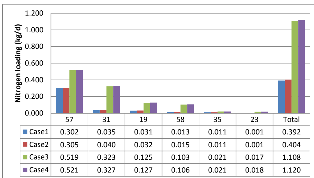
Figure 4-6. Nitrogen loading (kg/d) to the individual waterbodies for the four modeling cases.
