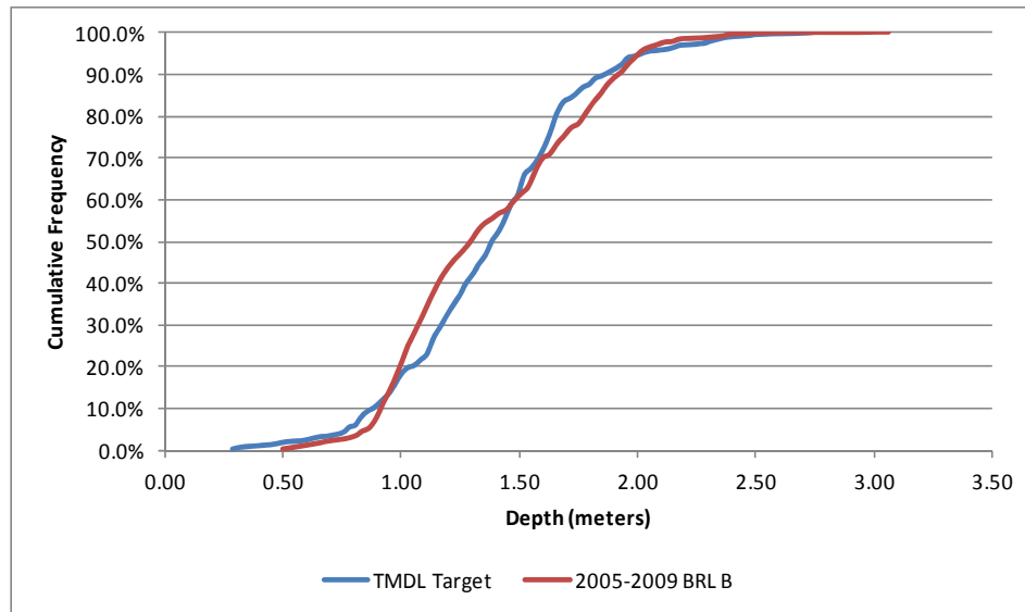
FIGURE 8: STEP 1 COMPLIANCE EVALUATION FOR BRL B FOR 2005-2009
