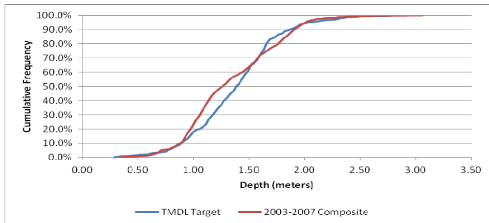
FIGURE 7: STEP 1 COMPLIANCE EVALUATION FOR BRL B FOR 2003-2007
