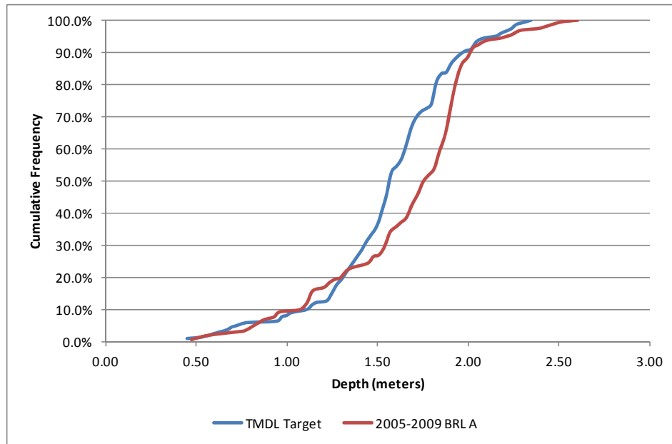
FIGURE 6: STEP 1 COMPLIANCE EVALUATION FOR BRL A FOR 2005-2009
