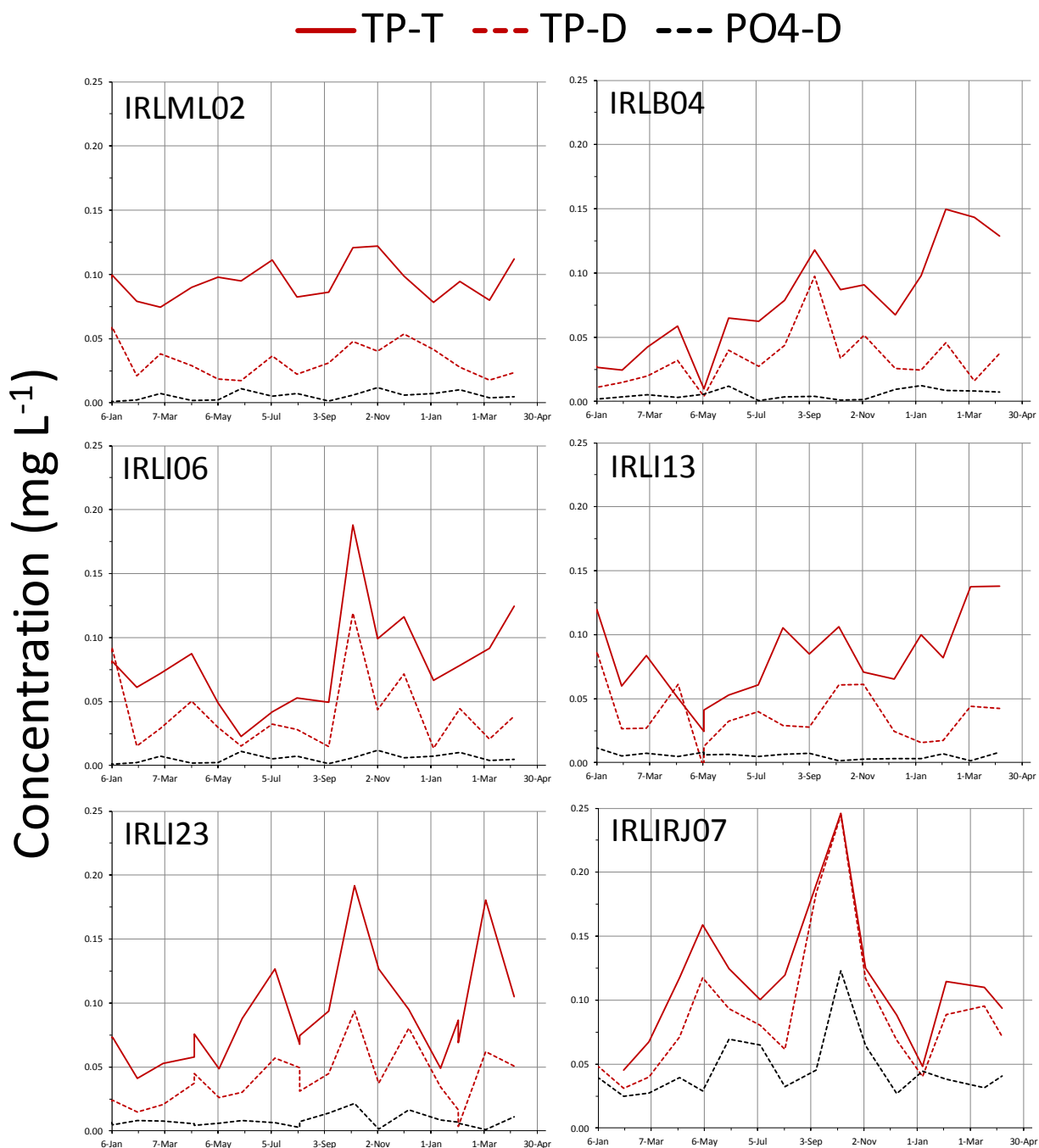
Figure 9. Concentrations of various forms of phosphorus
