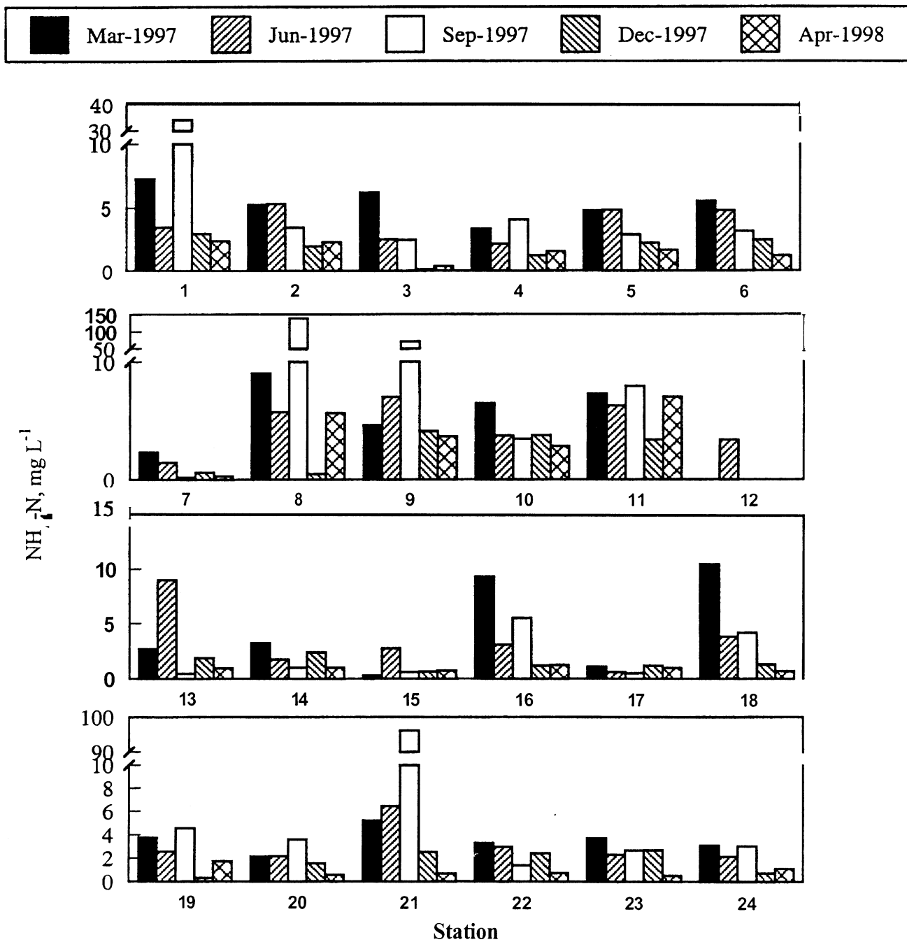
Figure 3.2. Seasonal changes in the porewater concentration of ammonium-N in the sediments of the Indian River Lagoon.
