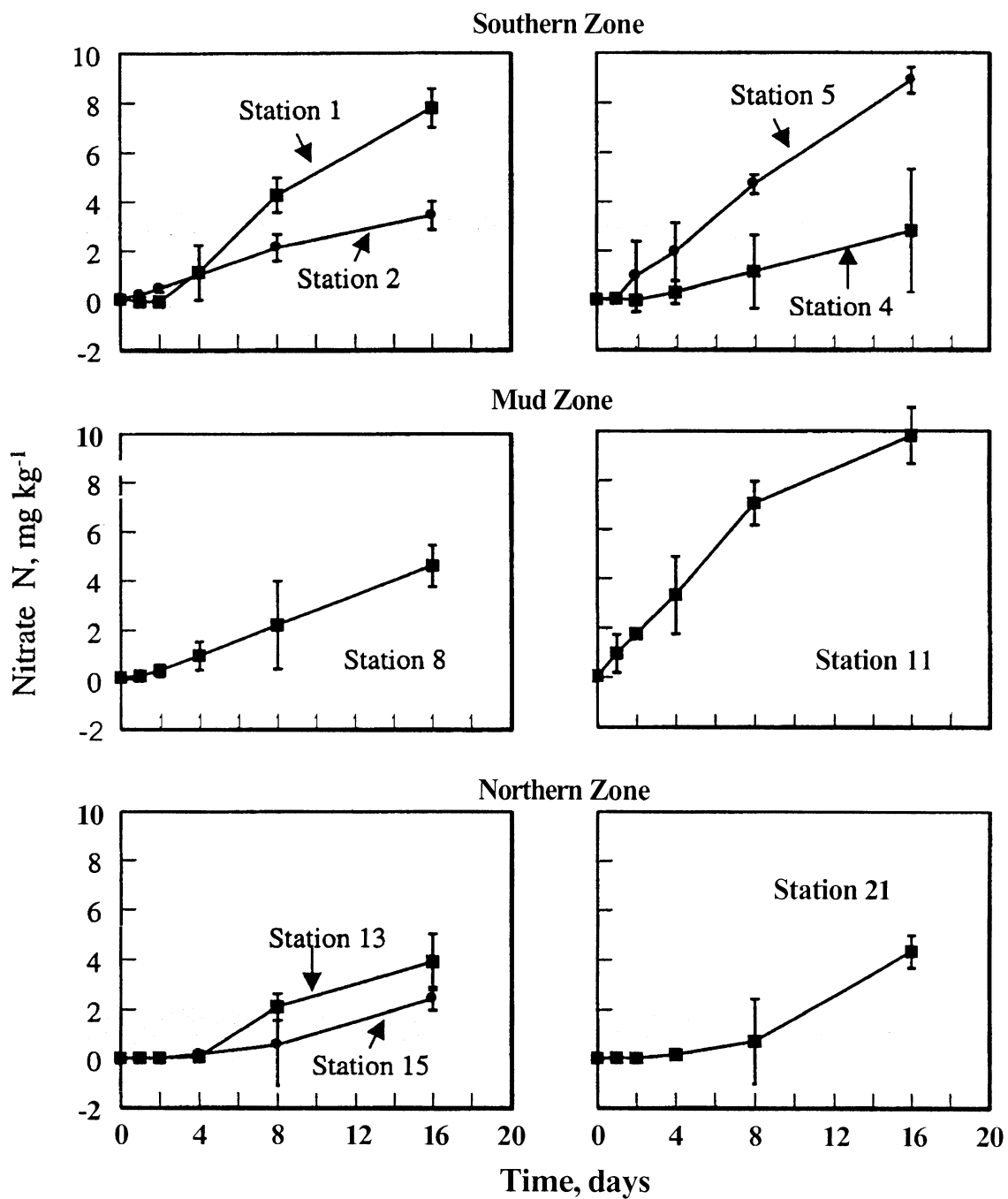
Fig. 6.6 Changes in \text{NO}_3\text{-N} concentration of sediments incubated under aerobic conditions.
