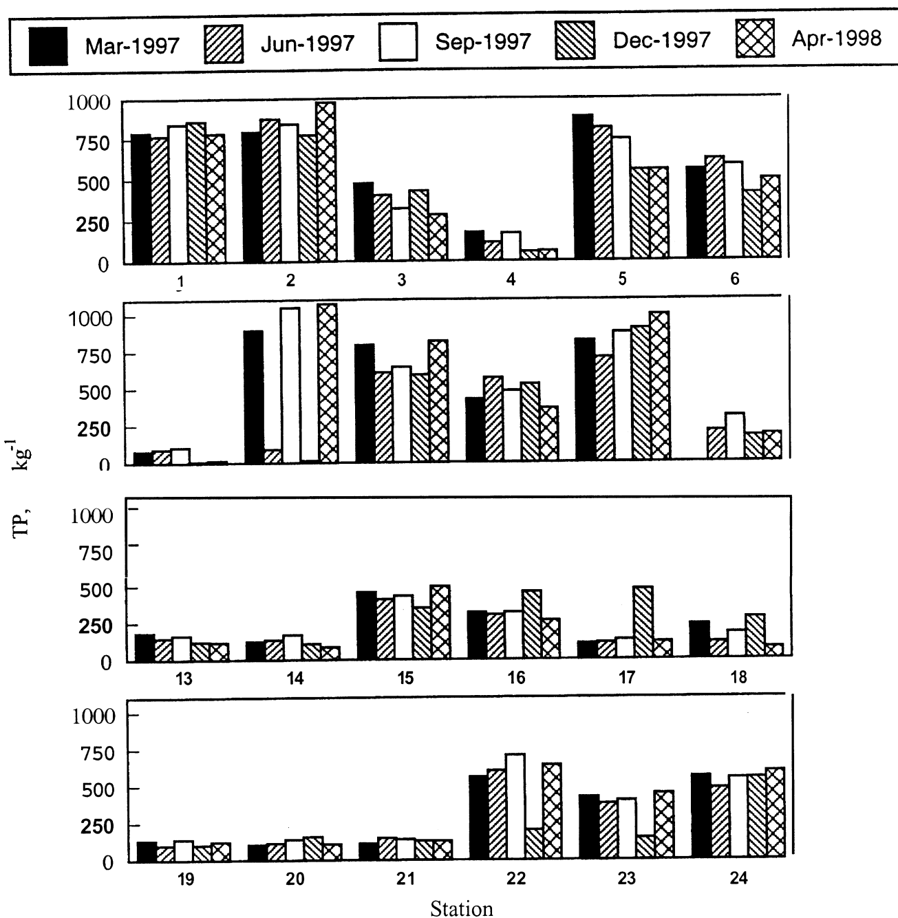
Figure 3.4. Seasonal changes in the total phosphorus content of the sediments of the Indian River Lagoon.
