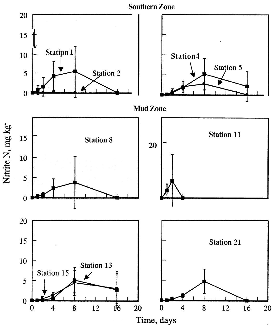
Fig. 6.5 Changes in \text{NO}_2\text{-N} concentration of sediments incubated under aerobic conditions.
