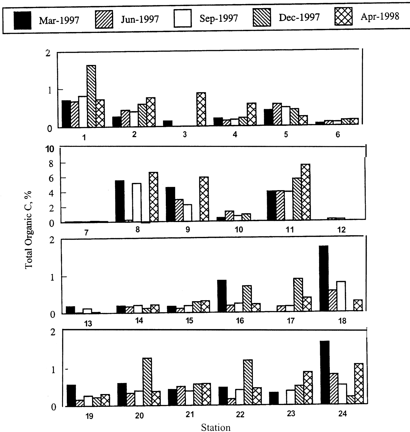
Figure 3.5. Seasonal changes in the total organic carbon content of the sediments of the Indian River Lagoon.
