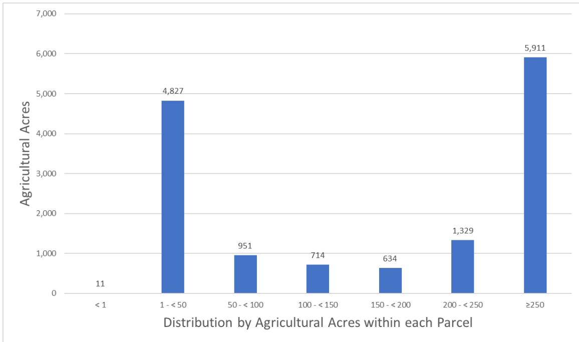
Figure B-10. Distribution by agricultural acres within each parcel, Indian Prairie Subwatershed
