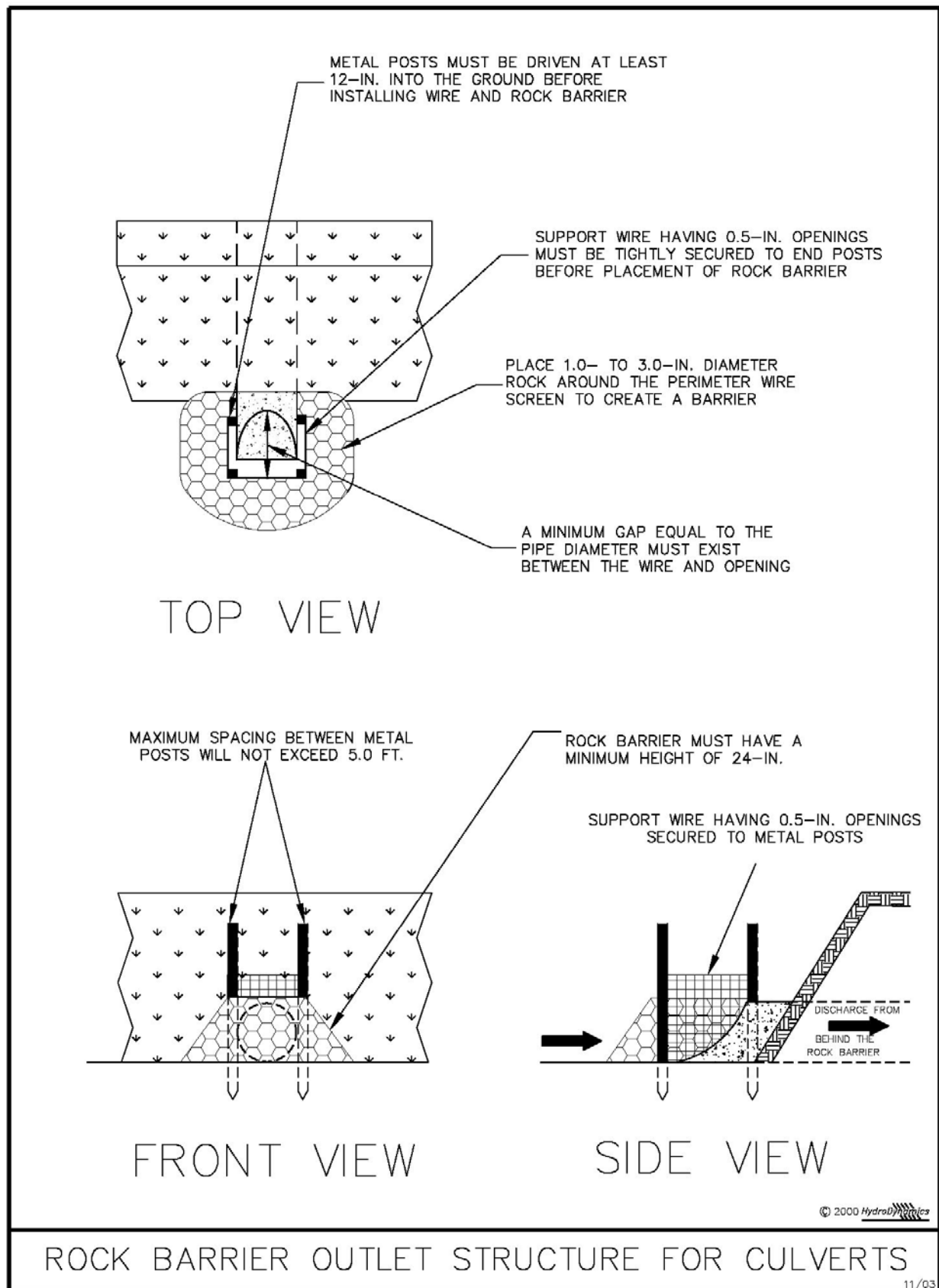
Figure IV-14: Illustration of a Rock Barrier Structure for Culverts
