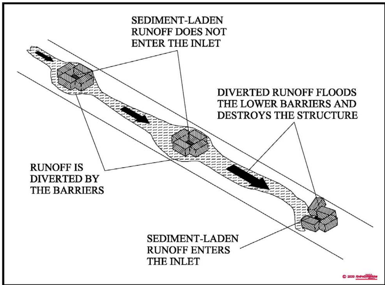
Figure V-124: How Barriers Around Area Drains on a Grade Fail During Runoff Events
