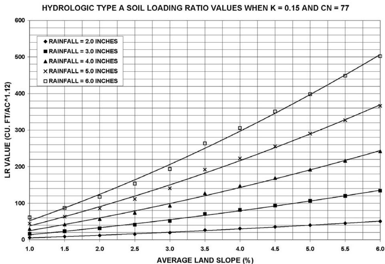
Figure IV-7: Hydrologic Type A Soils Loading Ratio Graph
