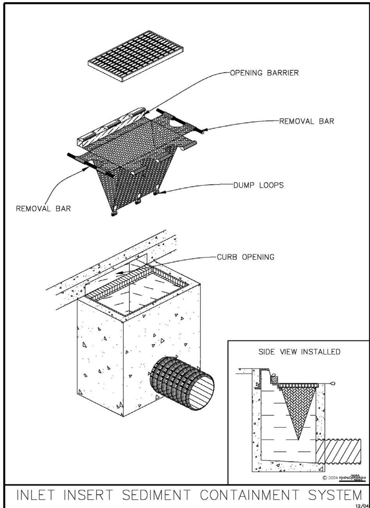
Figure V-13: Illustration of an Inlet Insert Sediment Containment System
