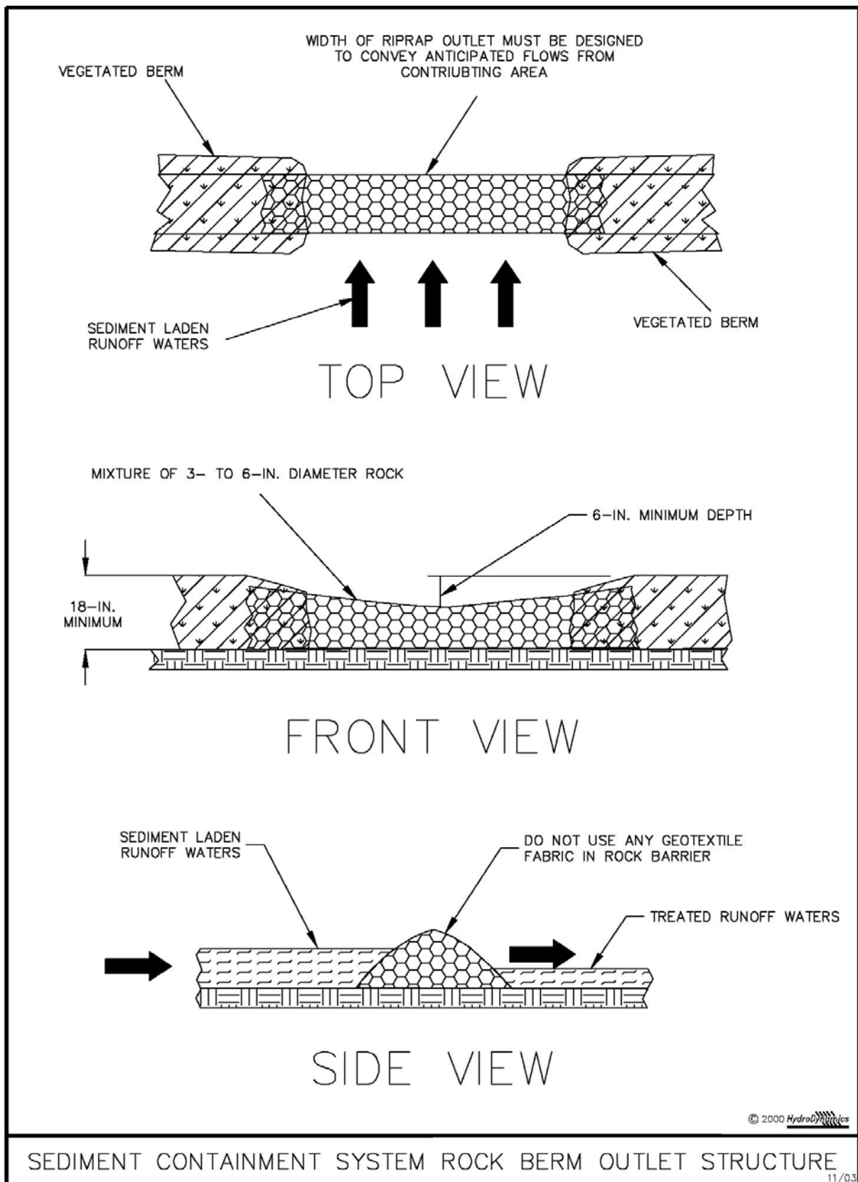
Figure IV-11: Illustration of a SCS Rock Berm Outlet Structure
