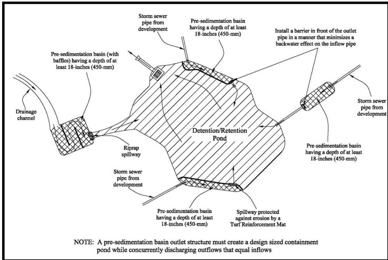
Figure IV-6: Conceptual Pre-Sedimentation (a.k.a. Forebay) Basins (No Scale)
