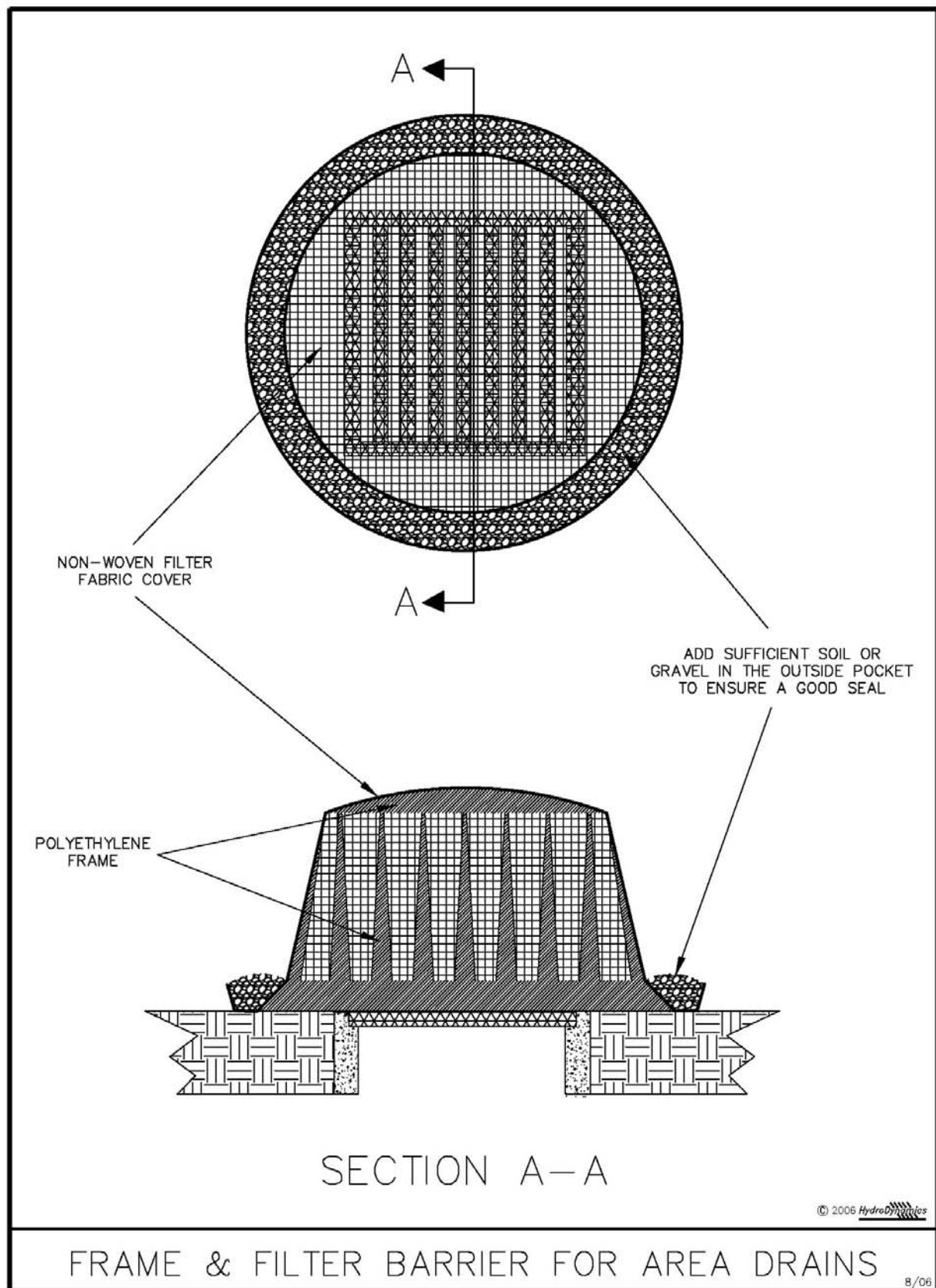
Figure V-9: Illustration of a Frame & Filter Barrier for Area Drains
