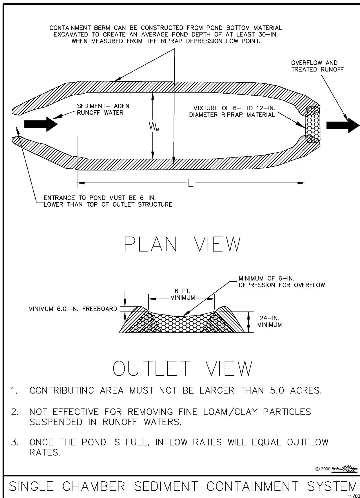
Figure IV-12: Illustration of a Single Chamber SCS
