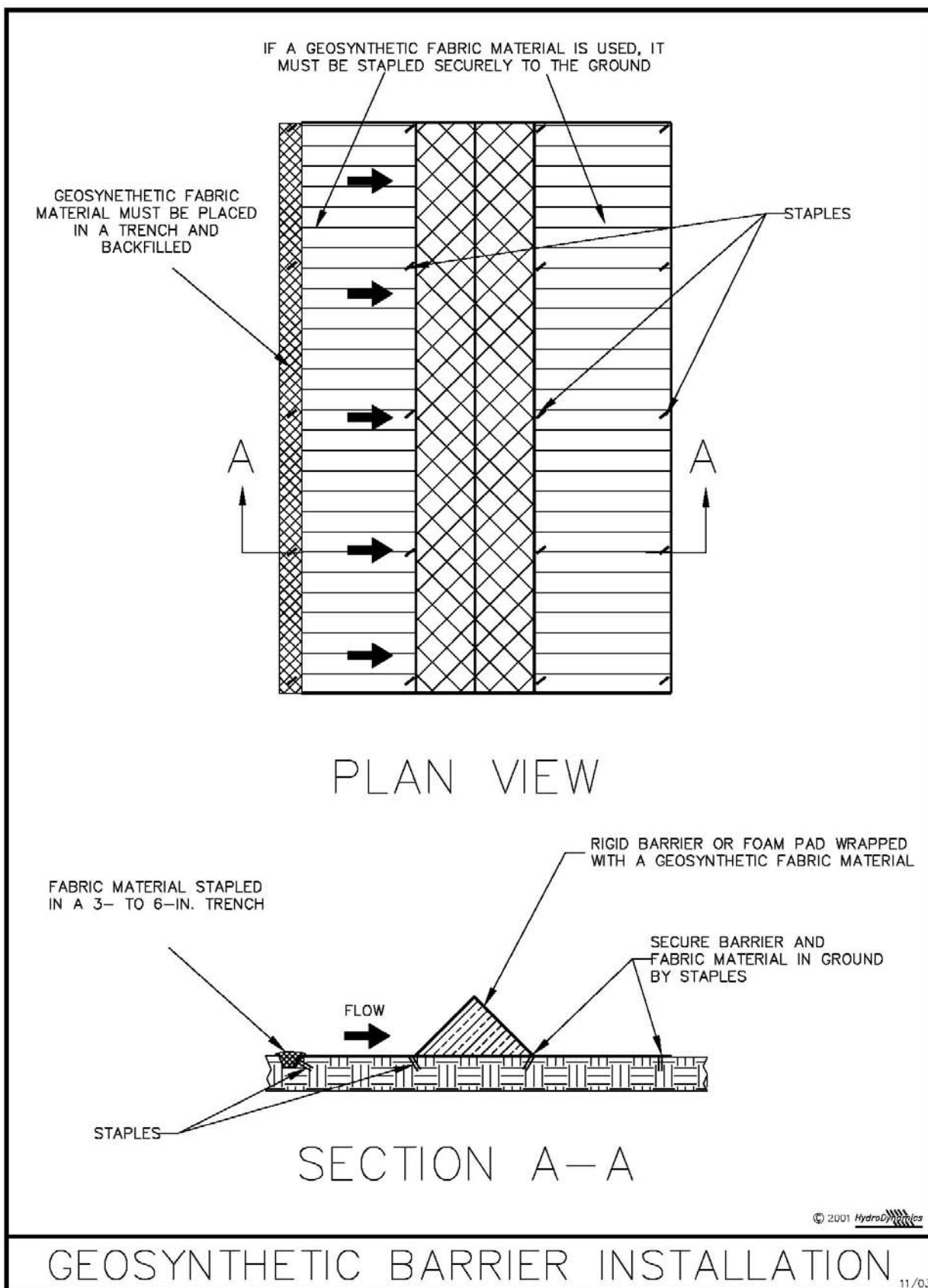
Figure V-5: Illustration of a Geosynthetic Barrier
