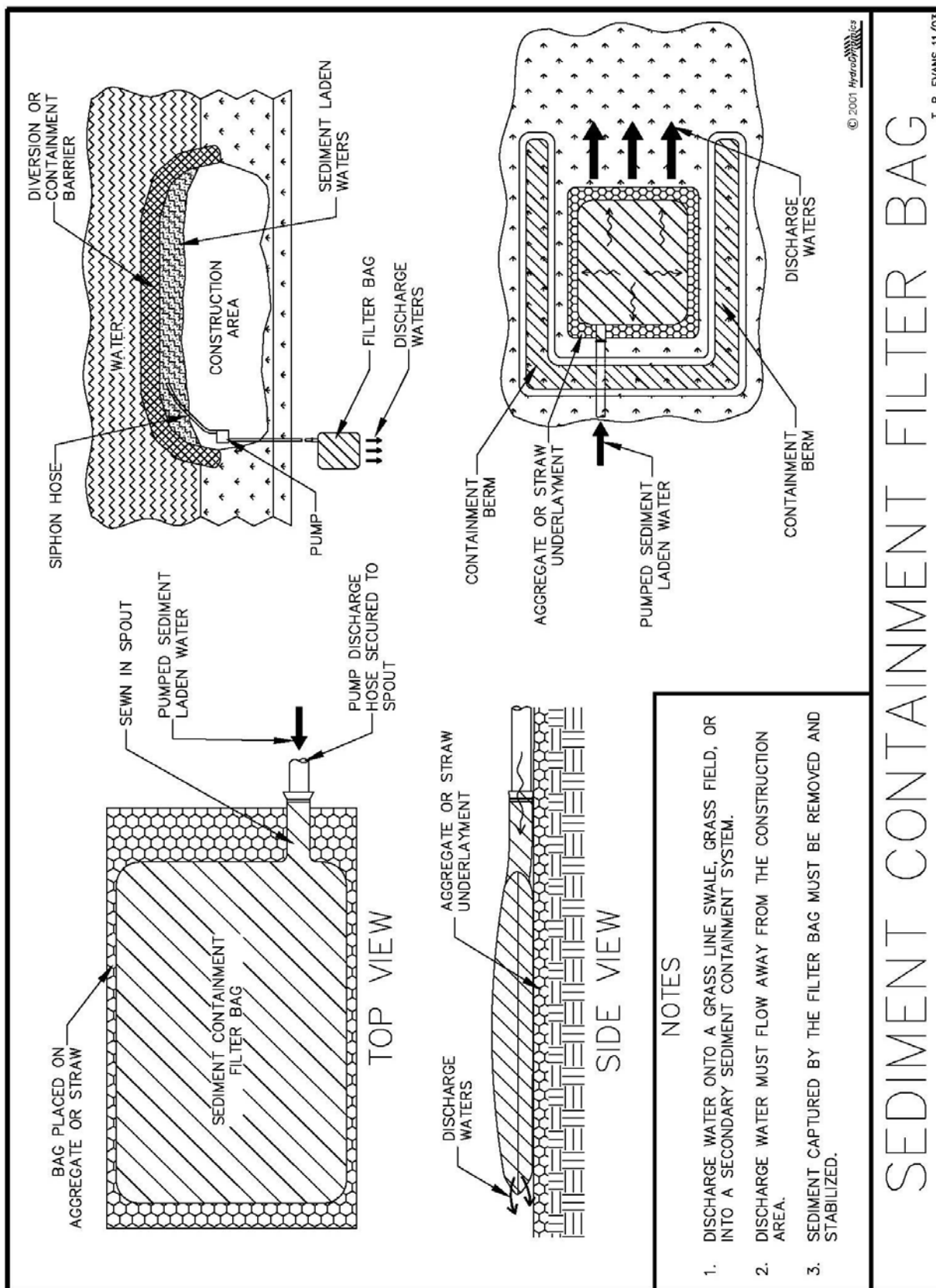
Figure IV-15: Illustration of a Sediment Containment System Filter Bag
