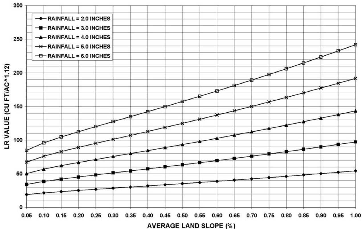
HYDROLOGIC TYPE D SOIL LOADING RATIO VALUES WHEN K = 0.37 AND CN = 94
