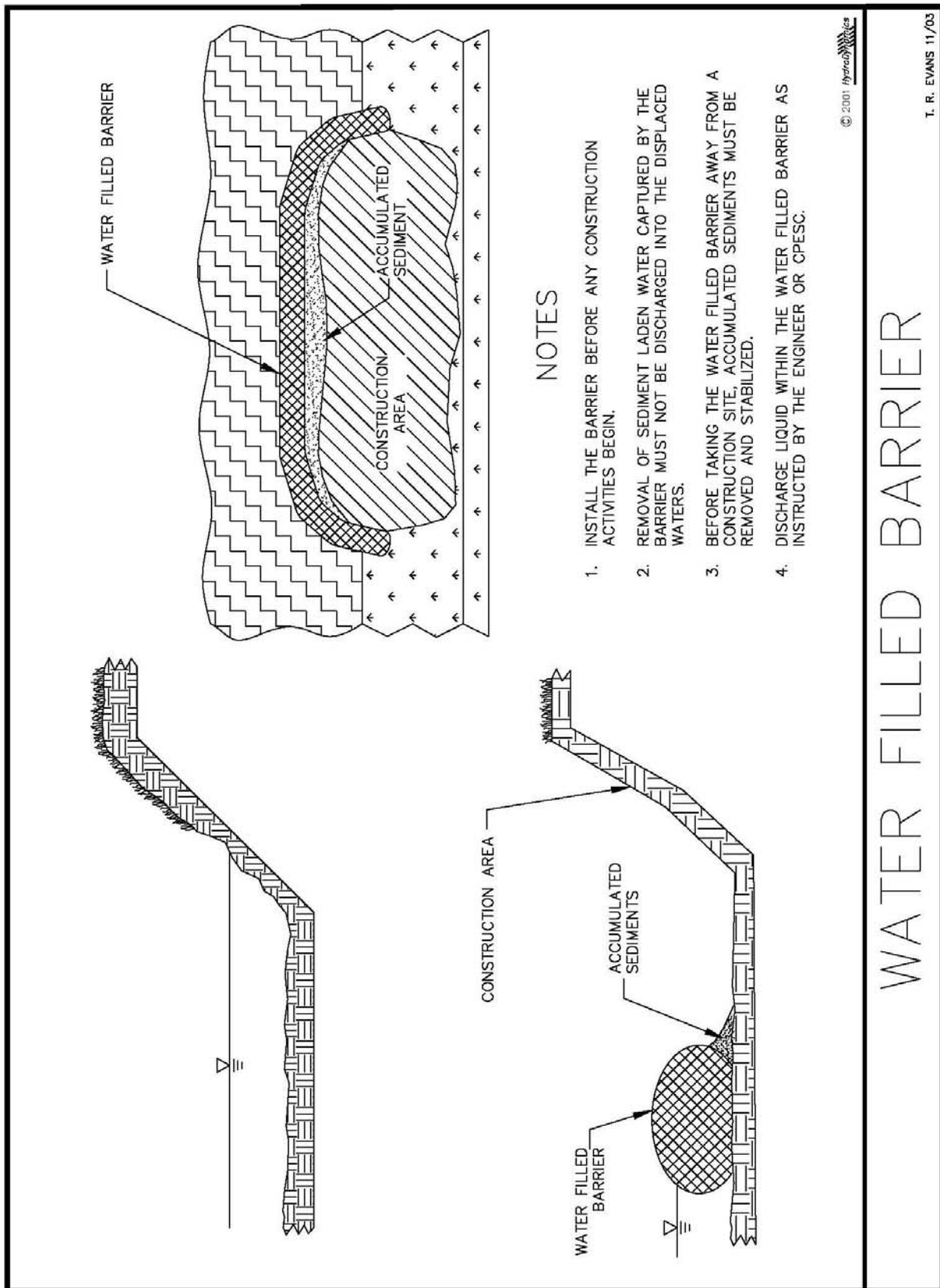
Figure V-7: Illustration of a Water Filled Barrier
