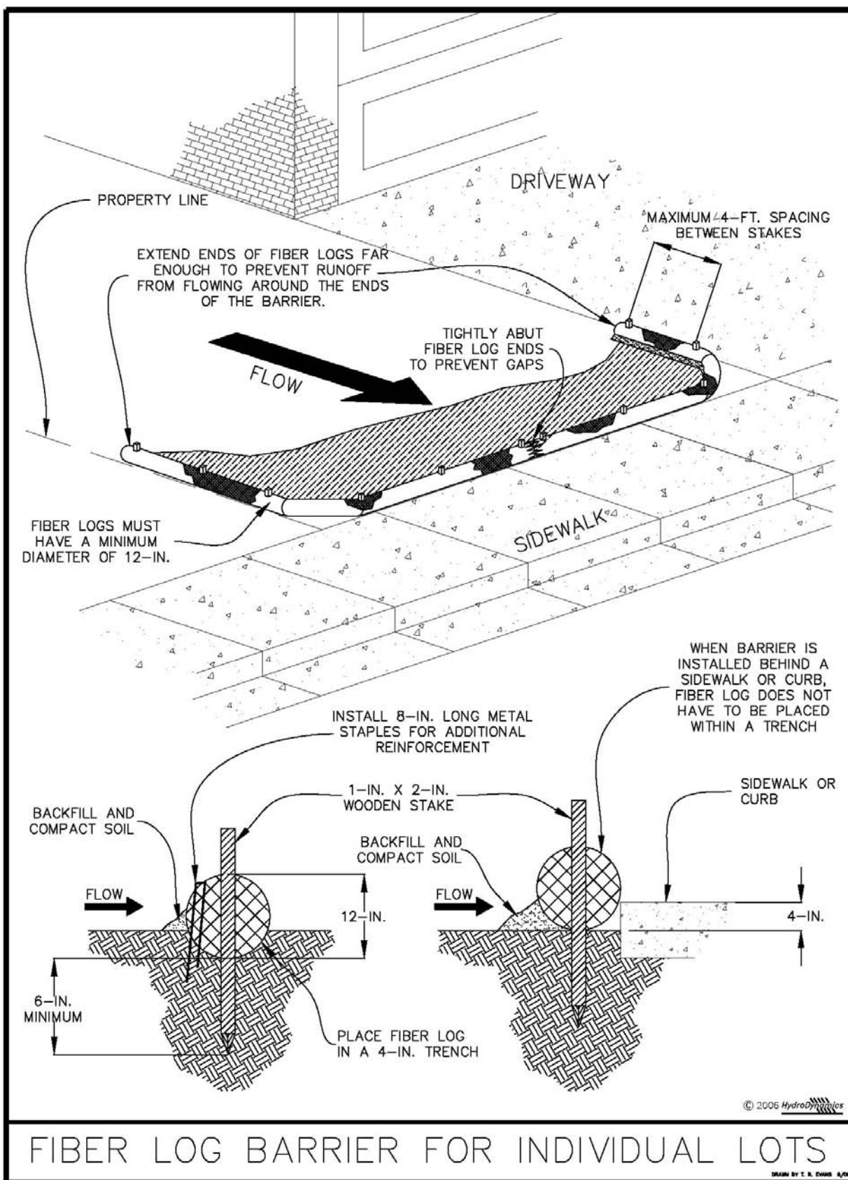
Figure V-3. Illustration of Fiber Log Barriers for Individual Lots
