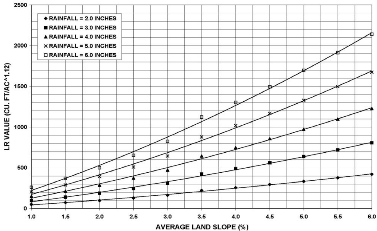
Figure IV-9: Hydrologic Type C Soils Loading Ratio Graph
