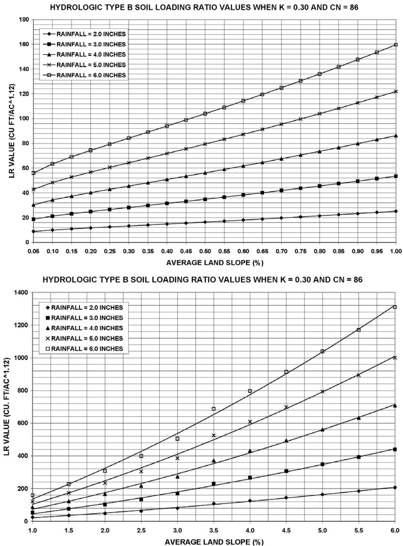
Figure IV-8: Hydrologic Type B Soils Loading Ratio Graph
