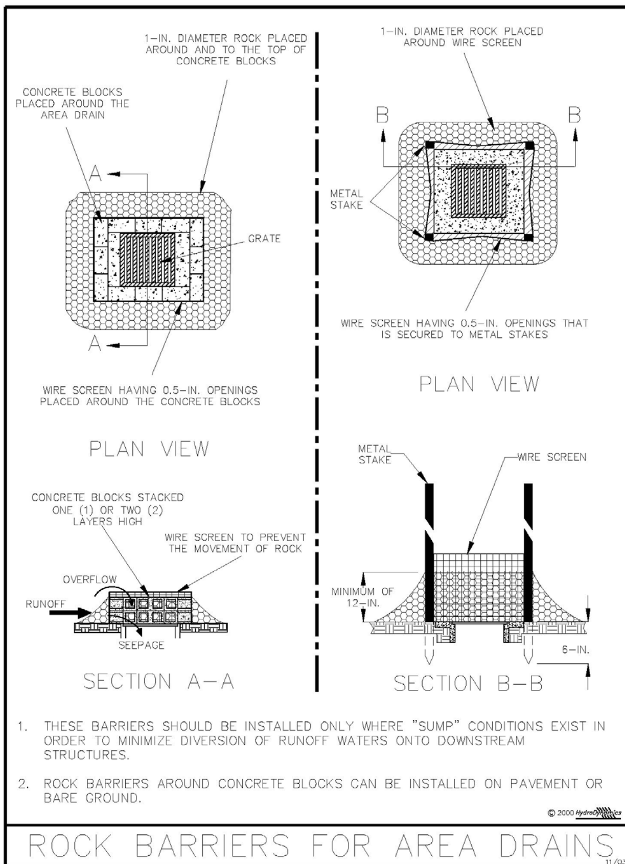
Figure V-8: Illustration of Rock Barriers around Area Drains
