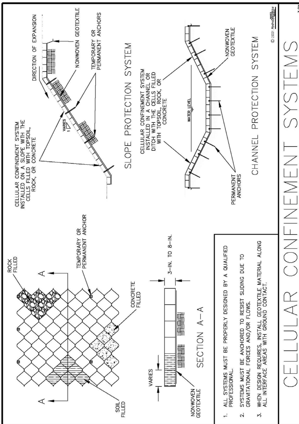
Figure V-15: Illustration of uses for Cellular Confinement Systems
