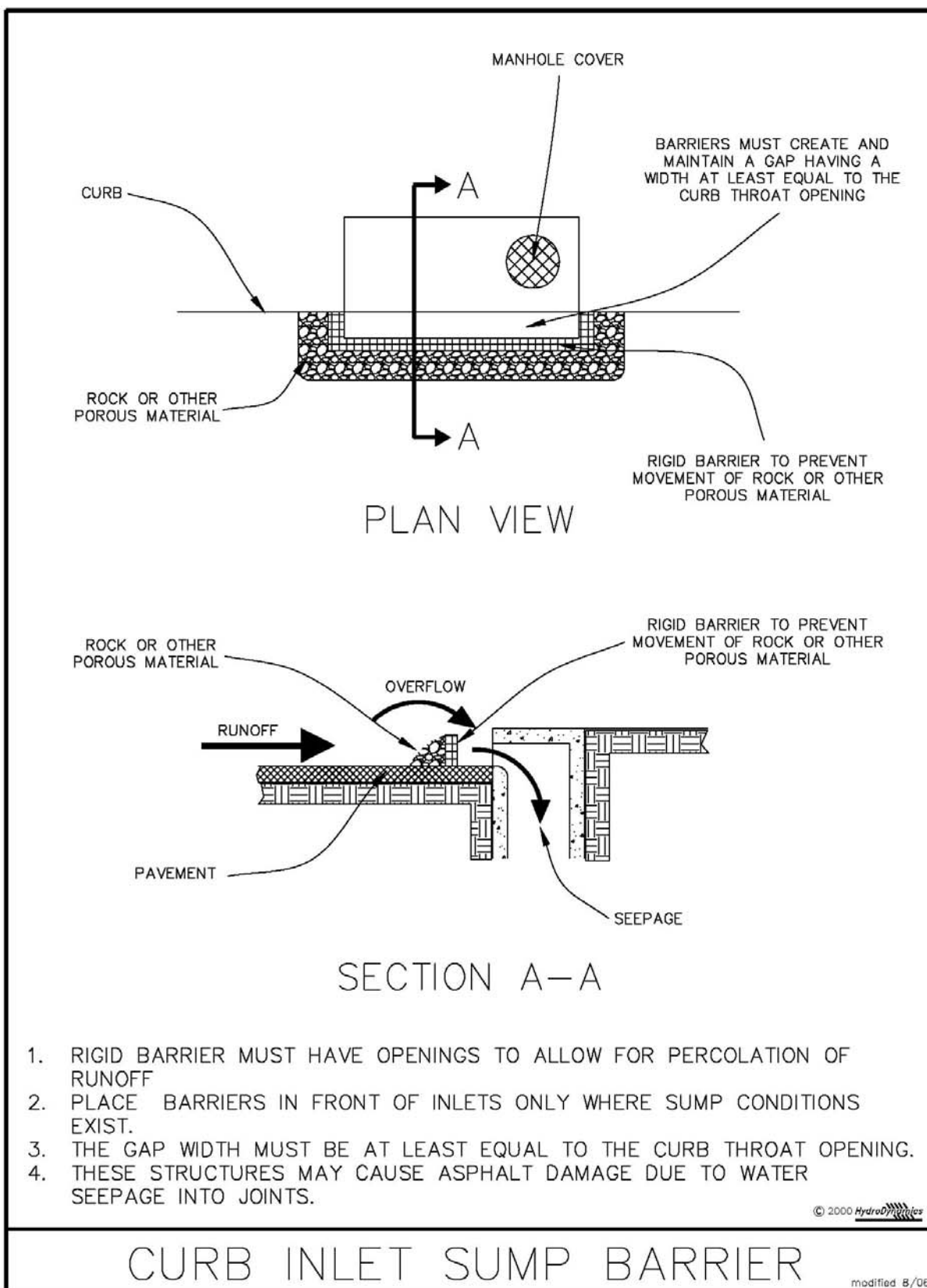
Figure V-10: Illustration of a Curb Inlet “Sump” Barrier
