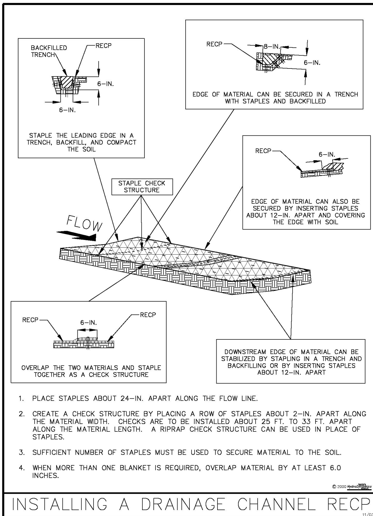
Figure III-4: Illustration of Installing a RECP in a Drainage Channel
