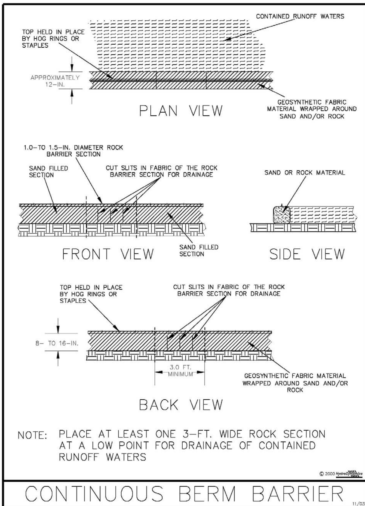
Figure V-4: Illustration of a Continuous Berm Barrier
