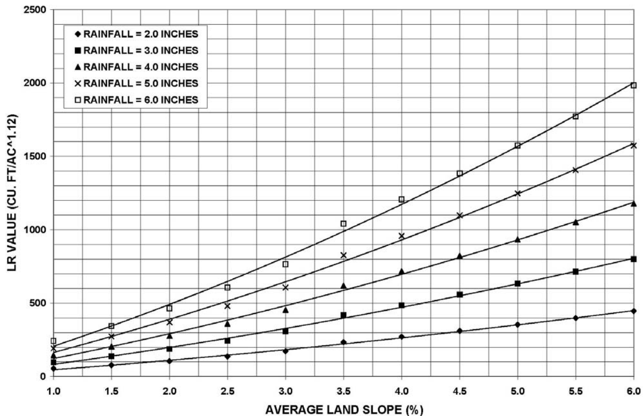
Figure IV-10: Hydrologic Type D Soils Loading Ratio Graph
