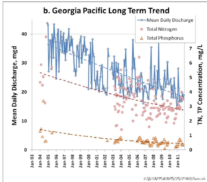
FIGURE 53: LONG-TERM TRENDS IN EFFLUENT DISCHARGE VOLUME TN AND TP CONCENTRATIONS FOR GEORGIA PACIFIC
