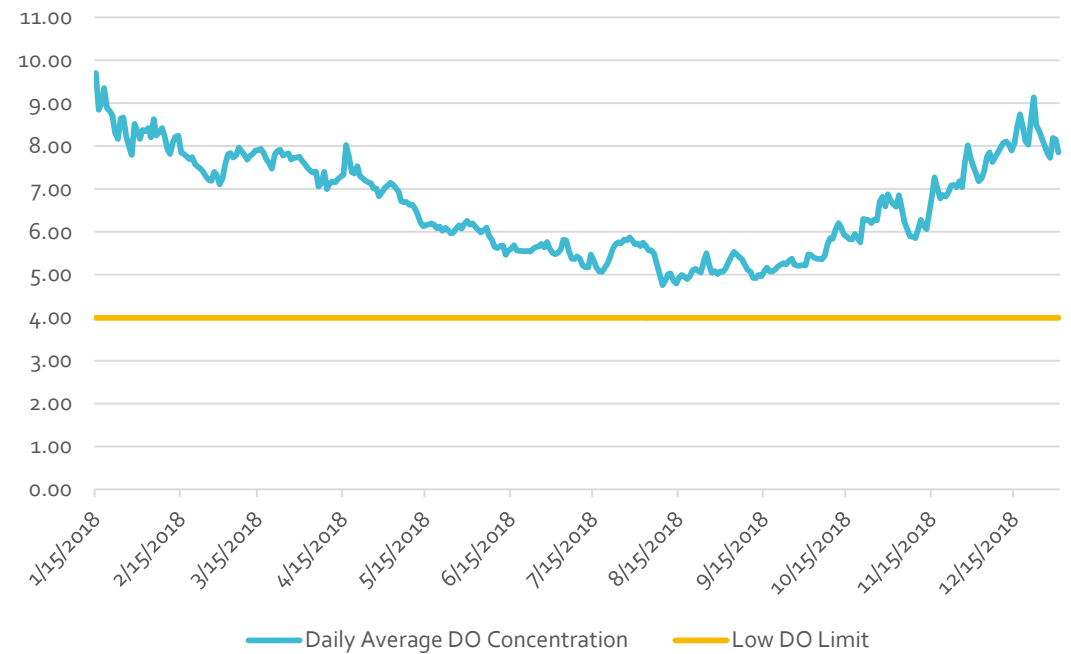
Dames Point Daily Average Dissolved Oxygen 2018
