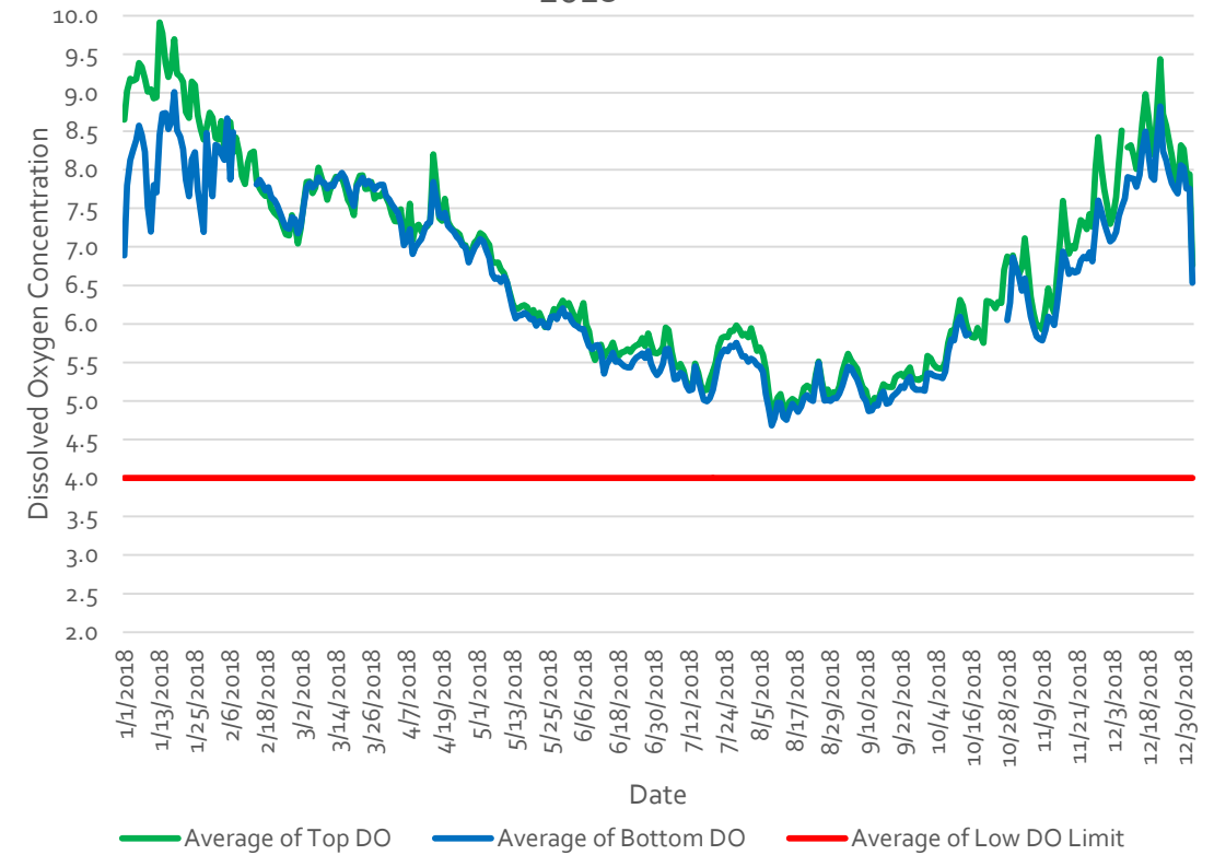
Dames Point Daily Average Dissolved Oxygen 2018
