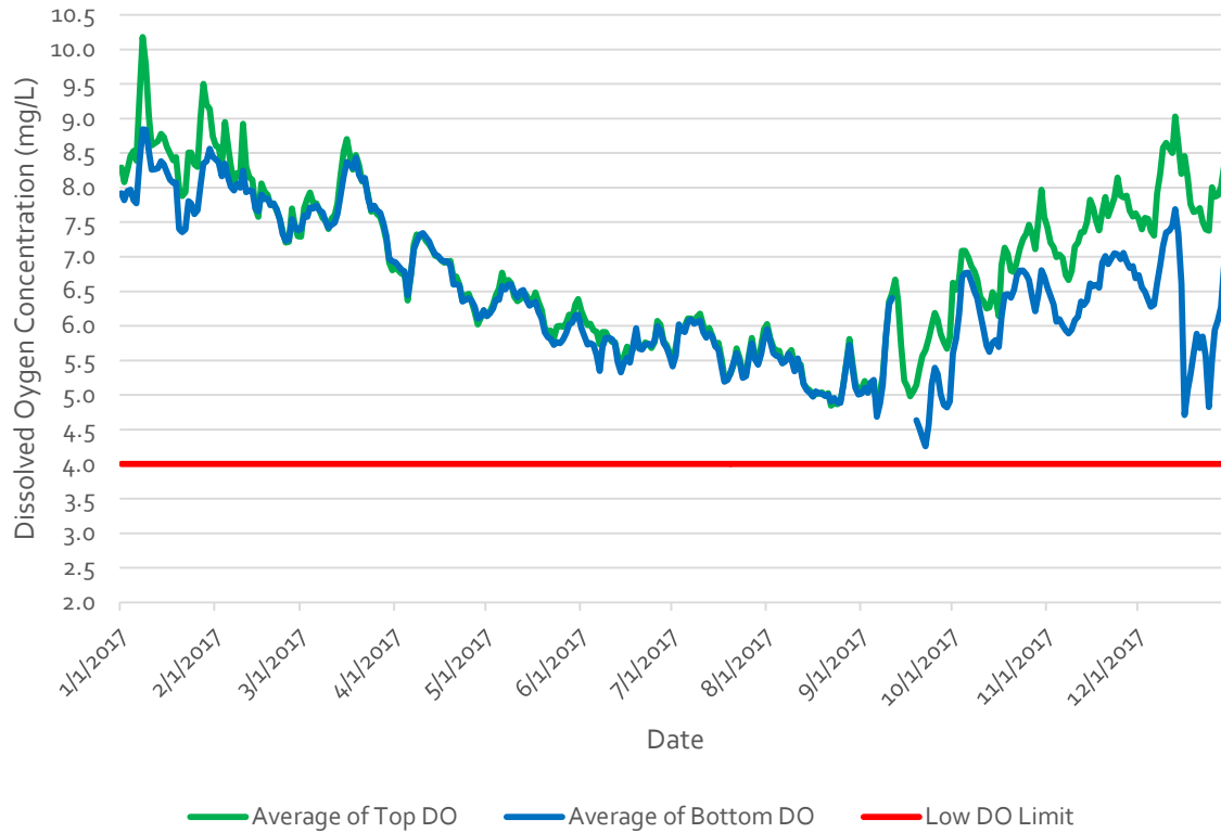
Dames Point Daily Average Dissolved Oxygen 2017
