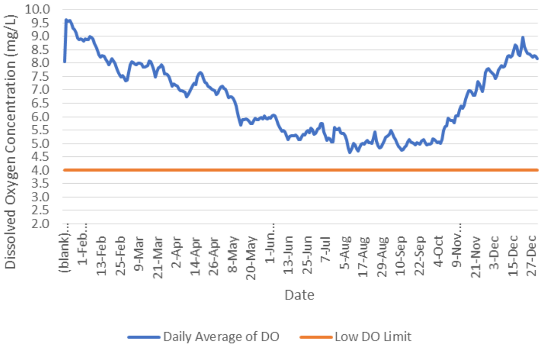
Clapboard Creek Daily Average Dissolved Oxygen 2018
