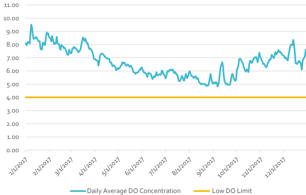
Dames Point Daily Average Dissolved Oxygen 2017
