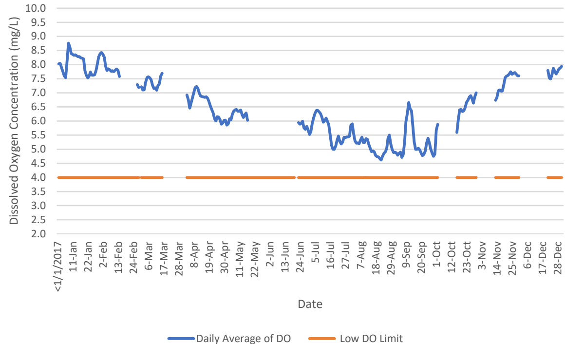
Clapboard Creek Daily Average Dissolved Oxygen 2017
