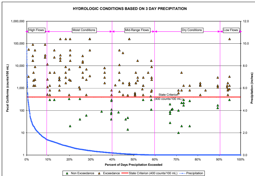
Figure 5.4. Fecal Coliform Data by Hydrologic Condition
