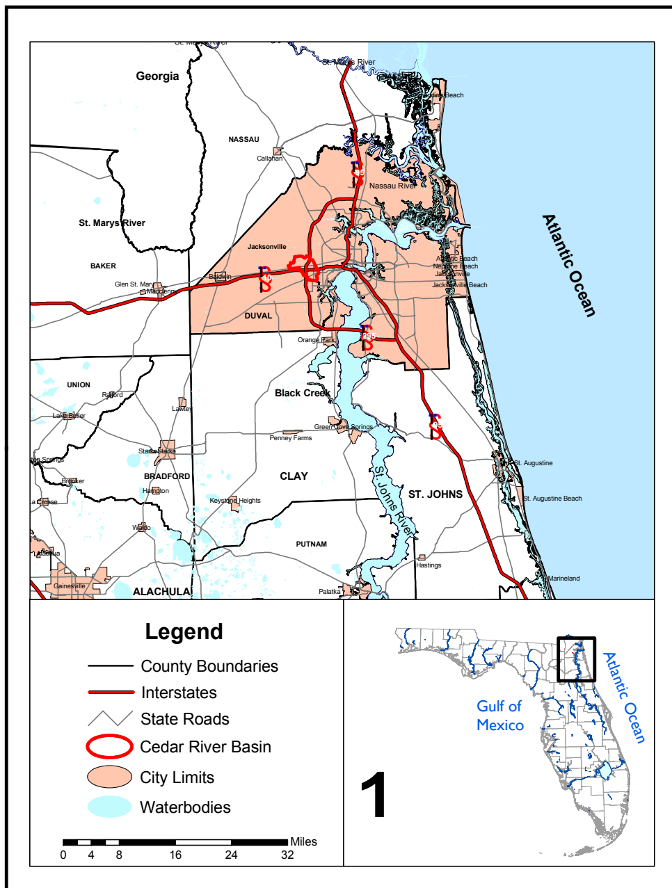
Figure 1.1. Location of Cedar River (2262) and Major Geopolitical Features in the St. Johns River Basin
