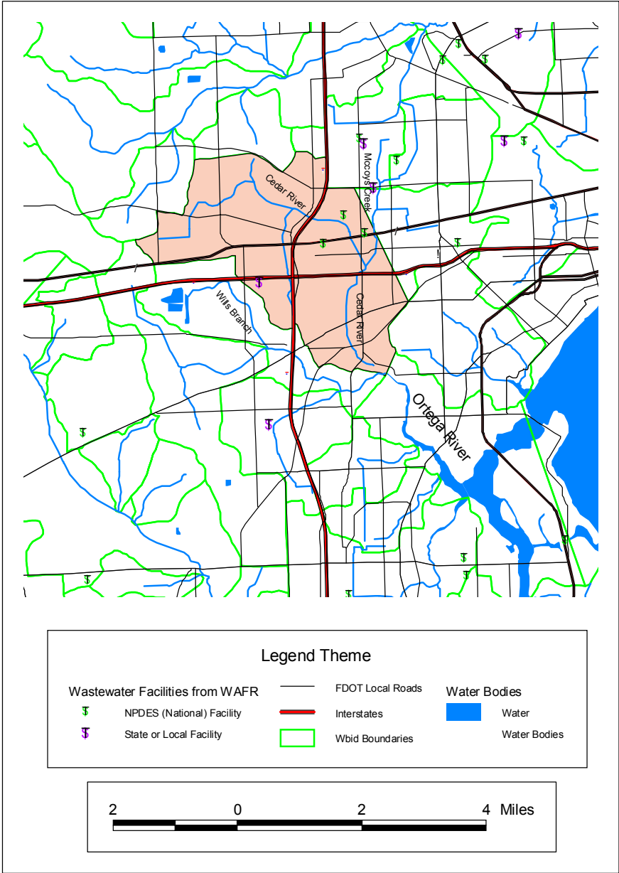
Figure 1.2. Cedar River WBID
