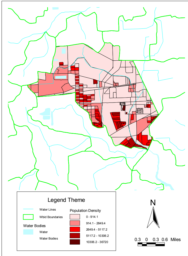
Figure 4.3. Population Density in the Cedar River Watershed
