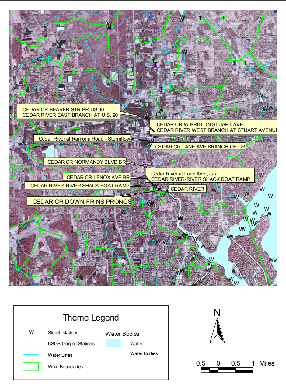
Figure 5.1. Historical Sample Sites in Cedar River Watershed
