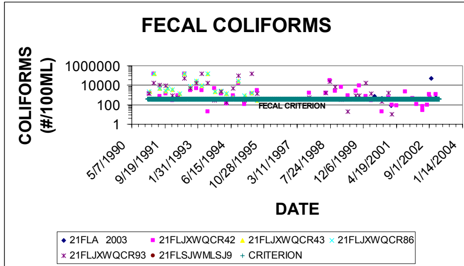
Figure 5.3. Total Coliform Historical Observations for Cedar River, WBID 2262
