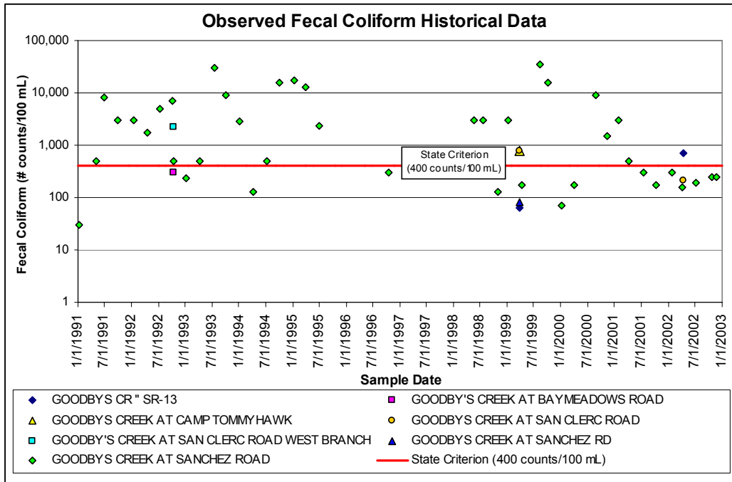
Figure 5.2. Historical Observations for Goodbys Creek
