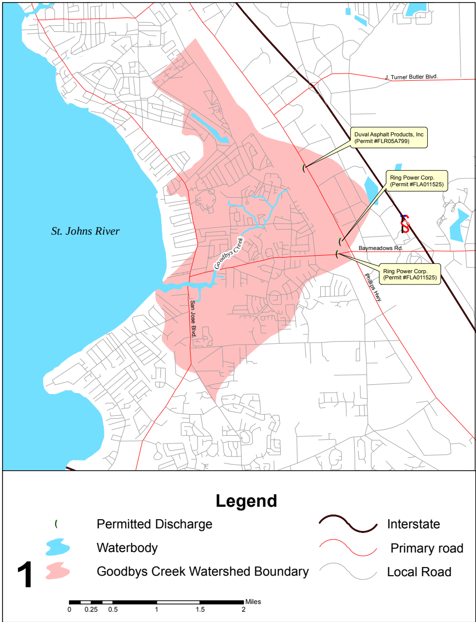
Figure 4.1. Location of Permitted Discharges in Goodbys Creek Watershed
