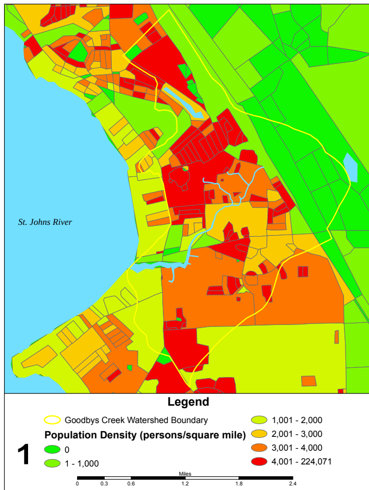
Figure 4.3. Population Density in the Goodbys Creek Watershed
