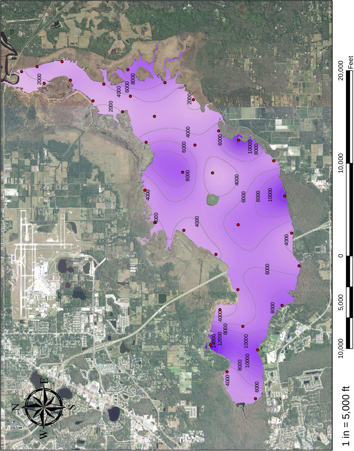
Figure 3-15. Isopleths of Total Nitrogen Flux ( \mu\text{g}/\text{m}^2\text{-day} ) into Lake Jesup from June 2009-August 2010.
