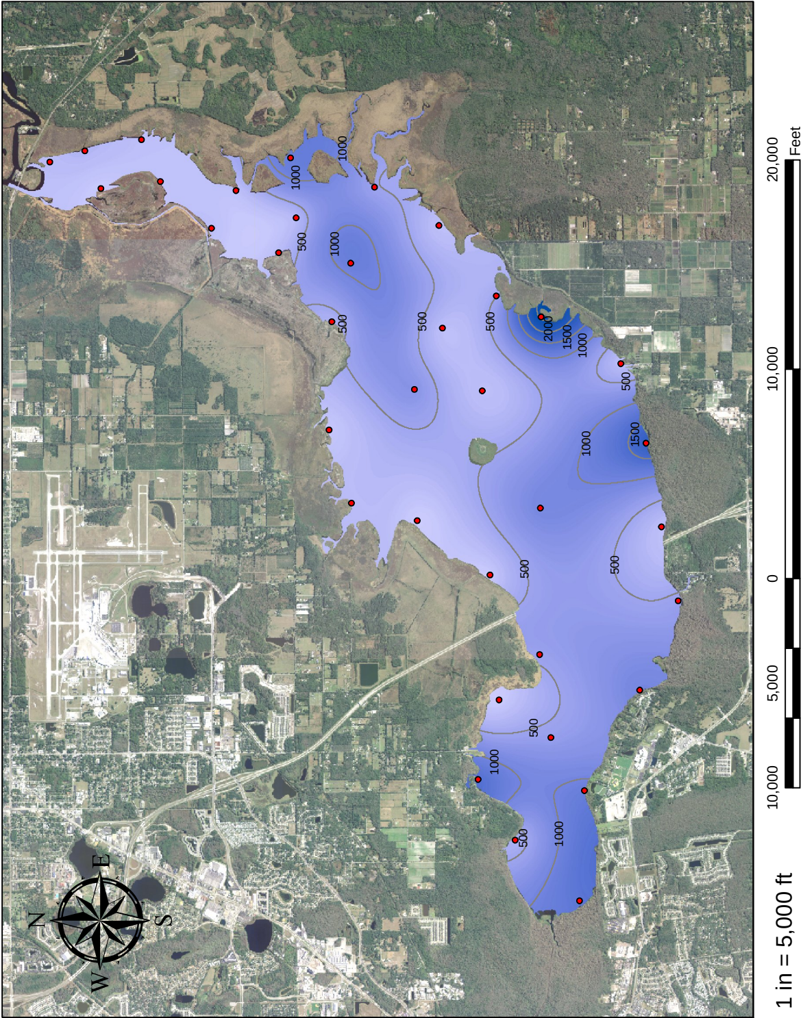
Figure 3-16. Isopleths of Total Phosphorus Flux ( \mu\text{g}/\text{m}^2\text{-day} ) into Lake Jesup from June 2009-August 2010.
