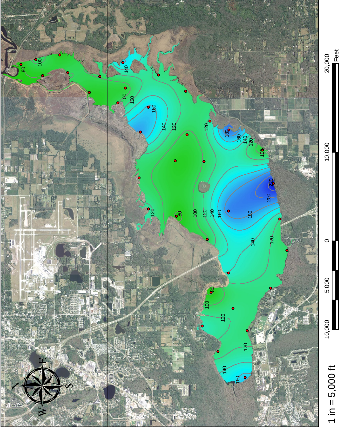
Figure 3-10. Mean Isopleths of Alkalinity (mg/l) in Groundwater Seepage Entering Lake Jesup from June 2009-August 2010.
