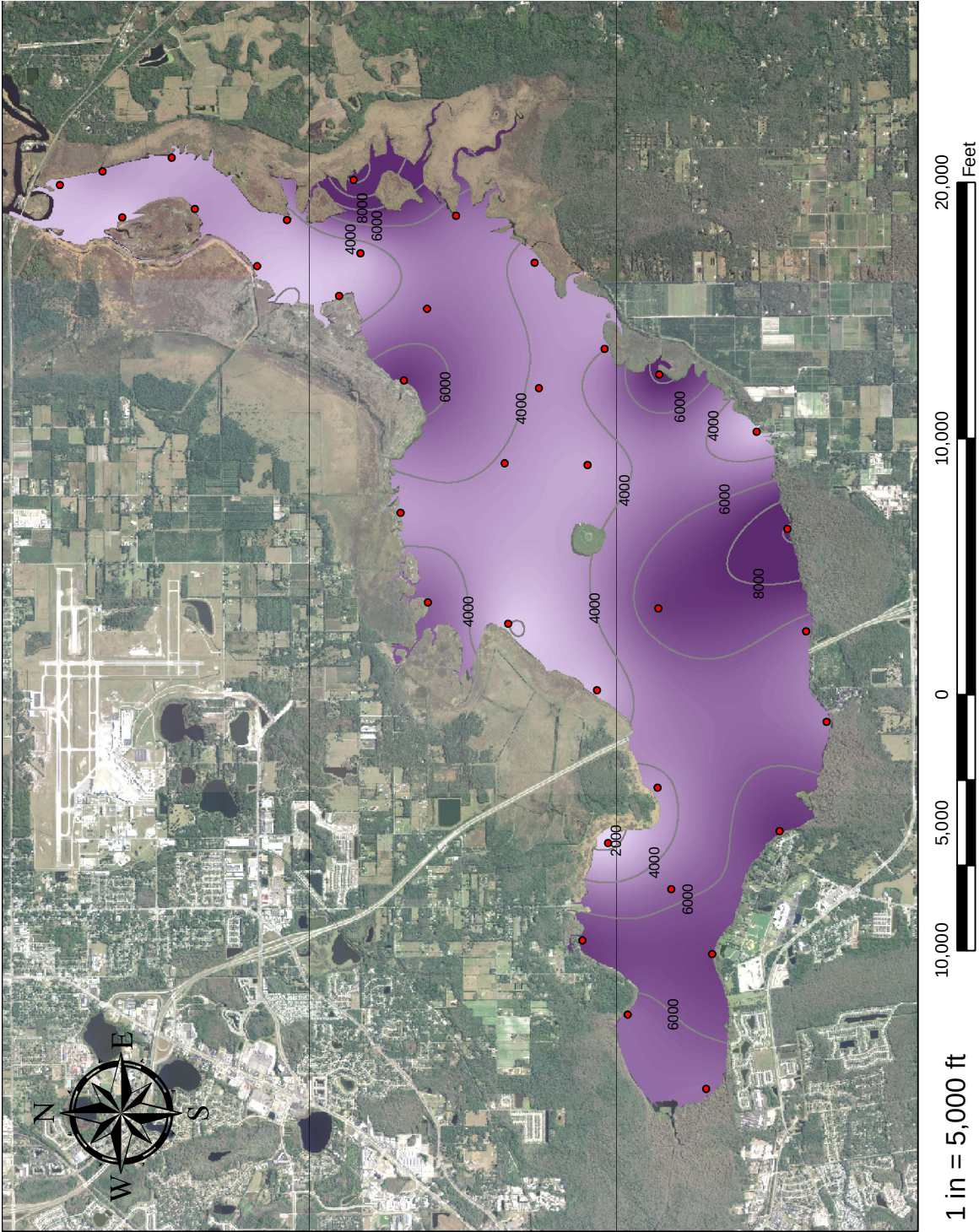
Figure 3-13. Mean Isopleths of Total Nitrogen ( \mu\text{g/l} ) in Groundwater Seepage Entering Lake Jesup from June 2009–August 2010.
