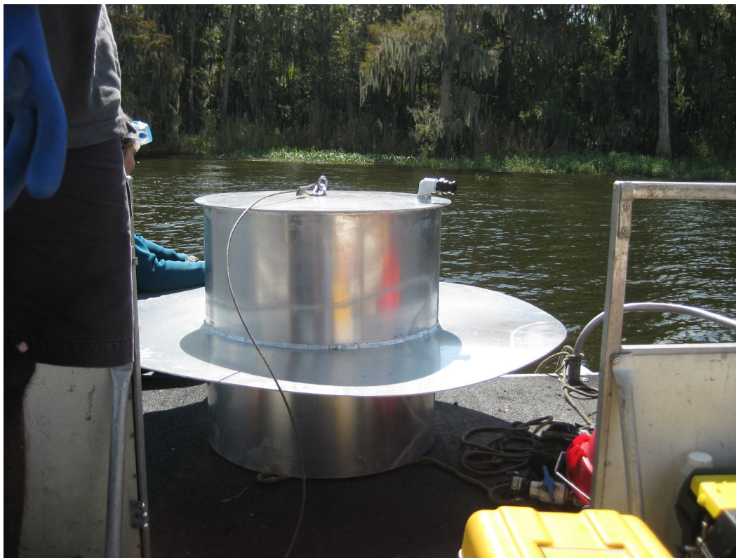
Figure 2-2. Typical Seepage Meter Used in Lake Jesup.
