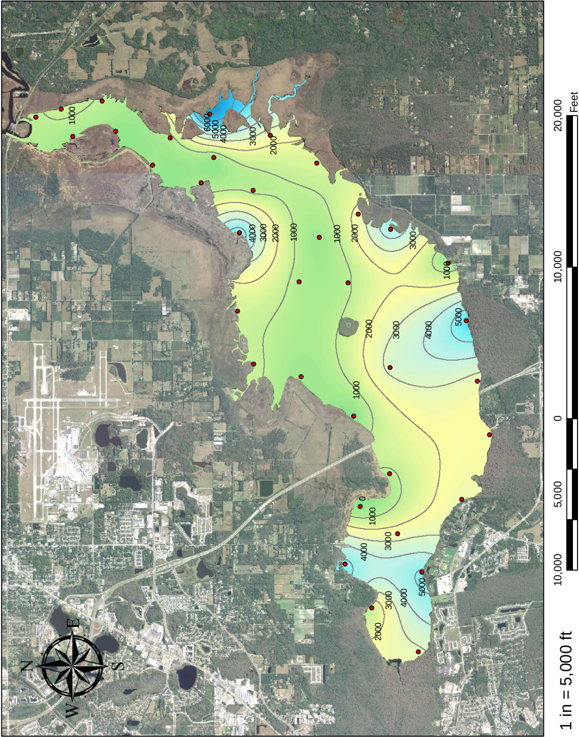
Figure 3-11. Mean Isopleths of Ammonia ( \mu\text{g/l} ) in Groundwater Seepage Entering Lake Jesup from June 2009-August 2010.
