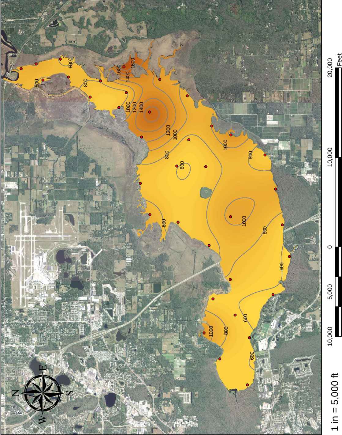
Figure 3-9. Mean Isopleths of Conductivity ( \mu\text{mho/cm} ) in Groundwater Seepage Entering Lake Jesup from June 2009–August 2010.
