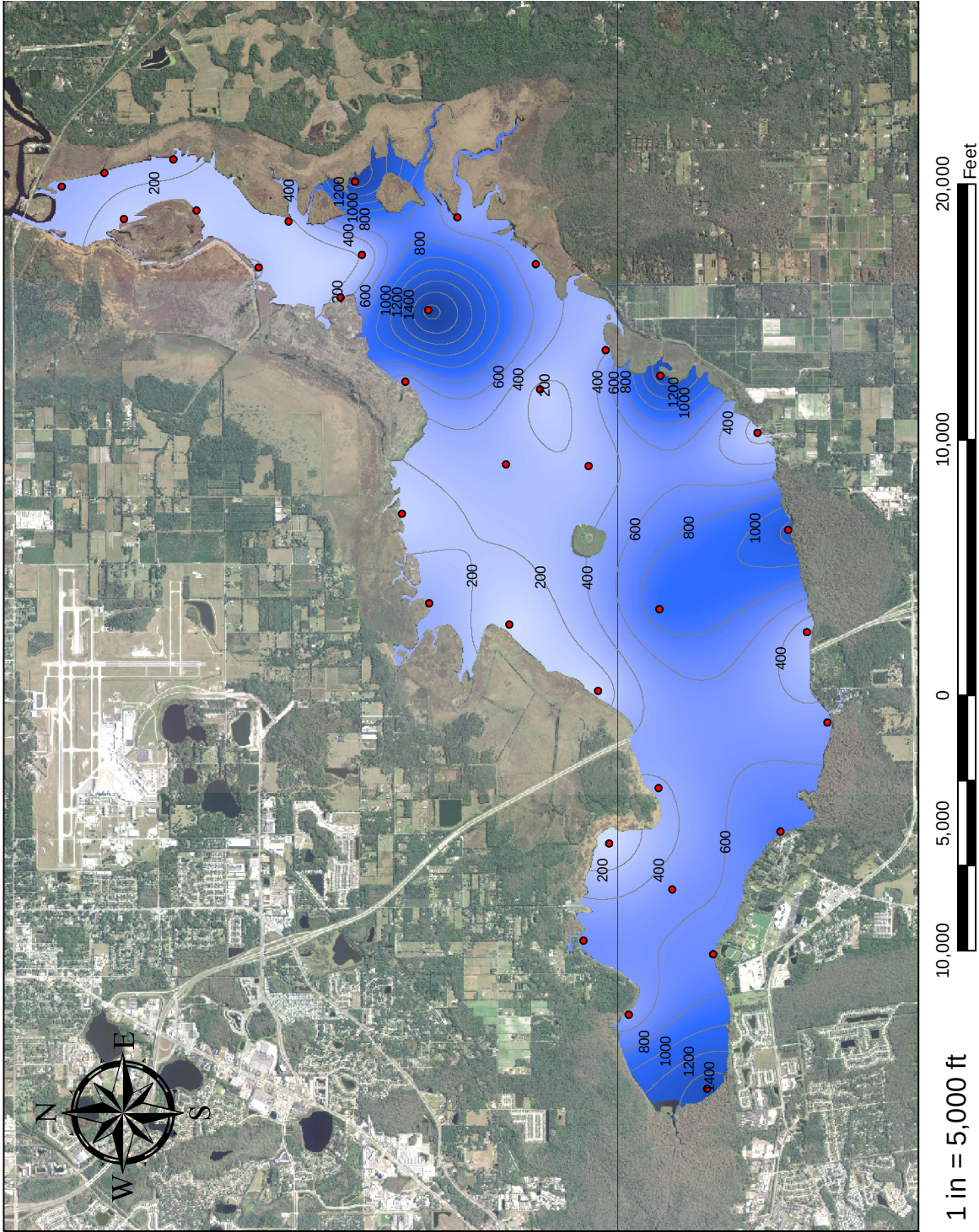
Figure 3-14. Mean Isopleths of Total Phosphorus ( \mu\text{g/l} ) in Groundwater Seepage Entering Lake Jesup from June 2009-August 2010.
