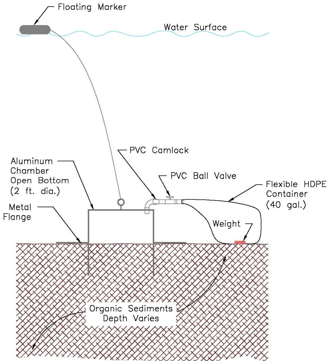
Figure 2-1. Typical Seepage Meter Installation.
