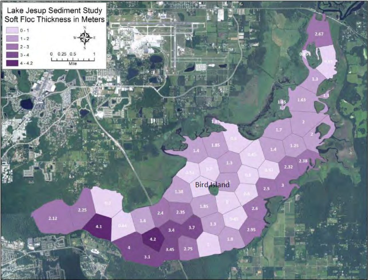
Figure A.2 – Thickness of the soft Sediment Layer in Lake Jesup (Brandt-Williams & Godfrey (n.d.))
