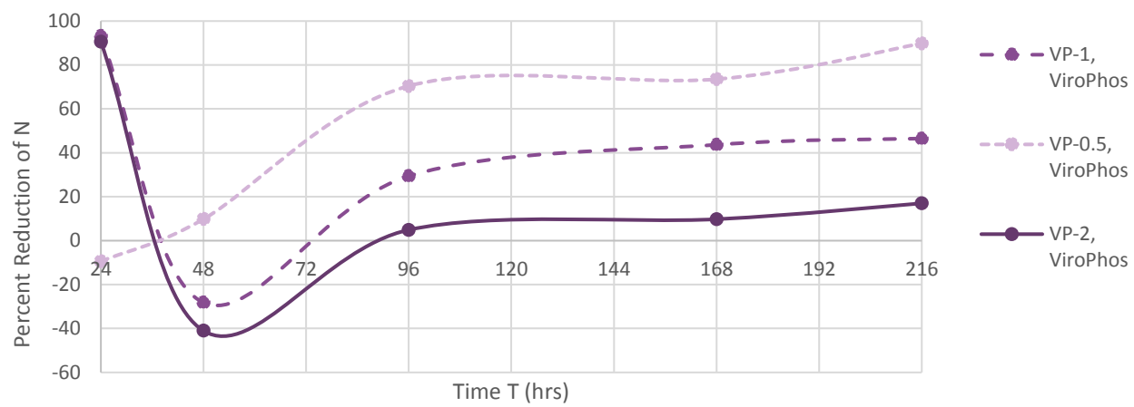
Figure A.13 – Average Percent Reduction of Ammonia using Treatment Alternative ViroPhos
