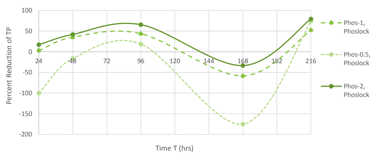
Figure A.12 – Average Percent Reduction of Total Phosphorus Using Treatment Alternative Phoslock
