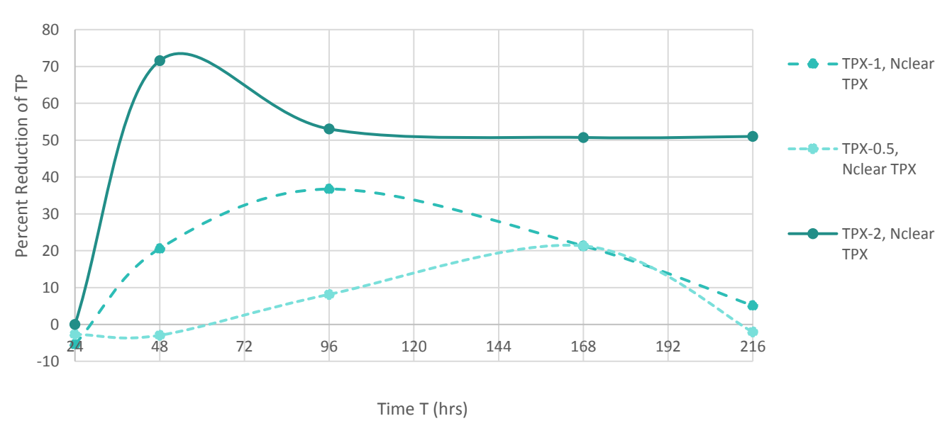
Figure A.12 – Average Percent Reduction of Total Phosphorus Using Treatment Alternative Phoslock
