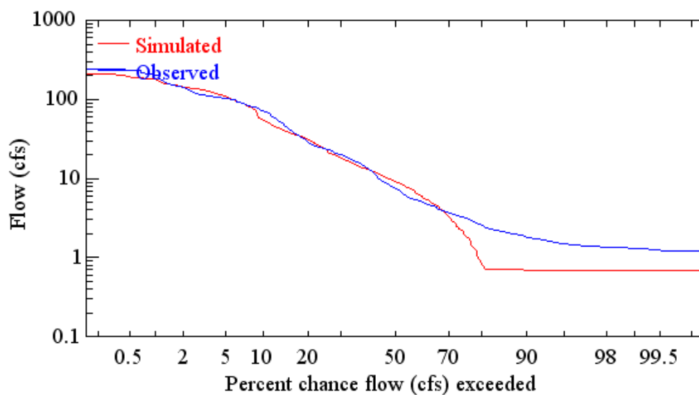
Figure B.18. Observed and simulated daily flow frequency curves for Howell Creek near Slavia (10/1997 – 09/1999).
