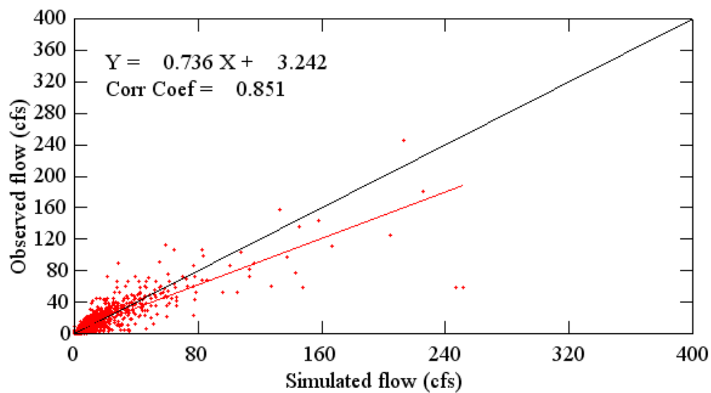
Figure B.15. Scatter plots of observed and simulated daily flows for Soldier Creek near Longwood (10/1999 – 09/2003).
