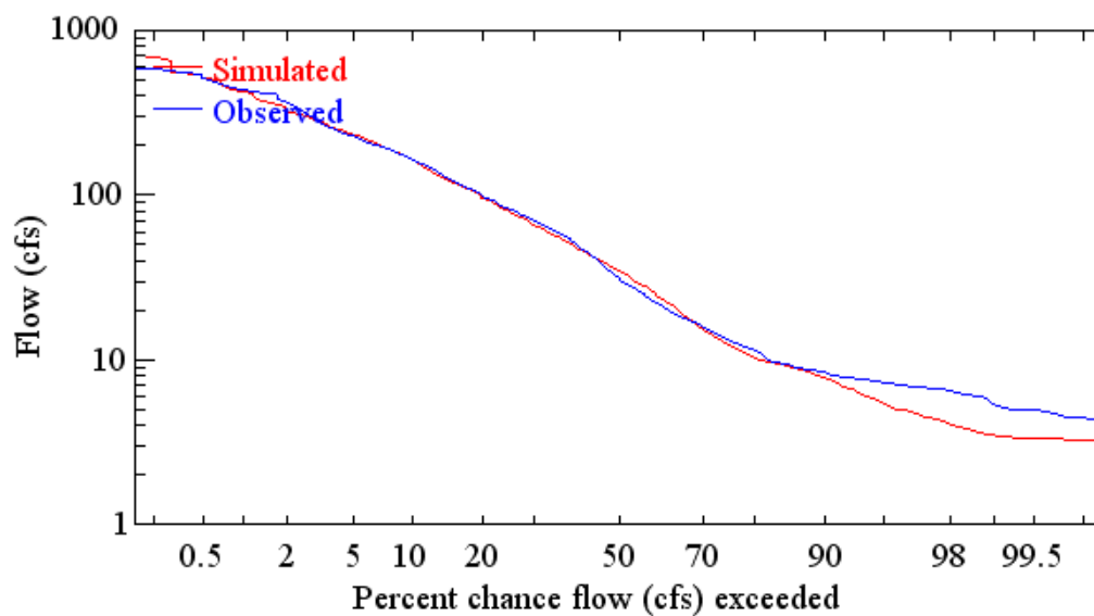
Figure B.6. Observed and simulated daily flow frequency curves for Howell Creek near Oviedo (10/1999 – 09/2003).
