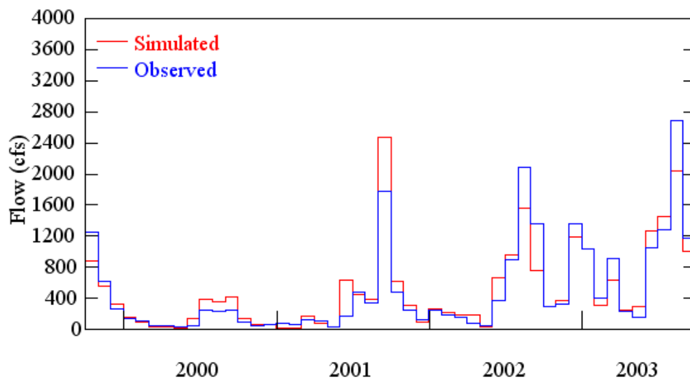
Figure B.9. Observed and simulated monthly flows for Gee Creek near Longwood (10/1999 – 09/2003).
