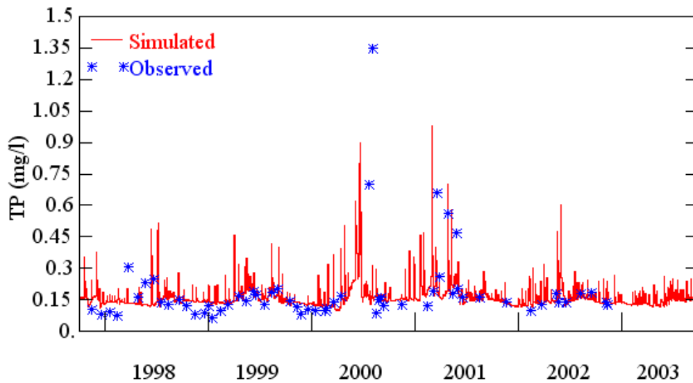
Figure 3.13. Observed and simulated TP concentrations for Soldier Creek near Longwood (10/1997 – 09/2003).
