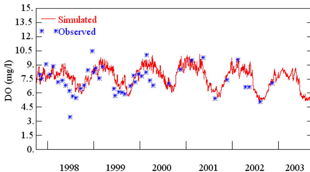
Figure C.3. Observed and simulated DO concentrations for Howell Creek near Oviedo (10/1997 – 09/2003).
