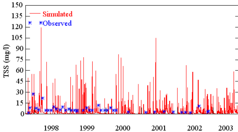
Figure C.9. Observed and simulated TSS concentrations for Gee Creek near Longwood (10/1997 – 09/2003).
