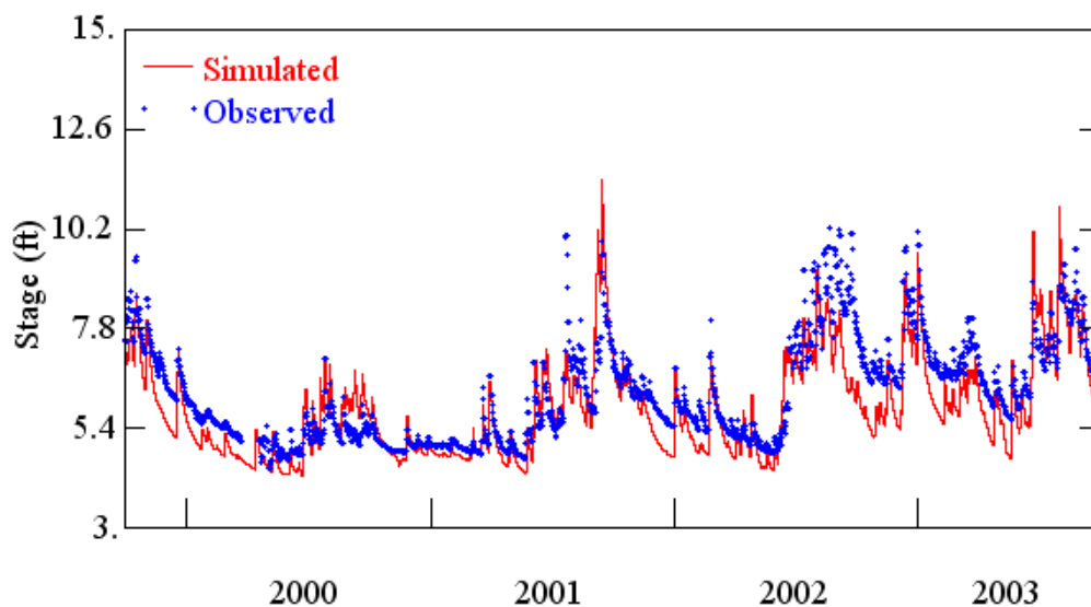
Figure B.8. Observed and simulated daily stages for Howell Creek near Oviedo (10/1999 – 09/2003).
