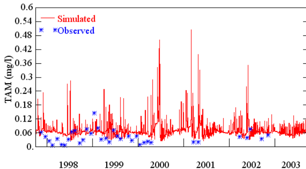
Figure C.18. Observed and simulated TAM concentrations for Soldier Creek near Longwood (10/1997 – 09/2003).
