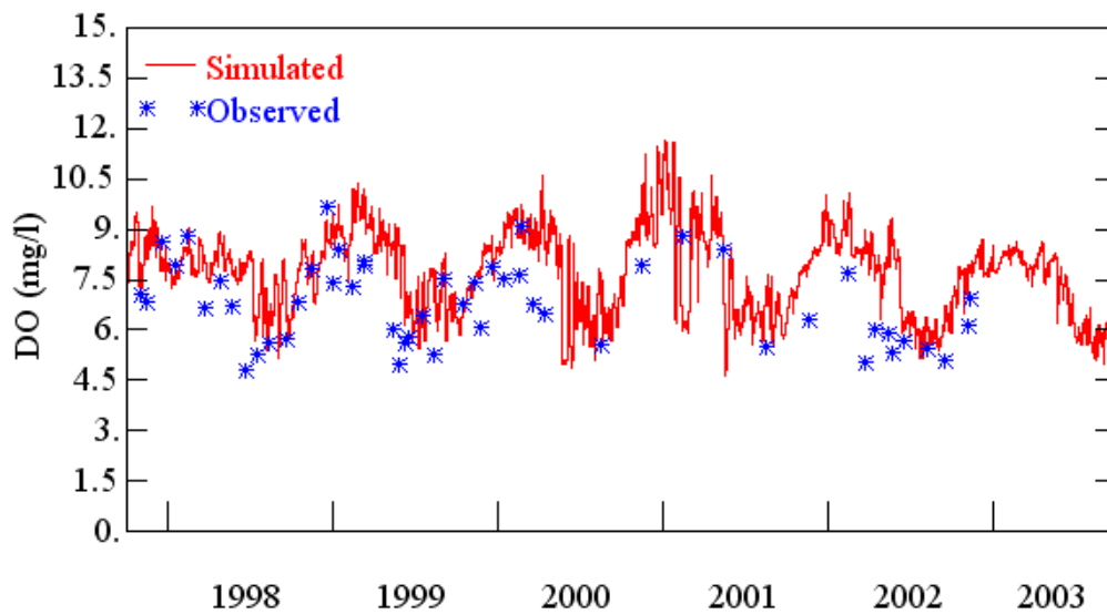
Figure C.10. Observed and simulated DO concentrations for Gee Creek near Longwood (10/1997 – 09/2003).
