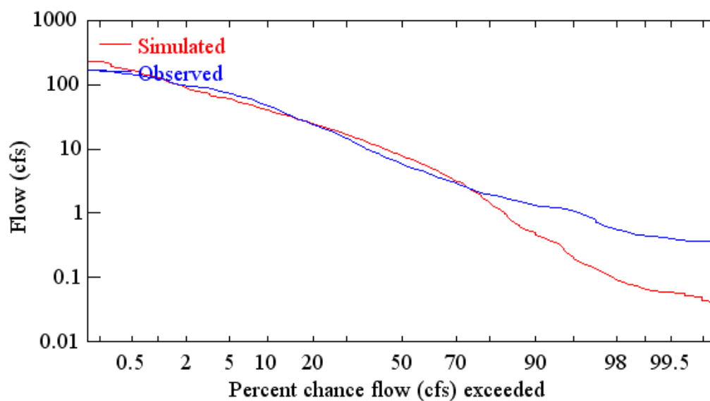
Figure B.10. Observed and simulated daily flow frequency curves for Gee Creek near Longwood (10/1999 – 09/2003).
