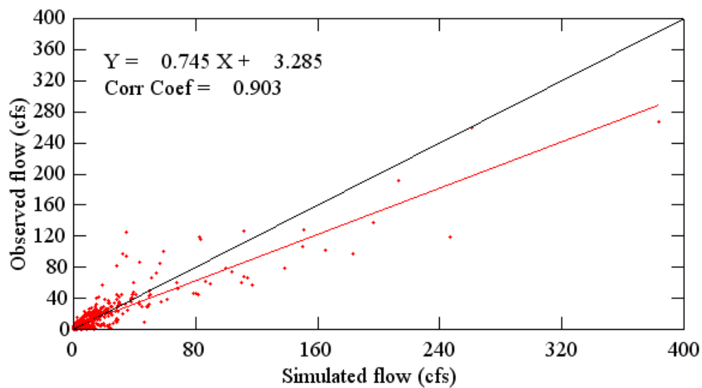
Figure B.27. Scatter plots of observed and simulated daily flows for Soldier Creek near Longwood (10/1997 – 09/1999).
