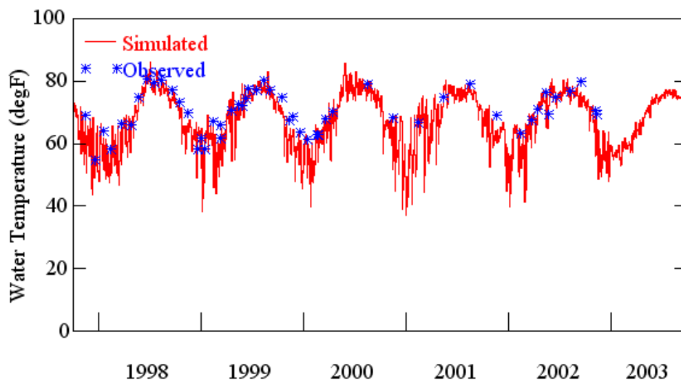
Figure C.15. Observed and simulated water temperature for Soldier Creek near Longwood (10/1997 – 09/2003).
