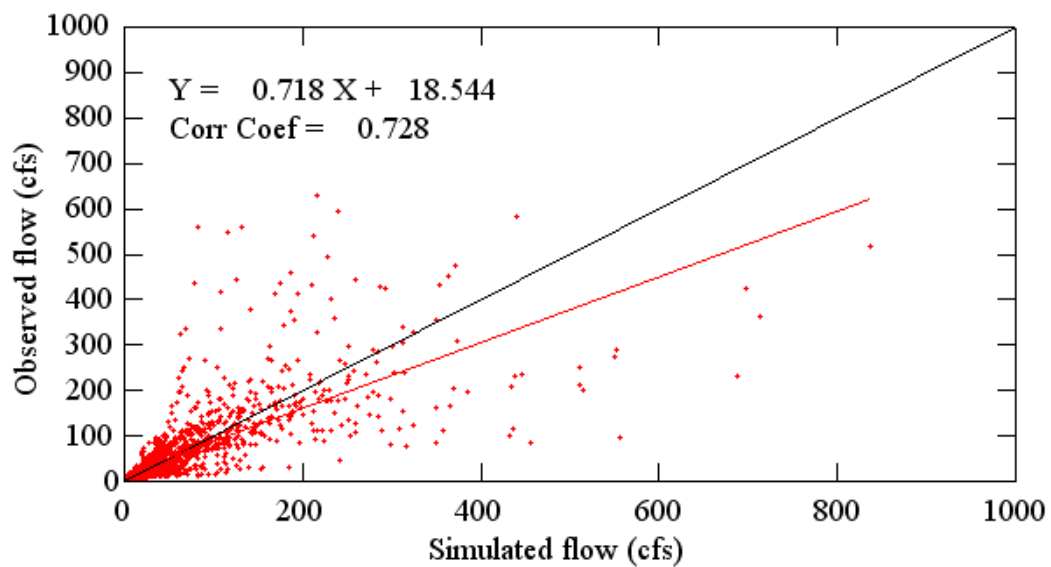
Figure B.7. Scatter plots of observed and simulated daily flows for Howell Creek near Oviedo (10/1999 – 09/2003).
