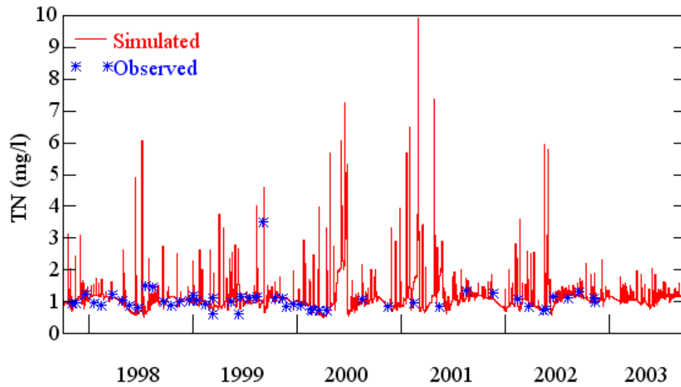
Figure 3.10. Observed and simulated TN concentrations for Gee Creek near Londwood (10/1997 – 09/2003).
