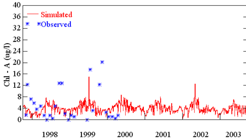
Figure C.7. Observed and simulated Chl – A concentrations for Howell Creek near Oviedo (10/1997 – 09/2003).
