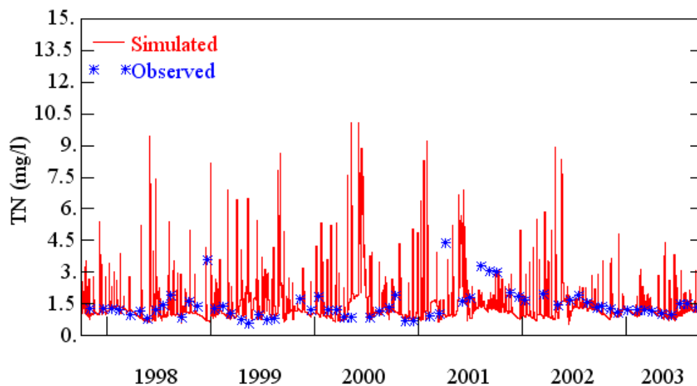
Figure 3.14. Observed and simulated TN concentrations for Six Mile Creek (10/1997 – 09/2003).
