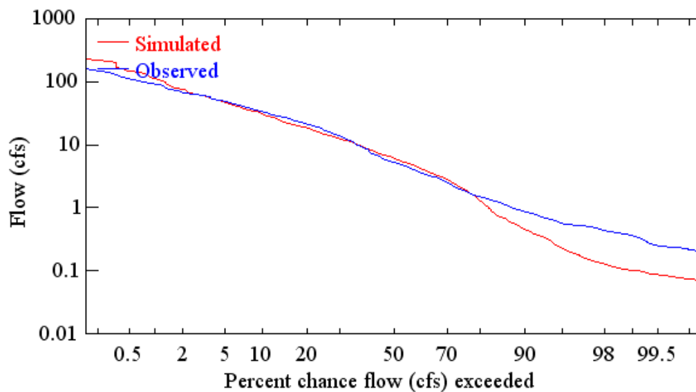
Figure B.14. Observed and simulated daily flow frequency curves for Soldier Creek near Longwood (10/1999 – 09/2003).
