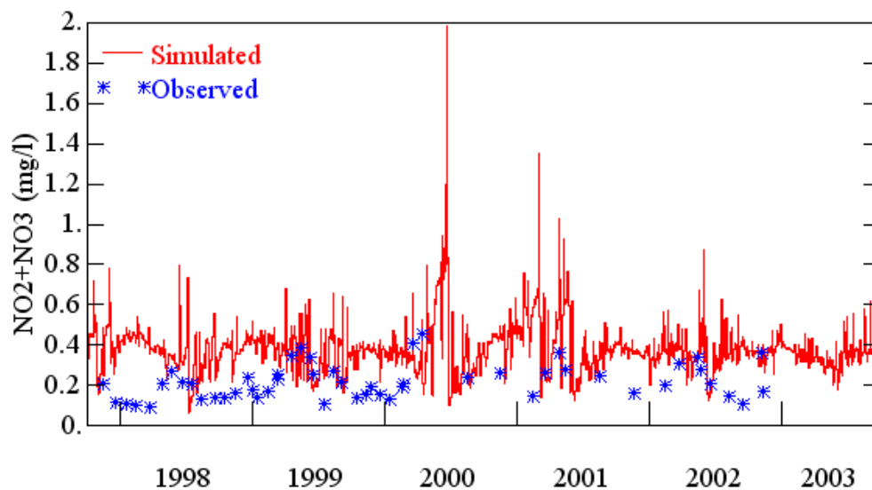
Figure C.19. Observed and simulated NO 2 +NO 3 concentrations for Soldier Creek near Longwood (10/1997 – 09/2003).
