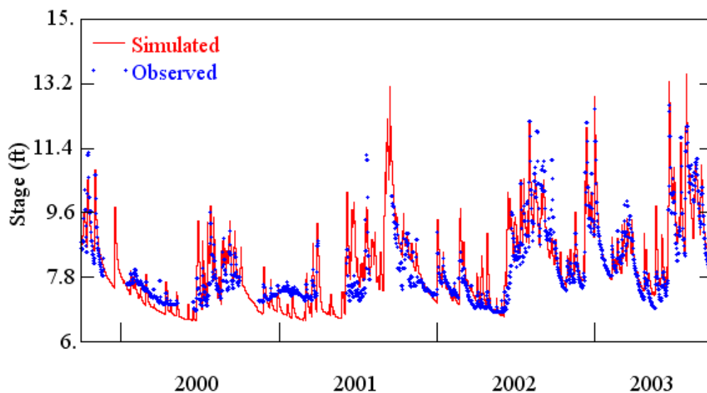
Figure B.12. Observed and simulated daily stages for Gee Creek near Longwood (10/1999 – 09/2003).
