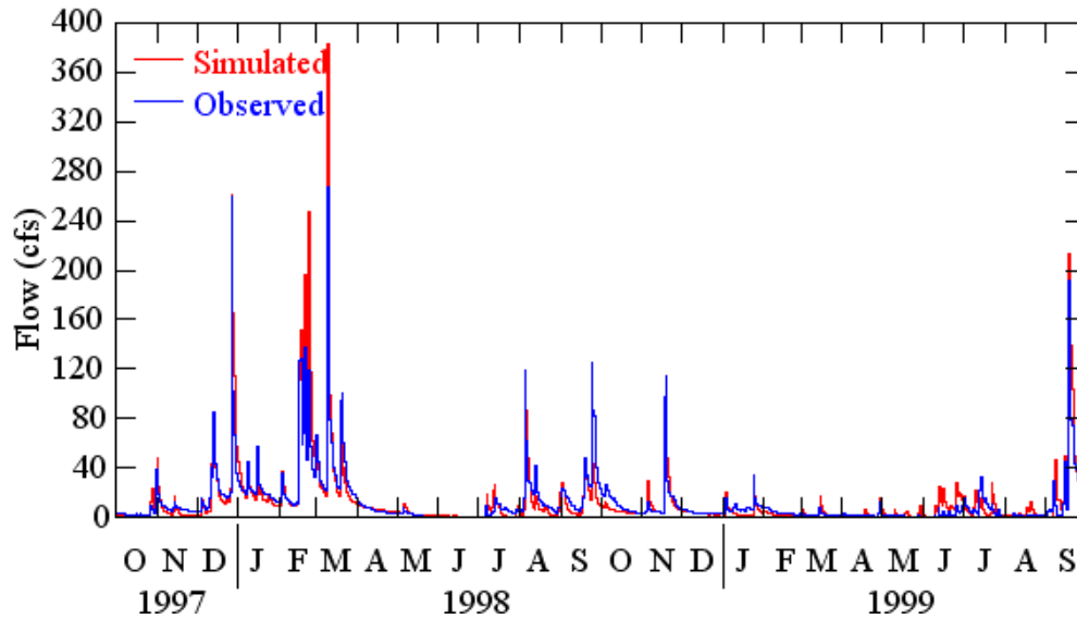
Figure 3.7. Observed and simulated daily flows for Soldier Creek near Longwood (10/1997 – 09/1999).
