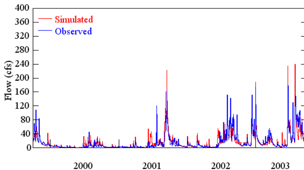
Figure 3.3. Observed and simulated daily flows for Gee Creek near Longwood (10/1999 – 09/2003).
