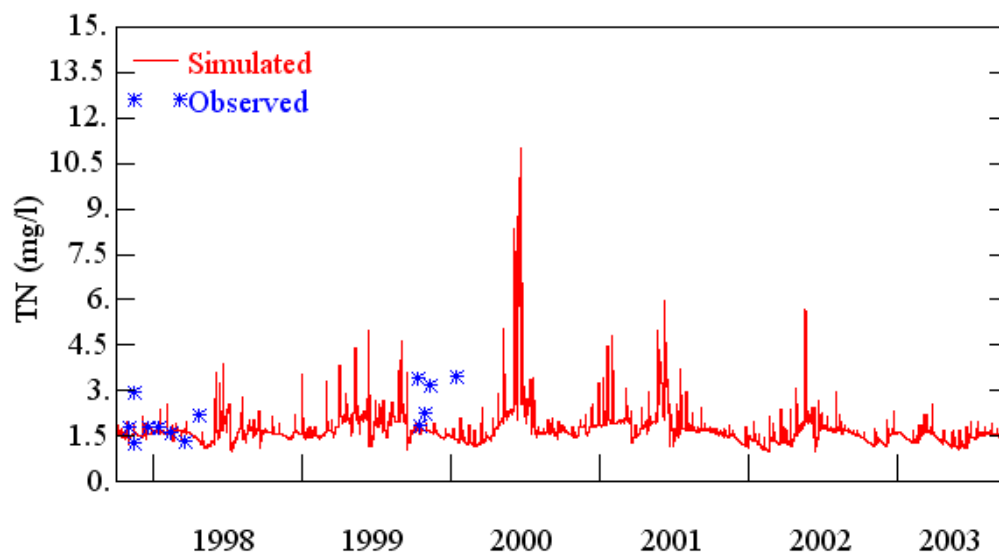
Figure 3.18. Observed and simulated TN concentrations for Chub Creek (10/1997 – 09/2003).
