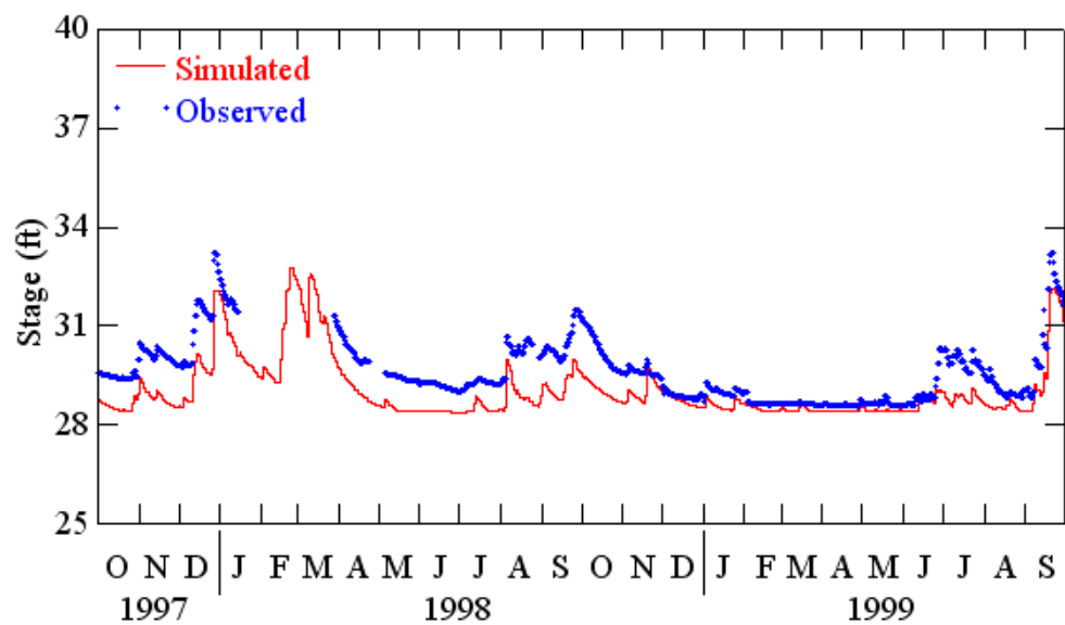
Figure B.20. Observed and simulated daily stages for Howell Creek near Slavia (10/1997 – 09/1999).
