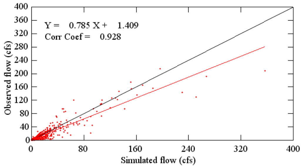
Figure B.23. Scatter plots of observed and simulated daily flows for Gee Creek near Longwood (10/1997 – 09/1999).
