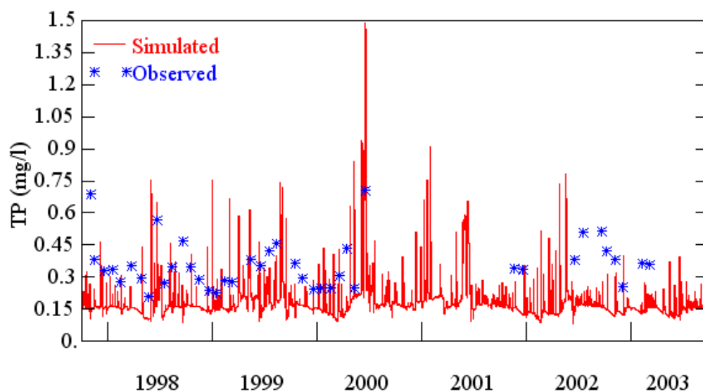
Figure 3.25. Observed and simulated TP concentrations for Solary Canal (10/1997 – 09/2003).
