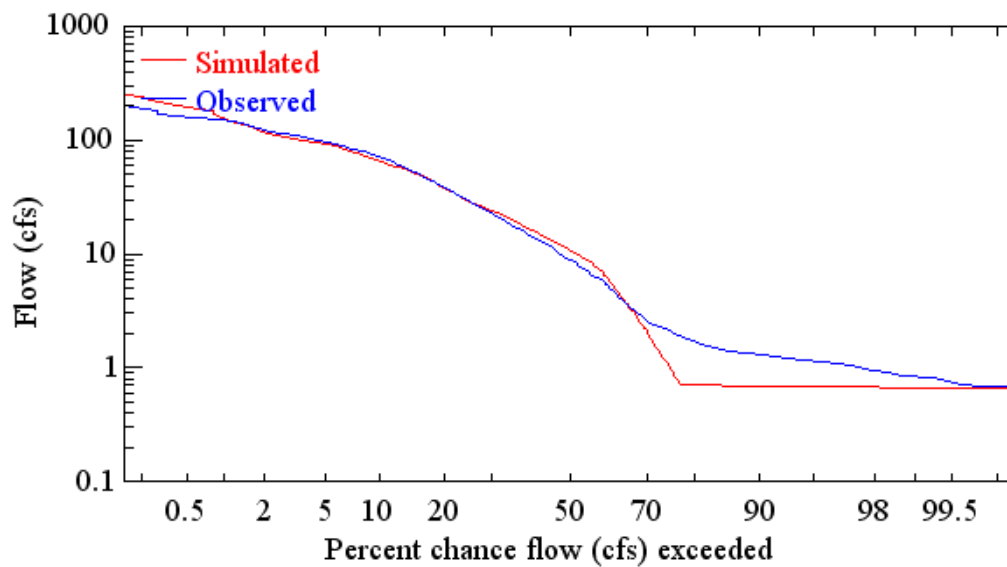
Figure B.2. Observed and simulated daily flows frequency curves for Howell Creek near Slavia (10/1999 – 09/2003).
