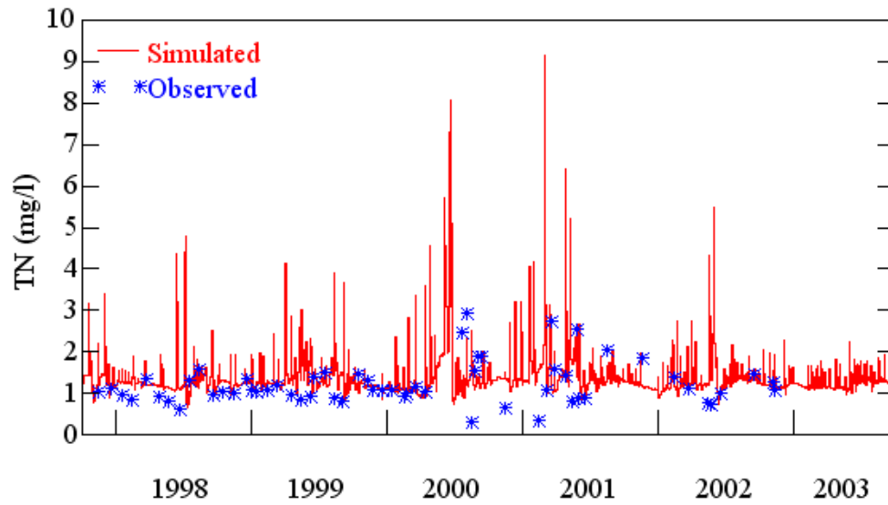
Figure 3.12. Observed and simulated TN concentrations for Soldier Creek near Longwood (10/1997 – 09/2003).
