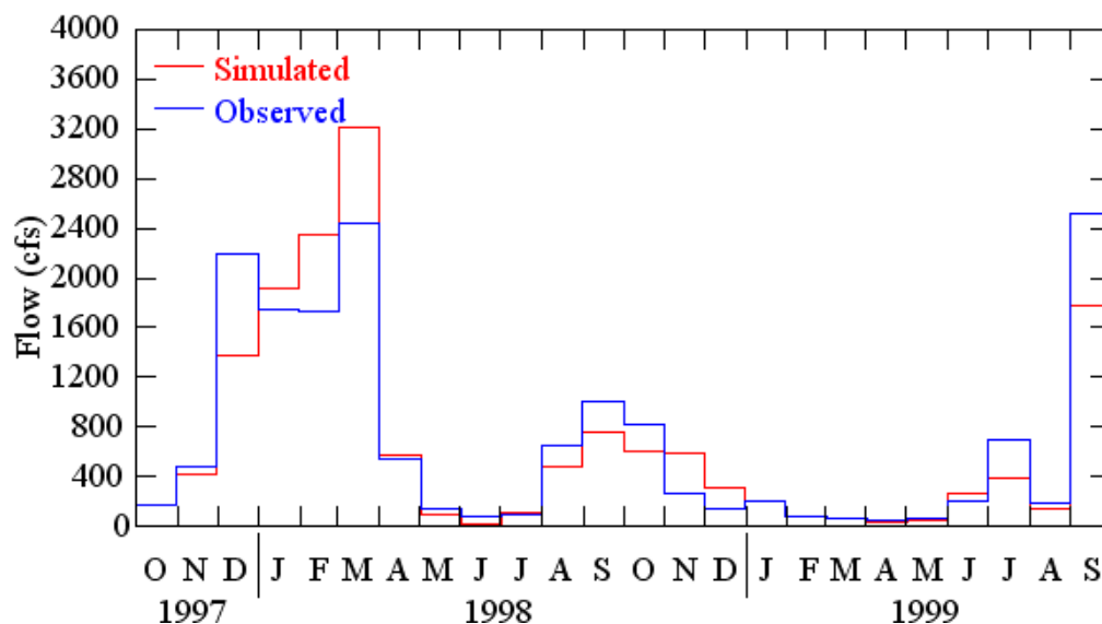
Figure B.17. Observed and simulated monthly flows for Howell Creek near Slavia (10/1997 – 09/1999).
