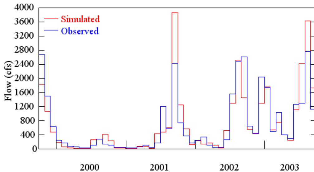
Figure B.1. Observed and simulated monthly flows for Howell Creek near Slavia (10/1999 – 09/2003).
