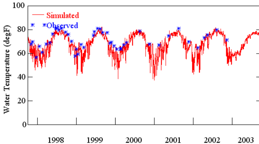
Figure C.1. Observed and simulated water temperature for Howell Creek near Oviedo (10/1997 – 09/2003).
