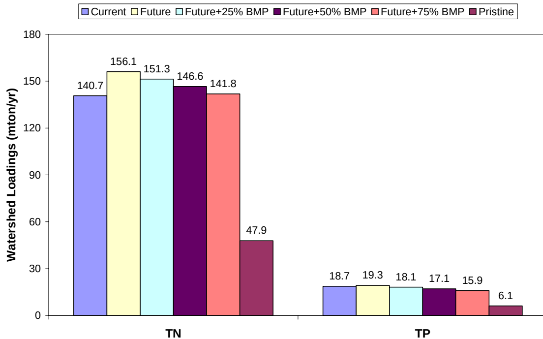
Figure 4.1. Comparison of average annual TN and TP loads to Lake Jesup for the six simulated scenarios.
