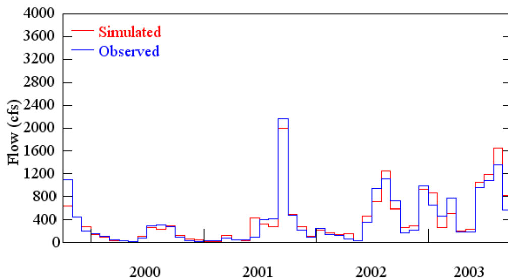
Figure B.13. Observed and simulated monthly flows for Soldier Creek near Longwood (10/1999 – 09/2003).
