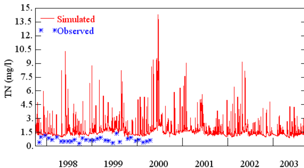
Figure 3.16. Observed and simulated TN concentrations for Navy Canal (10/1997 – 09/2003).
