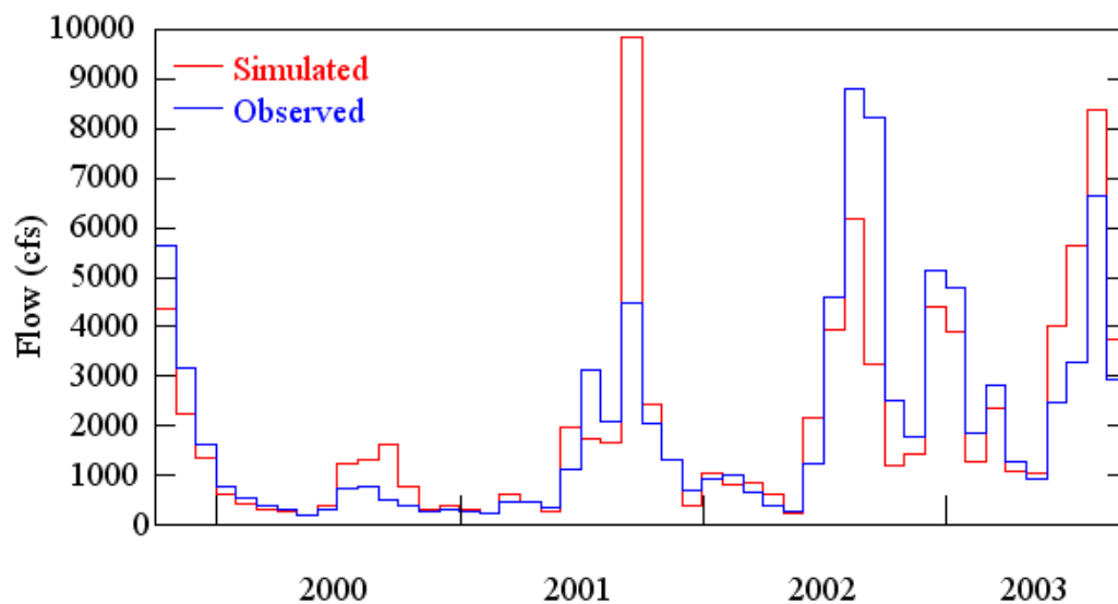
Figure B.5. Observed and simulated monthly flows for Howell Creek near Oviedo (10/1999 – 09/2003).
