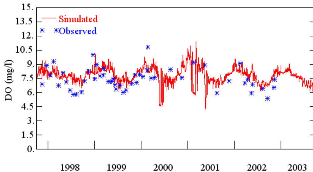
Figure C.17. Observed and simulated DO concentrations for Soldier Creek near Longwood (10/1997 – 09/2003).
