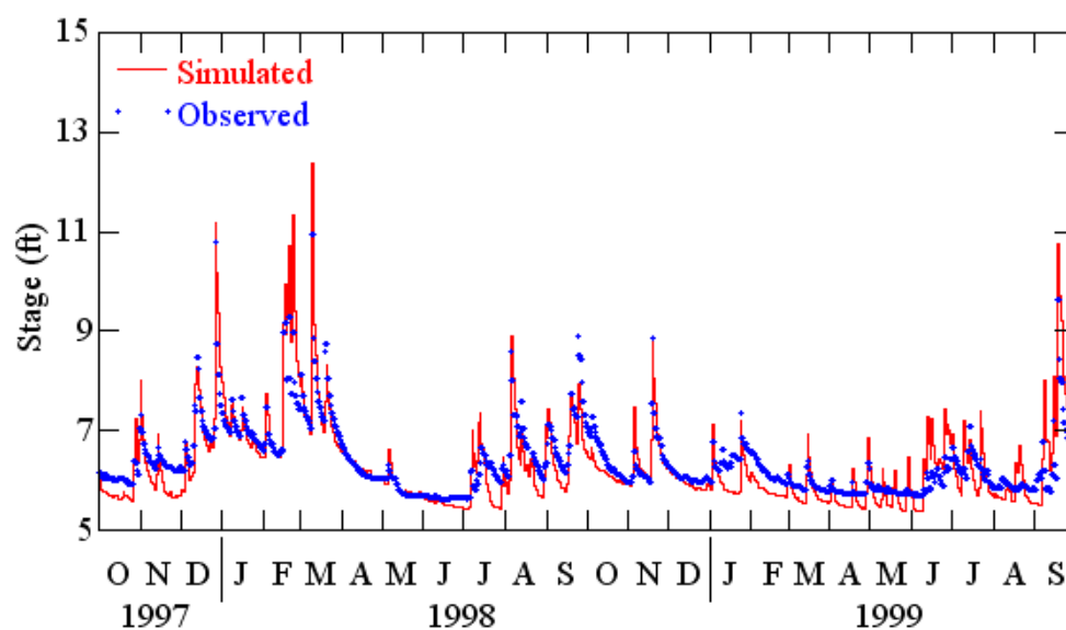
Figure B.28. Observed and simulated daily stages for Gee Creek near Longwood (10/1997 – 09/1999).
