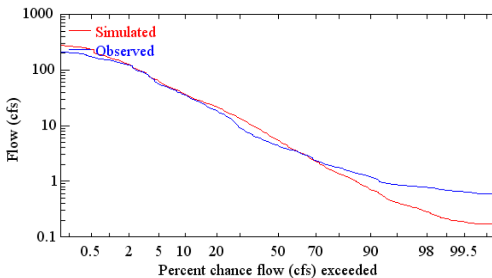
Figure B.22. Observed and simulated daily flow frequency curves for Gee Creek near Longwood (10/1997 – 09/1999).
