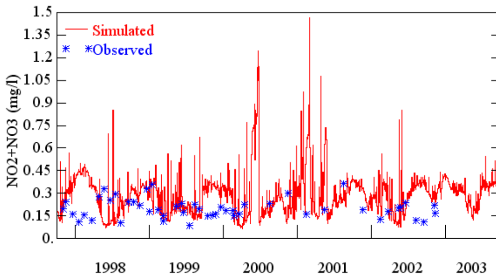
Figure C.12. Observed and simulated NO 2 +NO 3 concentrations for Gee Creek near Longwood (10/1997 – 09/2003).
