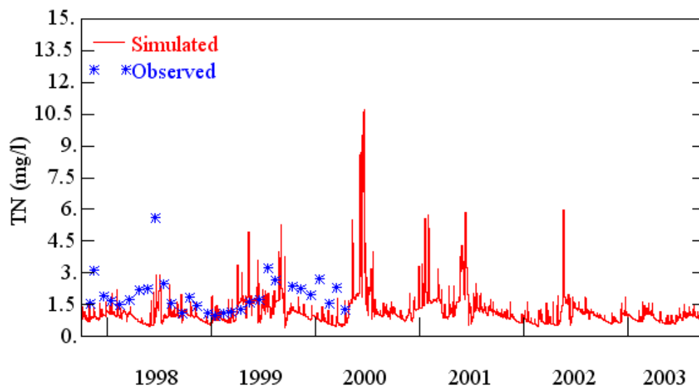
Figure 3.20. Observed and simulated TN concentrations for Salt Creek (10/1997 – 09/2003).
