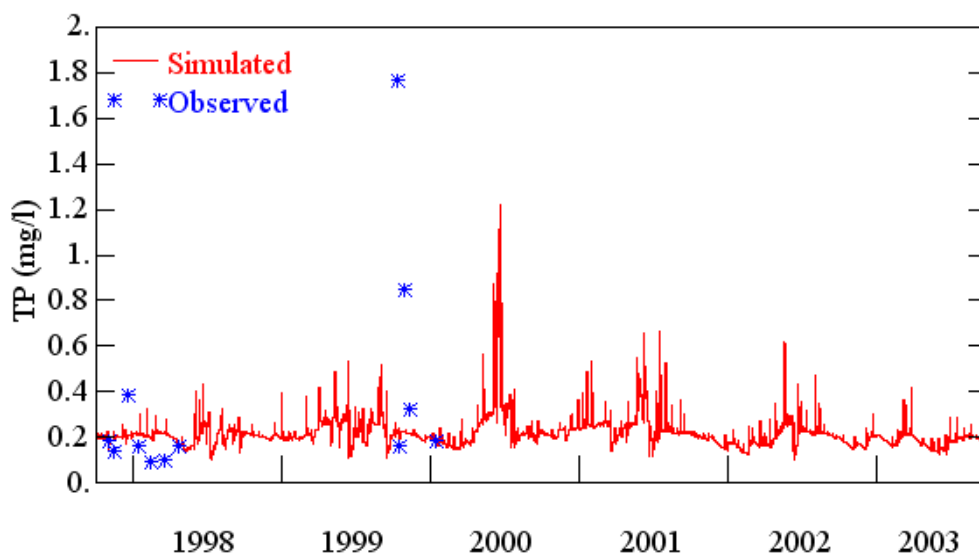
Figure 3.19. Observed and simulated TP concentrations for Chub Creek (10/1997 – 09/2003).
