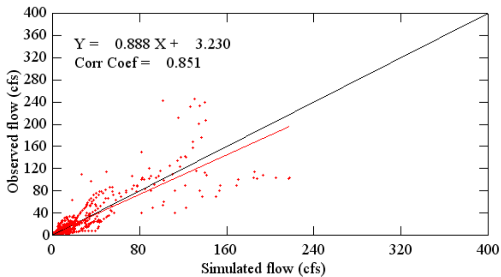
Figure B.19. Scatter plots of observed and simulated daily flows for Howell Creek near Slavia (10/1997 – 09/1999).
