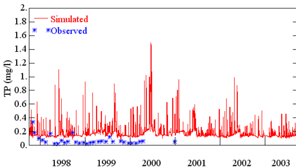
Figure 3.17. Observed and simulated TP concentrations for Navy Canal (10/1997 – 09/2003).
