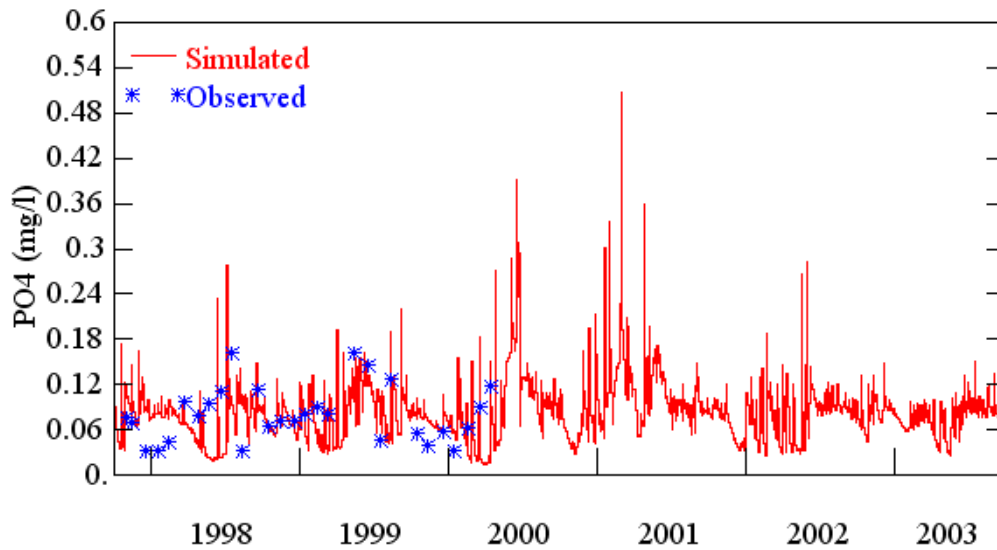
Figure C.13. Observed and simulated PO4 concentrations for Gee Creek near Longwood (10/1997 – 09/2003).
