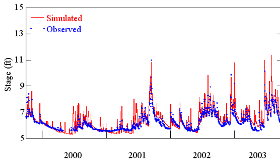
Figure B.16. Observed and simulated daily stages for Soldier Creek near Longwood (10/1999 – 09/2003).
