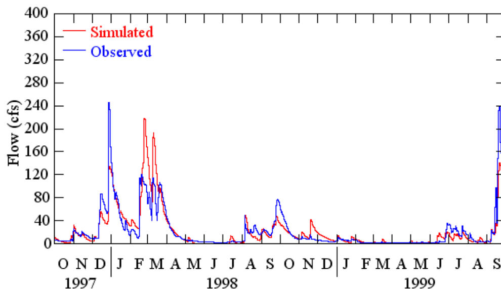
Figure 3.5. Observed and simulated daily flows for Howell Creek near Slavia (10/1997 – 09/1999).
