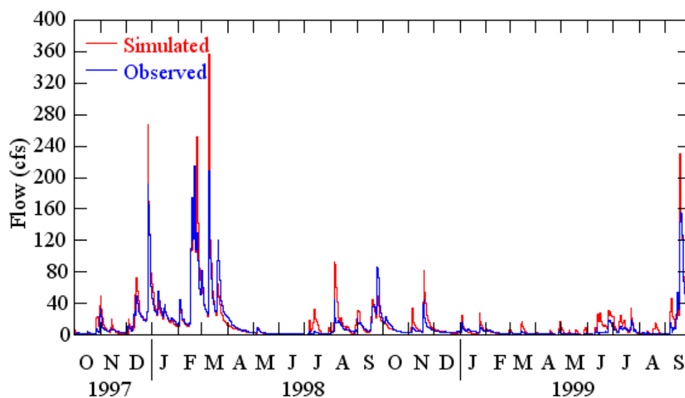
Figure 3.6. Observed and simulated daily flows for Gee Creek near Longwood (10/1997 – 09/1999).
