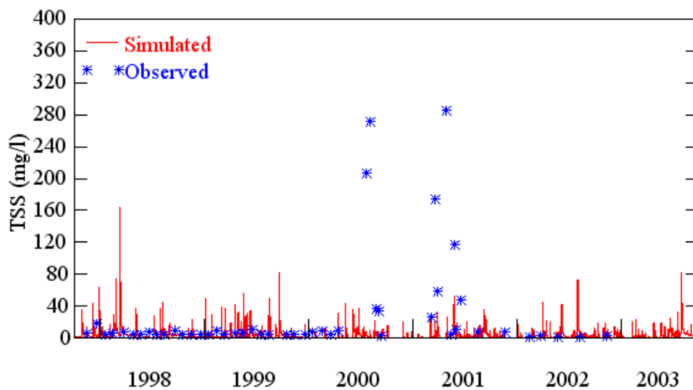
Figure C.16. Observed and simulated TSS concentrations for Soldier Creek near Longwood (10/1997 – 09/2003).
