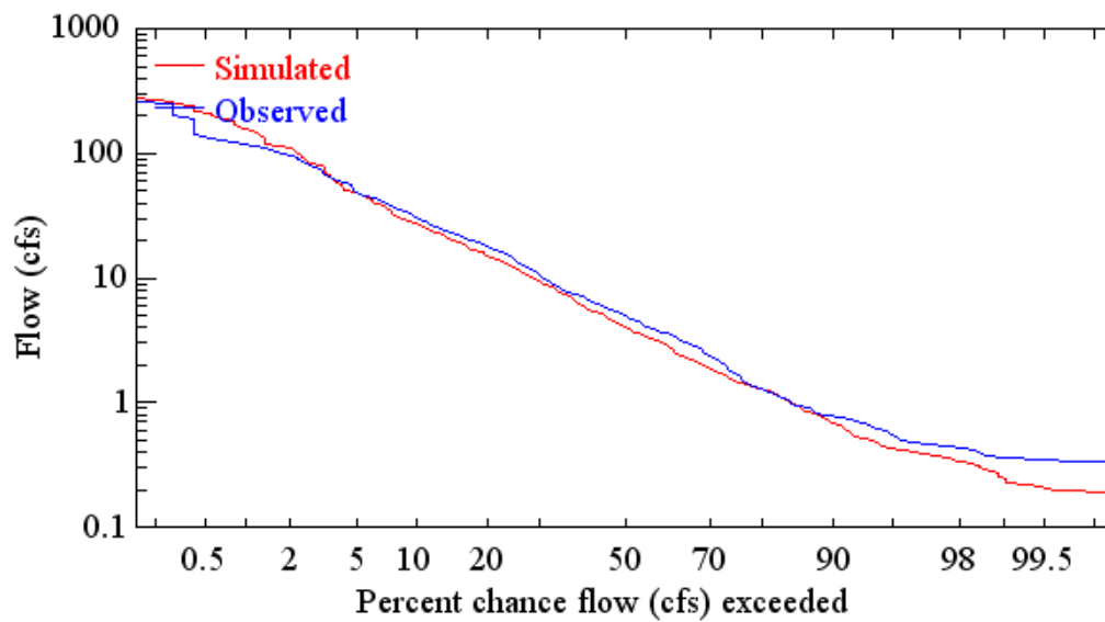
Figure B.26. Observed and simulated daily flow frequency curves for Soldier Creek near Longwood (10/1997 – 09/1999).
