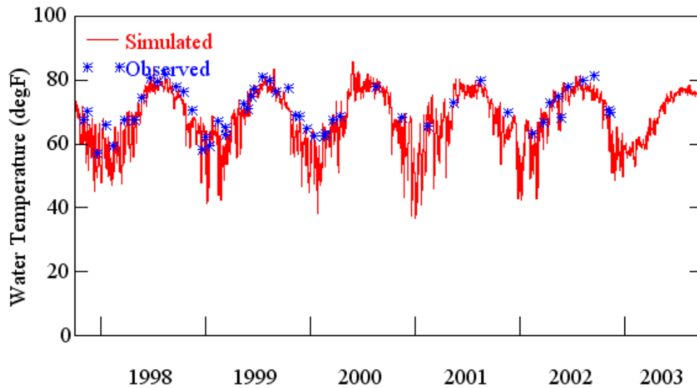
Figure C.8. Observed and simulated water temperature for Gee Creek near Longwood (10/1997 – 09/2003).
