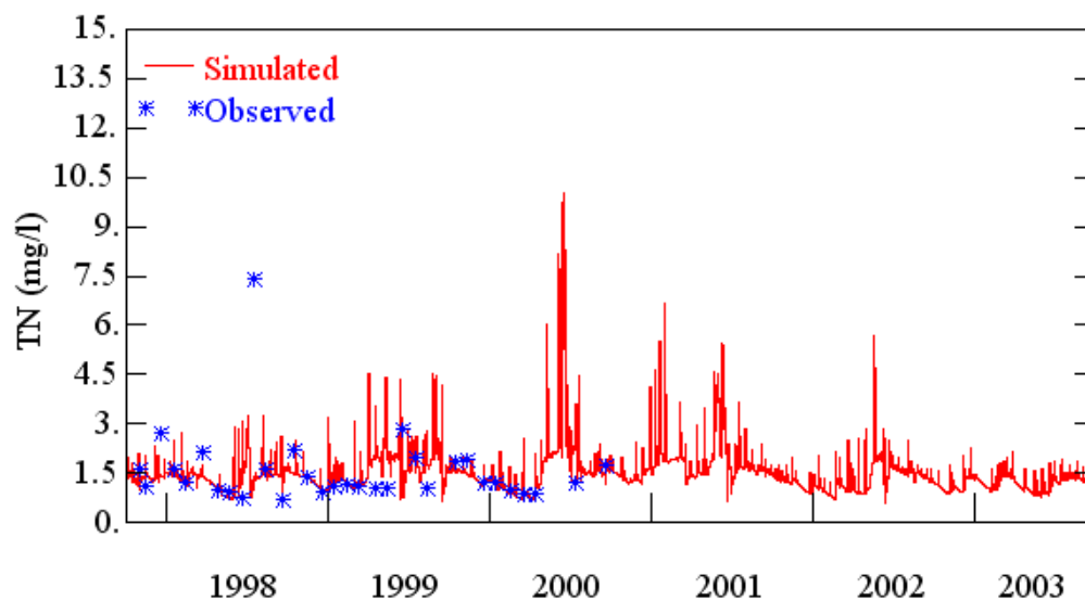
Figure 3.22. Observed and simulated TN concentrations for Sweetwater Creek (10/1997 – 09/2003).
