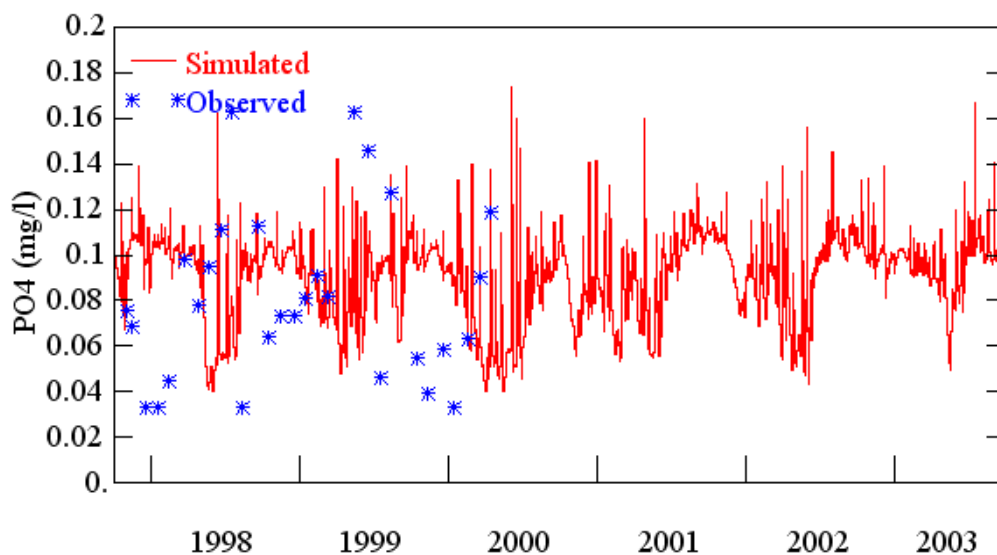
Figure C.6. Observed and simulated PO 4 concentrations for Howell Creek near Oviedo (10/1997 – 09/2003).
