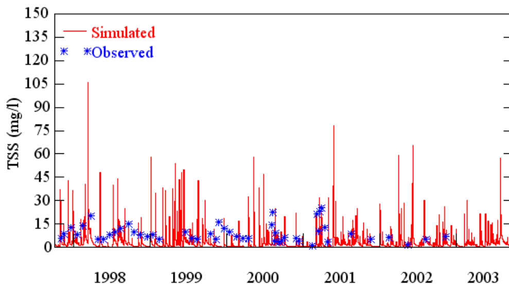
Figure C.2. Observed and simulated TSS concentrations for Howell Creek near Oviedo (10/1997 – 09/2003).
