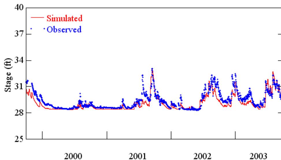
Figure B.4. Observed and simulated daily stages for Howell Creek near Slavia (10/1999 – 09/2003).
