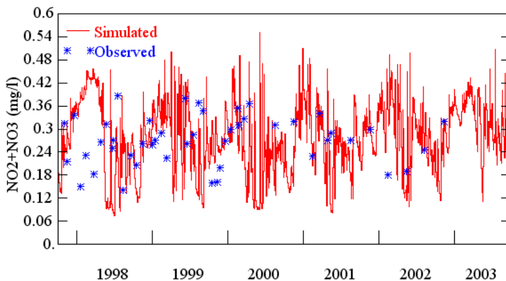
Figure C.5. Observed and simulated NO 2 +NO 3 concentrations for Howell Creek near Oviedo (10/1997 – 09/2003).
