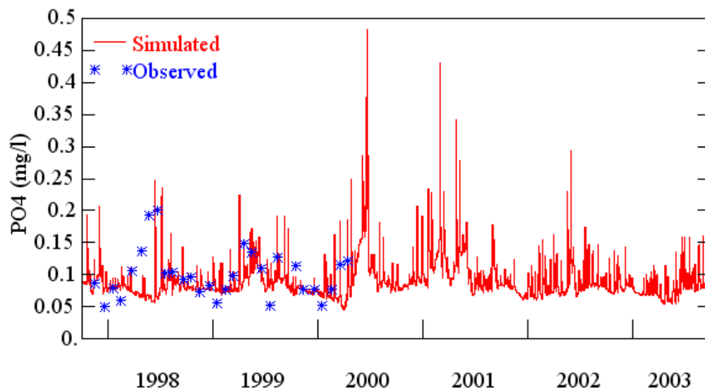
Figure C.20. Observed and simulated PO 4 concentrations for Soldier Creek near Longwood (10/1997 – 09/2003).
