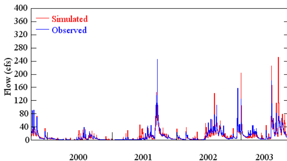
Figure 3.4. Observed and simulated daily flows for Soldier Creek near Longwood (10/1999 – 09/2003).
