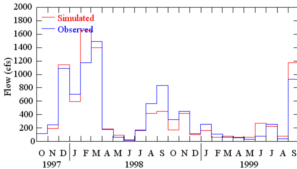
Figure B.25. Observed and simulated monthly flows for Soldier Creek near Longwood (10/1997 – 09/1999).
