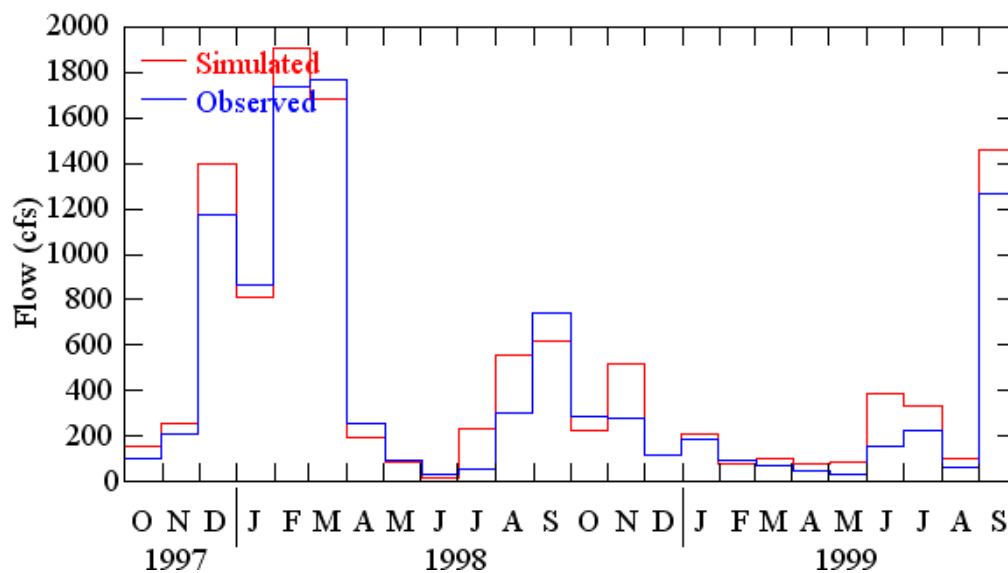
Figure B.21. Observed and simulated monthly flows for Gee Creek near Longwood (10/1997 – 09/1999).
