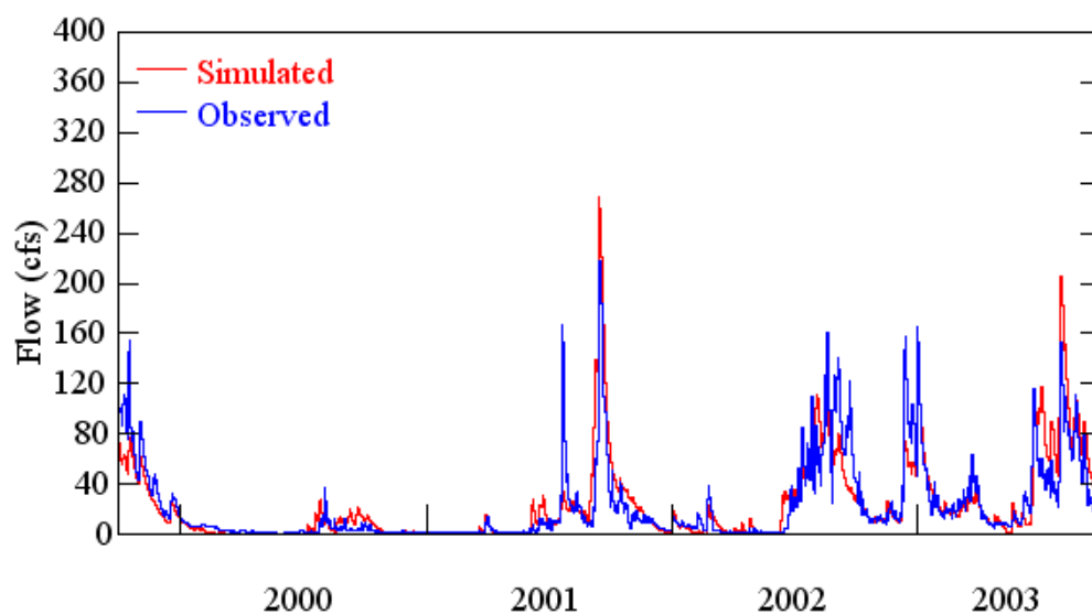
Figure 3.2. Observed and simulated daily flows for Howell Creek near Slavia (10/1999 – 09/2003).
