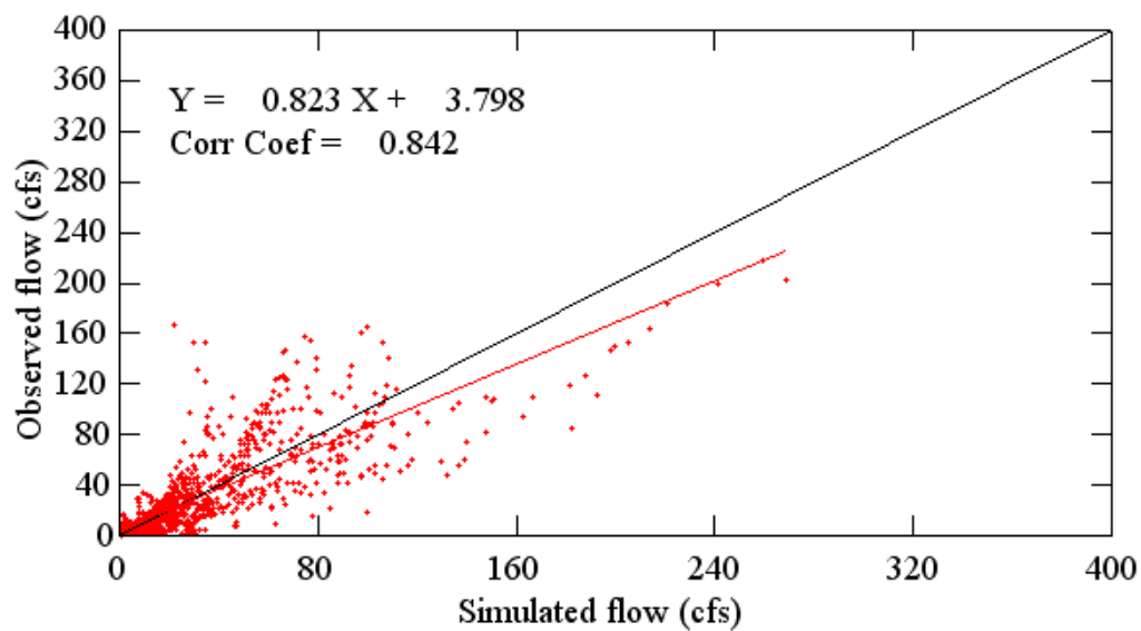
Figure B.3. Scatter plots of observed and simulated daily flows for Howell Creek near Slavia (10/1999 – 09/2003).
