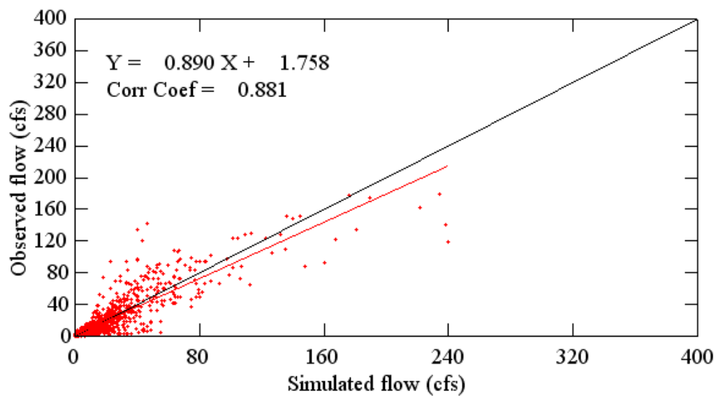
Figure B.11. Scatter plots of observed and simulated daily flows for Gee Creek near Longwood (10/1999 – 09/2003).
