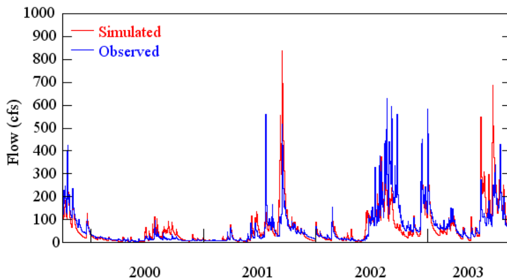
Figure 3.1. Observed and simulated daily flows for Howell Creek near Oviedo (10/1999 – 09/2003).
