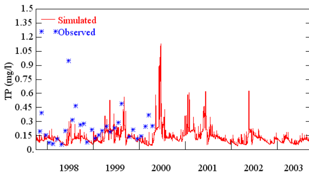
Figure 3.21. Observed and simulated TP concentrations for Salt Creek (10/1997 – 09/2003).
