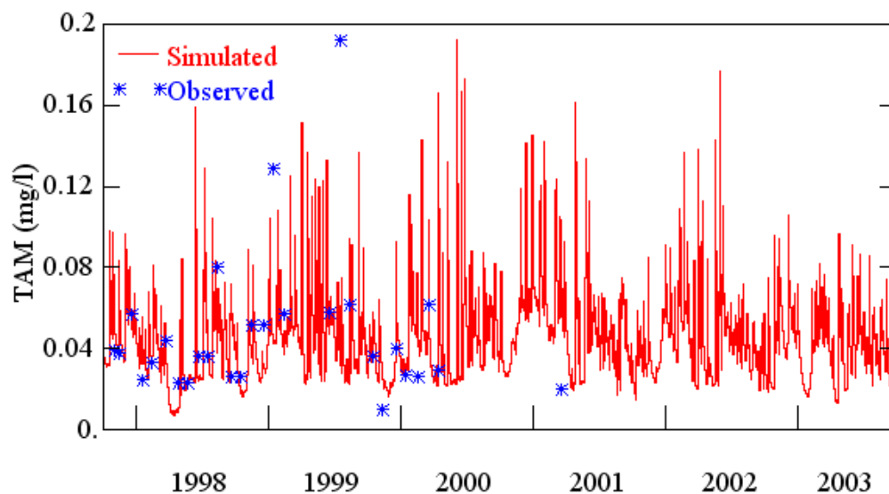
Figure C.4. Observed and simulated TAM concentrations for Howell Creek near Oviedo (10/1997 – 09/2003).
