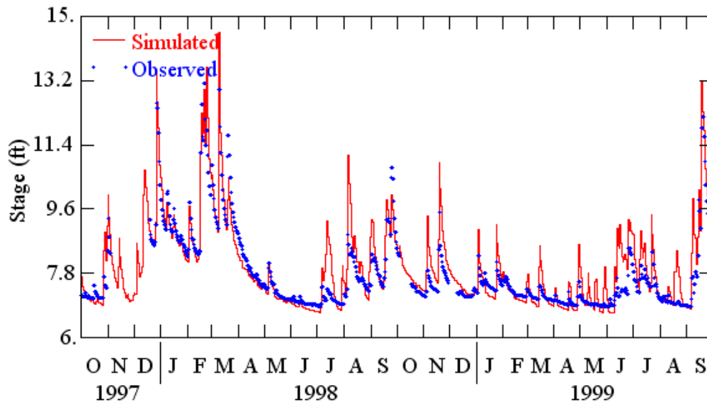
Figure B.24. Observed and simulated daily stages for Gee Creek near Longwood (10/1997 – 09/1999).
