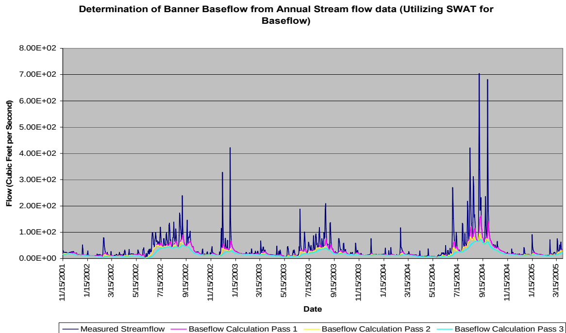
Figure 4.8. Base flow data obtained from Banner Dam USGS data, utilizing the SWAT Baseflow program.
