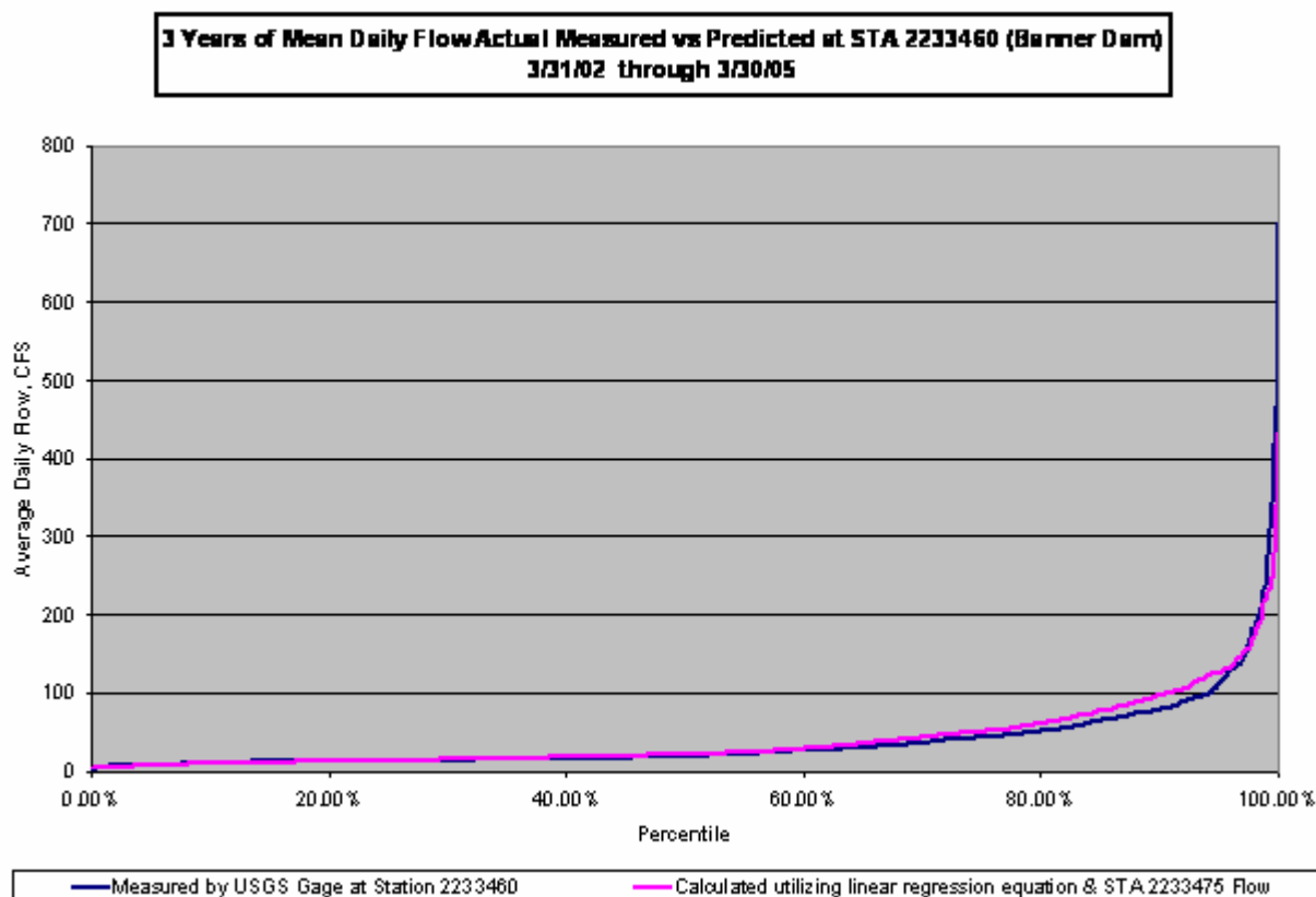
Figure 4.6b Analysis of 3 years of Predicted versus Actual Flow at STA 2233460 (Banner Dam).
