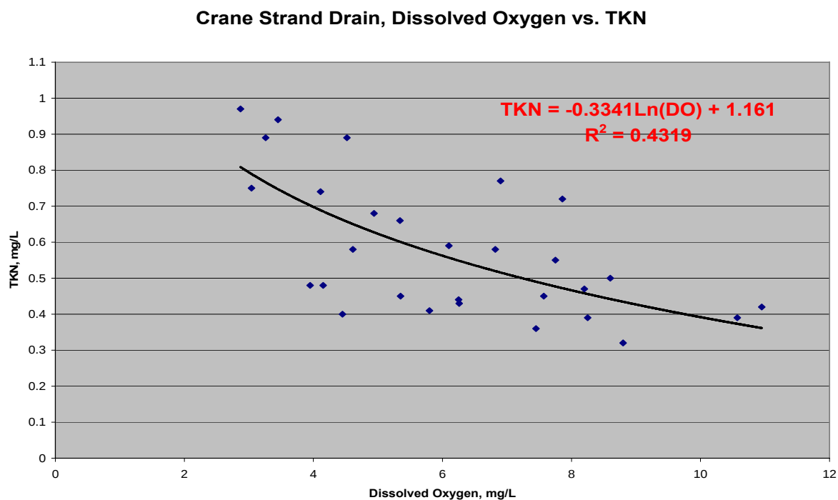
Figure 3.6. Relationship between DO and TKN
