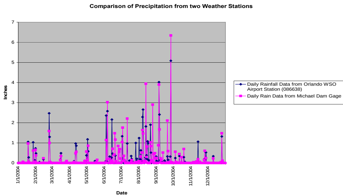
Figure 4.12 Comparison between weather data from Michael Dam and Orlando Airport Stations
