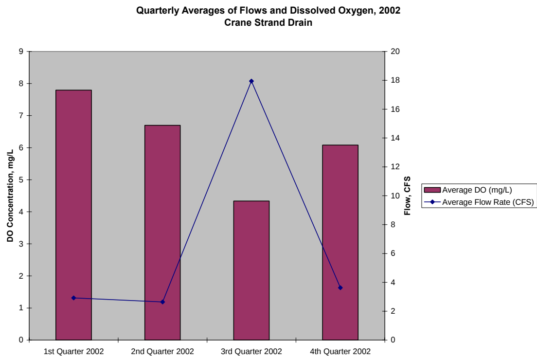
Figure 5.2. Relationship between Quarterly Average DO and Flow Rate
