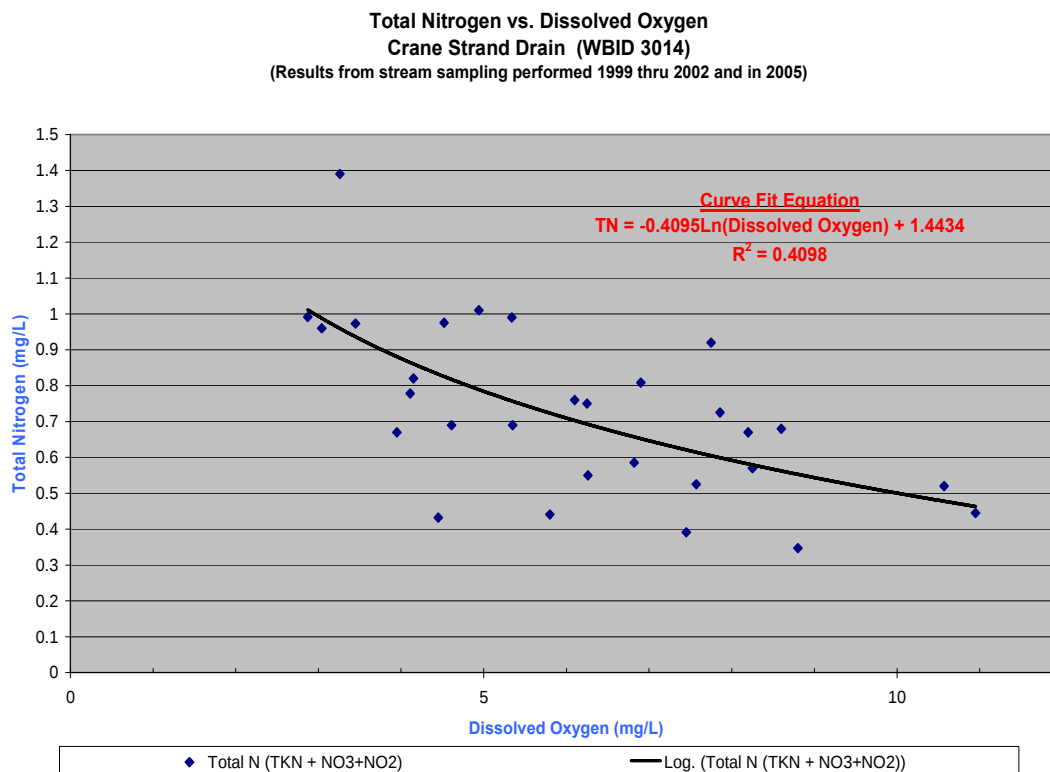
Figure 3.4. Relationship between DO and Total Nitrogen
