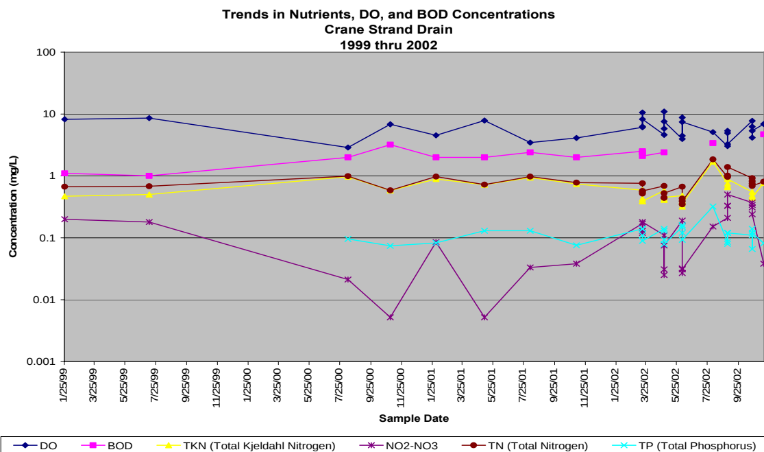
Figure 3.3. Trends in Nutrient, DO, and BOD Concentrations, Crane Strand Drain
