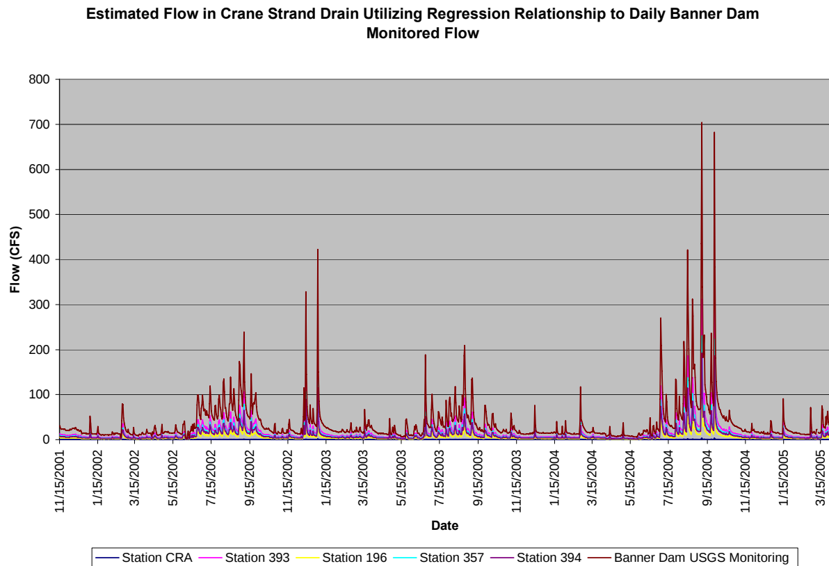
Figure 4.7 Utilizing Flow Data from USGS gage Station to generate 3 years of flow data for sampling stations within the Crane Strand Drain.
