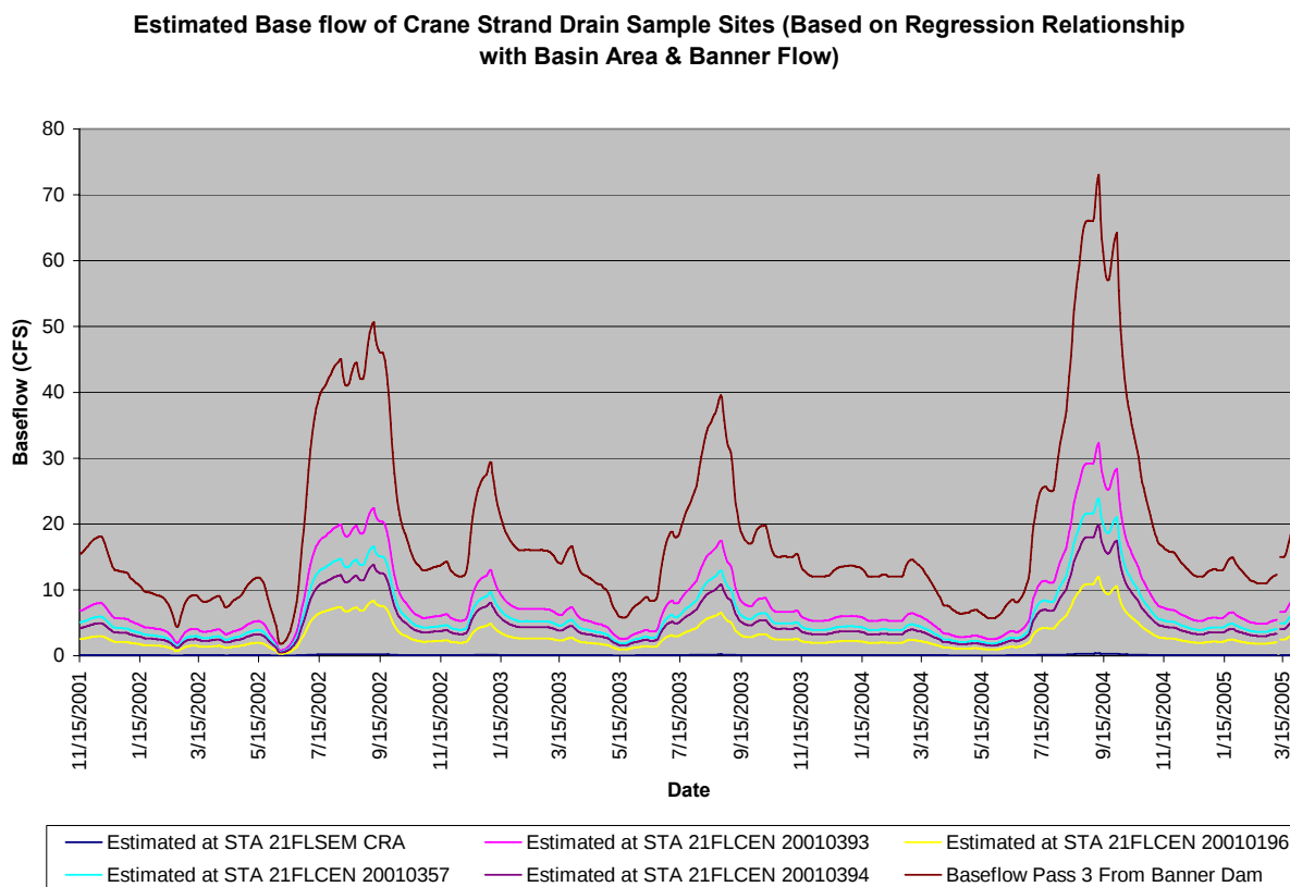
Figure 4.9. Base flow data obtained generated for Crane Strand Drain Sample Stations utilizing established flow relationship with Banner Dam flow.
