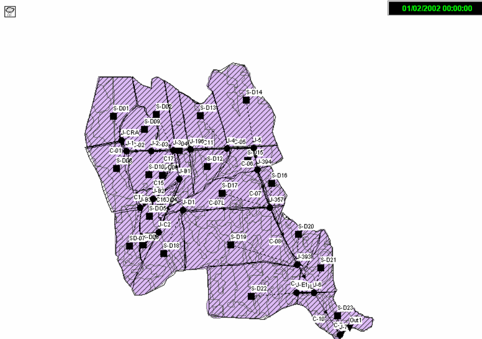
Figure 4.10 Basic Components of SWMM applied to Crane Strand Drain
