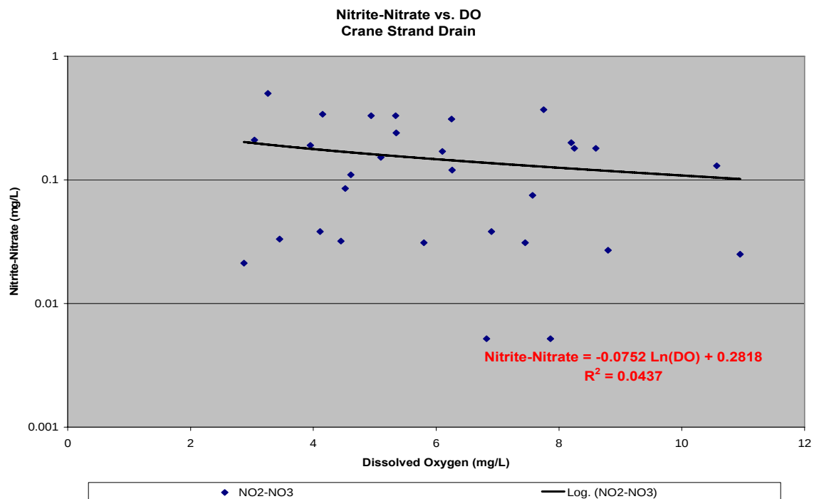
Figure 3.5. Relationship between DO and Nitrite-Nitrate
