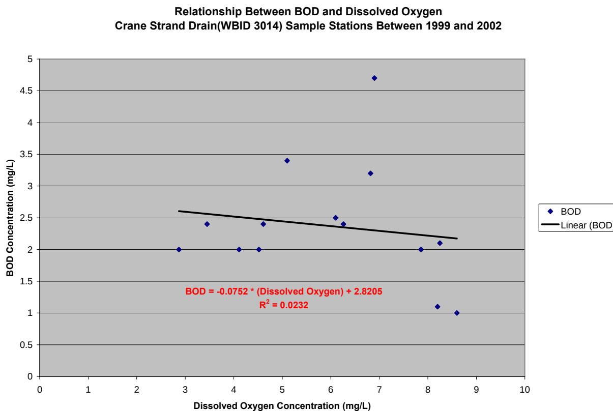
Figure 3.1. Relationship between DO and BOD
