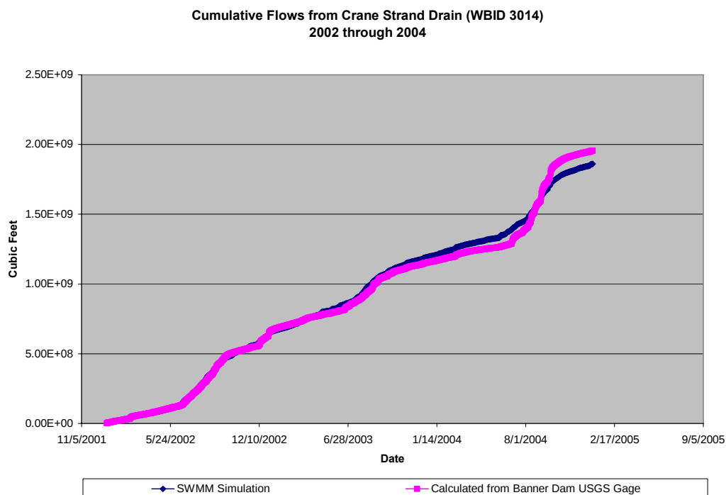
Figure 4.13 Modeling Cumulative Flow from Crane Strand Drain, 2002 through 2004
