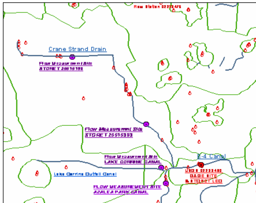
Figure 4.5a STORET sample sites and Flow Measurement Sites on 2/24/05 (Flow meter and USGS gage)
