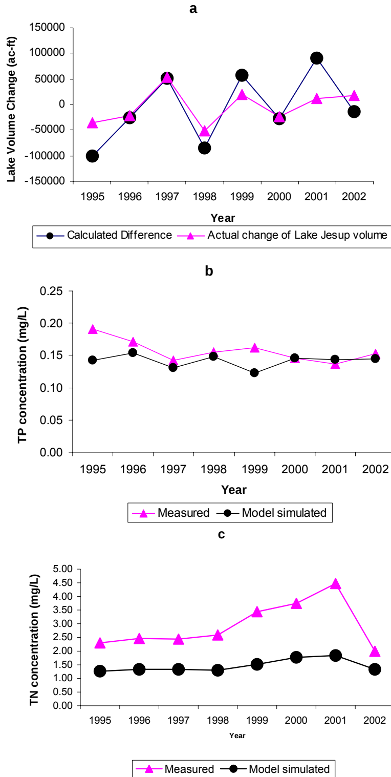
Figures 5.4-a, 5.4-b, 5.4-c. Results for flow and TN and TP calibrations, using the Bathtub model, 1995–2002
