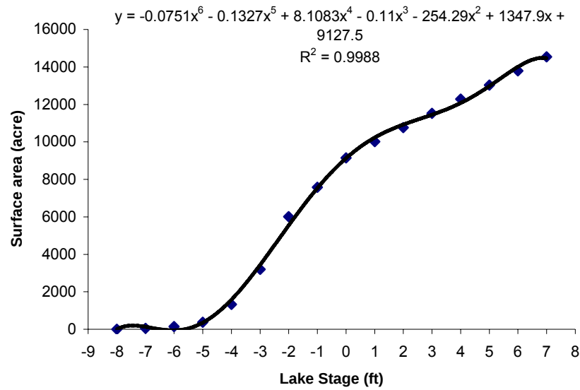
Figure 4.8. Characteristic curve between lake stage and lake surface area for Lake Jesup
