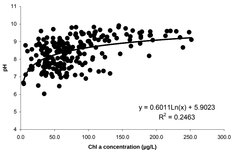
Figure 5.9. Relationship between pH and chl a concentration for Lake Jesup
