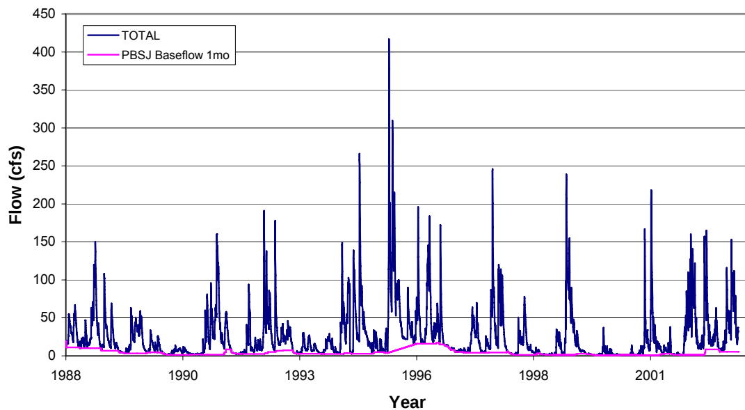
Figure 4.5. Results of the baseflow analysis, 1988–2003
