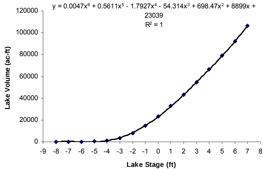
Figure 4.9. Characteristic curve between lake stage and lake cumulative volume for Lake Jesup
