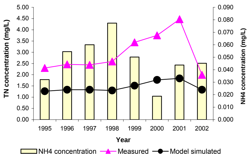
Figure 5.6. Dynamics of ammonia concentration in Lake Jesup, 1995–2002
