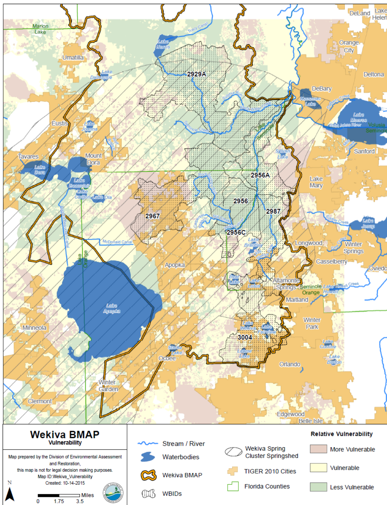
Figure 2.2. Floridan Aquifer Vulnerability Map for the WSA
