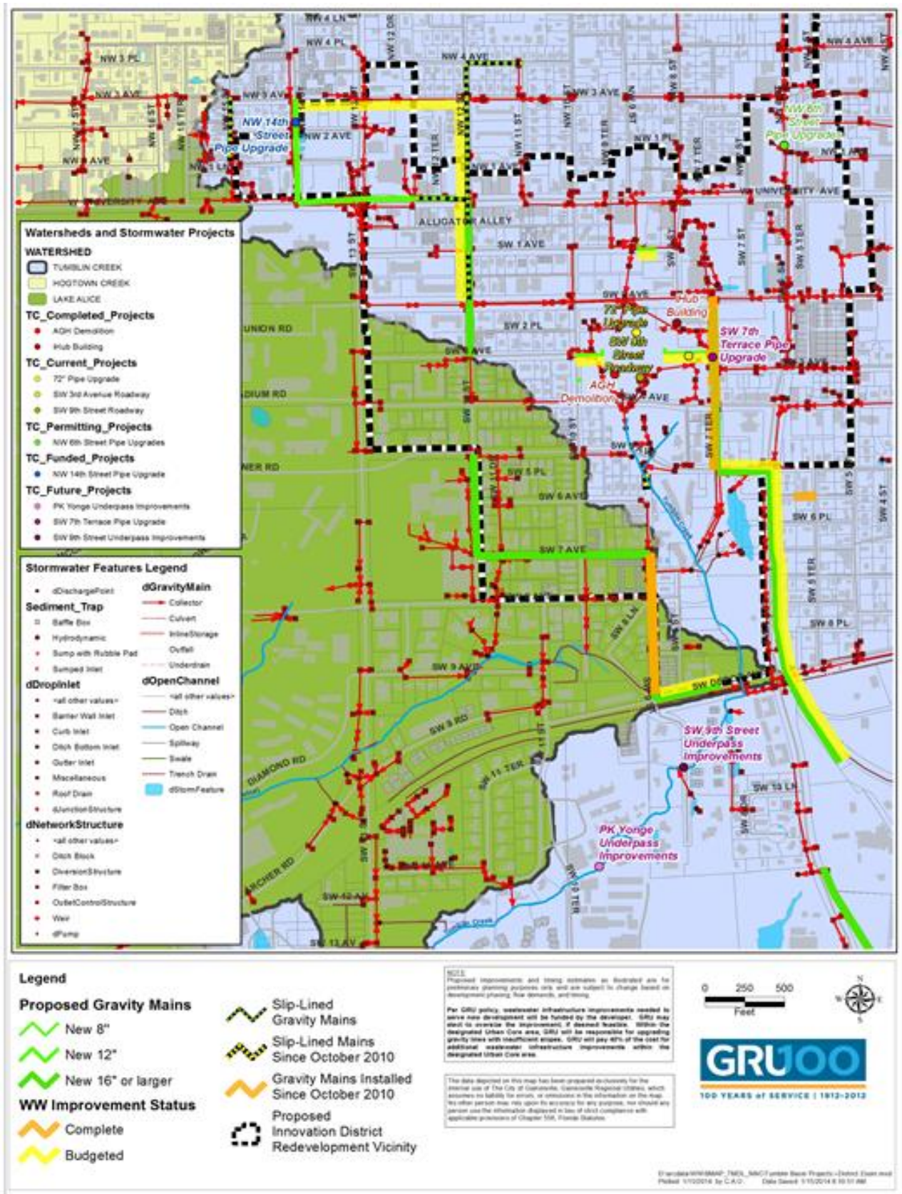
FIGURE 6: SEWER AND STORMWATER SYSTEM UPGRADES FOR THE INNOVATION SQUARE DISTRICT
