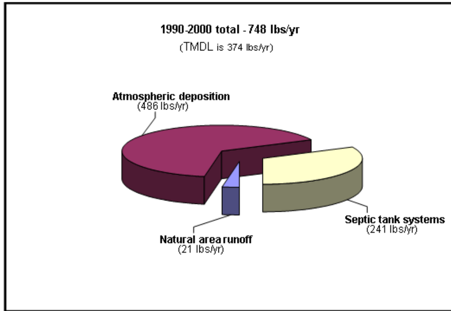
FIGURE 16: BASELINE TP LOADING TO LAKE WAUBERG
