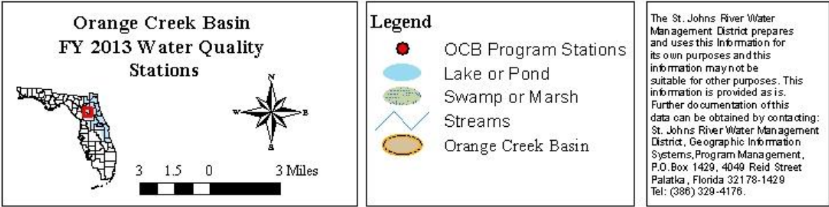
FIGURE 25: SJRWMD WATER QUALITY SAMPLING STATIONS, 2013
