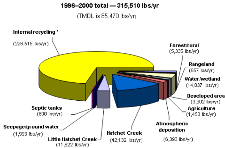
FIGURE 20: BASELINE TN LOADING TO NEWNANS LAKE
