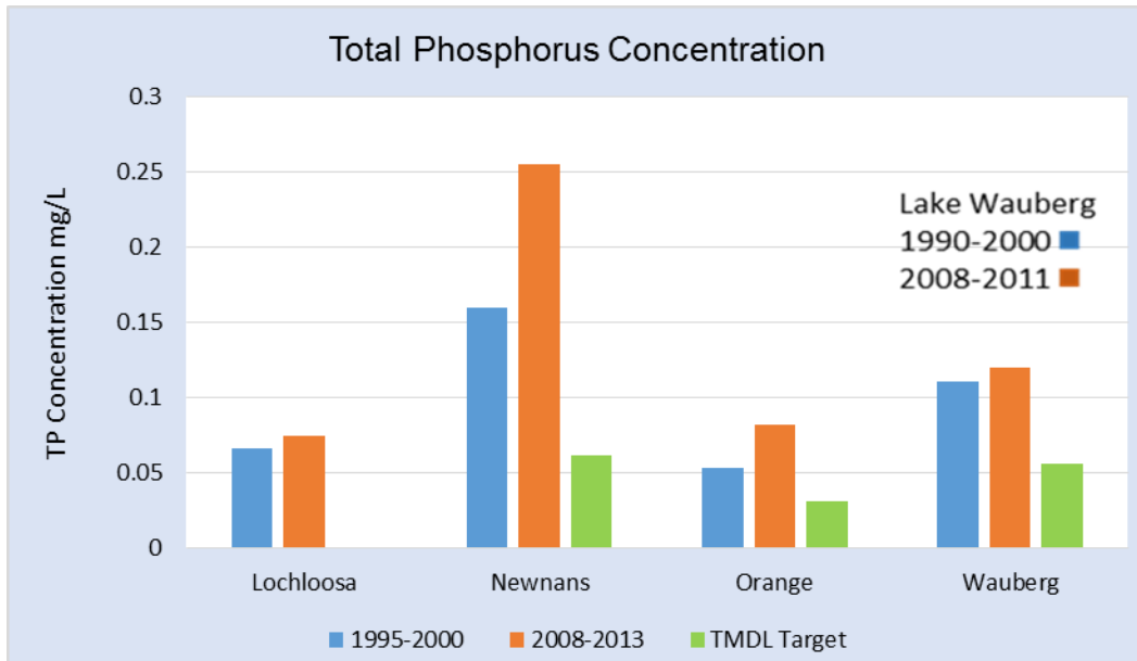
FIGURE 12: AVERAGE ANNUAL TOTAL PHOSPHORUS CONCENTRATION COMPARISONS
