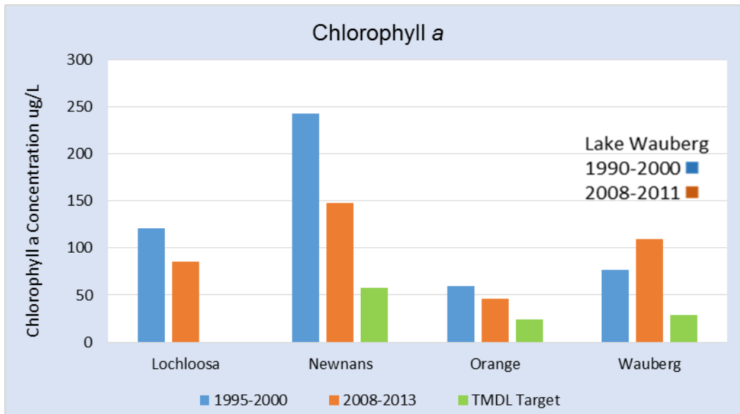
FIGURE 14: AVERAGE ANNUAL CHLOROPHYLL- a CONCENTRATION COMPARISONS
