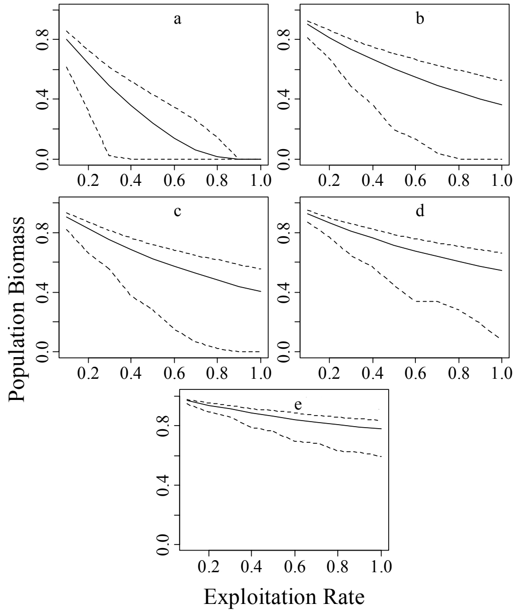
Figure 2-3. Total population biomass as a function of exploitation rate and gill net mesh size for an annual harvest interval. Panels are arranged as follows: panel a, 51-mm mesh; panel b, 64-mm mesh; panel c, 76-mm mesh; panel d, 89-mm mesh; panel e, 102-mm mesh. Dashed lines represent the 95% confidence intervals obtained via parametric bootstrap of the maximum lifetime reproductive rate.
