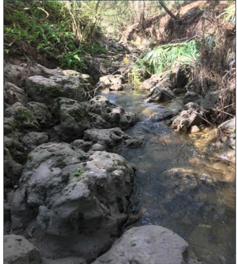
Example of stream bed incision into the Hawthorn formation
