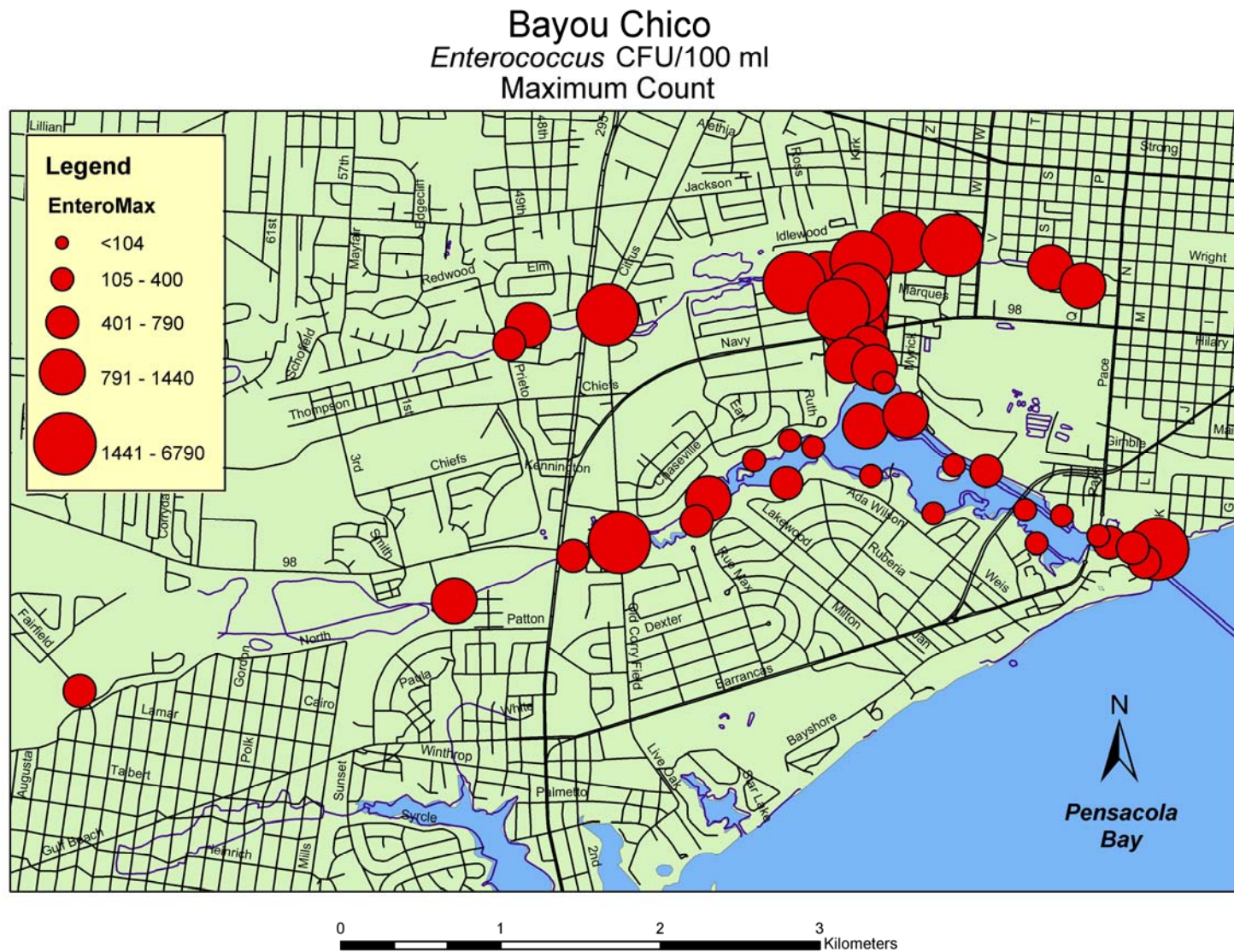
Figure 21. Bayou Chico station data for Enterococcus maximum counts.
