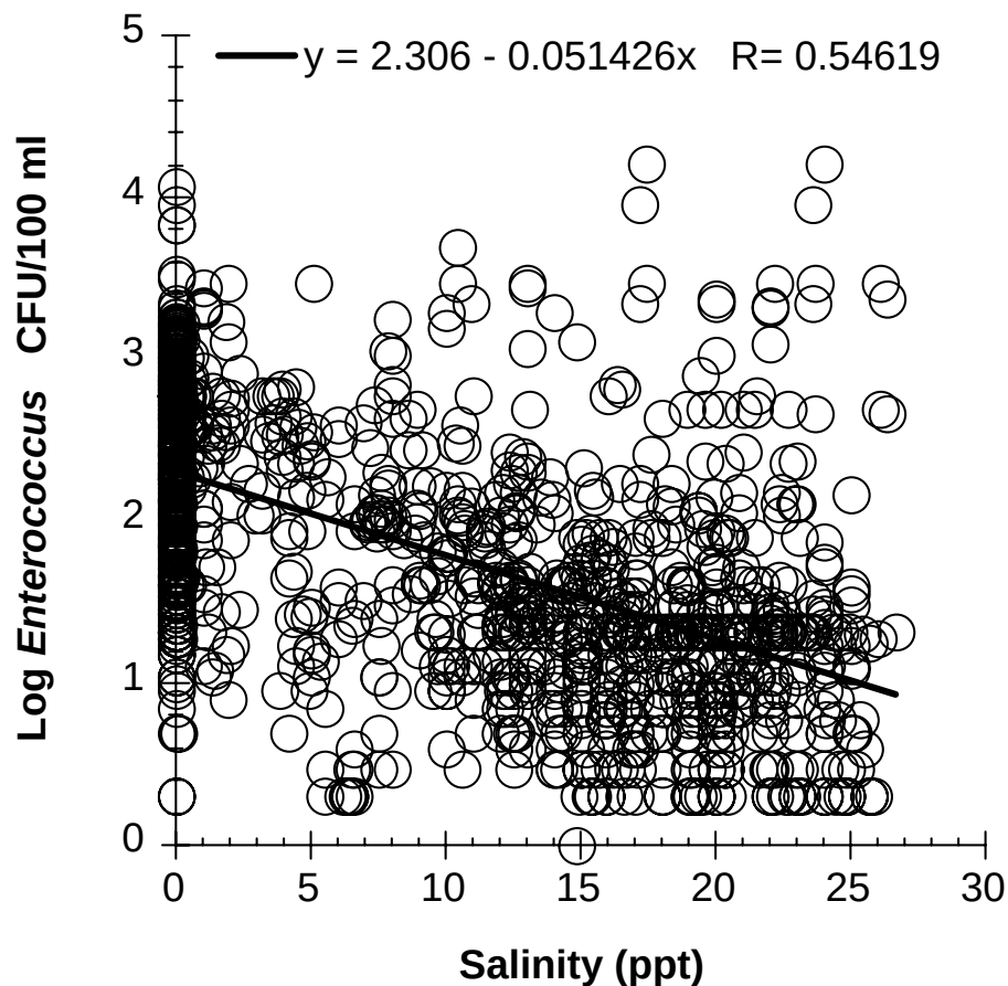
Figure 30. Conservative mixing diagrams for Enterococcus in Bayou Texar, including only stations south from the 12 Avenue Bridge.
