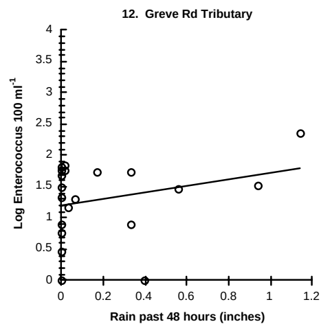
Figure 11. Station-specific analysis of rainfall dependence in Bayou Grande, continued.
