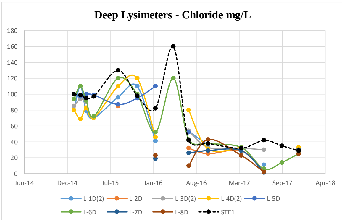
Figure 6. Deep Lysimeters – Chloride mg/L
