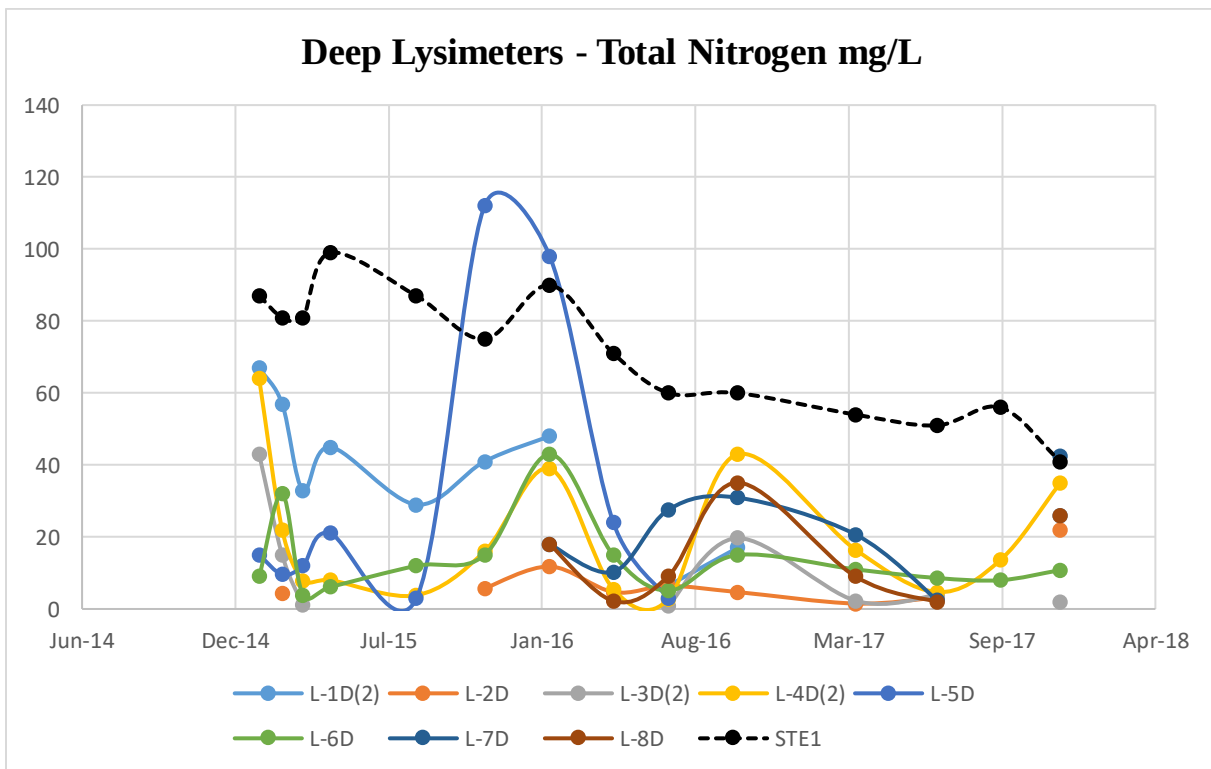
Figure 12. Deep Lysimeters – Total Nitrogen mg/L 2015-2017
