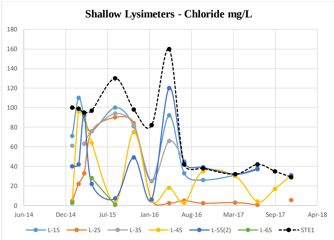
Figure 3. Shallow Lysimeters – Chloride mg/L
