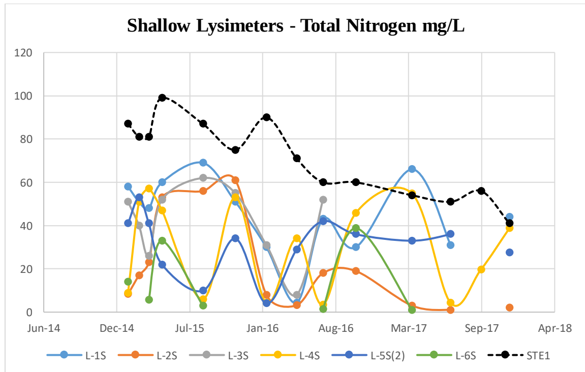
Figure 4. Shallow Lysimeters – Total Nitrogen mg/L
