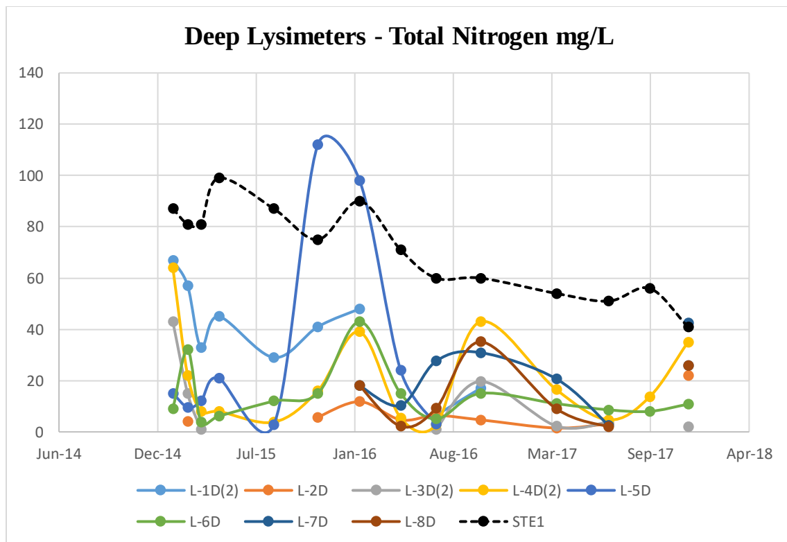
Figure 7. Deep Lysimeters – Total Nitrogen mg/L 2015-2017
