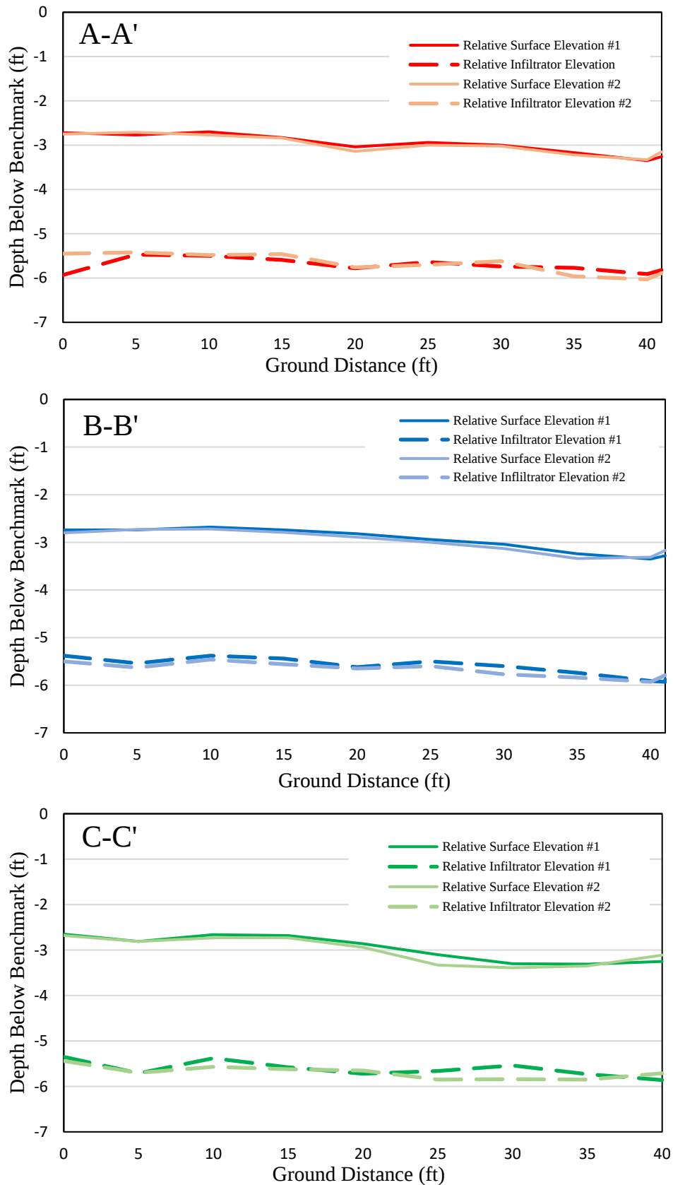
Figure 14. Cross Sections of Relative Surface Elevations & Infiltrators December 2017
