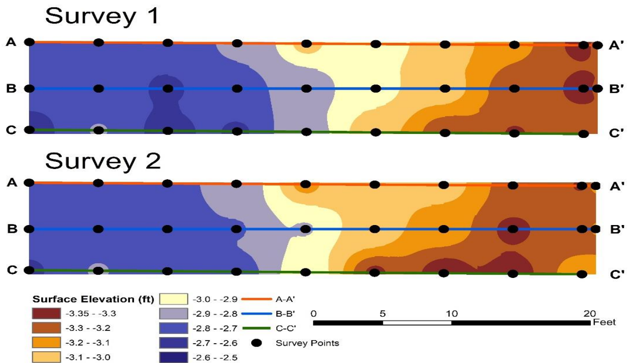
Figure 13. Land Surface Elevation (LSE) Survey of Drainfield December 2017
