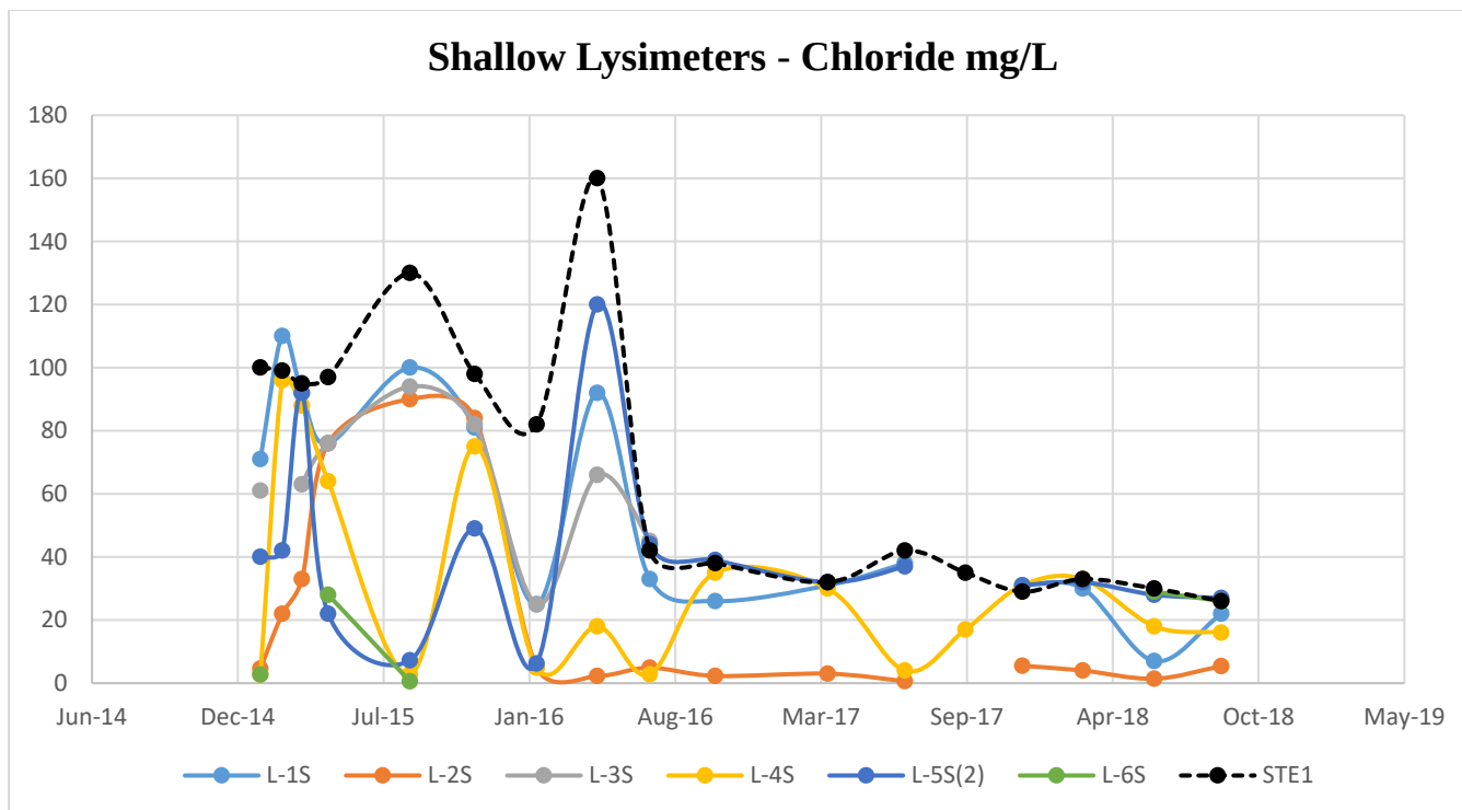
Figure 3. Shallow Lysimeters – Chloride mg/L
