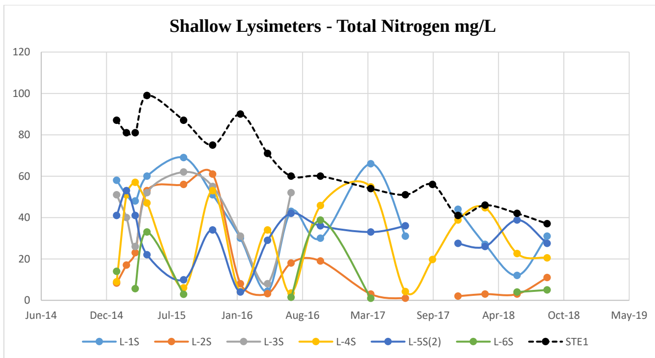
Figure 4. Shallow Lysimeters – Total Nitrogen mg/L
