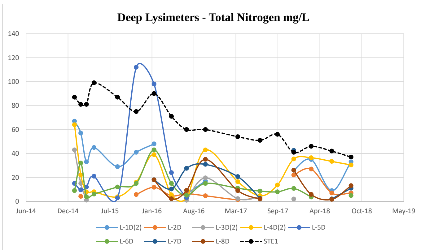
Figure 12. Deep Lysimeters – Total Nitrogen mg/L 2016-2018
