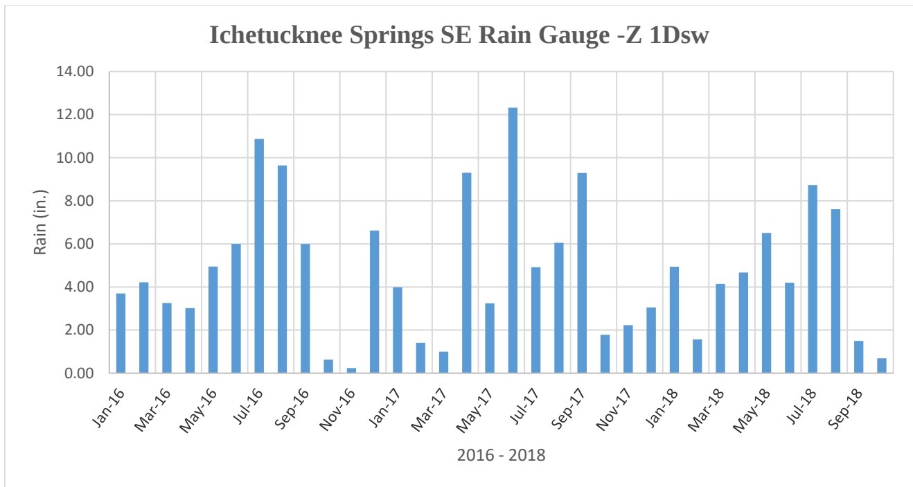
Figure 2. Monthly Rainfall Data 2016 - 2018 Park Manager's Residence
