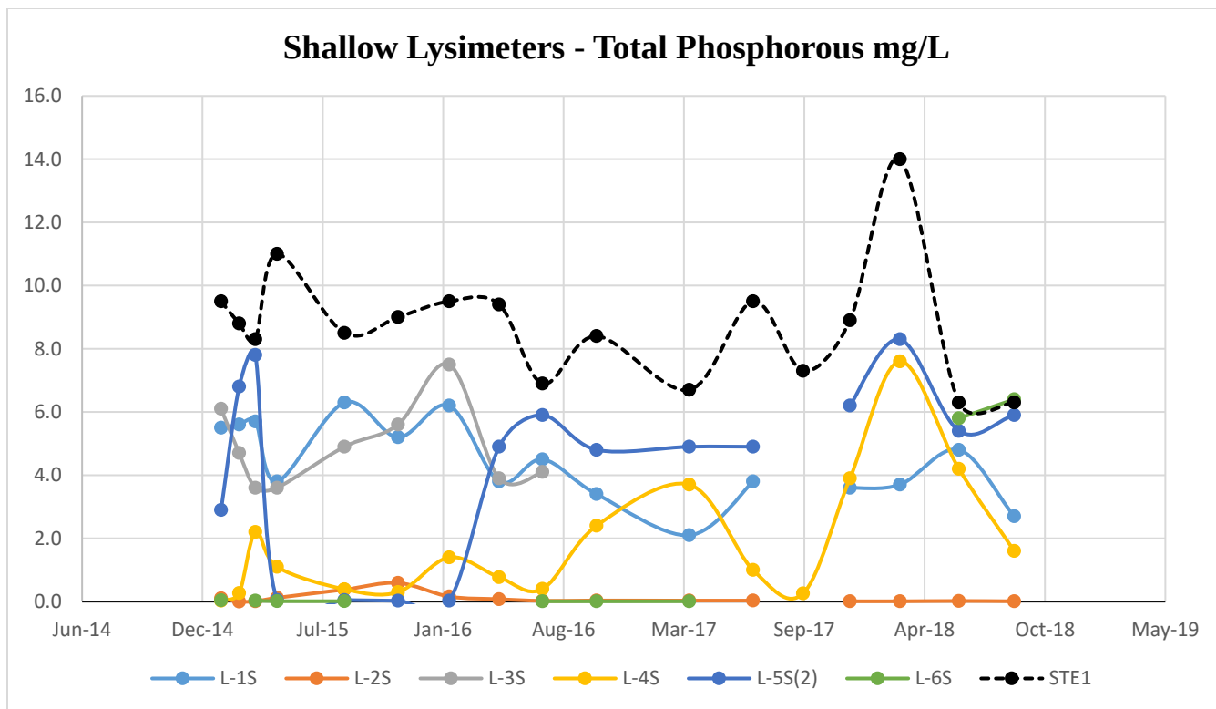
Figure 5. Shallow Lysimeters – Total Phosphorous mg/L
