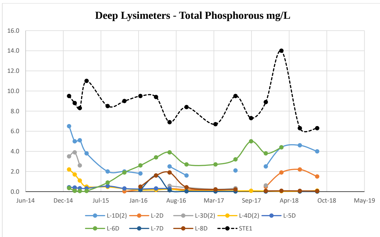
Figure 8. Deep Lysimeters – Total Phosphorous mg/L 2015-2018
