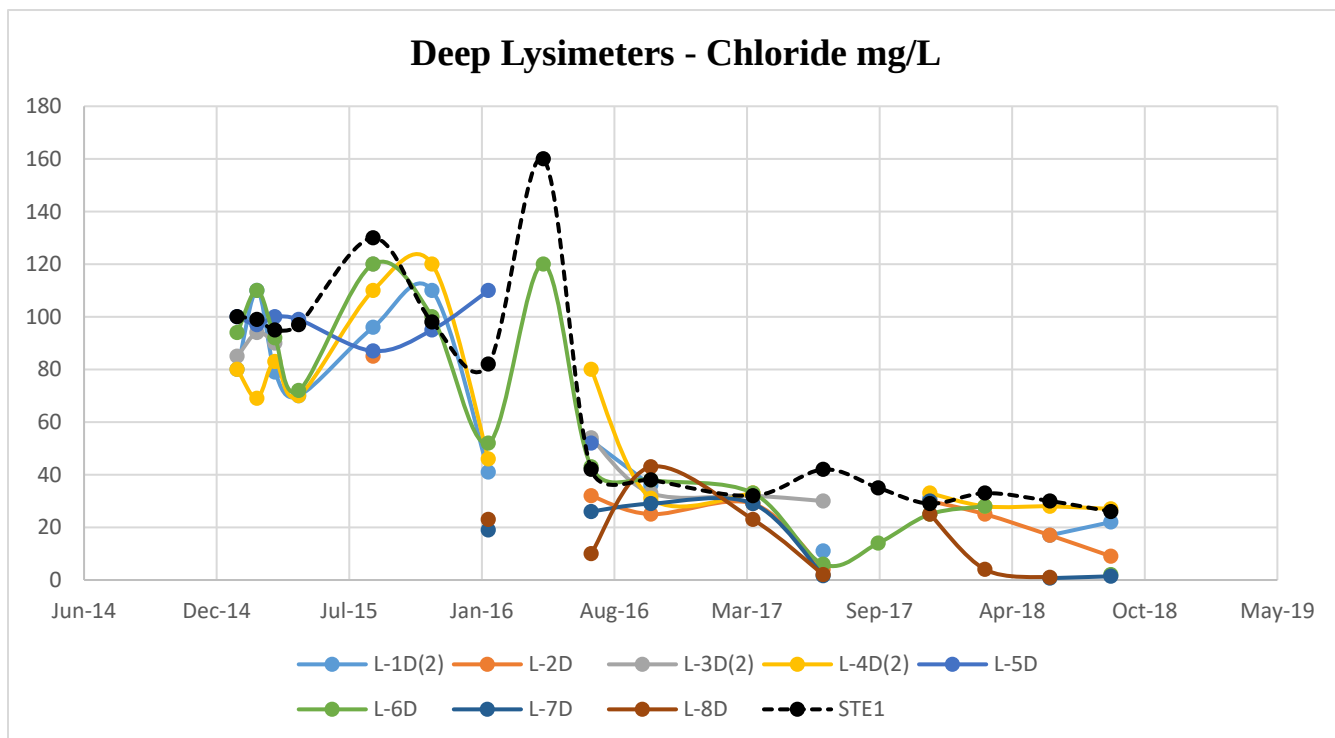
Figure 6. Deep Lysimeters – Chloride mg/L
