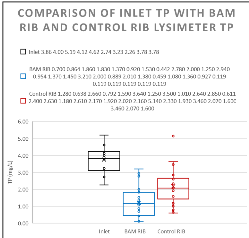
Figure 17 Comparison of Inlet and Lysimeter Total Phosphorus Using Reclaimed Water
