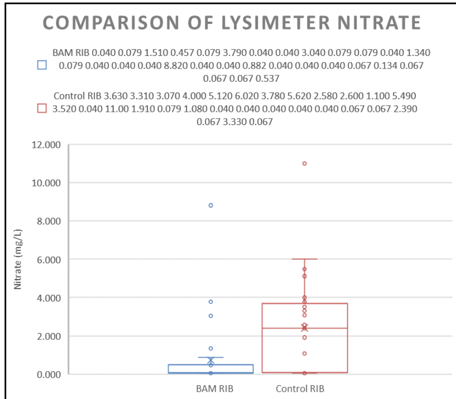
Figure 13 Comparison of Nitrate under the BAM and Control RIBs Using Reclaimed Water
