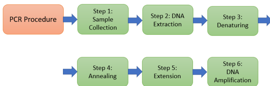
Figure 21 PCR Procedure
