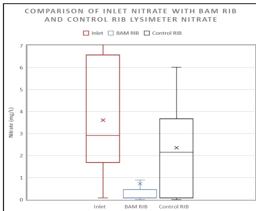
Figure 14 Comparison of Inlet and Lysimeter Nitrate Concentrations Using Reclaimed Water
