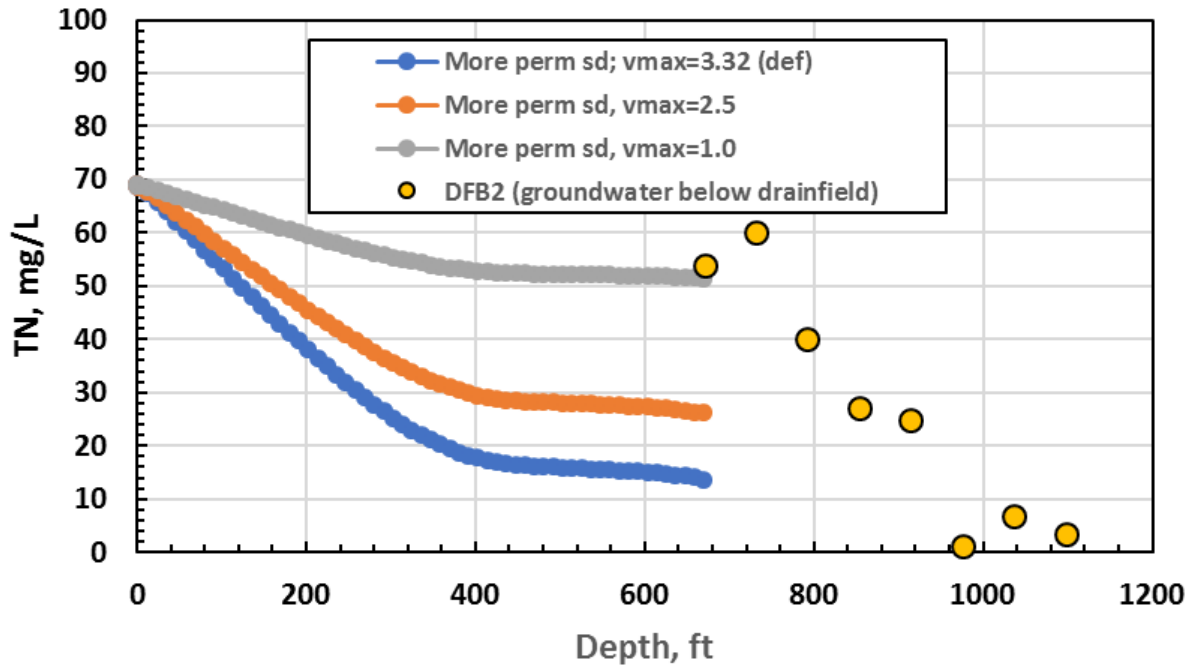
Figure 41. STUMOD-FL simulations of TN concentrations in groundwater at several depths beneath a septic tank drainfield at a selected site in Orange County (Aley et al. 2007)
