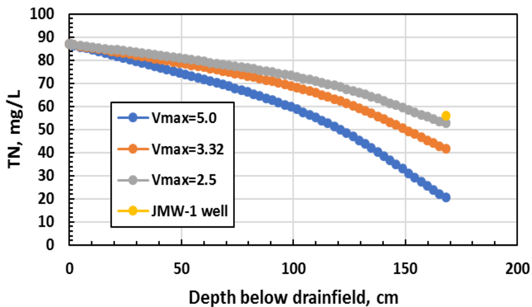
Figure 39. STUMOD-FL simulations of TN attenuation with calibration from shallow monitoring well at Site J
