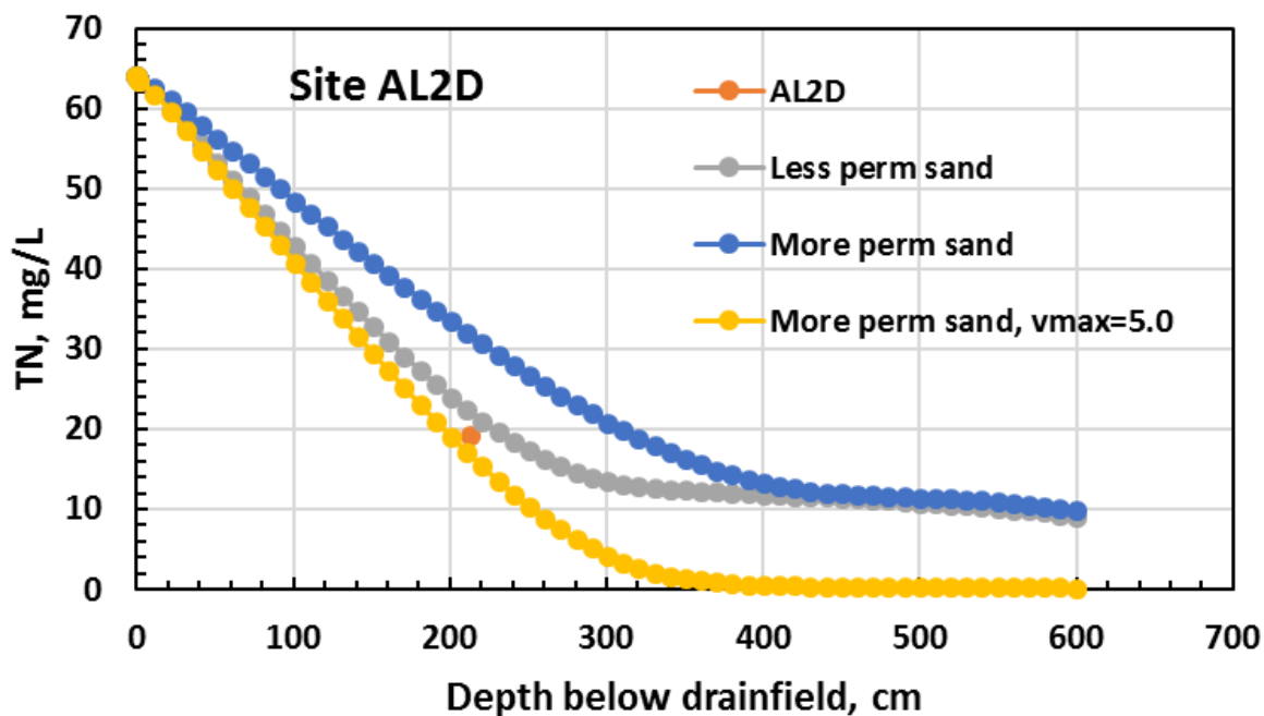
Figure 36. STUMOD-FL simulations of TN attenuation with calibration from deeper lysimeter at Site A
