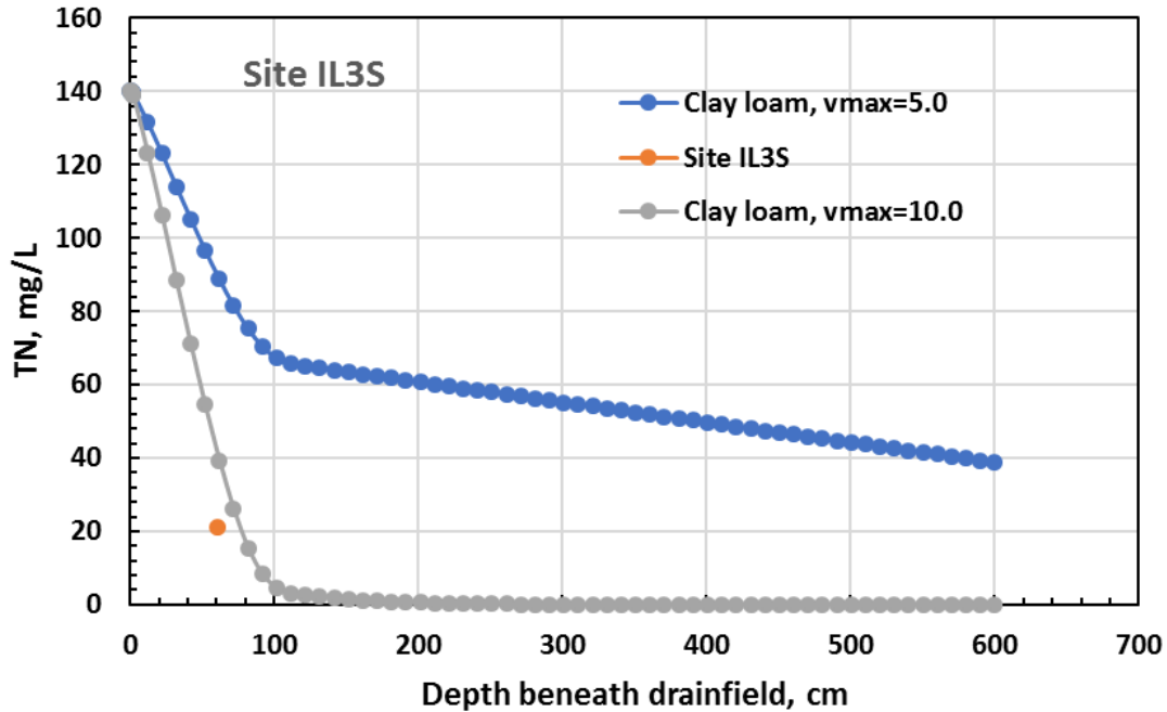
Figure 40. STUMOD-FL simulations of TN attenuation with calibration from shallow lysimeter at Site I
