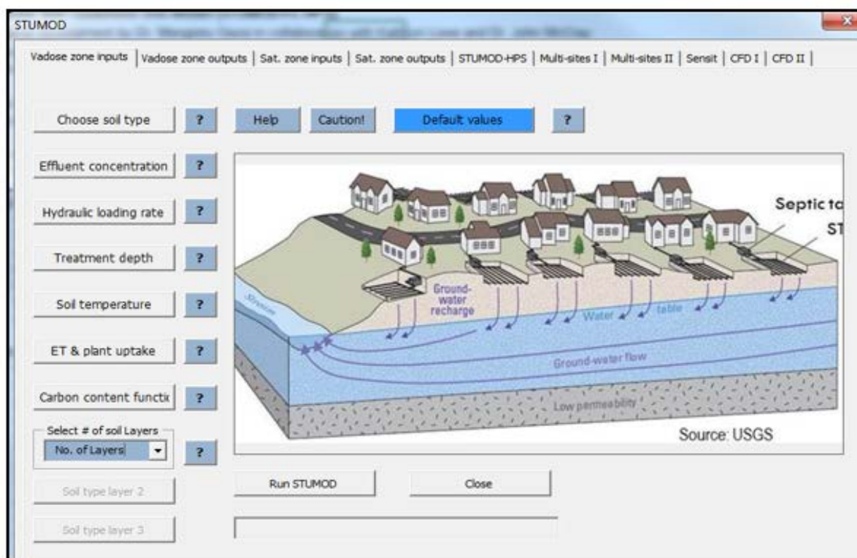
Figure C-1d. User interface showing parameters used in STUMOD to estimate nitrogen fate and transport from OSTDS
