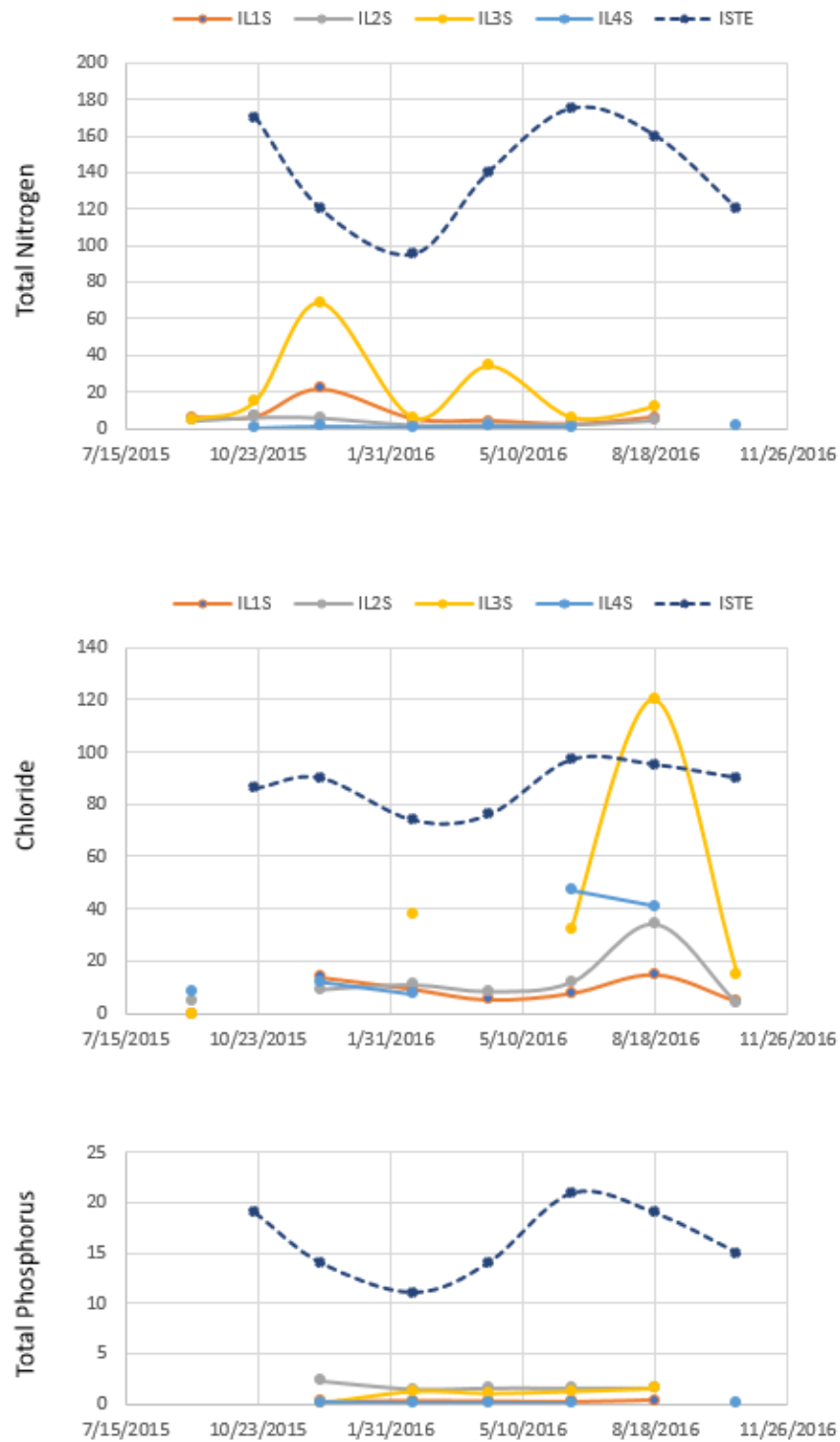
Figure 29. Lysimeter and STE monitoring results for TN, chloride, and TP at Site I (in mg/L)
