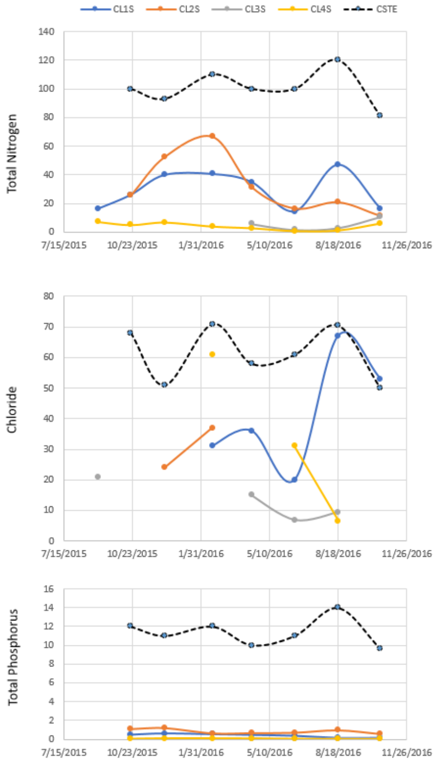
Figure 16. Lysimeter and STE monitoring results for TN, chloride, and TP at Site C (in mg/L)
