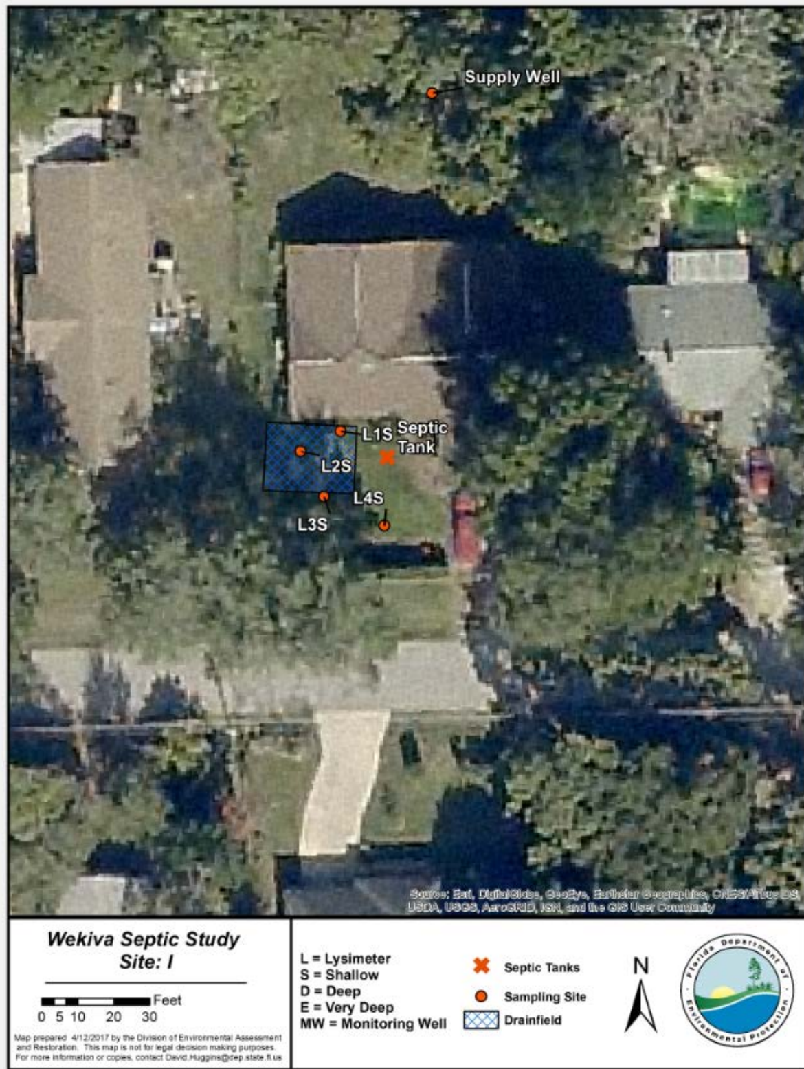
Figure 28. Septic system and monitoring devices at Site I
