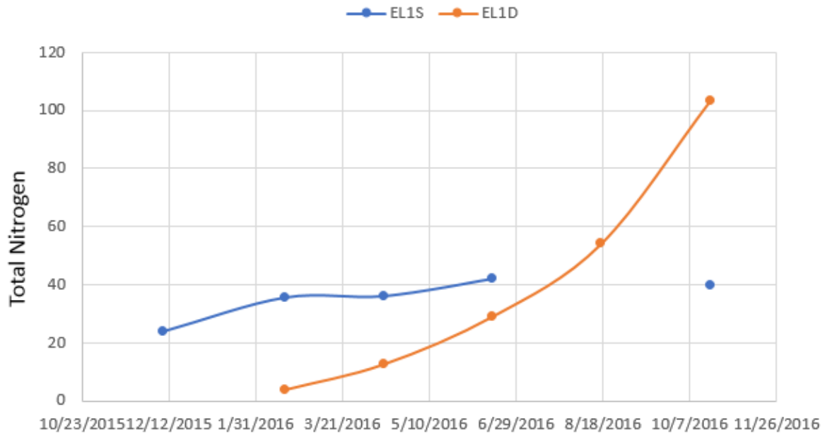
Figure 21. Plot showing TN concentrations (in mg/L) in paired lysimeters EL1S (5-ft depth) and EL1D (10-ft depth)
