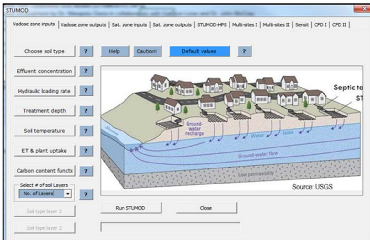
Figure 35. User interface showing parameters used in STUMOD-FL to estimate nitrogen fate and transport from OSTDS
