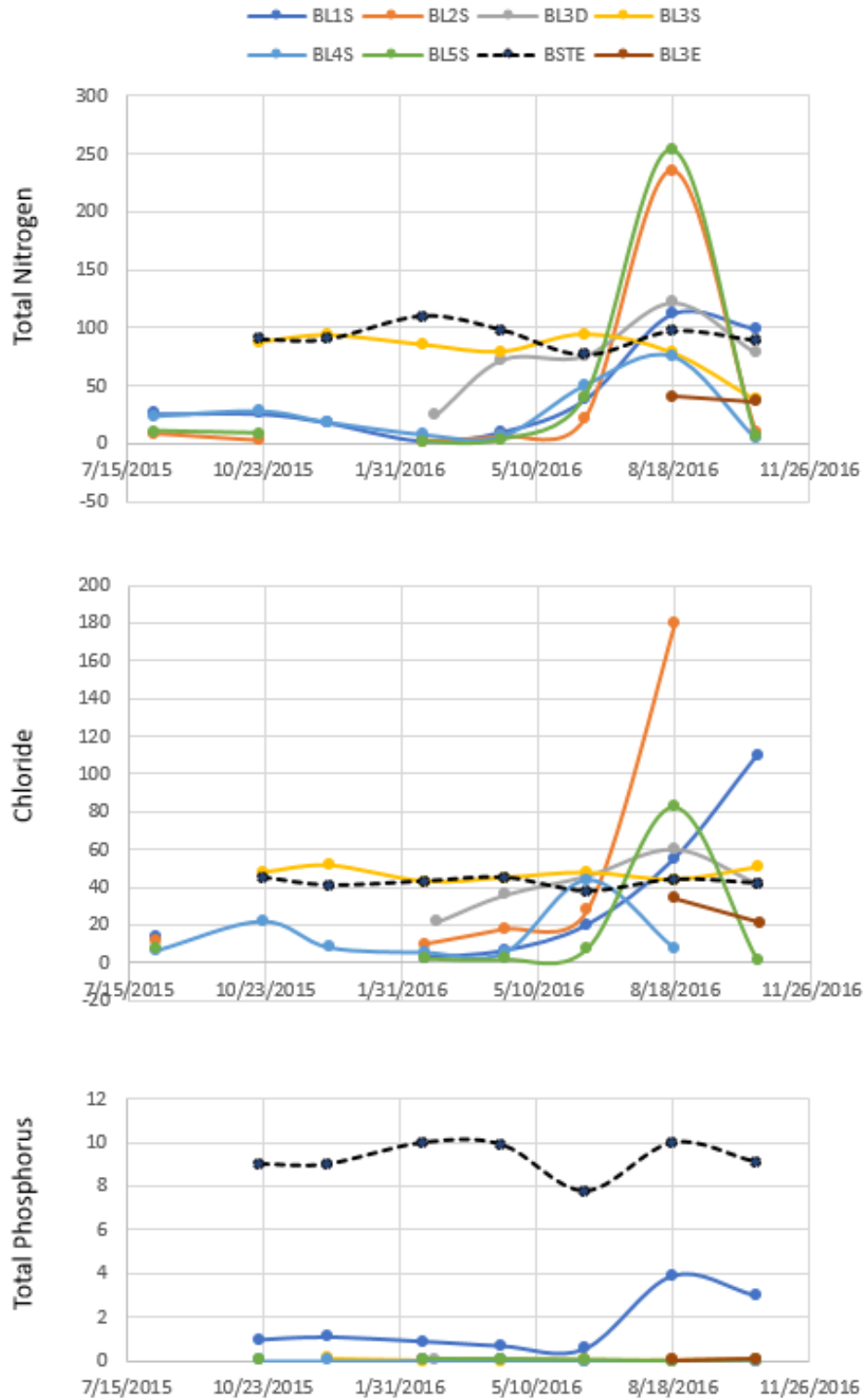
Figure 13. Lysimeter and STE monitoring results for TN, chloride, and TP at Site B (in mg/L)
