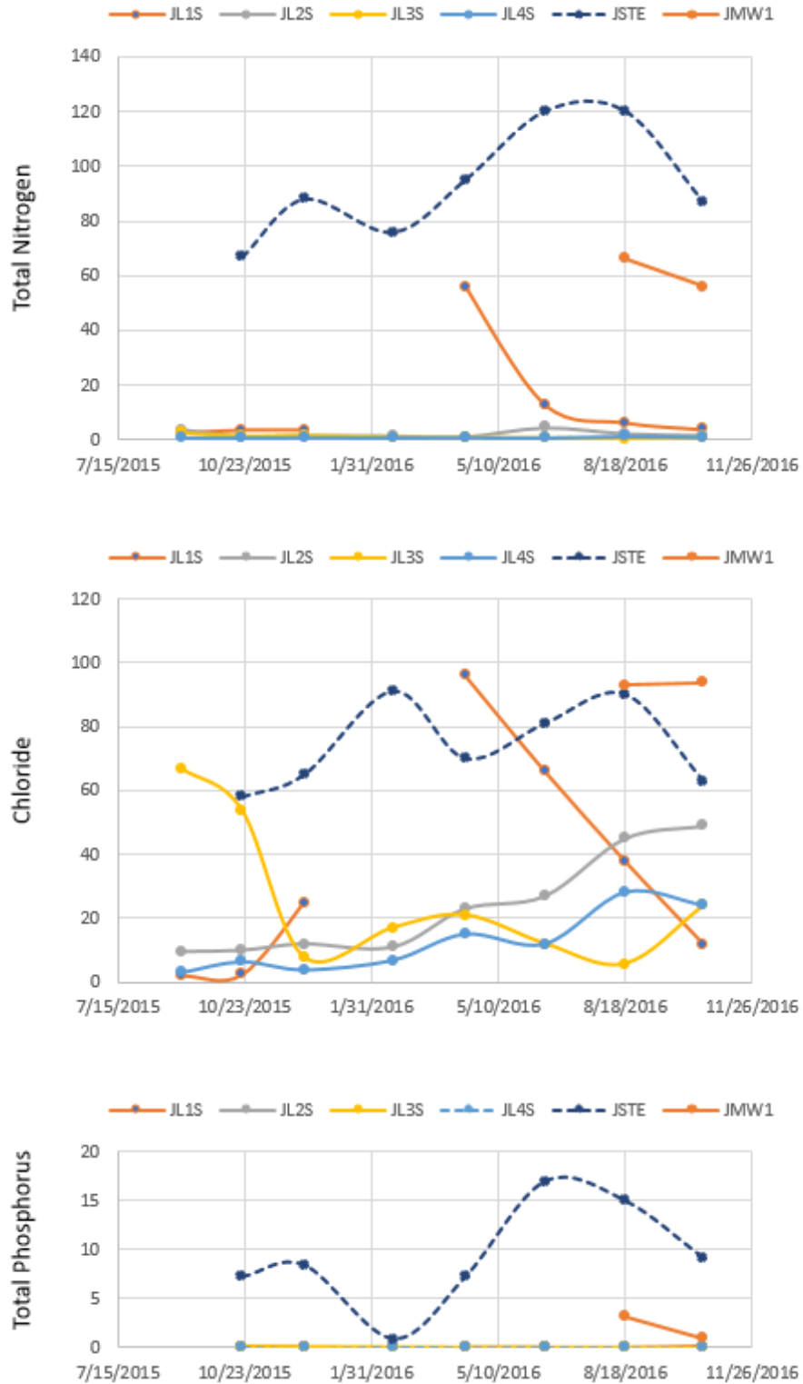
Figure 31. Lysimeter, monitoring well and STE monitoring results for TN, chloride, and TP at Site J (in mg/L)
