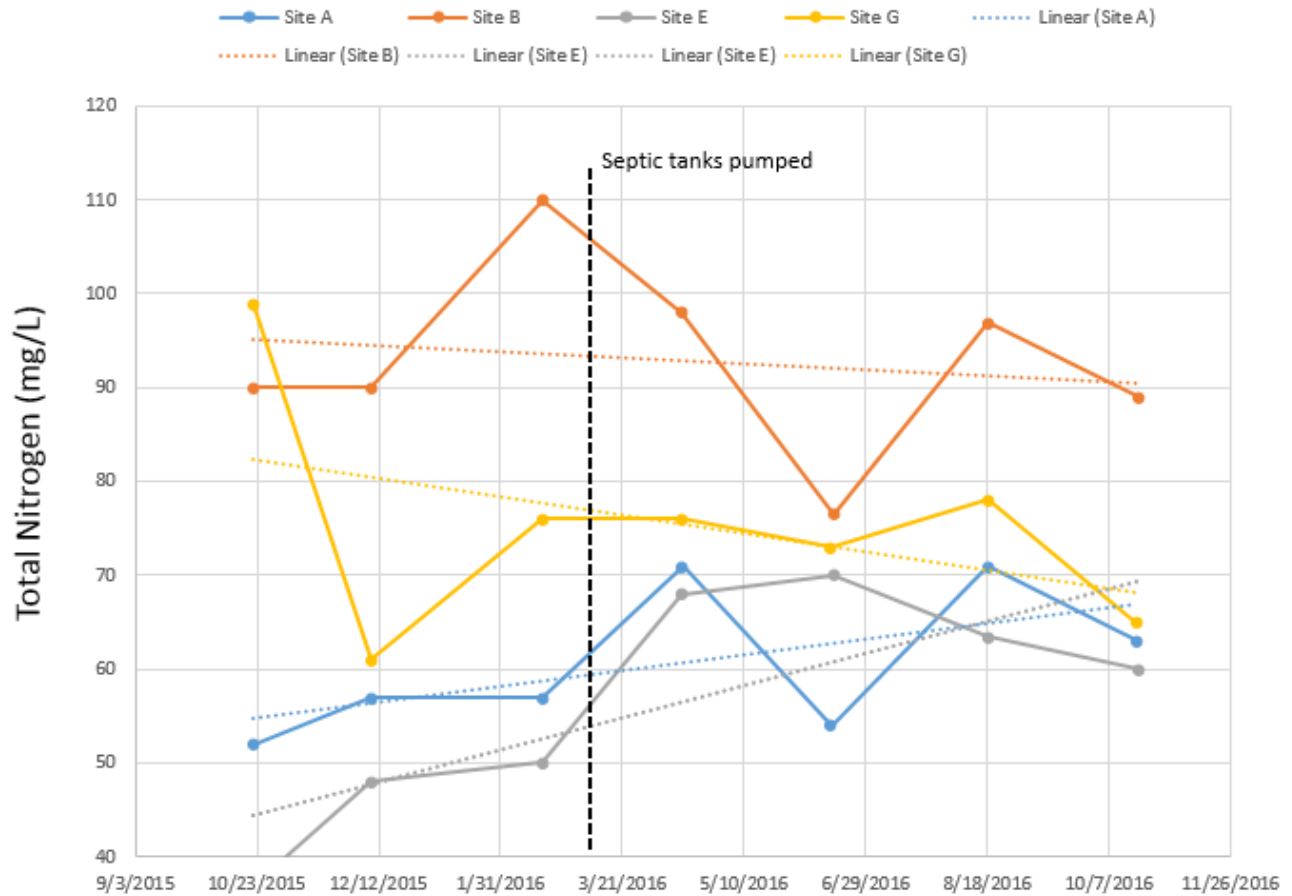
Figure 8. TN concentration trends in septic tanks before and after pump-out (in mg/L)
