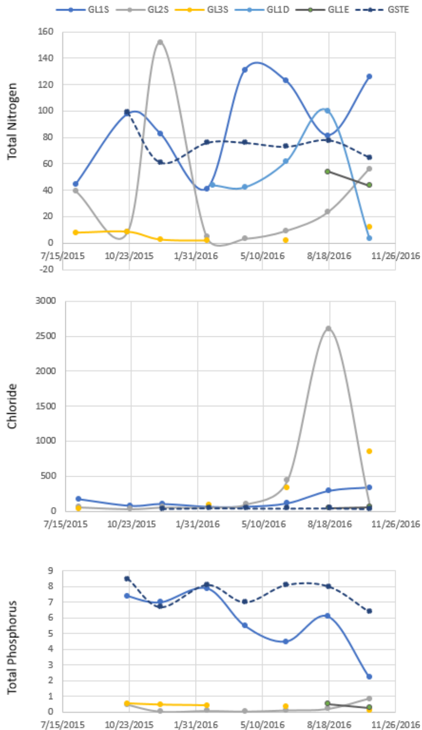
Figure 26. Lysimeter and STE monitoring results for TN, chloride, and TP at Site G (in mg/L)
