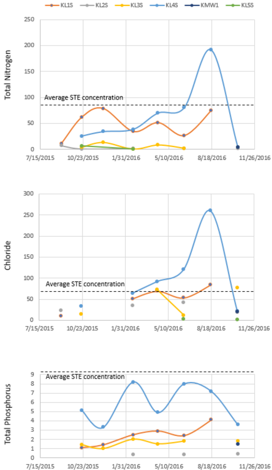
Figure 33. Lysimeter, monitoring well, and STE monitoring results for TN, chloride, and TP at Site K (in mg/L)
