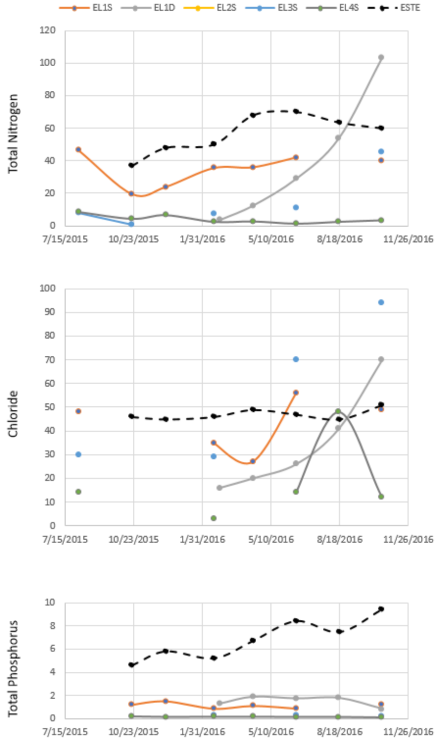
Figure 20. Lysimeter and STE monitoring results for TN, chloride, and TP at Site E (in mg/L)
