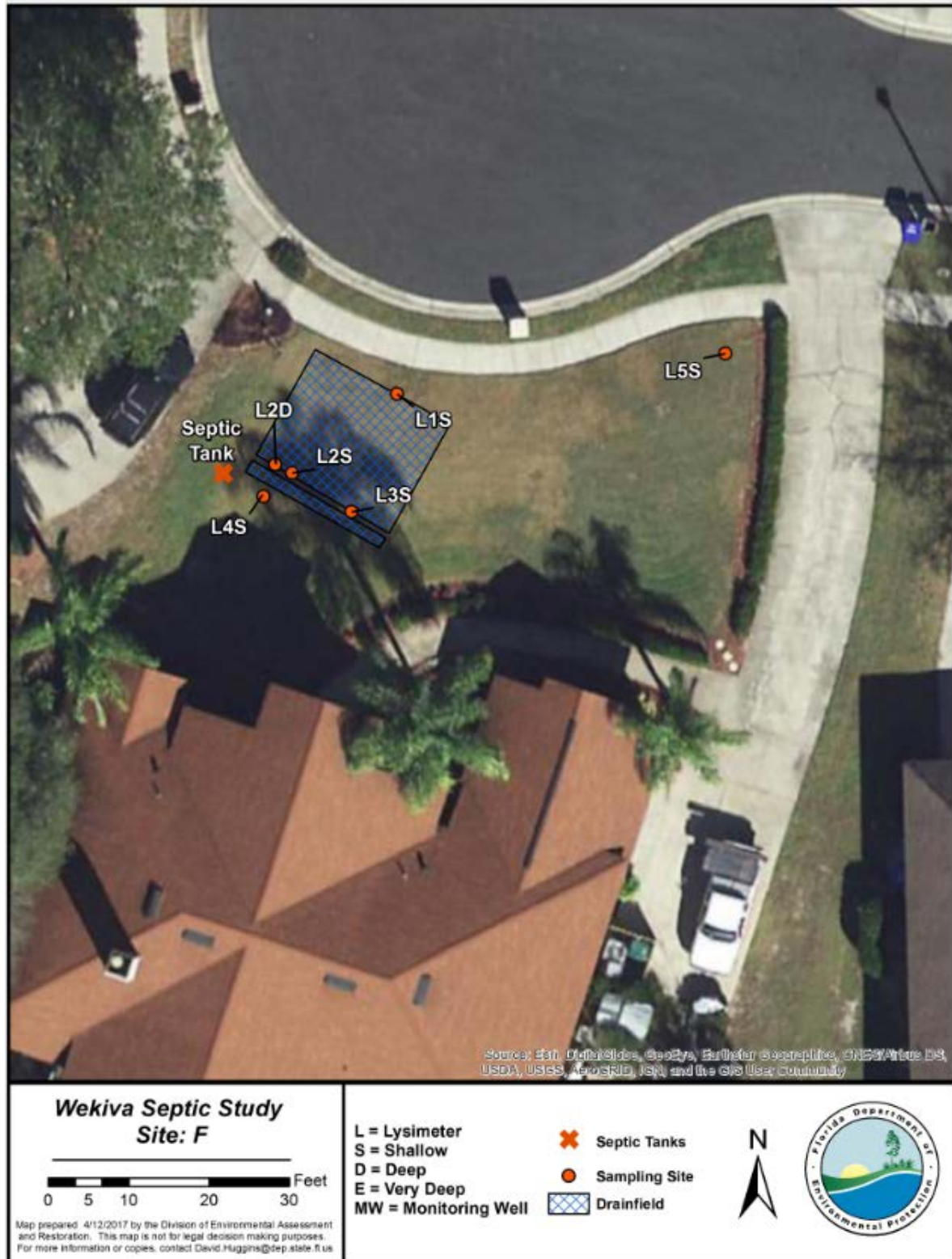
Figure 22. Septic system and monitoring devices at Site F
