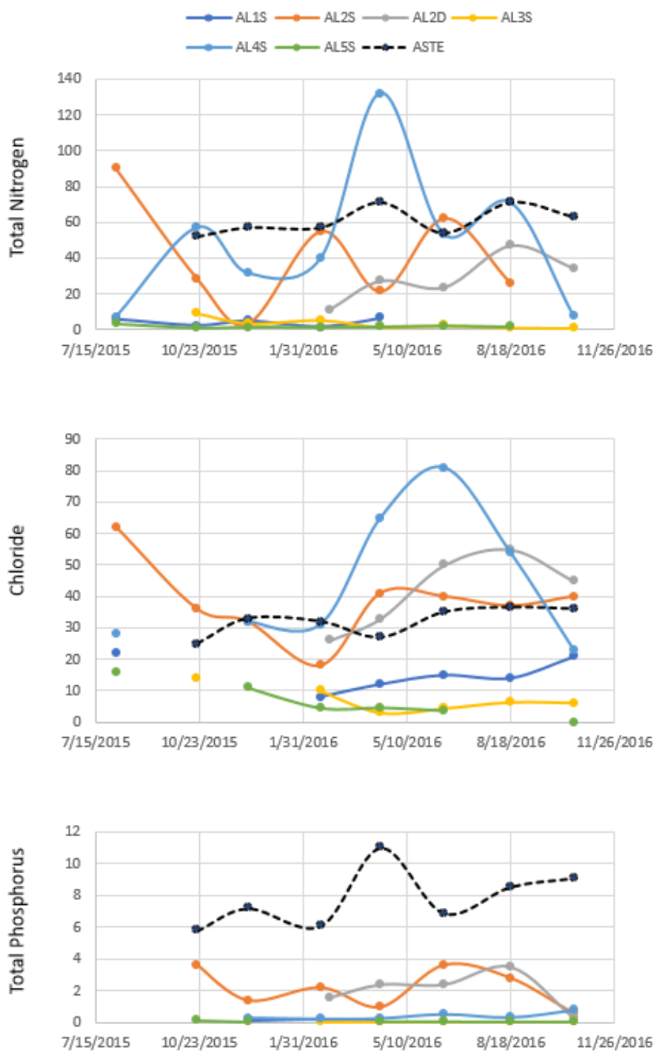
Figure 10. Lysimeter and STE monitoring results for TN, chloride, and TP at Site A (in mg/L)
