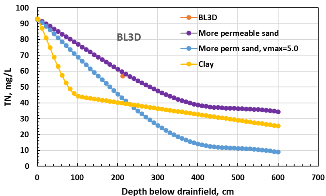
Figure 36. STUMOD-FL simulations of TN attenuation with calibration from deeper lysimeter at Site A
