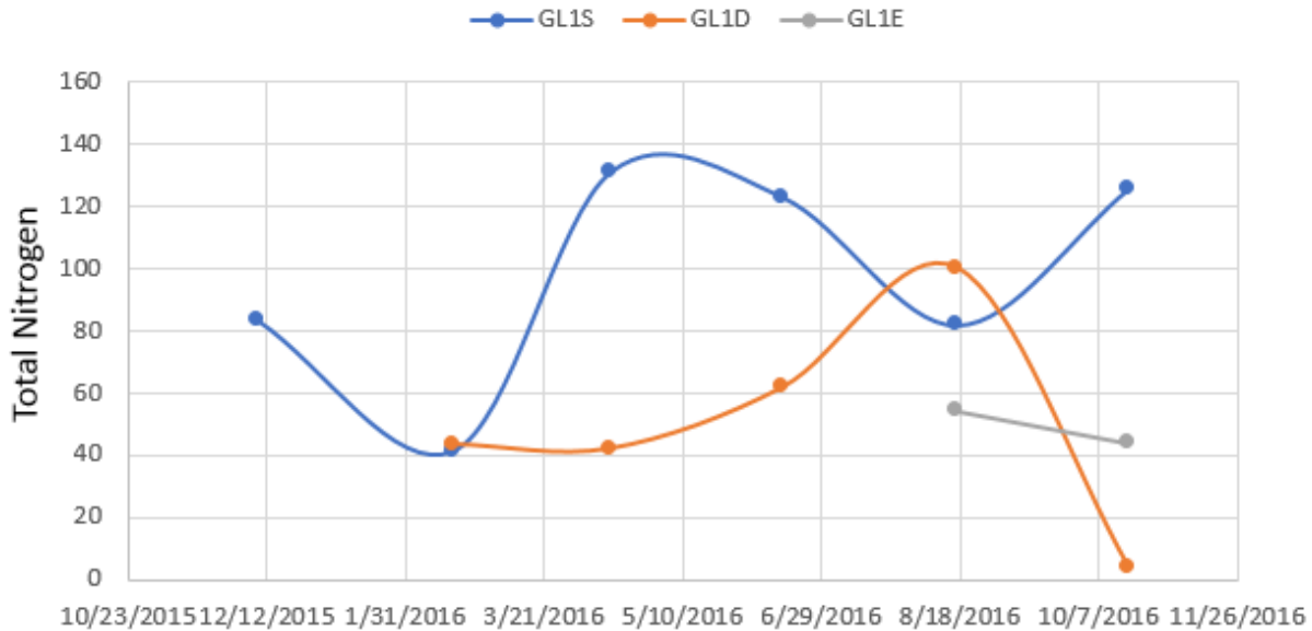
Figure 27. Plot showing TN concentrations (in mg/L) for lysimeters GL1S (5-ft depth), GL1D (10-ft depth), and GL1E (15-ft depth)
