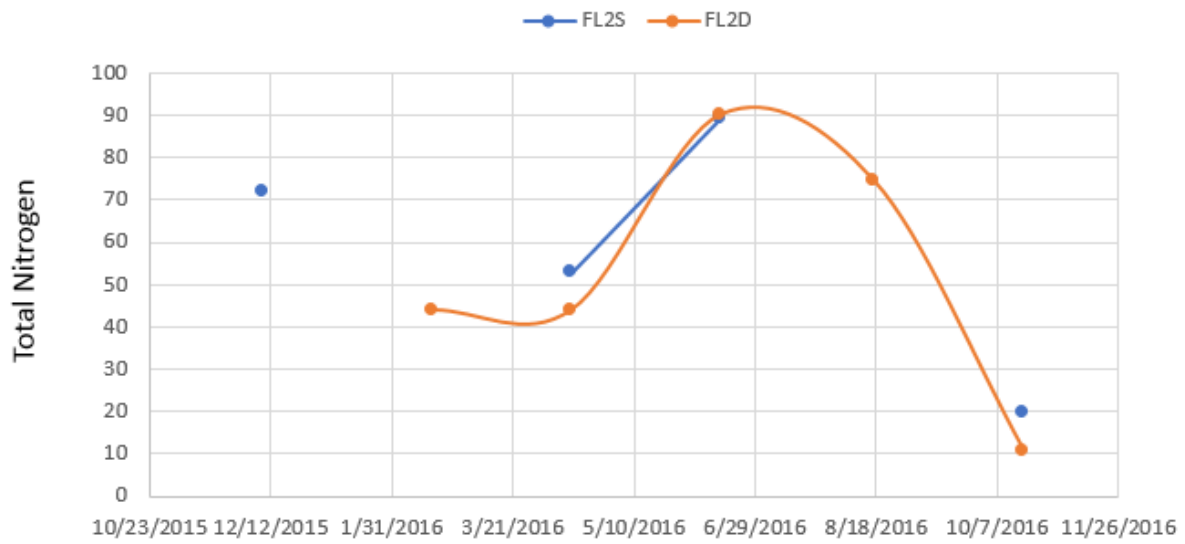
Figure 24. Plot showing TN concentrations (in mg/L) in paired lysimeters FL2S (5-ft depth) and FL2D (10-ft depth).
