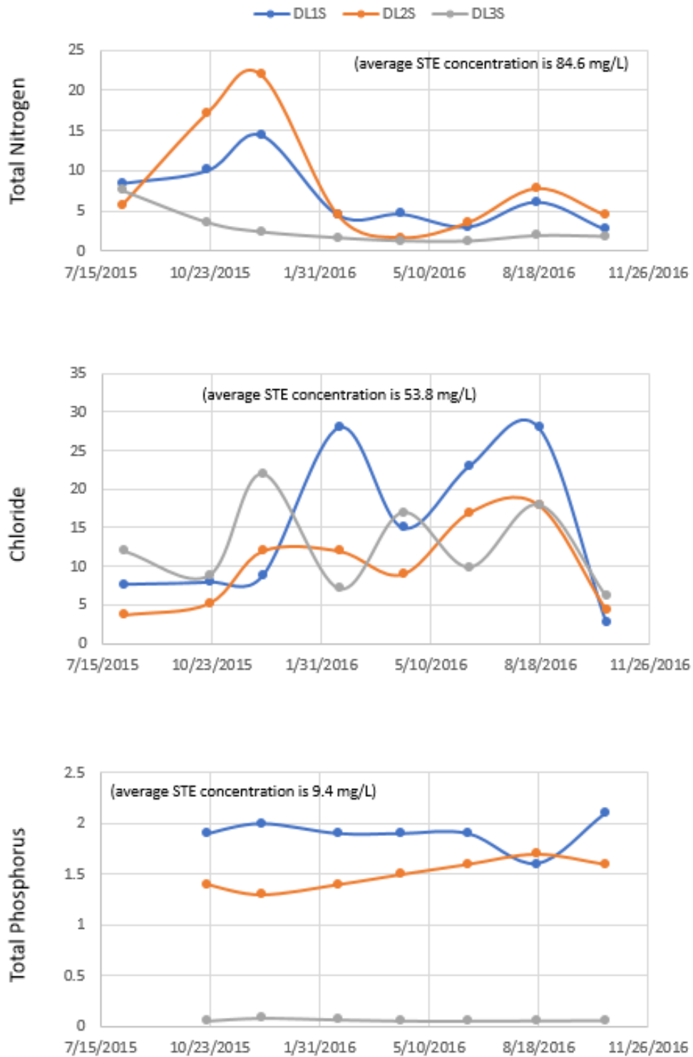
Figure 18. Lysimeter and STE monitoring results for TN, chloride, and TP at Site D (in mg/L)
