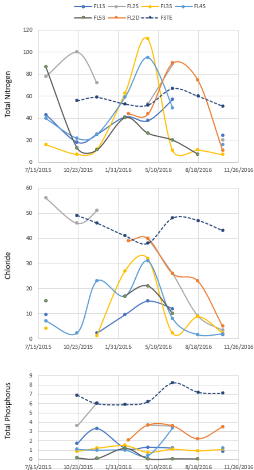
Figure 23. Lysimeter and STE monitoring results for TN, chloride, and TP at Site F (in mg/L)
