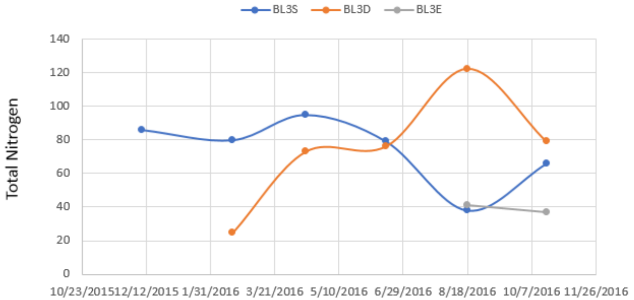
Figure 14. Plot showing TN concentrations (in mg/L) in paired lysimeters BL3S (5-ft depth), BL3D (10-ft depth), and BL3E (15-ft depth)
