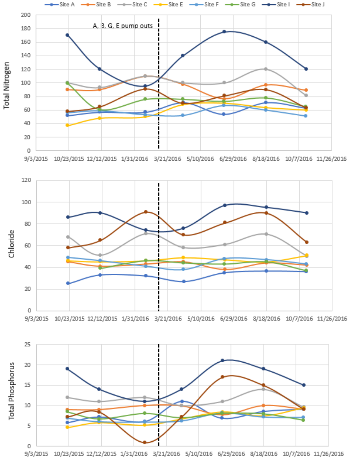
Figure 7. Nitrogen, chloride, and phosphorus concentrations in STE
