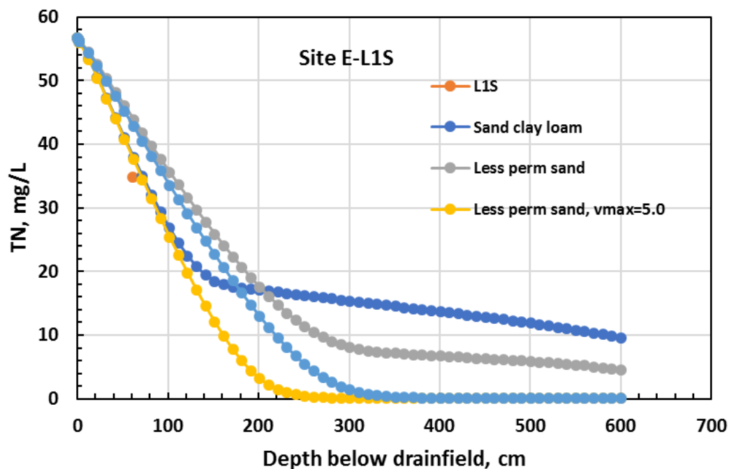
Figure 38. STUMOD-FL simulations of TN attenuation with calibration from shallow lysimeter at Site E
