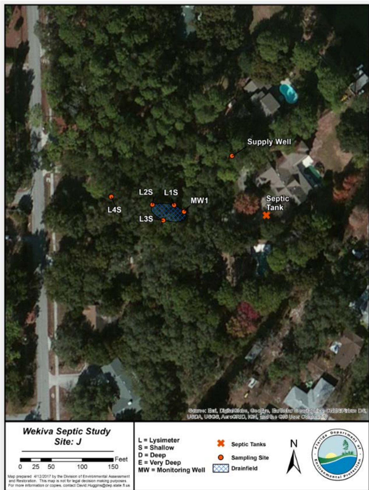
Figure 30. Septic system and monitoring devices at Site J
