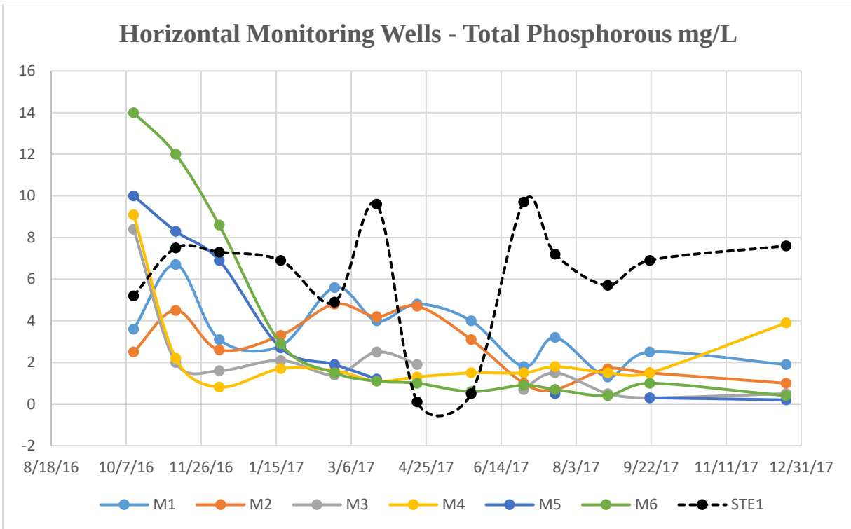
Figure 9. Horizontal Monitoring Wells – Total Phosphorous mg/L
