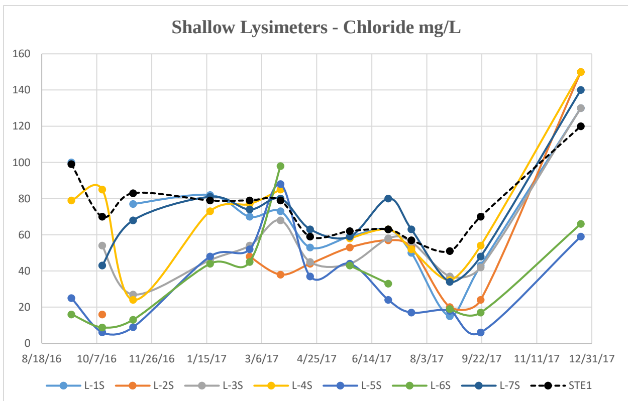
Figure 4. Shallow Lysimeters – Chloride mg/L
