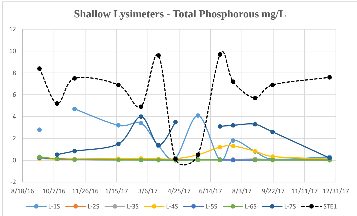
Figure 6. Shallow Lysimeters – Total Phosphorous mg/L
