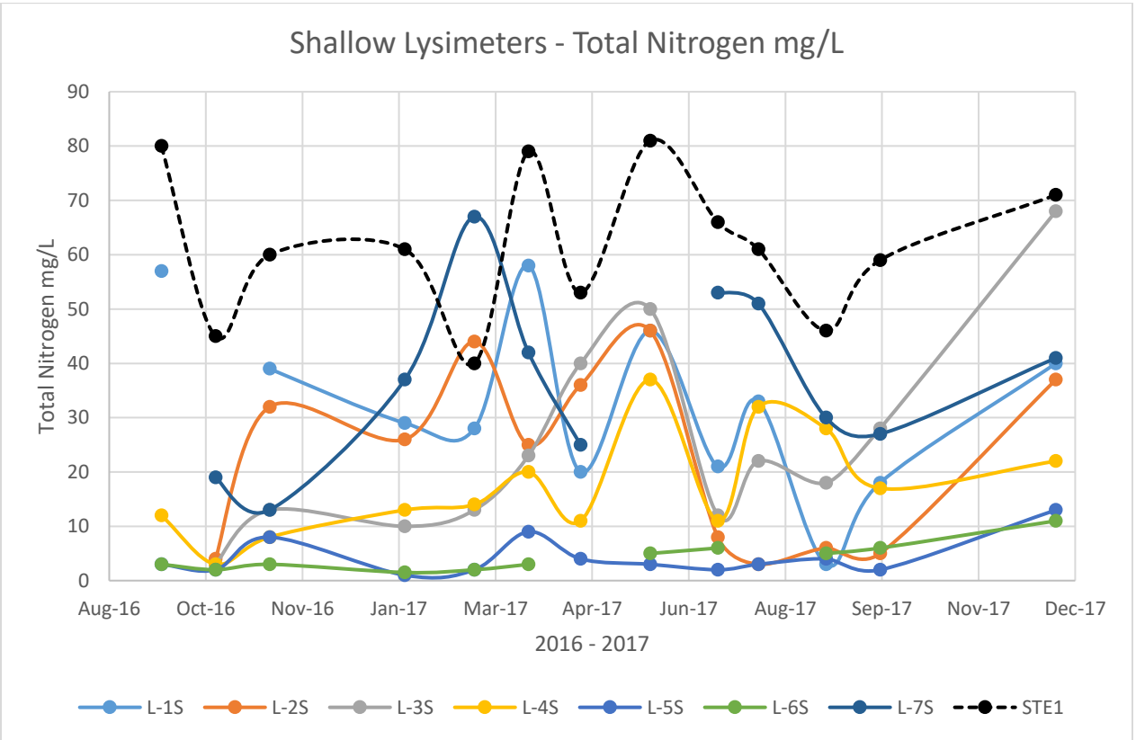
Figure 13. Monthly Rainfall (inches) and Shallow Lysimeters – Total Nitrogen (mg/L)
