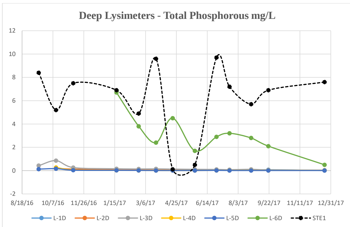
Figure 12. Deep Lysimeters – Total Phosphorous mg/L
