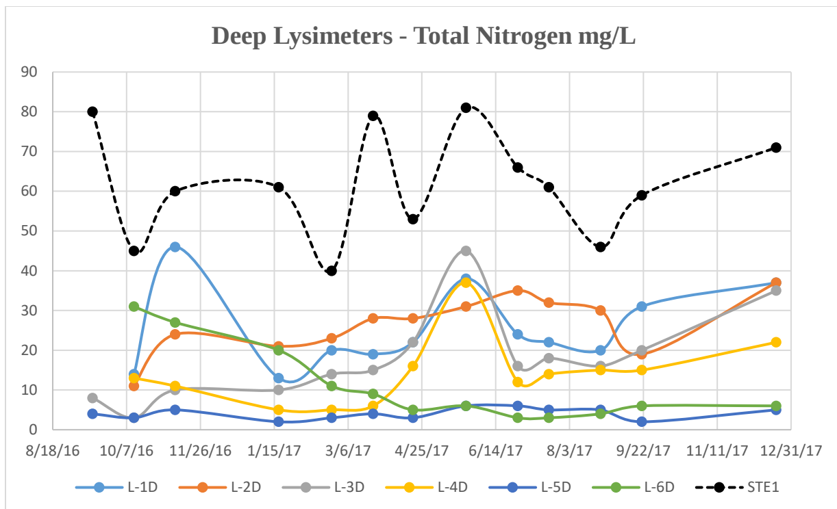
Figure 11. Deep Lysimeters – Total Nitrogen mg/L
