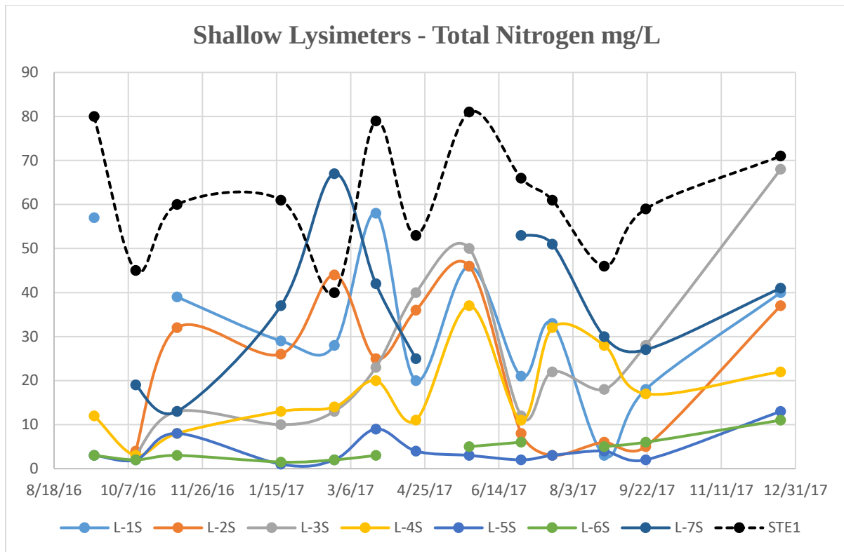
Figure 5. Shallow Lysimeters – Total Nitrogen mg/L
