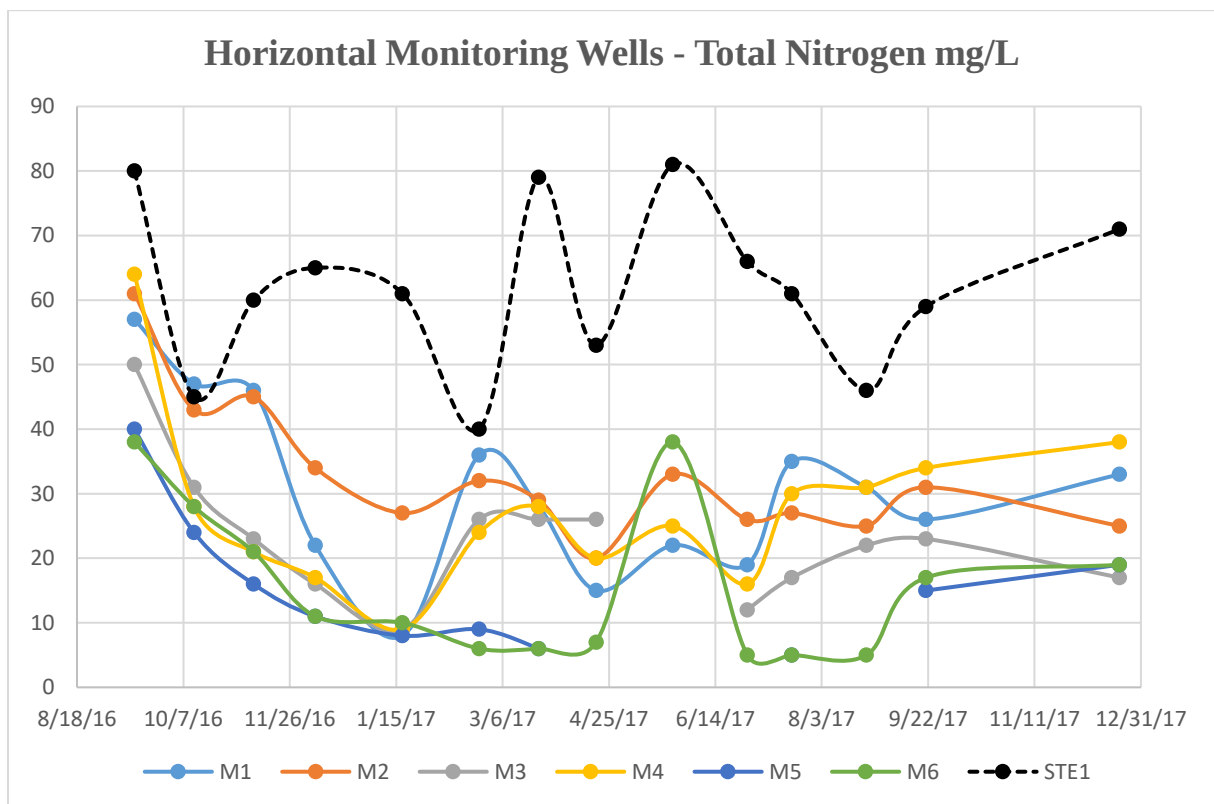
Figure 8. Horizontal Monitoring Wells – Total Nitrogen mg/L
