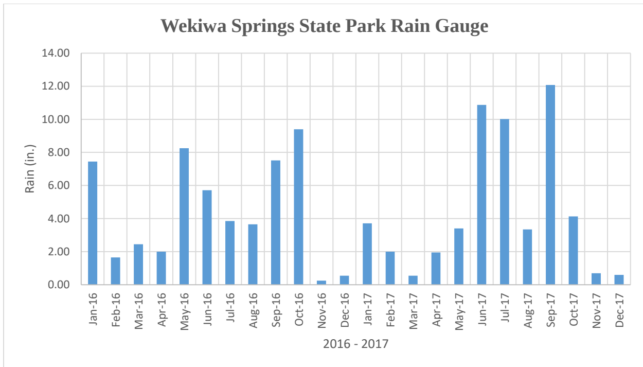
Figure 3. Monthly Rainfall Data 2016 – 2017 Wekiwa Springs State Park Rain Gauge
