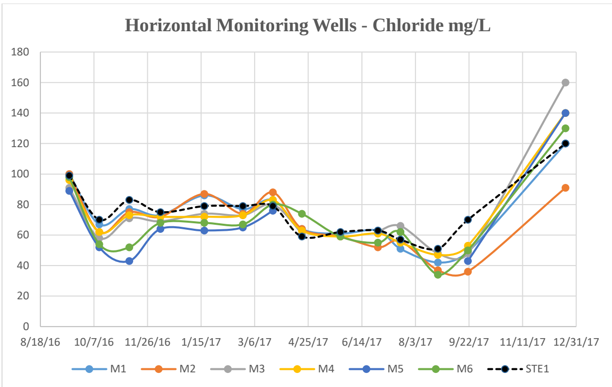
Figure 7. Horizontal Monitoring Wells – Chloride mg/L
