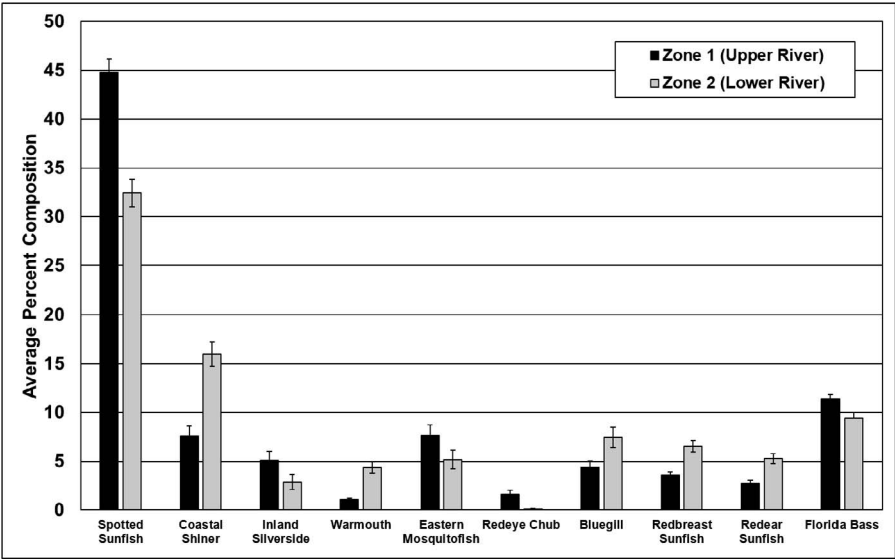
Figure 4. Average percent composition ( \pm standard error) of the ten species most attributing to the differences in fish communities between zones captured in the Rainbow River System during the study by zone (Zone 1 = Upper River, Zone 2 = Lower River).
