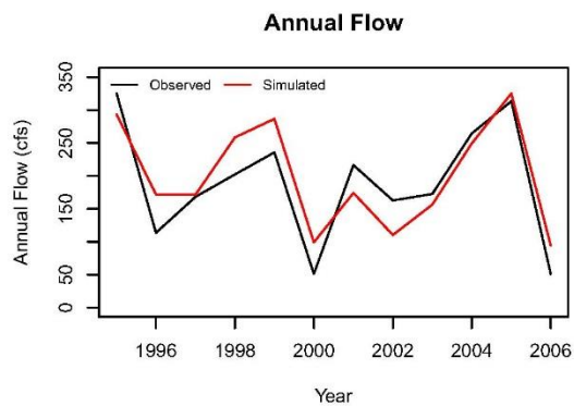
Comparison plots of observed vs simulated flow, concentration, and load at S49
