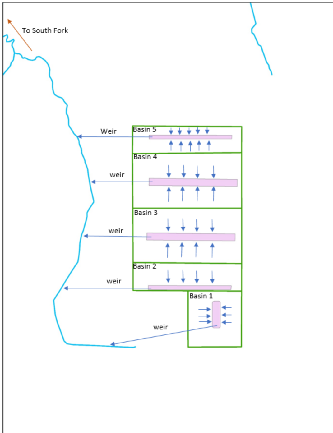
Figure 22. Model schematics accounting for HSL-01 project.
