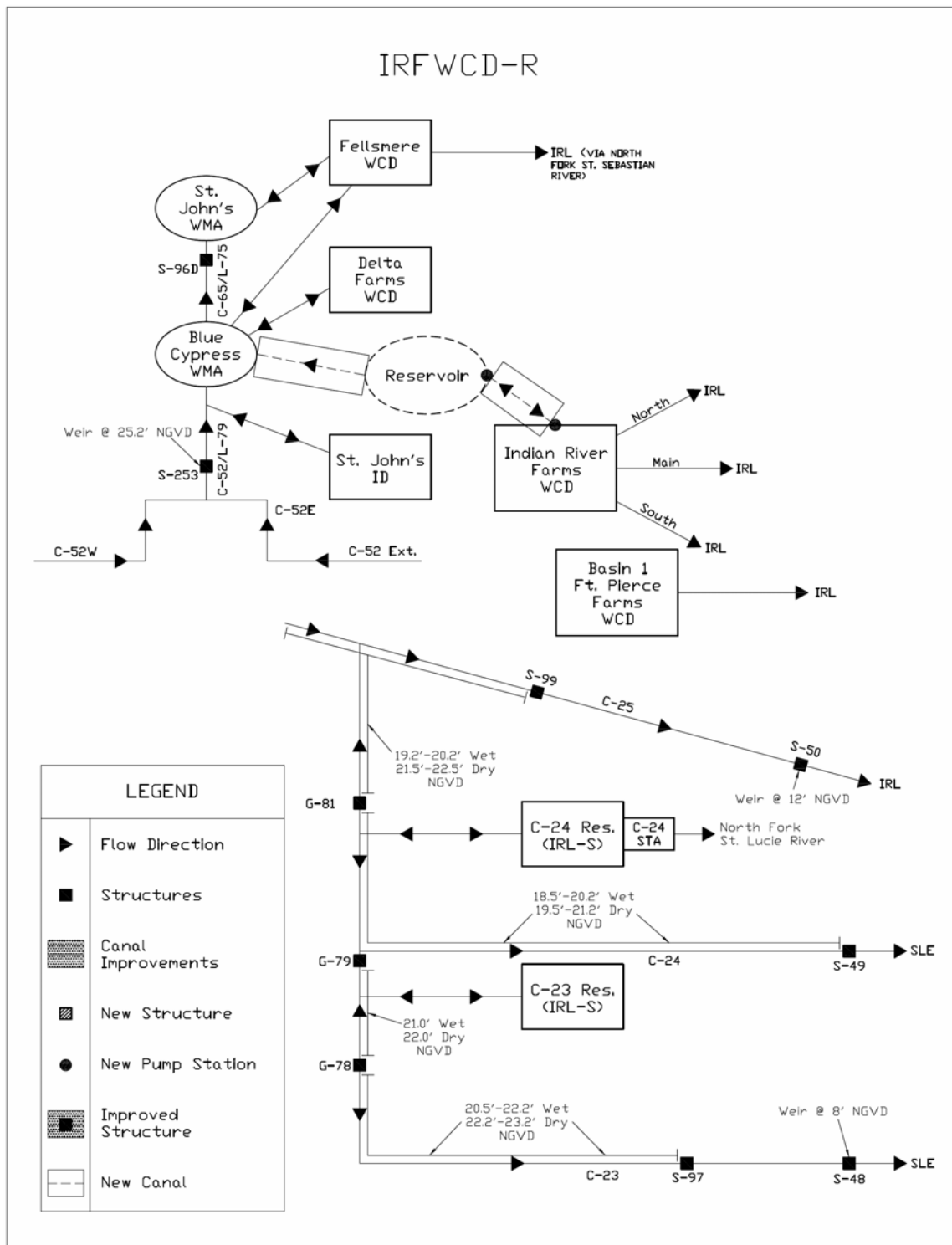
Figure 38. Schematic of the Indian River Farms Water Control District Reservoir Alternative.
