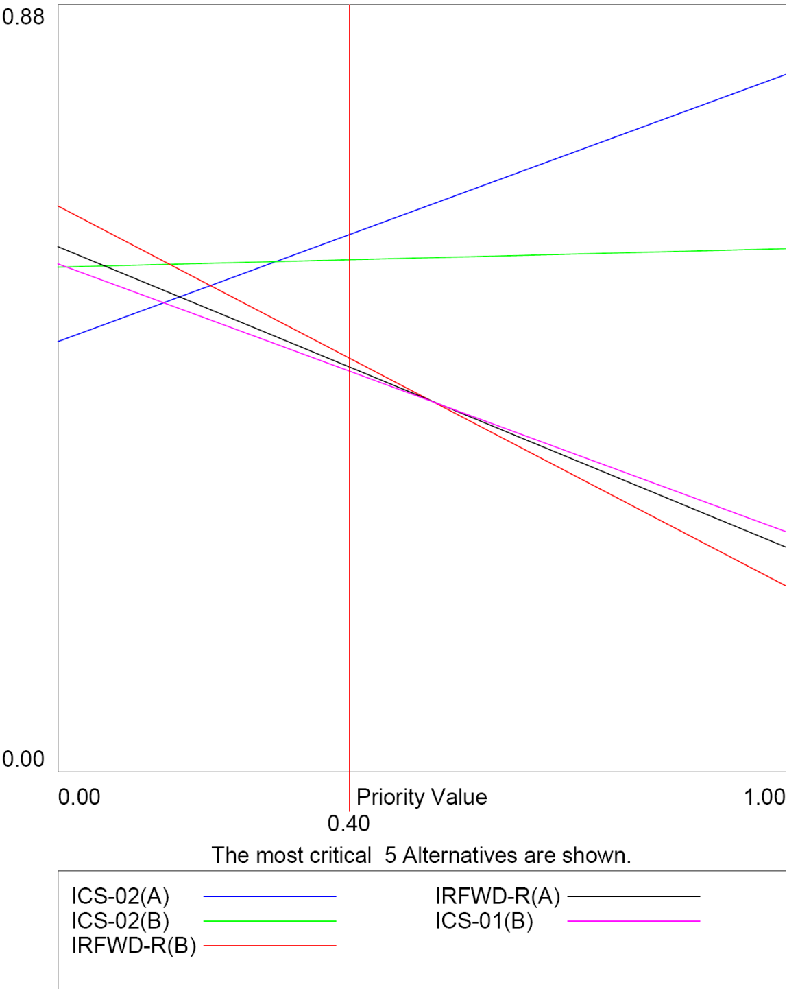
Figure 57. Sensitivity of alternative scores to the weighting applied to “discharge delivery rate”.
