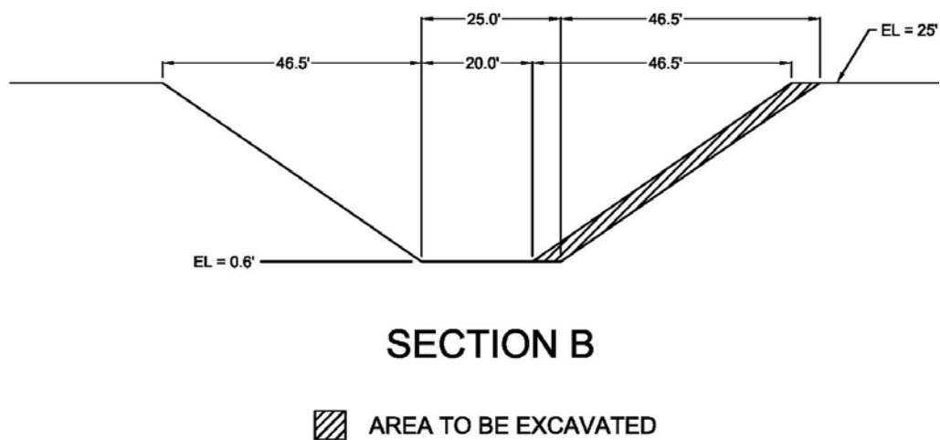
Figure 64. Proposed canal cross sections for C-25 improvements.
