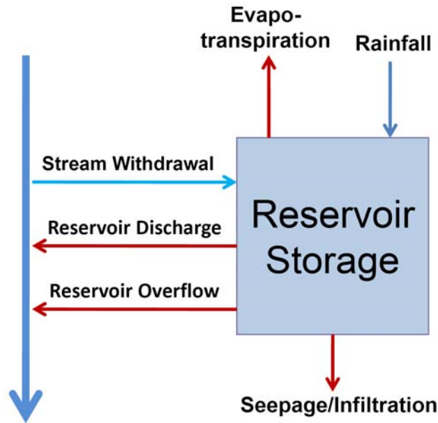
Figure 48. RESOPT water budget components.
