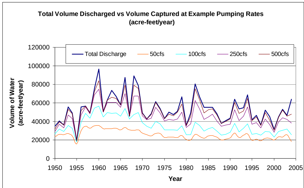
Figure 3. Potential Main Canal flow volumes that could be captured and stored based on pump capacities from 50 to 500 cfs (Figure 12, PBS&J 2006).
