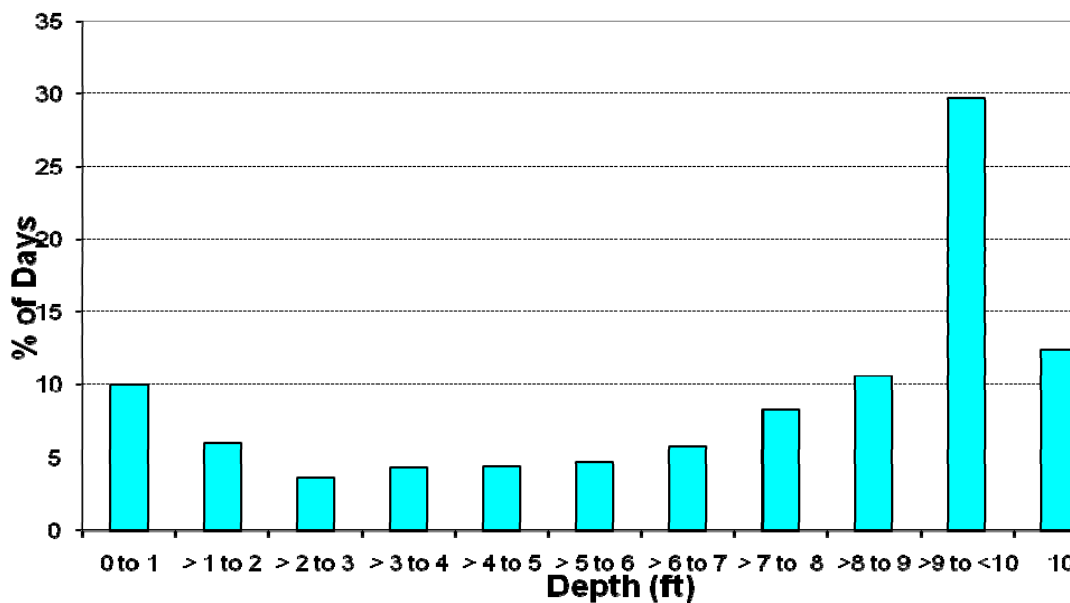
Figure 62. ICS-02(A) reservoir depth distribution with 185 cfs discharge delivery rate for the period of record 1965 to 2005.
