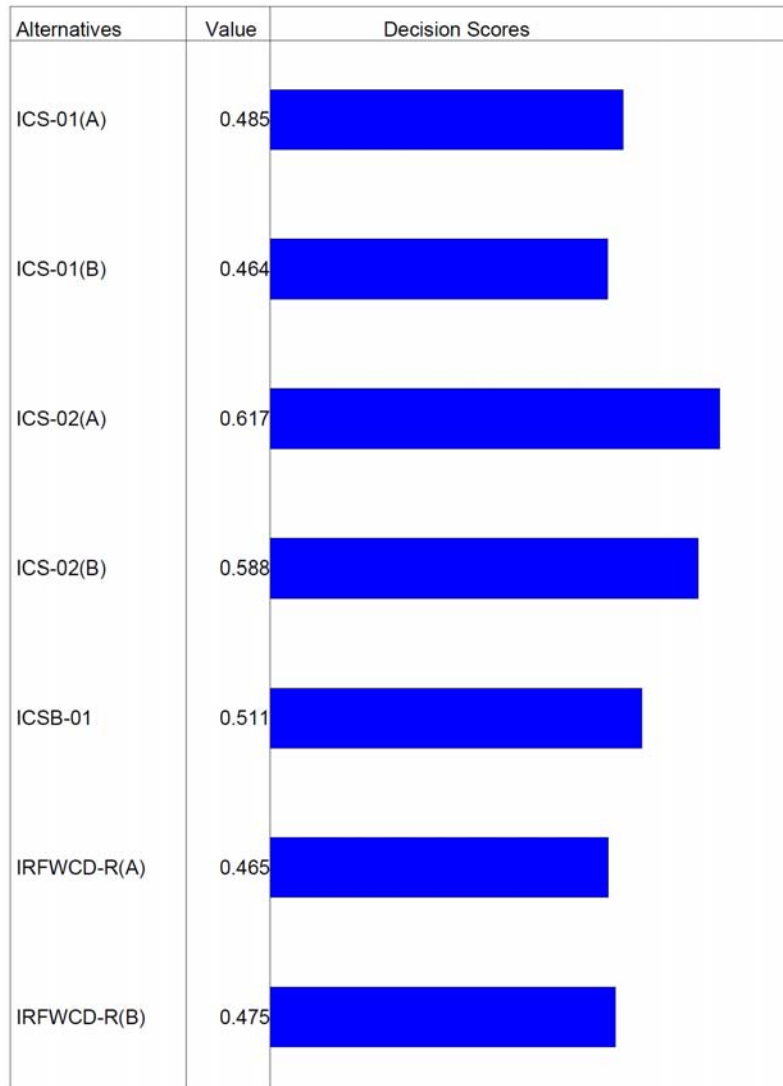
Figure 55. Alternative scores.
