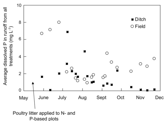
Fig. 2. Disconnected trends in field runoff and receiving ditch water quality for the 2003 growing season at Princess Anne, MD (data adapted from Kleinman et al., 2007).
