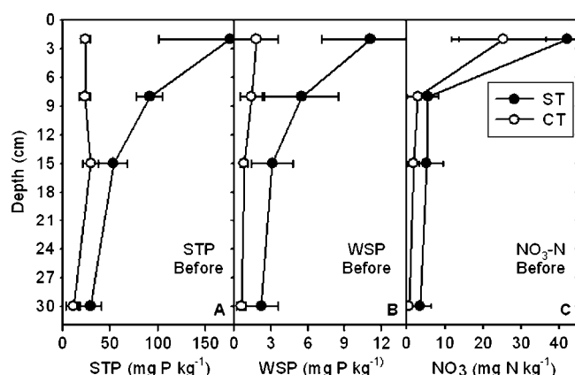
Fig. 2. Soil-extractable Mechlich I P (STP), water-soluble P (WSP), and NO 3 -N before rainfall simulations, with depth and between tillage treatments: strip tillage (ST) and conventional tillage (CT). Error bars are standard deviations.
