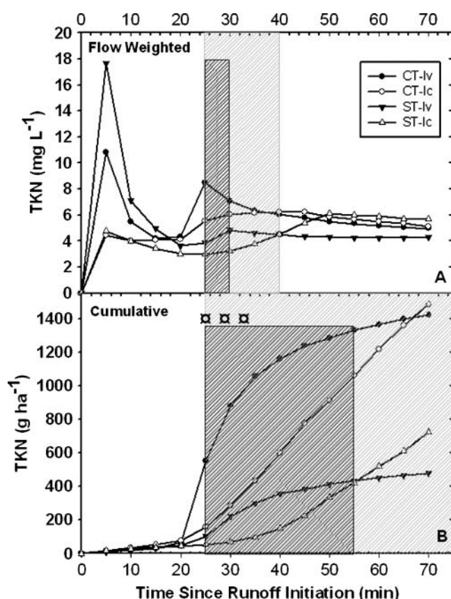
Fig. 6. (A) Cumulative flow-weighted concentrations of total N (TKN) for 70 min of runoff, and (B) cumulative total N (TKN) losses. Gray shading indicates a significant difference ( p < 0.05 ) between tillage treatments strip tillage (ST) and conventional tillage (CT). Black shading indicates a significant difference ( p < 0.05 ) between rainfall intensity patterns, constant rate (Ic) and variable rate (Iv). The symbol □ indicates interaction was significant ( p < 0.05 ) between tillage and intensity pattern for runoff periods (5 min) above which are labeled.
