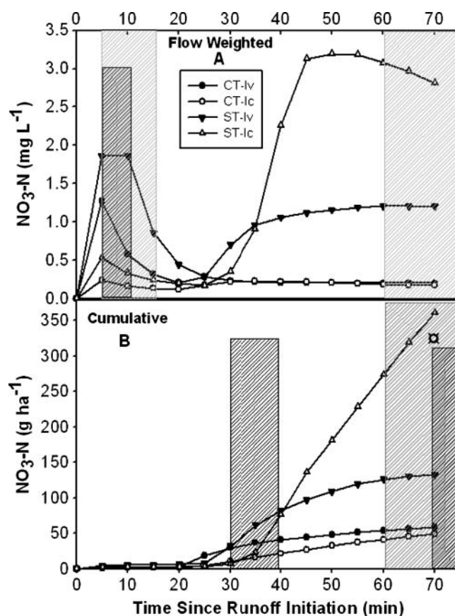
Fig. 5. (A) Cumulative flow-weighted concentrations of \text{NO}_3\text{-N} for 70 min of runoff, and (B) cumulative \text{NO}_3\text{-N} losses. Gray shading indicates a significant difference ( p < 0.05 ) between tillage treatments, strip tillage (ST) and conventional tillage (CT). Black shading indicates a significant difference ( p < 0.05 ) between rainfall intensity patterns, constant rate (Ic) and variable rate (Iv). The symbol □ indicates interaction was significant ( p < 0.05 ) between tillage and intensity pattern for runoff periods above which are labeled.
