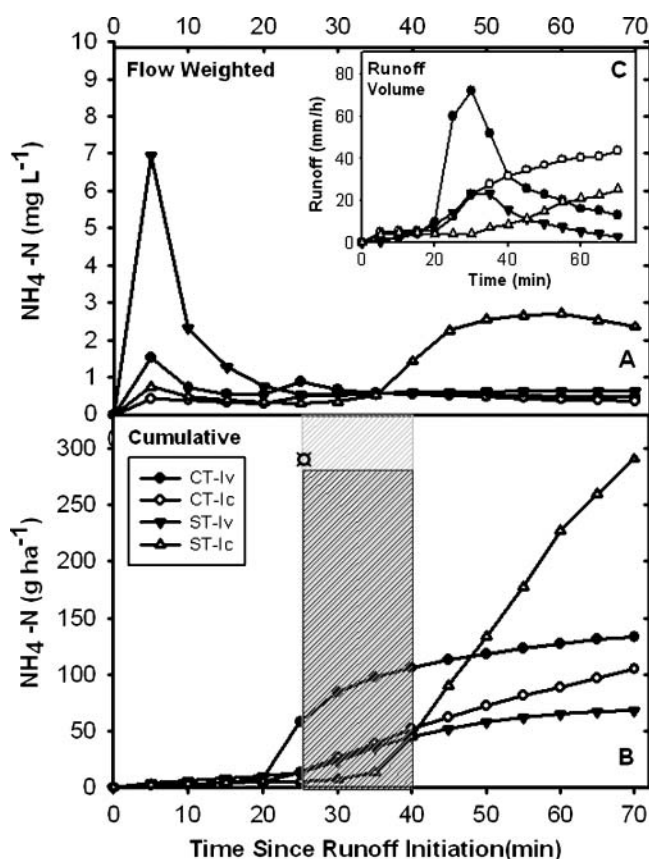
Fig. 3. (A) Cumulative flow-weighted concentrations of NH 4 -N for 70 min of runoff, and (B) cumulative NH 4 -N losses. The symbol at each 5-min period represents a composite sample for that time period and treatment. Gray shading indicates a significant difference ( p < 0.05 ) between tillage treatments strip tillage (ST) and conventional tillage (CT). Black shading indicates a significant difference ( p < 0.05 ) between rainfall intensity patterns, constant rate (Ic) and variable rate (Iv). The symbol □ indicates interaction was significant ( p < 0.05 ) between tillage and intensity pattern for runoff periods (5 min) above which are labeled. In graph A, the inserted graph depicts runoff rates for each treatment studied.
