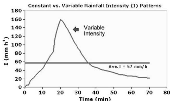
Fig. 1. Rainfall intensity patterns for constant and variable intensity treatments.
