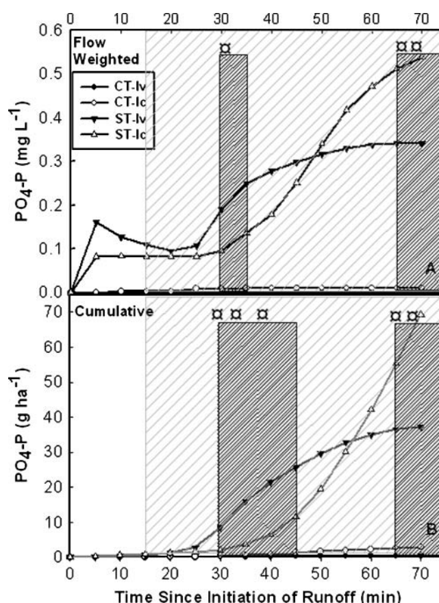
Fig. 7. (A) Cumulative flow-weighted concentrations of \text{PO}_4\text{-P} for 70 min of runoff, and (B) cumulative \text{PO}_4\text{-P} losses. Gray shading indicates a significant difference ( p < 0.05 ) between tillage treatments, strip tillage (ST) and conventional tillage (CT). Black shading indicates a significant difference ( p < 0.05 ) between rainfall intensity patterns, constant rate (Ic) and variable rate (Iv). The symbol □ indicates interaction was significant ( p < 0.05 ) between tillage and intensity pattern for runoff periods above which are labeled.
