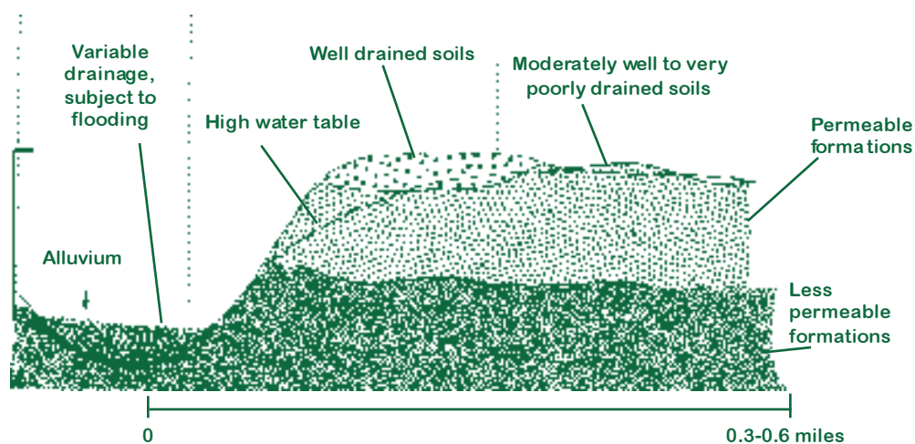
Figure 14. Relationship between landscape position, water table depth, and soil series in the Middle Coastal Plain (from Daniels et al., 1984).
