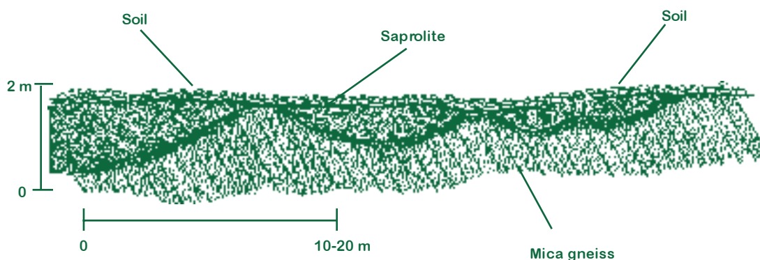
Figure 15. Relationship between soil and saprolite (from Daniels et al., 1984).
