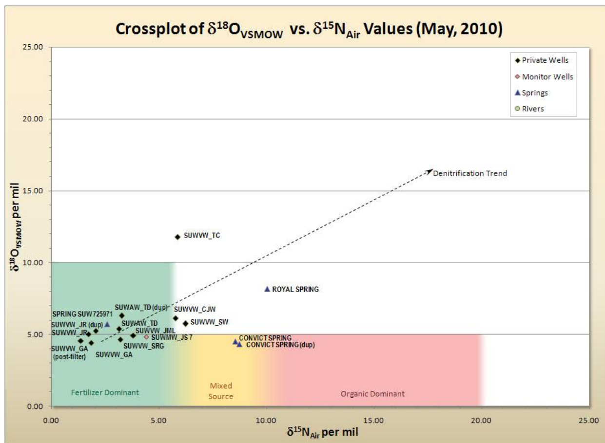
Figure 17. \delta^{15}\text{N} versus \delta^{18}\text{O} for May samples.
