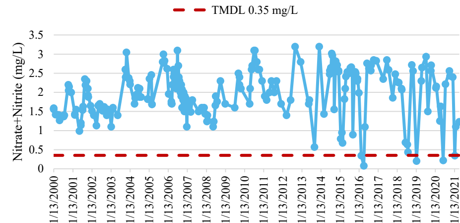
Troy Spring Nitrate Concentration
