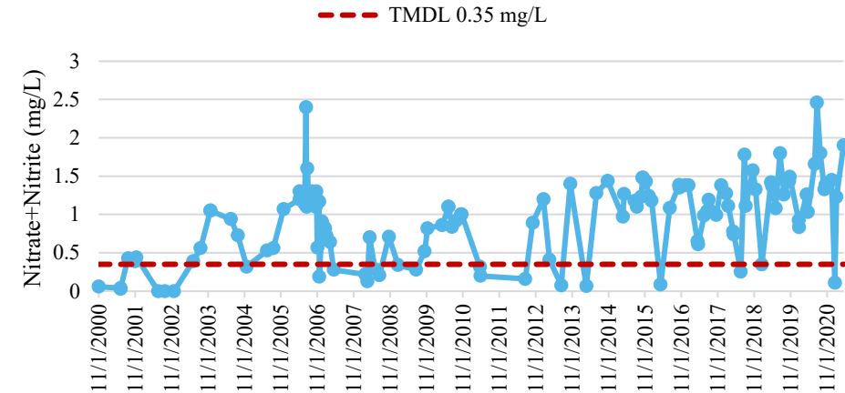
Falmouth Spring Nitrate Concentration
