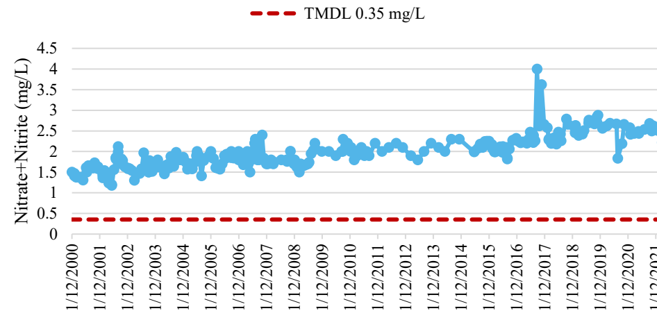
Manatee Springs Nitrate Concentration
