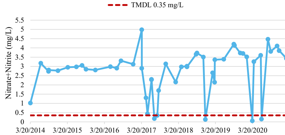
Peacock Springs Nitrate Concentration
