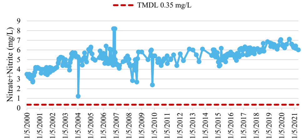
Fanning Springs Nitrate Concentration
