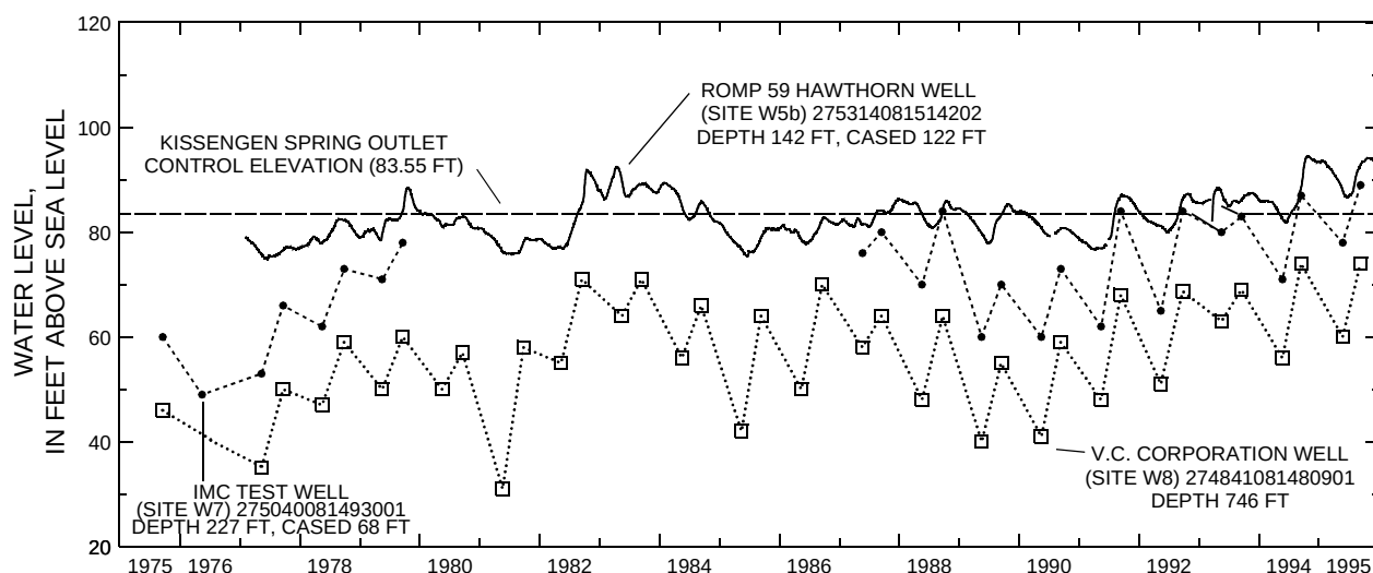
Figure 14. Ground-water levels in the intermediate aquifer system at the ROMP 59 Hawthorn well and in the Upper Floridan aquifer at the V.C. Corporation well, and composite ground-water levels in the intermediate aquifer system and Upper Floridan aquifer in the IMC Test Well, 1975-95.
