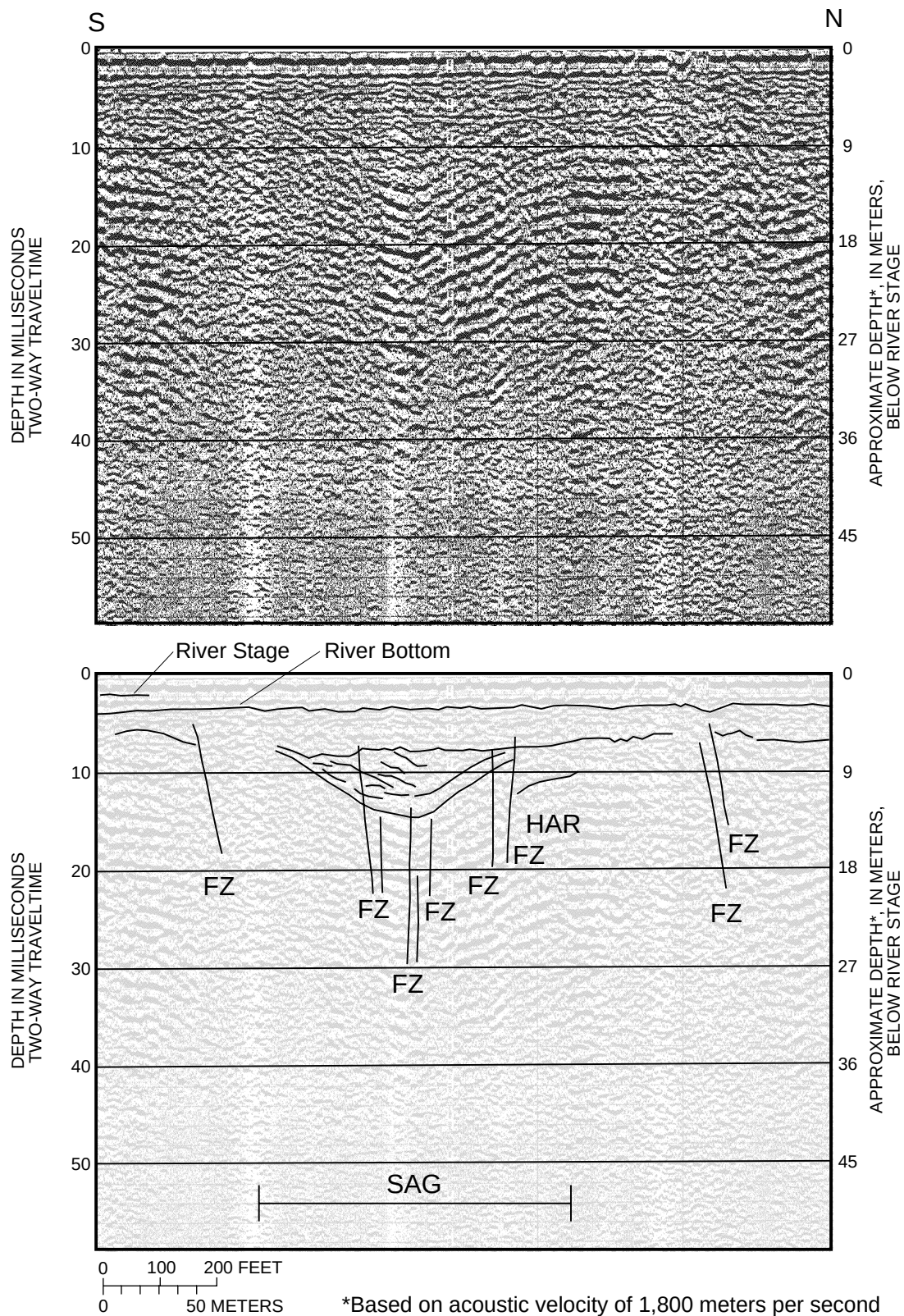
Figure 31d. Seismic-reflection profile and interpretation along the middle Peace River south of Fort Meade. (See figure 24 for location.)
