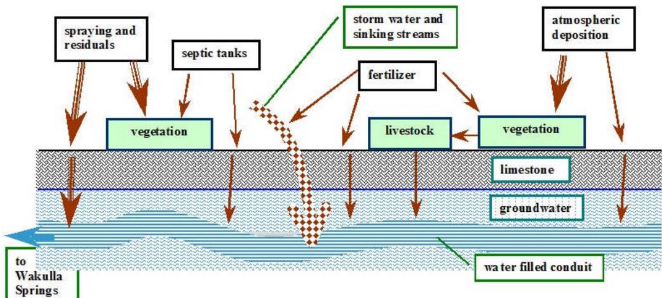
FIGURE 8: SCHEMATIC OF SOURCES, RESERVOIRS, AND PATHWAYS OF NITROGEN IN THE UNCONFINED PORTION OF THE WAKULLA SPRINGSHED
