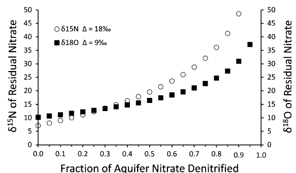
Fig. 5 Results from modeling the isotopic dynamics of nitrate in the Floridan aquifer as a closed system with single source with \delta^{15}\text{N} of 7.1‰ and \delta^{18}\text{O} of 10.2‰ which is affected by denitrification. Open circles denote \delta^{15}\text{N} and filled squares denote \delta^{18}\text{O} behavior. Closed system Rayleigh equations were used to model the isotopic dynamics (Fry 2006). Setting the fractionations factors for denitrification to 18‰ for ^{15}\text{N} and 9‰ for ^{18}\text{O} yielded residual nitrate with \delta^{15}\text{N-NO}_3 of approximately +20‰ and \delta^{18}\text{O-NO}_3 of +15‰, when 50% of the nitrate was lost to denitrification
