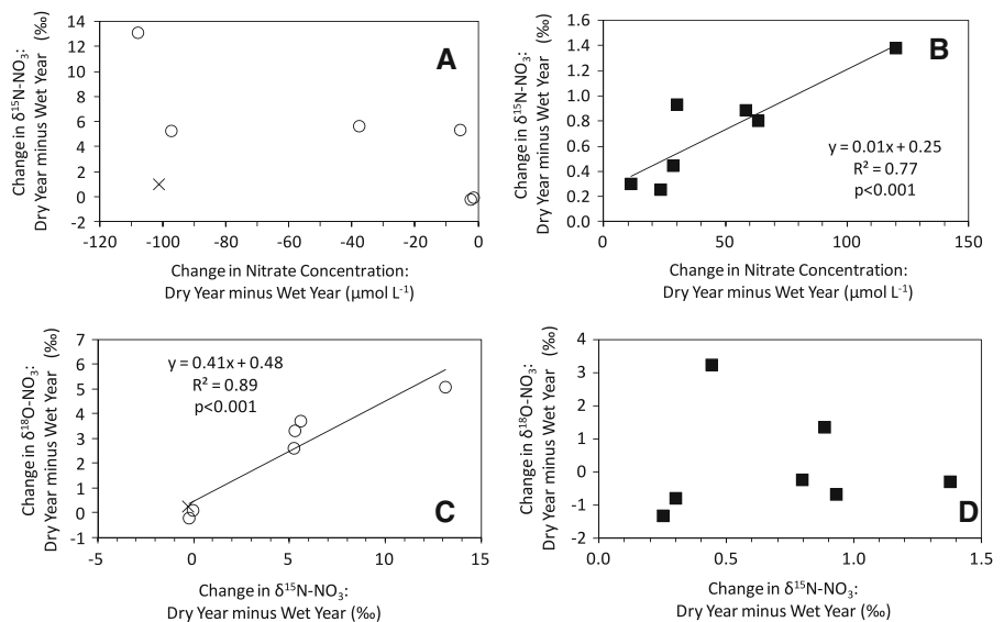
Fig. 4 Relationships between the \delta^{15}\text{N} values of nitrate and nitrate concentration in years with above normal (“Wet”) and below normal (“Dry”) precipitation. We considered 2005/2006 to be wet years and 2008 was considered a dry year. In these analyses we separated springs in which nitrate decreased from 2005/2006 to 2008 (a and c) from springs in which nitrate increased (b and d)
