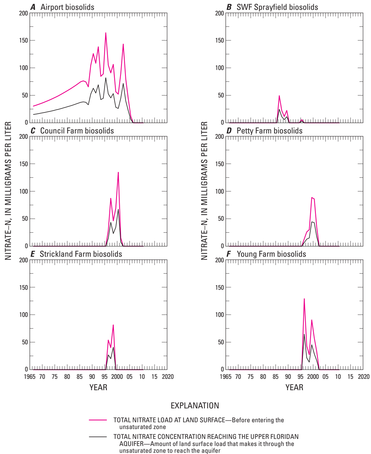
Figure 17. Land surface nitrate-N concentration and concentration recharging the Upper Floridan aquifer from biosolids disposal for the A , Tallahassee airport, B , Southwest Farm (SWF) sprayfield, and C , Council, D , Petty, E , Strickland, and F , Young farm sites (shown on fig. 1).
