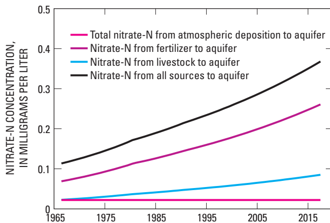
Figure 40. Simulated nitrate-N concentrations in recharge from atmospheric deposition, fertilizer, livestock, and total sources in the Leon County part of the study area (excluding the uninhabited areas).
