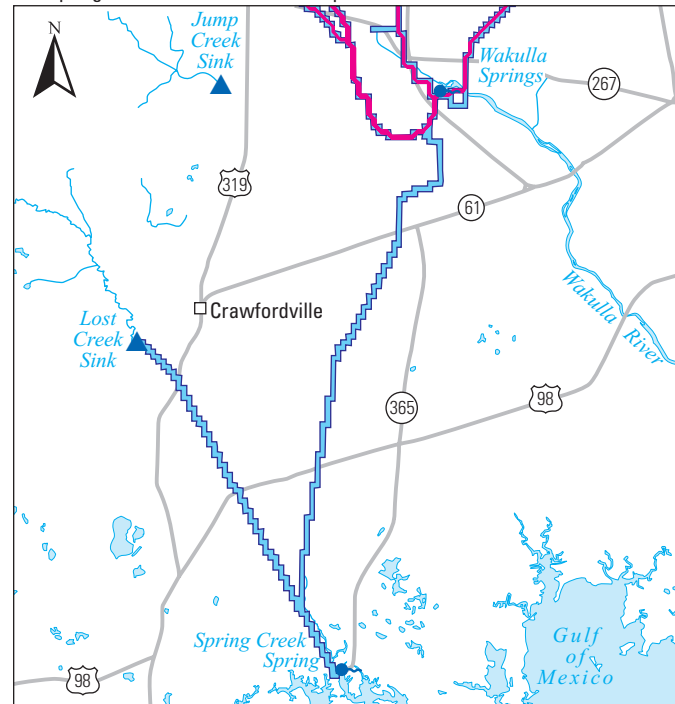
B Simulated Wakulla Springs flow = 655 cubic feet per second and simulated Spring Creek flow = 87 cubic feet per second
