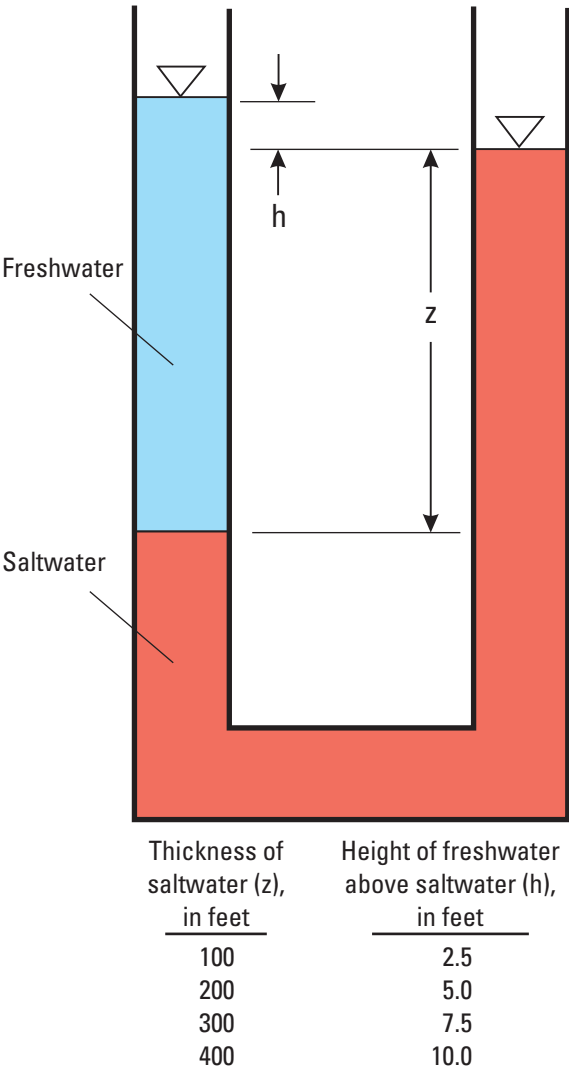
Figure 12. Hydrostatic balance between freshwater and saltwater illustrated by a U-tube (modified from Todd, 1980).
