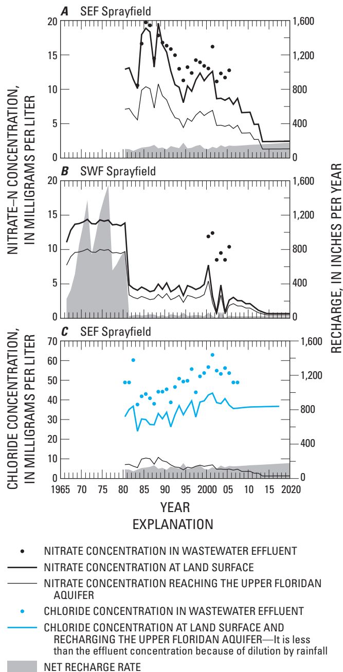
Figure 14. Nitrate-N and chloride concentrations and recharge rates at the Southeast Farm (SEF) and Southwest Farm (SWF) sprayfields. (Data from Jamie Shakar, City of Tallahassee, written commun., 2005).
