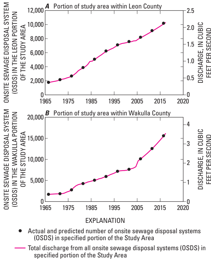
Figure 29. Total onsite sewage disposal system (OSDS) discharges for Leon and Wakulla Counties.
