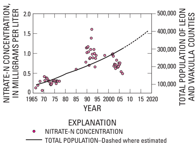
Figure 2. Nitrate-N concentration in Wakulla Springs from 1966 through 2007 compared to Leon and Wakulla County population. (Data sources: Population data is from the U.S. Census Bureau (2005), nitrate-N concentrations are from the U.S. Geological Survey and Jamie Shakar, City of Tallahassee, written commun., 2005).
