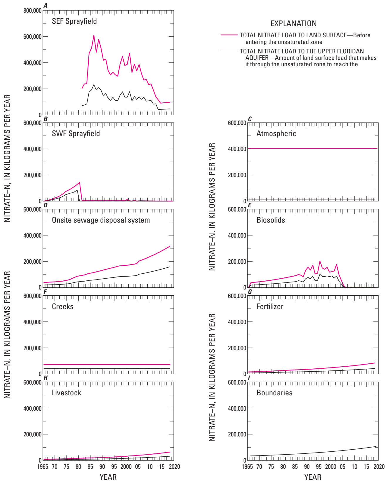
Figure 13. Nitrate-N loading to land surface and the Upper Floridan aquifer from 1966 through 2018.
