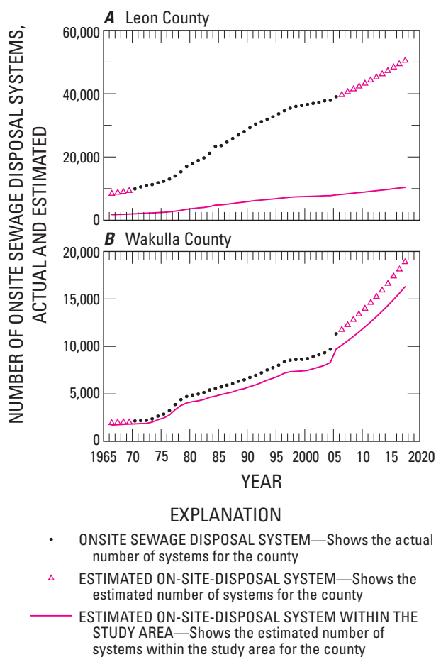
Figure 15. Actual and estimated number of onsite sewage disposal systems in A, Leon and B, Wakulla Counties from 1966 to 2018.
