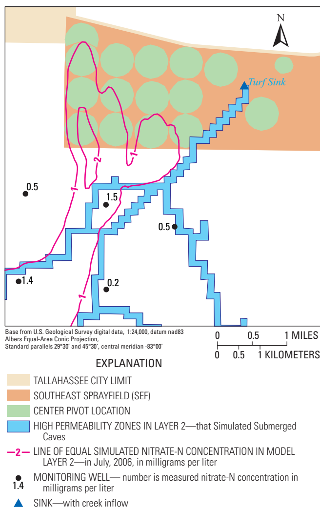
Figure 36. Simulated and measured nitrate-N concentrations at the Southeast Farm (SEF) sprayfield in model layer 2 in 2006.
