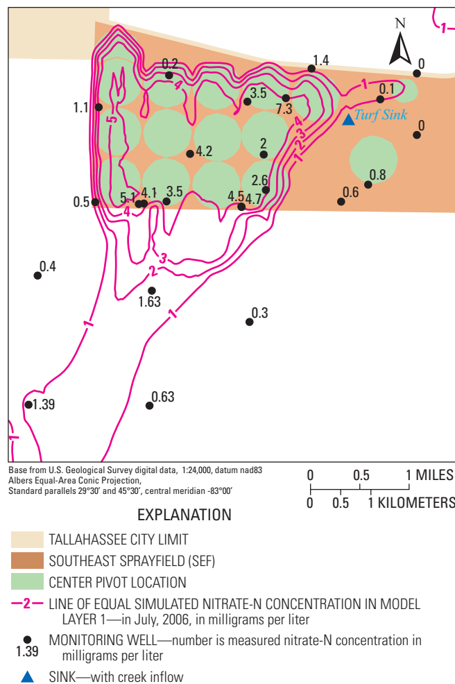
Figure 35. Simulated and measured nitrate-N concentrations at the Southeast Farm (SEF) sprayfield in model layer 1 in 2006.
