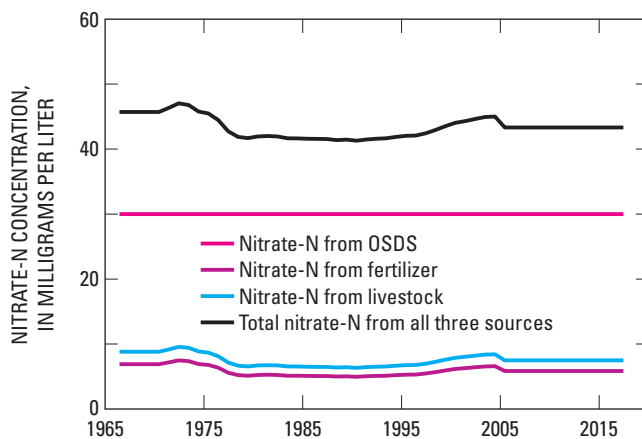
Figure 39. Simulated nitrate-N concentrations reaching the Upper Floridan aquifer at each onsite sewage disposal system (OSDS) location in Wakulla County (concentrations are the sum of OSDS, fertilizer, and livestock nitrate-N).
