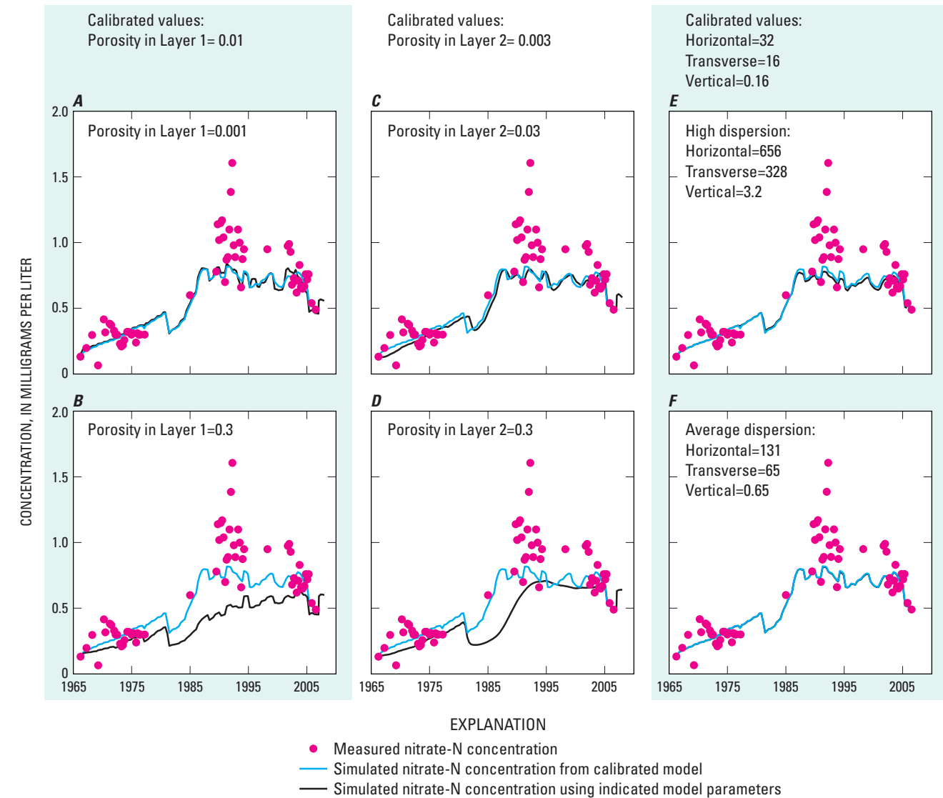
Figure 60. Results of the subregional fate and transport model sensitivity analysis.
