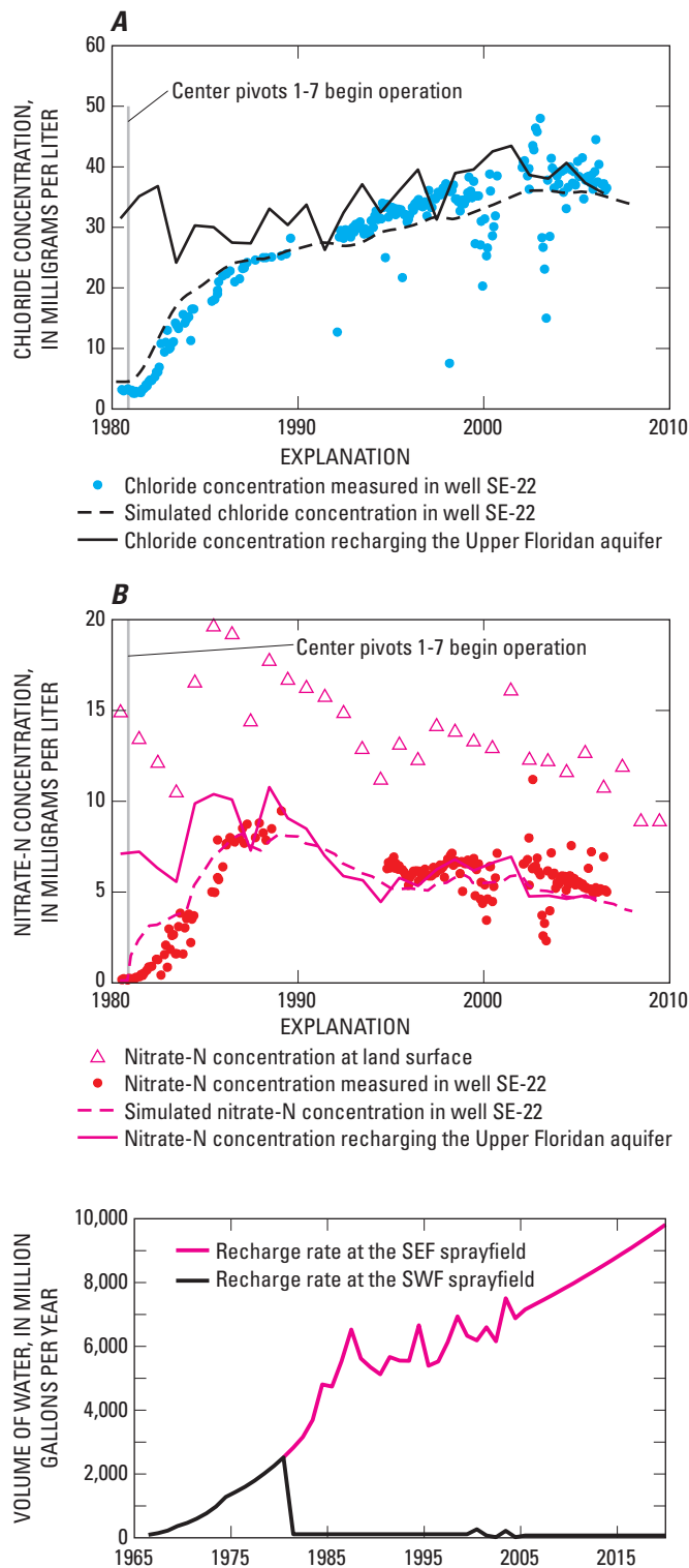
Figure 37. Measured and simulated A, chloride and B, nitrate-N concentrations at well SE-22 (location of well SE-22 is shown on figure 3).
