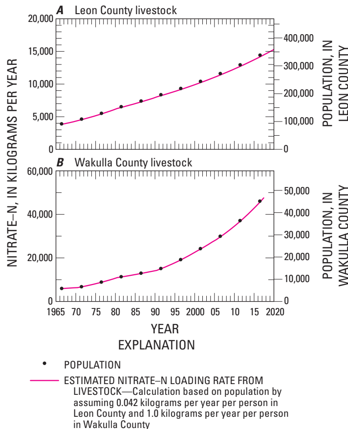
Figure 19. Nitrate-N loading from animal wastes on A, Leon, and B, Wakulla Counties.
