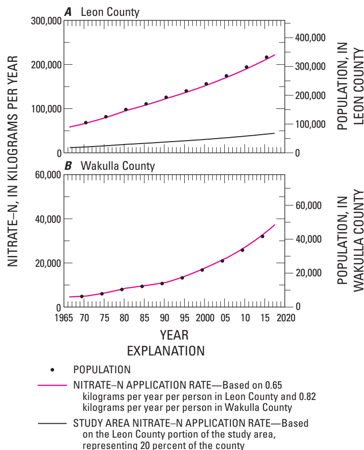
Figure 18. Nitrate-N load from domestic fertilizer application on A, Leon, and B, Wakulla Counties.
