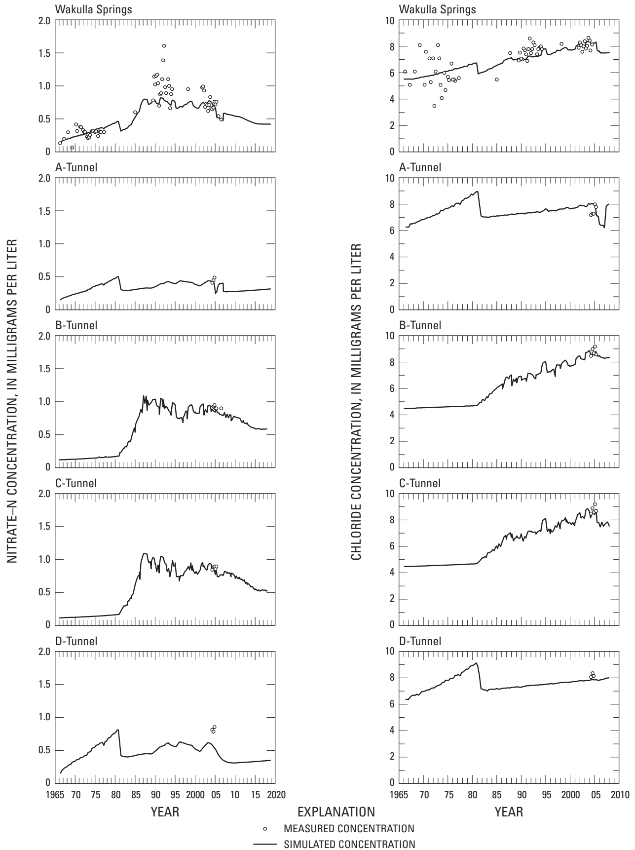
Figure 22. Measured and simulated nitrate-N and chloride concentrations in Wakulla Springs, A-, B-, C- and D-tunnels.
