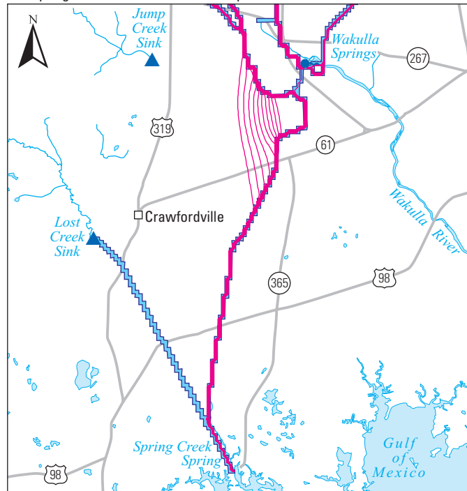
A Simulated Wakulla Springs flow = 368 cubic feet per second and simulated Spring Creek flow = 329 cubic feet per second
