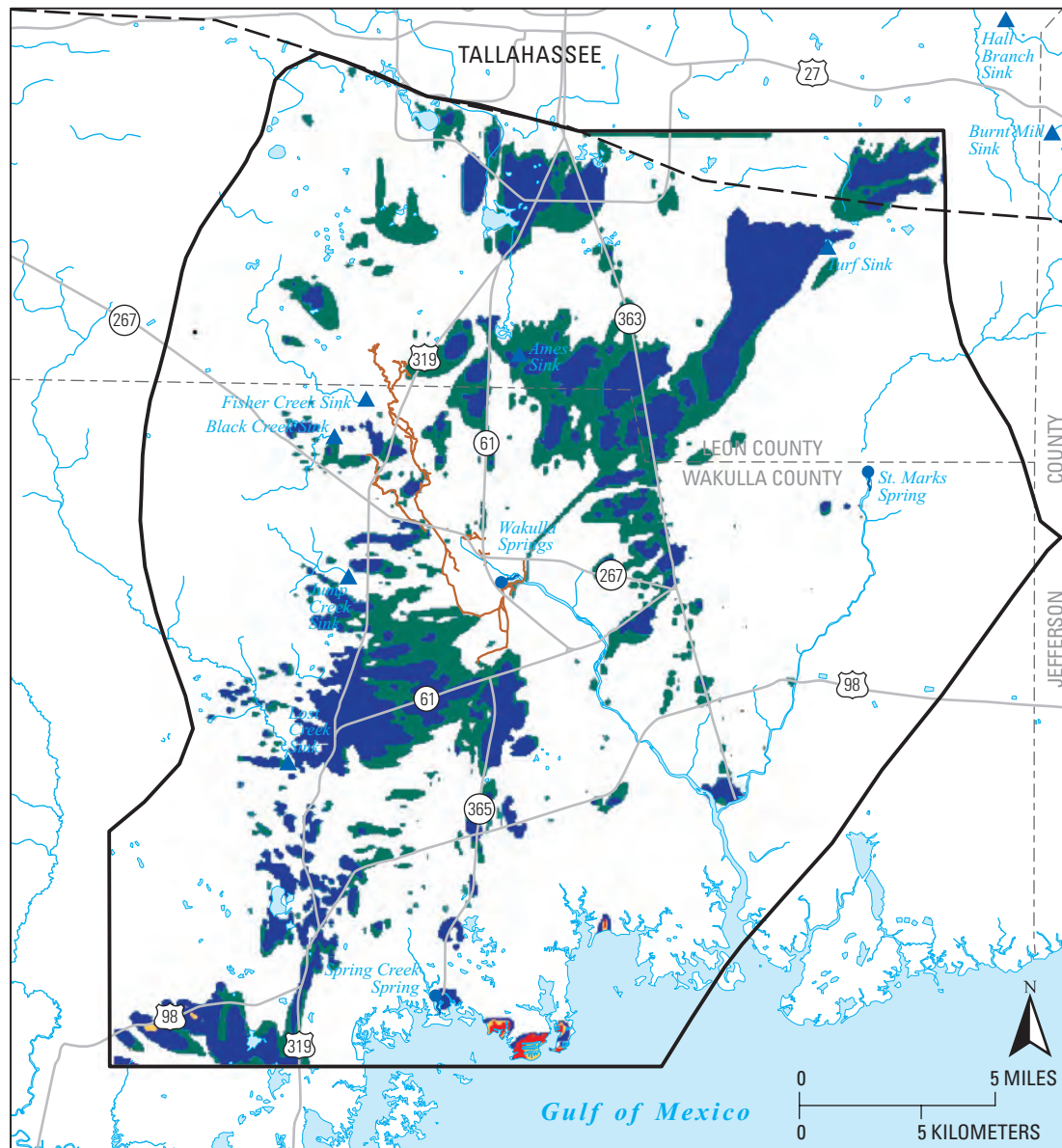
Figure 53. Simulated nitrate-N concentration in the Upper Floridan aquifer for scenario 2 in model layer 1 at the end of 2007, assuming Wakulla Springs is fully capturing the flow in the A-, K-, and R-tunnels.
