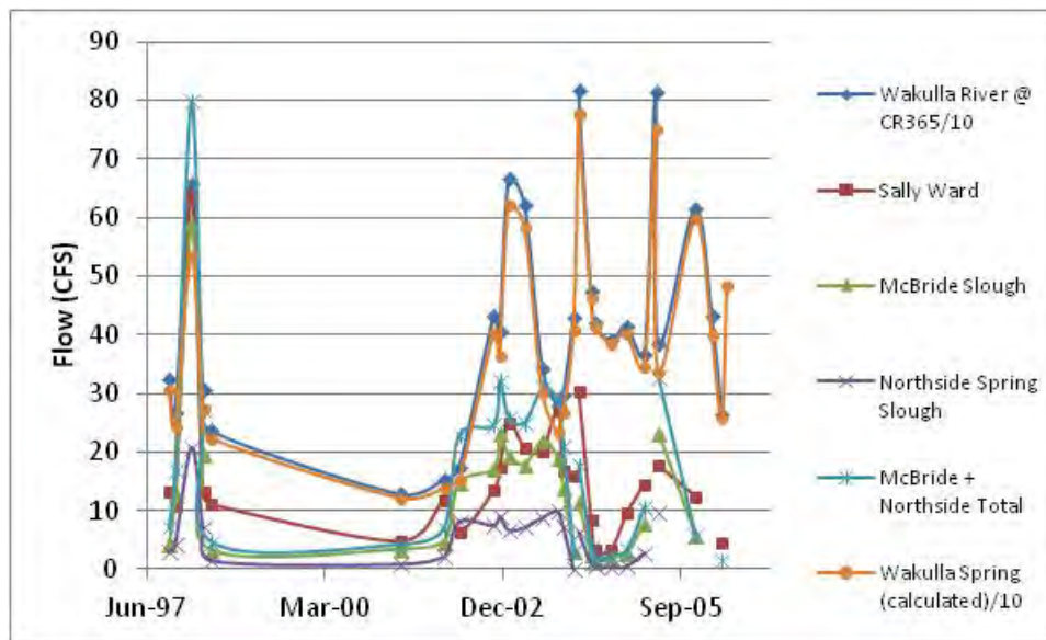
Figure 3.4. Flow (in cfs) in the Upper Wakulla River, Wakulla Spring, McBride Slough, Northside Spring, and Sally Ward Spring, 1997–2005
