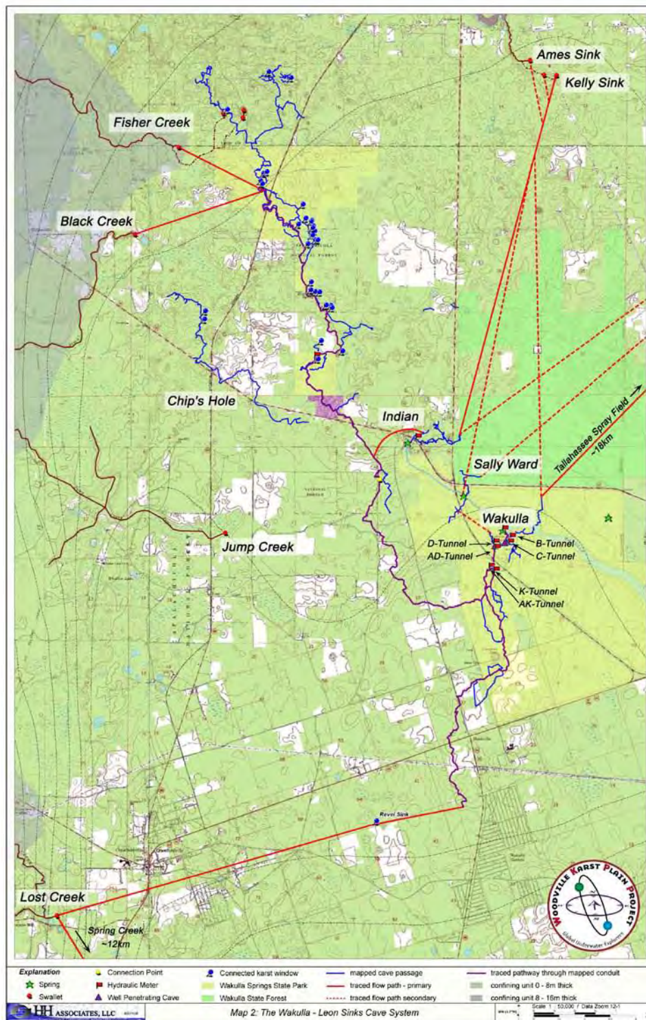
Figure 1.6. Wakulla Spring, Conduits and Sinking Streams
