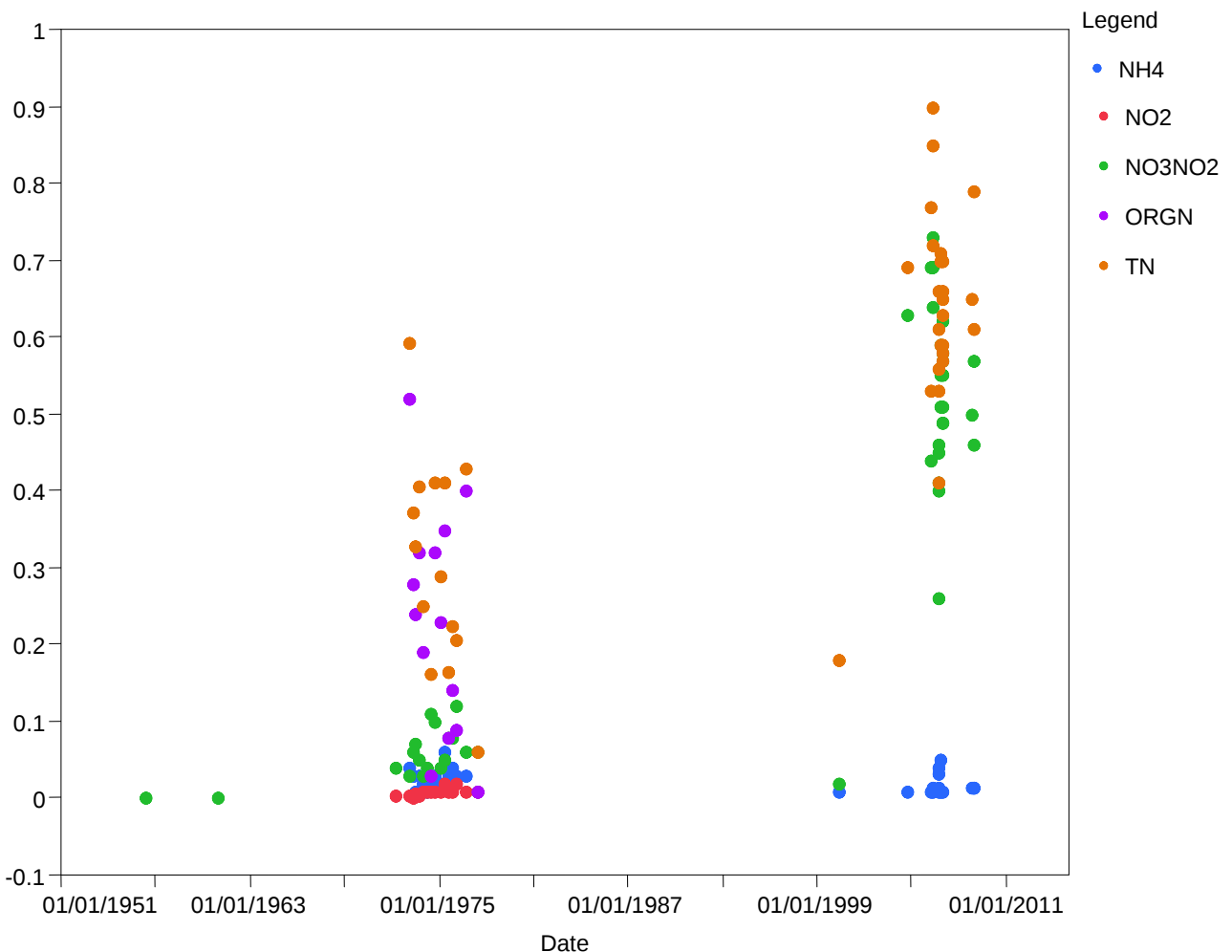
Figure 3.8. Nitrogen Species (in mg/L) for the Upper Wakulla River, 1951–2011
