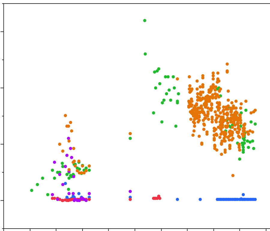
Figure 3.10. Nitrogen Species (in mg/L) for Wakulla Spring, without Outliers, 1961–2011
