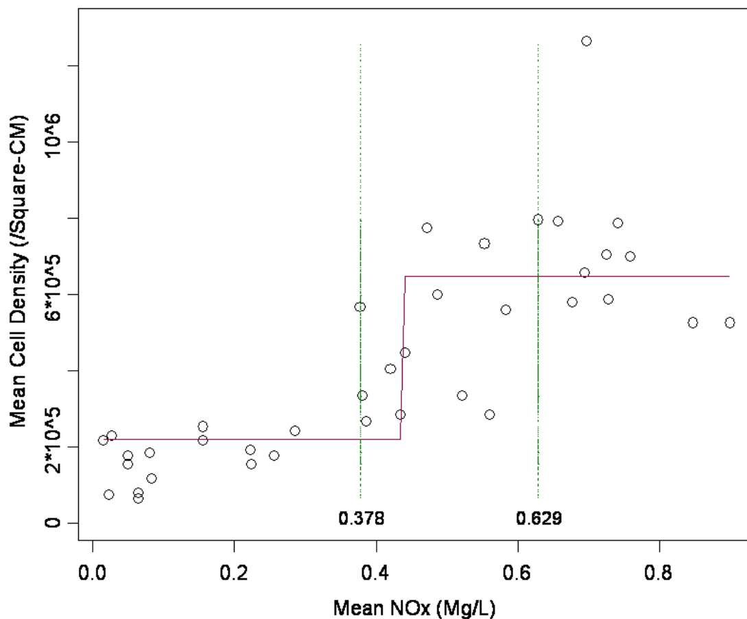
Figure 5.6. Change-Point Analyses (the 95% Confidence Interval)
