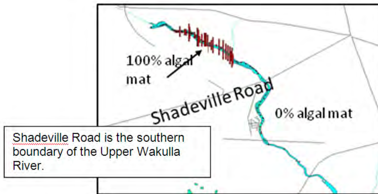
Figure 3.1. HAPI Survey Results (2001) Showing Algal Mat Distribution in the Upper Wakulla River
