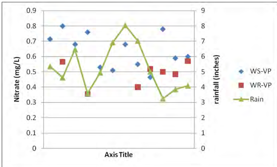
Figure 5.9. Monthly Median Nitrate Concentrations for Wakulla Spring and River for the Verified Period Data
