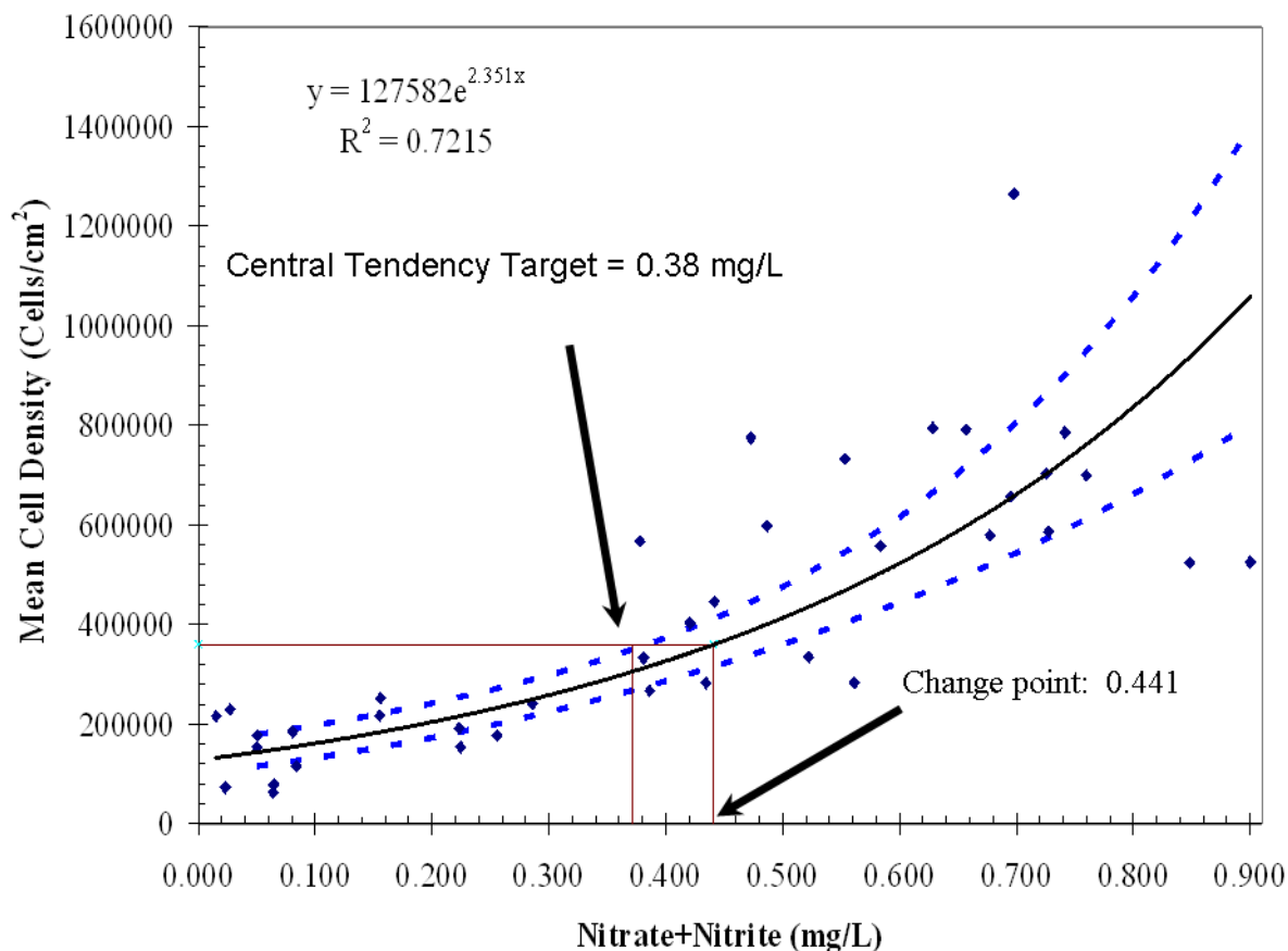
Figure 5.7. Central Tendency and Upper 95% Confidence Interval Approach
