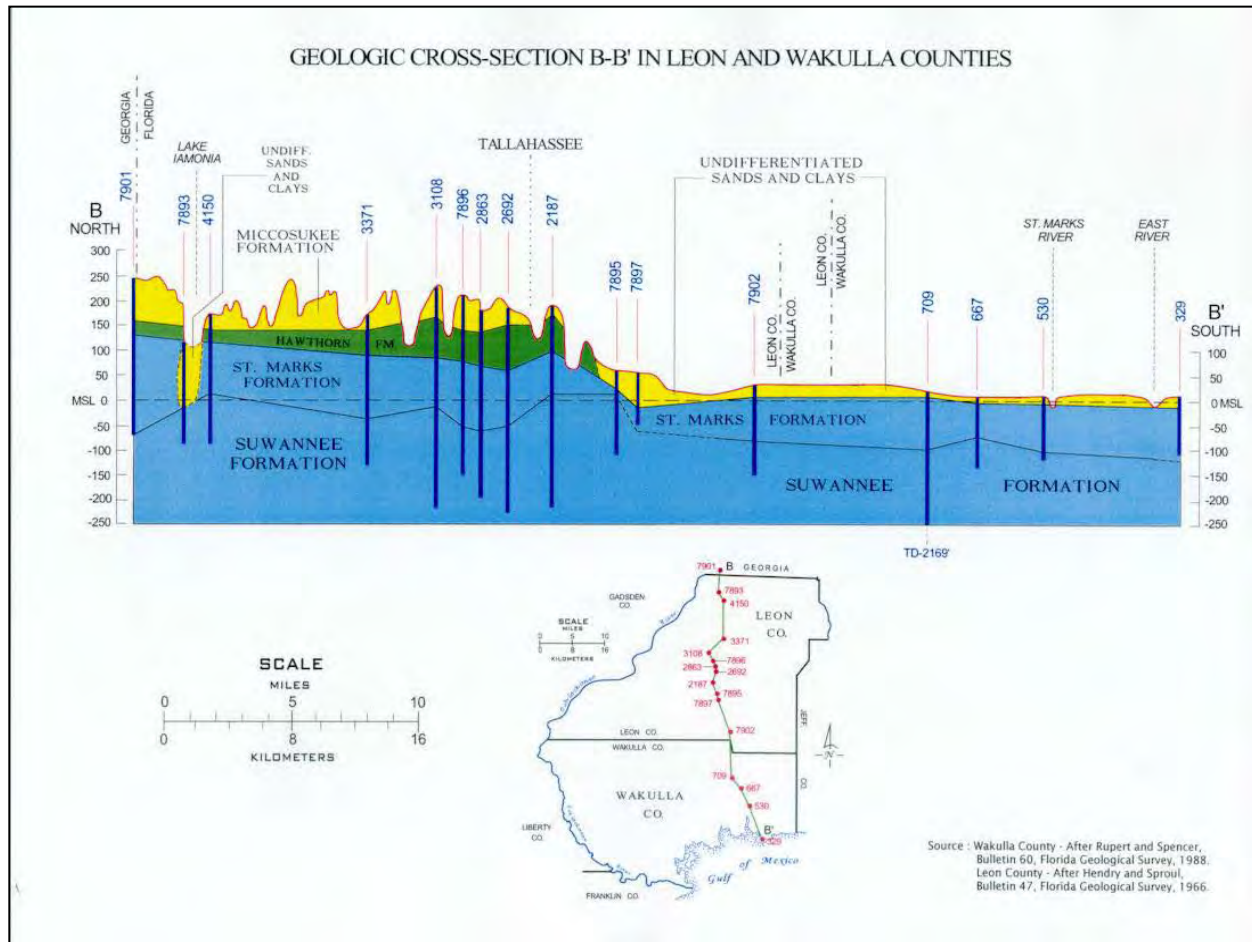
Figure 1.4. Generalized Geologic Cross-Section through the Wakulla River Watershed
