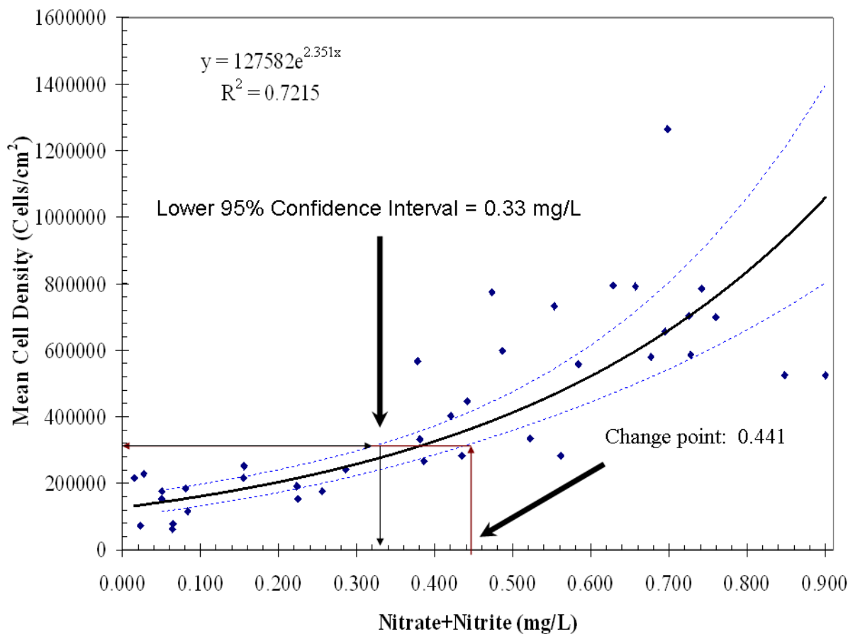
Figure 5.8. Upper and Lower 95% Confidence Interval Approach
