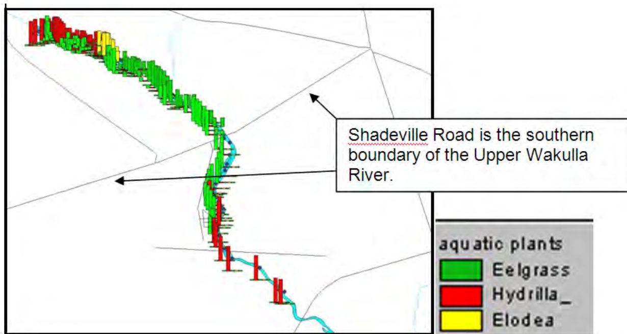
Figure 3.2. HAPI Survey Results (2001) Showing Macrophyte Distribution in the Upper and Middle Wakulla River
