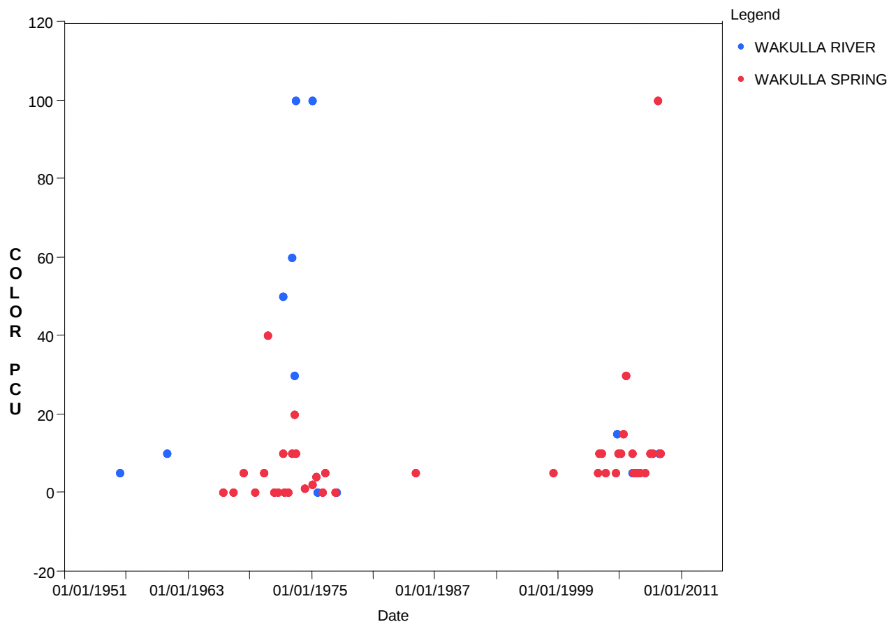
Figure 3.5. Color (in PCUs) in the Upper Wakulla River and Wakulla Spring, 1951–2011
