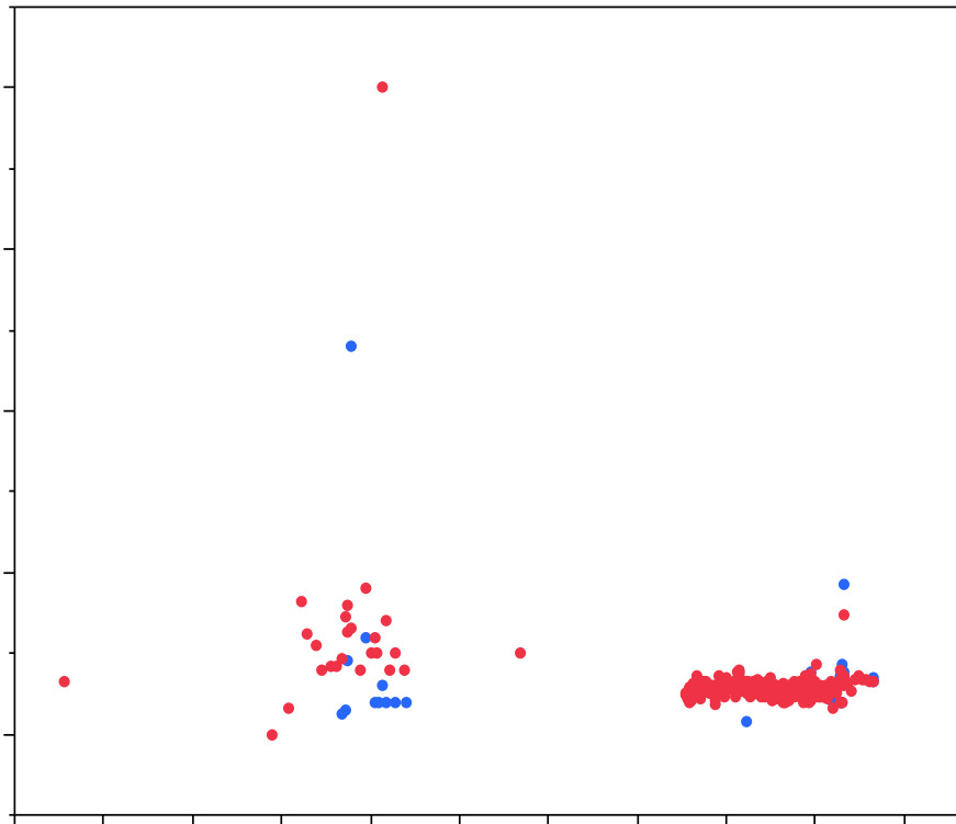
Figure 3.7. TP (in mg/L) in the Upper Wakulla River and Wakulla Spring, 1951–2011
