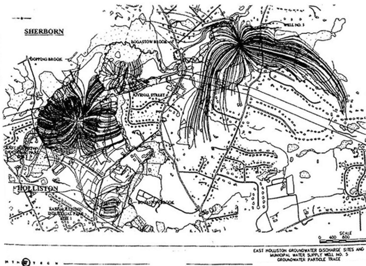
Figure 3-4 Particle Tracking of Wastewater Discharge and Nearby Water Supply Well Intake
