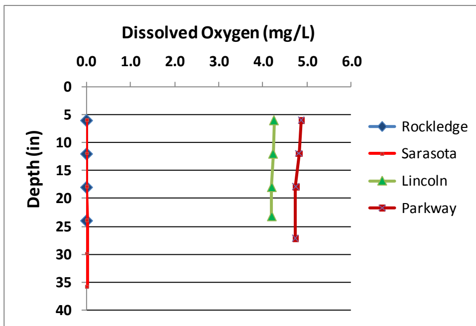
Figure 19 – Dissolved oxygen profiles in baffle boxes
