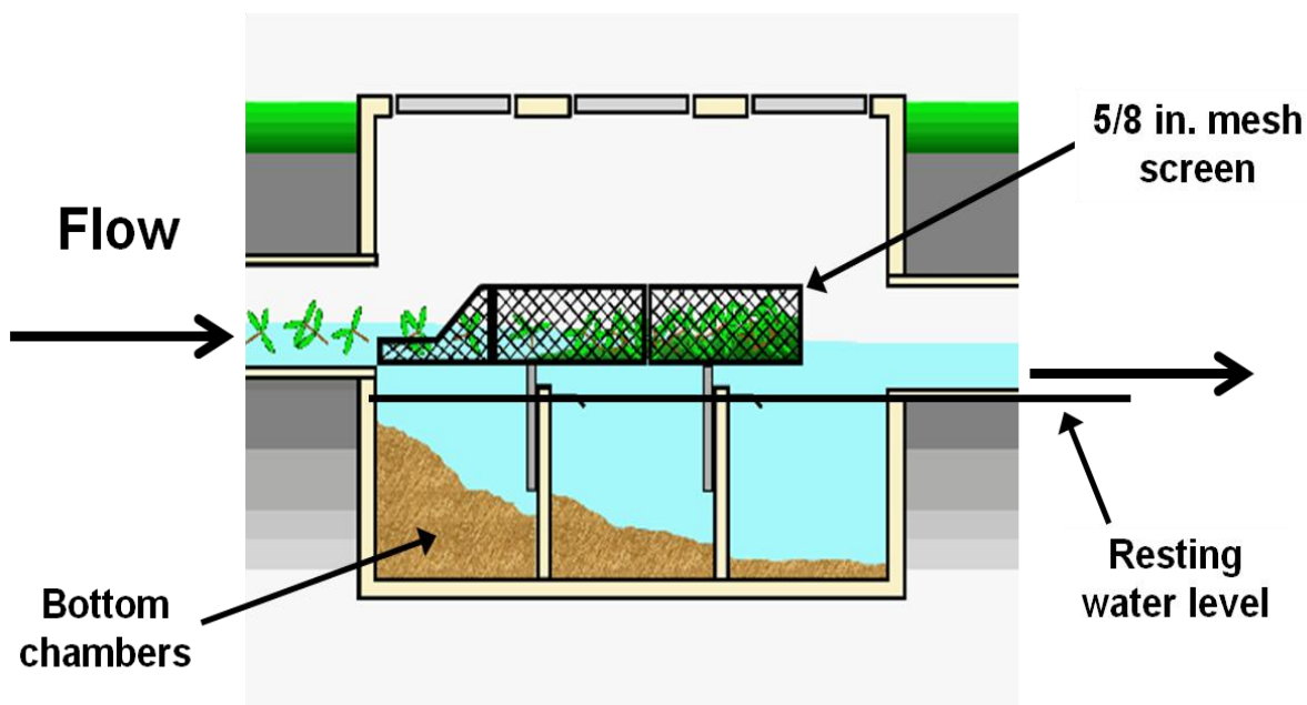
Figure 1 - Schematic of Type 2 baffle box showing sieve screen
