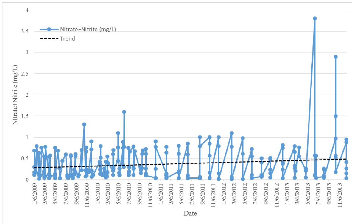
FIGURE 6: TRENDS IN NITRATE + NITRITE IN THE SANTA FE RIVER, 2009-2013
