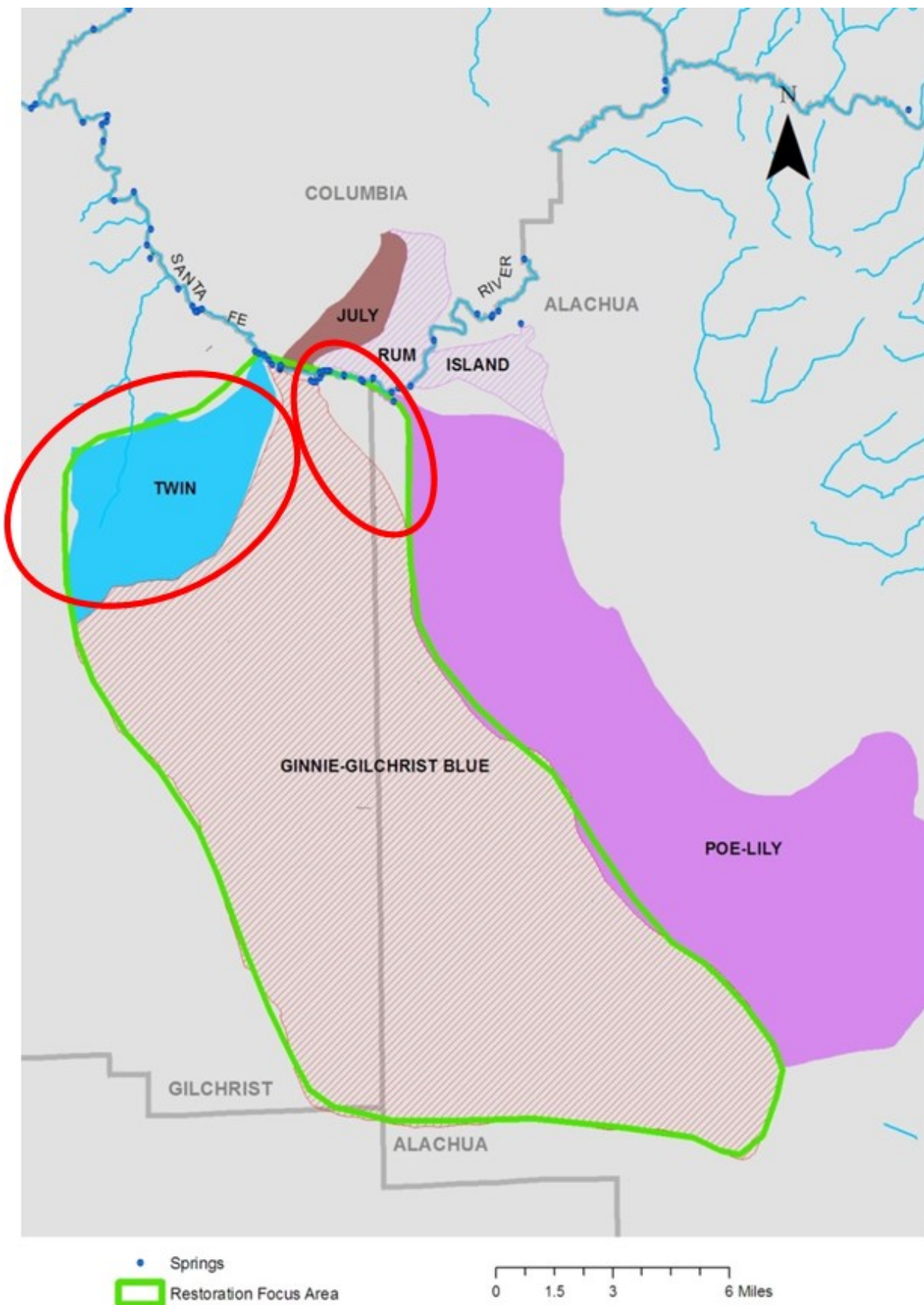
FIGURE 2: SANTA FE RIVER BASIN RFA
