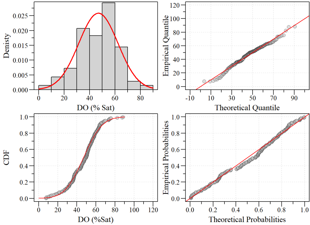
Figure 13. Evaluation of dissolved oxygen empirical and theoretical normal distribution for for only monitoring locations within Cypress Creek (WBID 3235C; see Appendix B ) during the period of record. Top left: Density histogram of the data compared to the theoretical distribution (red line); Top right: quantile-quantile (Q-Q) plot; Bottom left: cumulative distribution function (CDF) relative to theoretical normal distribution CDF (red line); Bottom right: probability-probability (P-P) plot.
